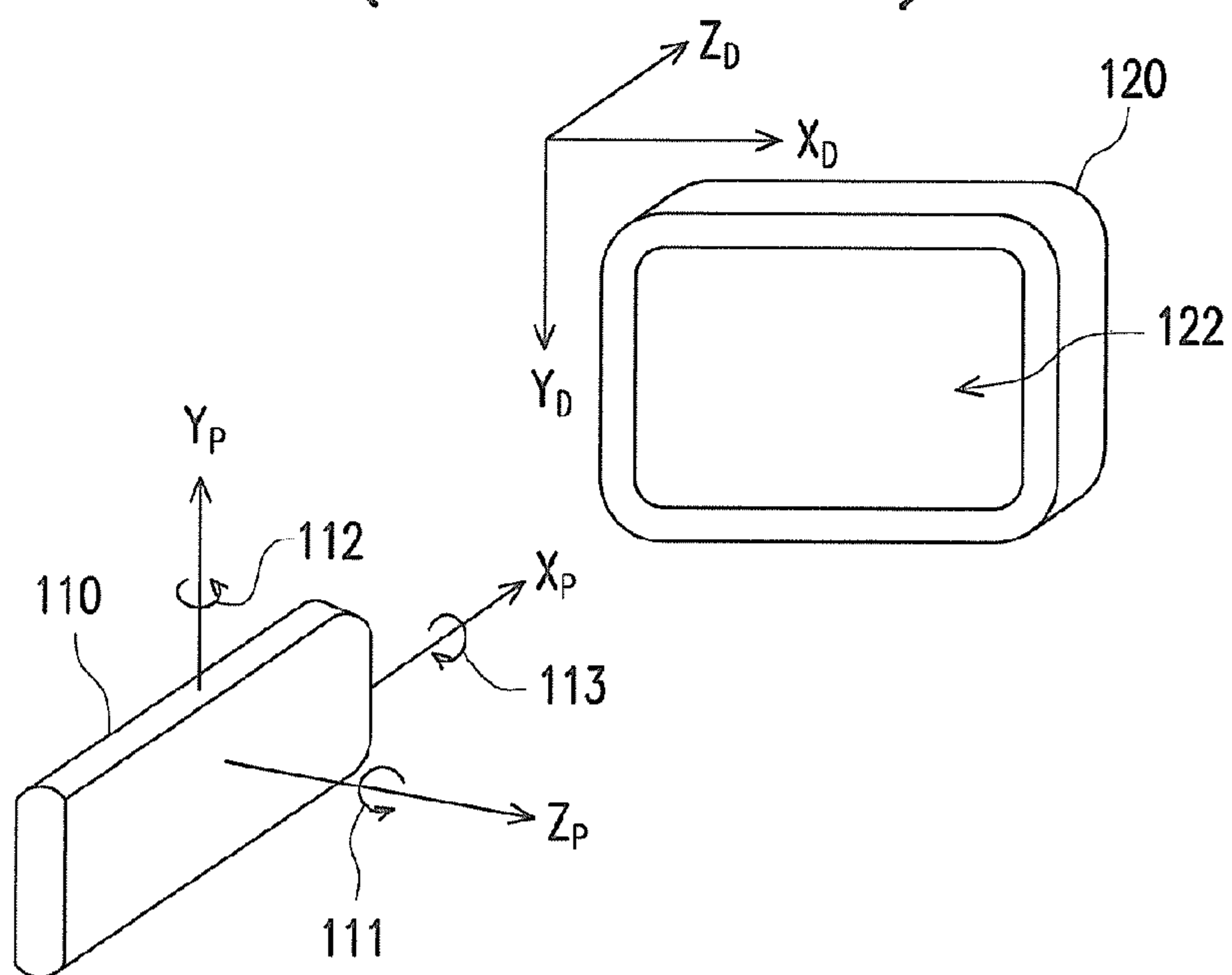
FIG. 1 (RELATED ART)
