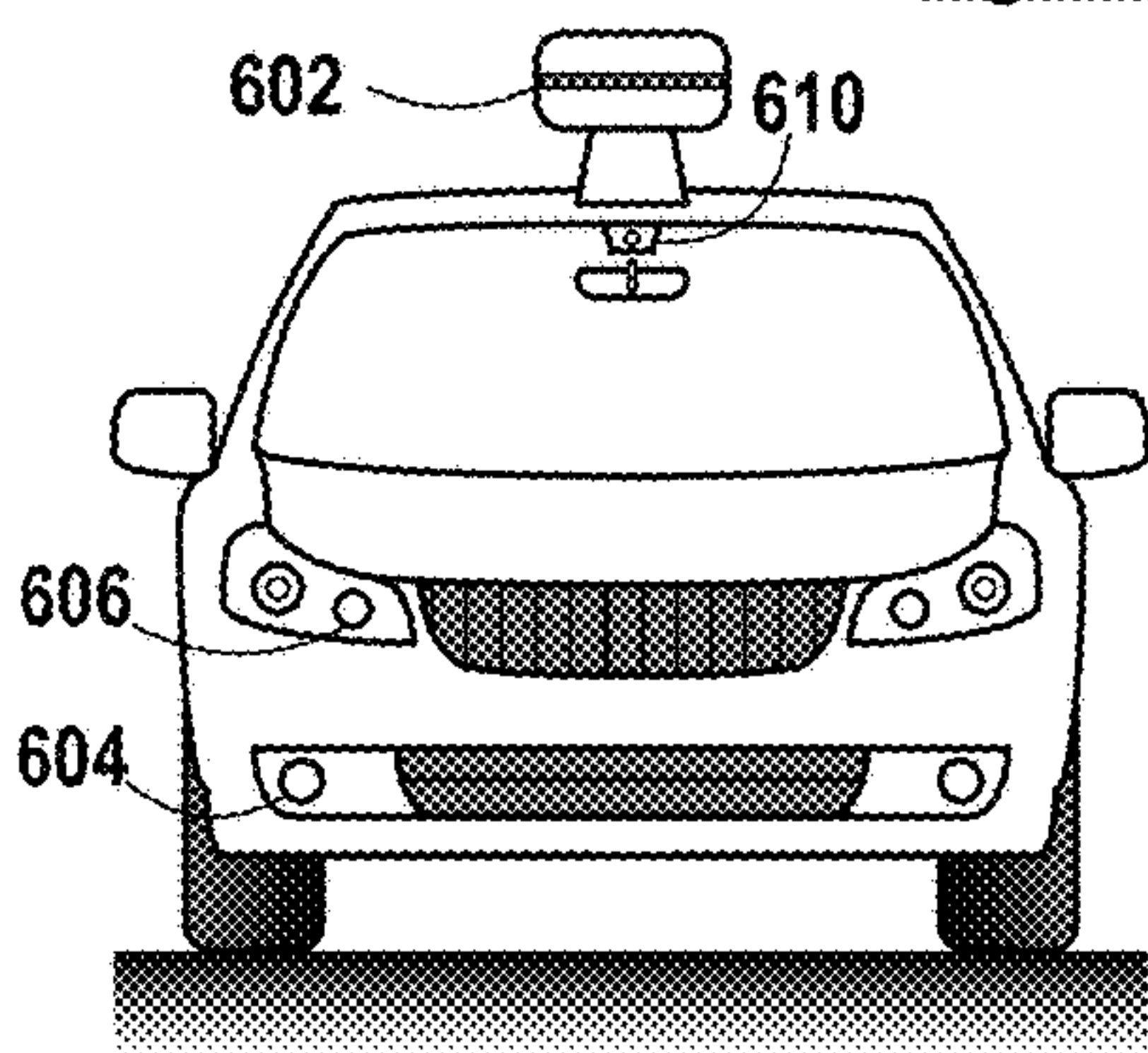
Front View
