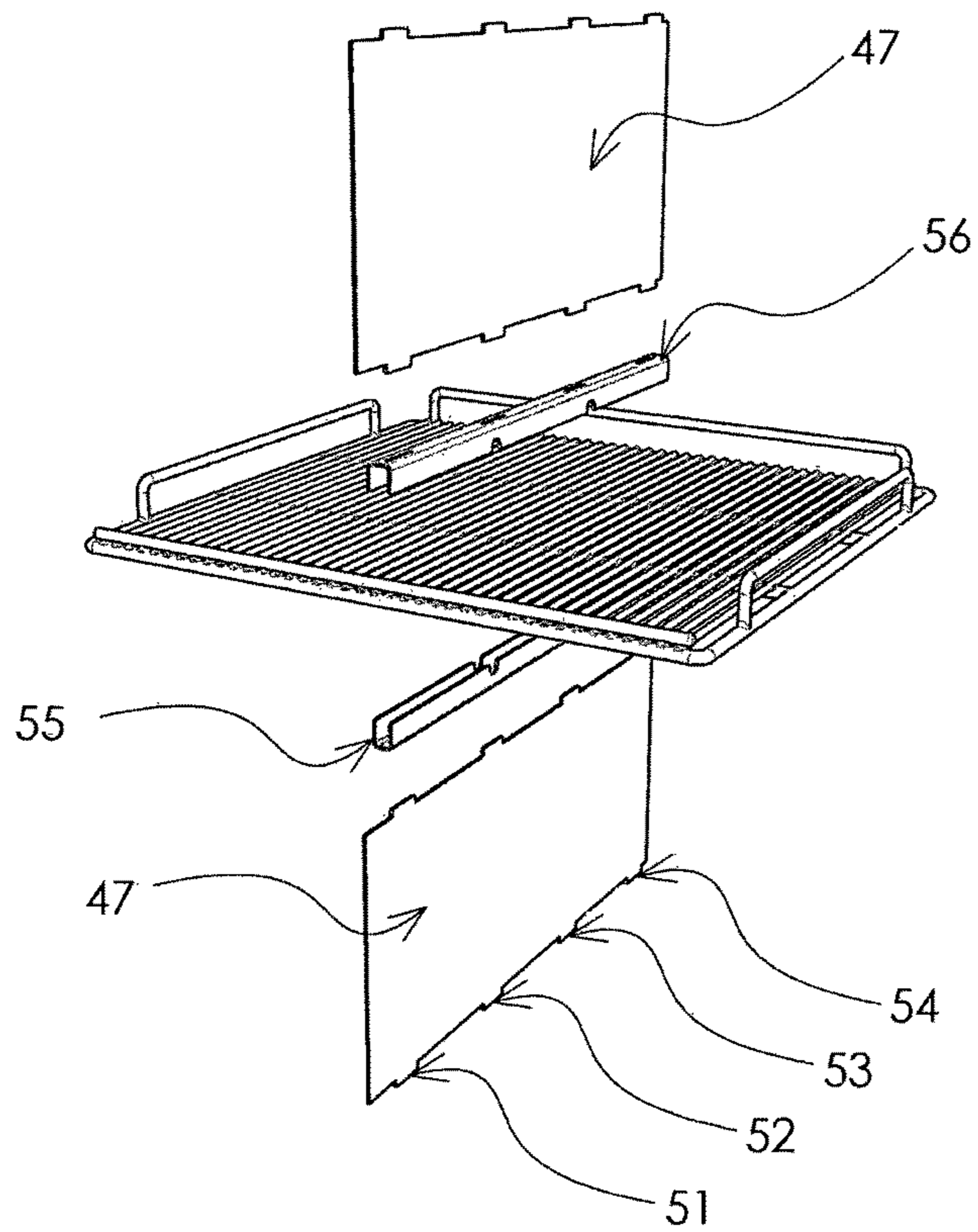
EXPLODED VIEW
