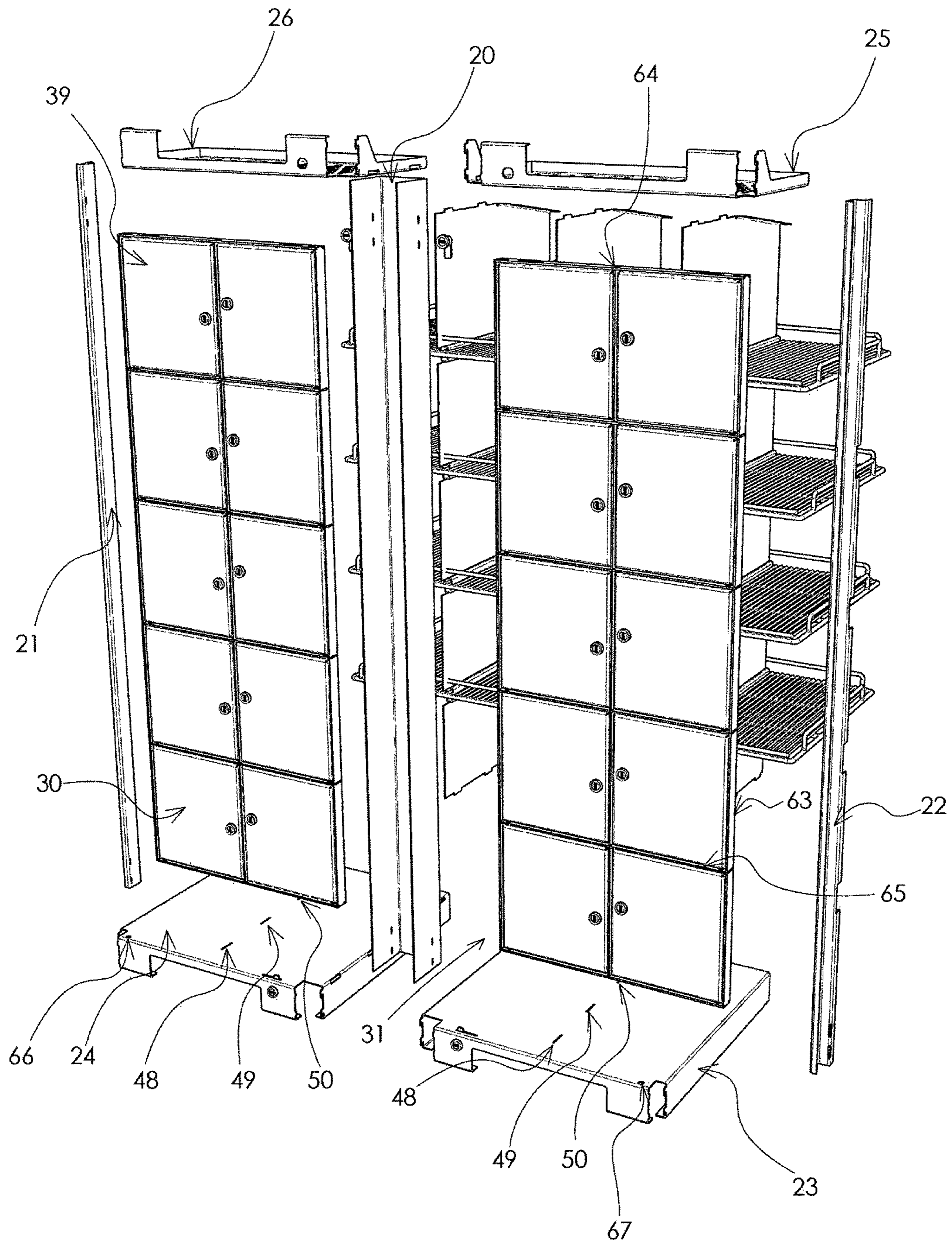
FIGURE 8.
