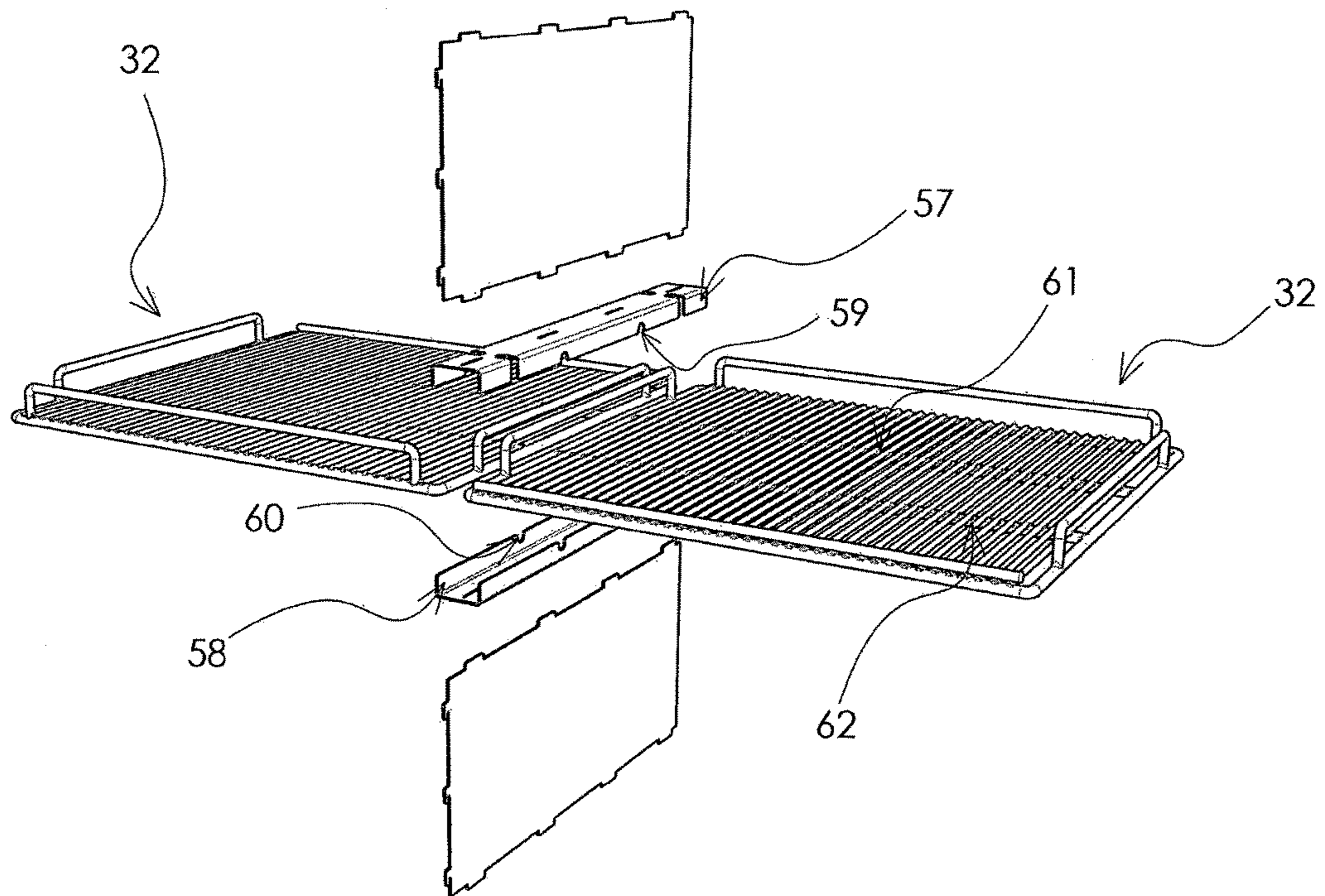
EXPLODED VIEW
