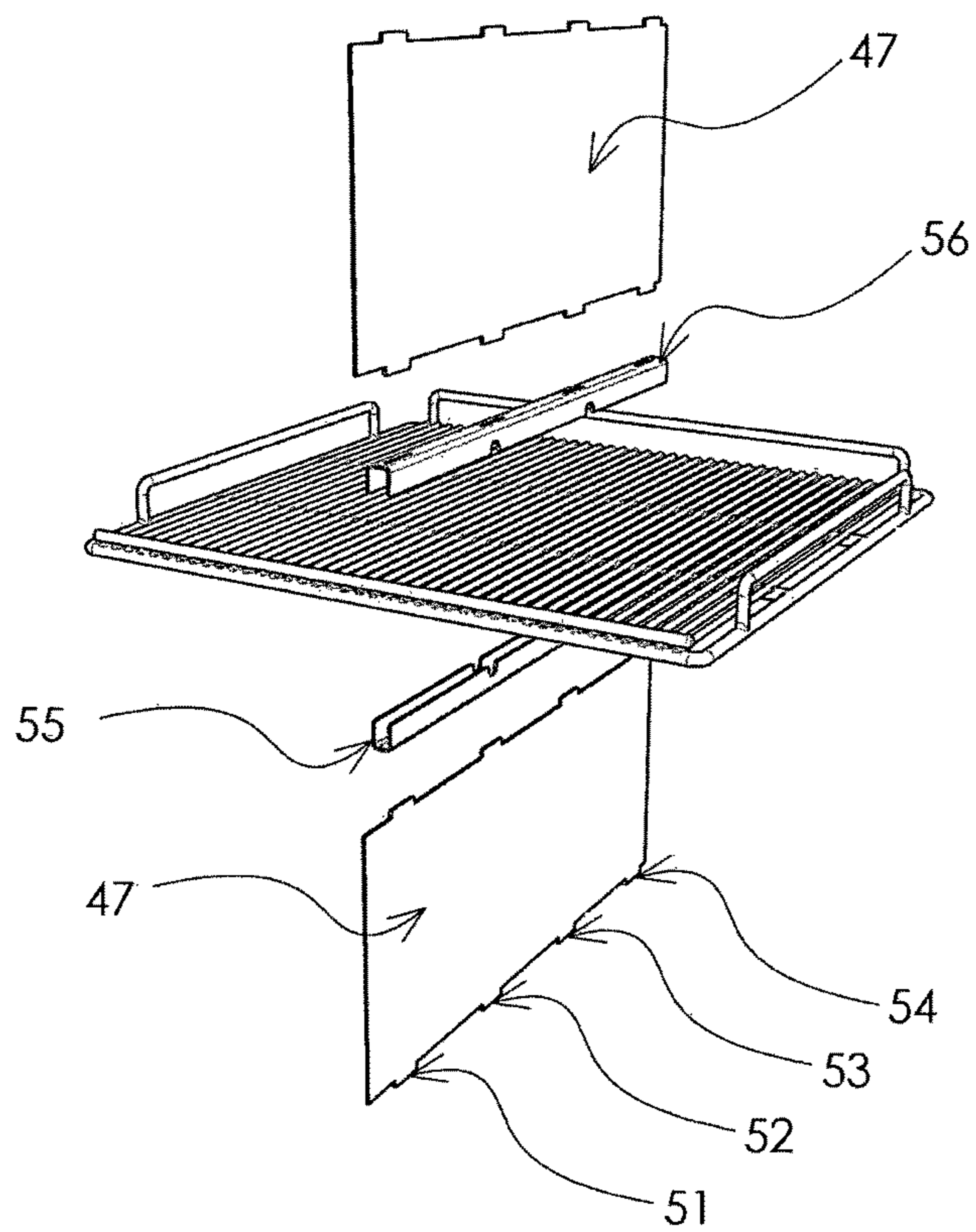
EXPLODED VIEW
