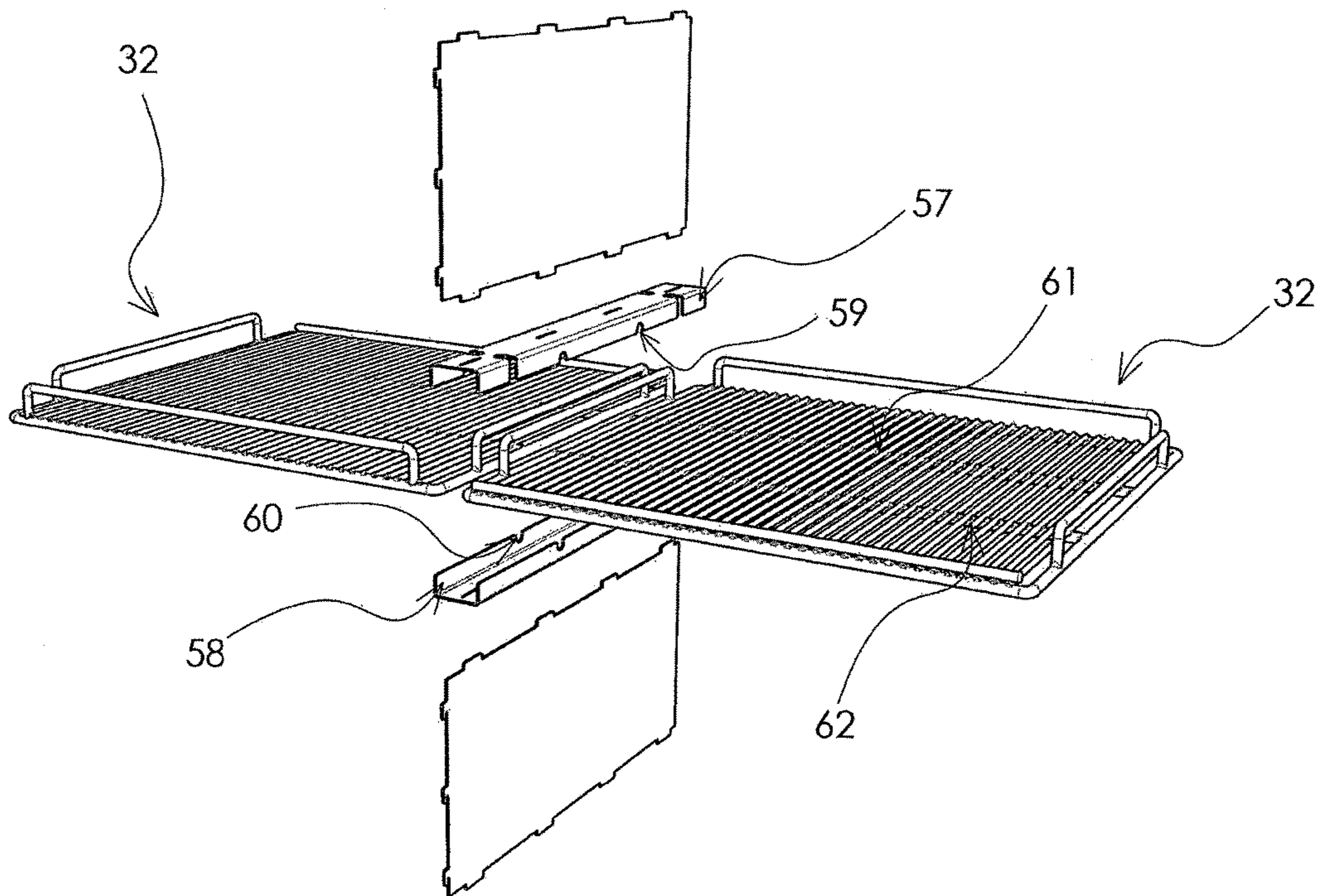
EXPLODED VIEW
