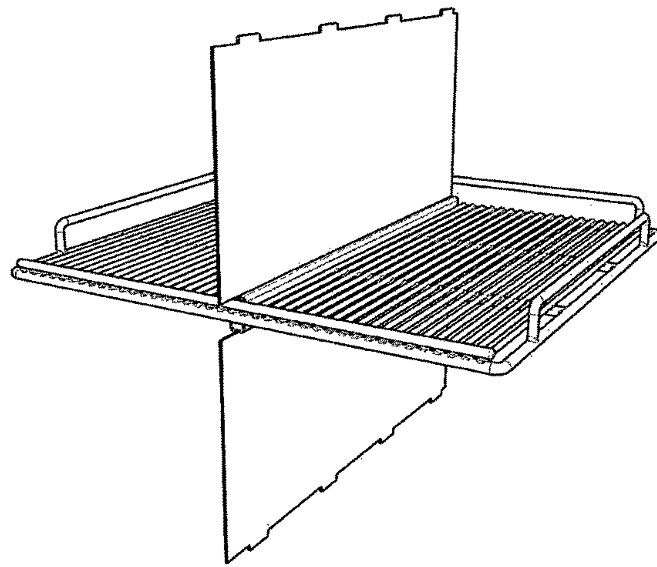
ASSEMBLED VIEW
