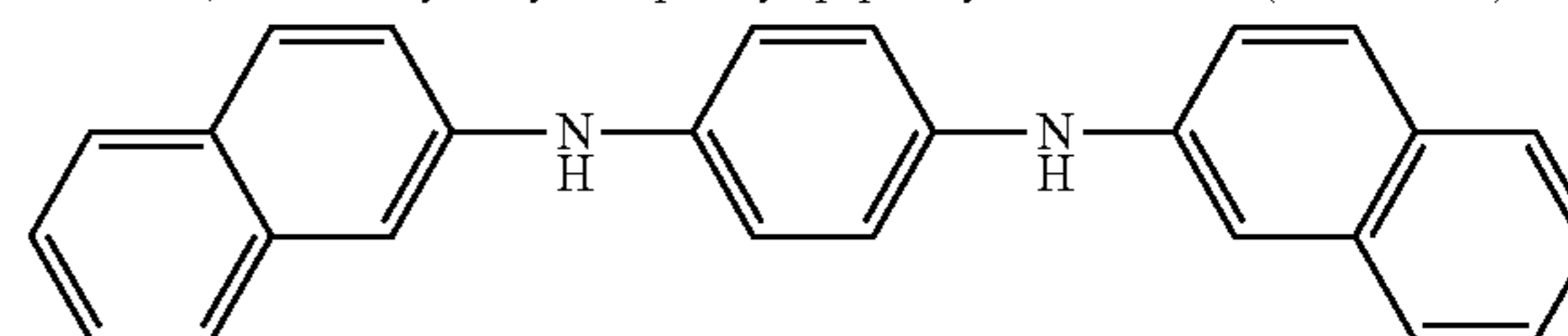
N,N'-Di-2-naphtyl-p-phenylenediamine (DNPD)
