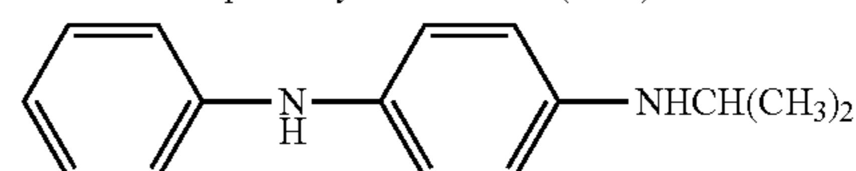
N-Isopropyl-N'-phenyl-p-phenylenediamine (IPPD)
