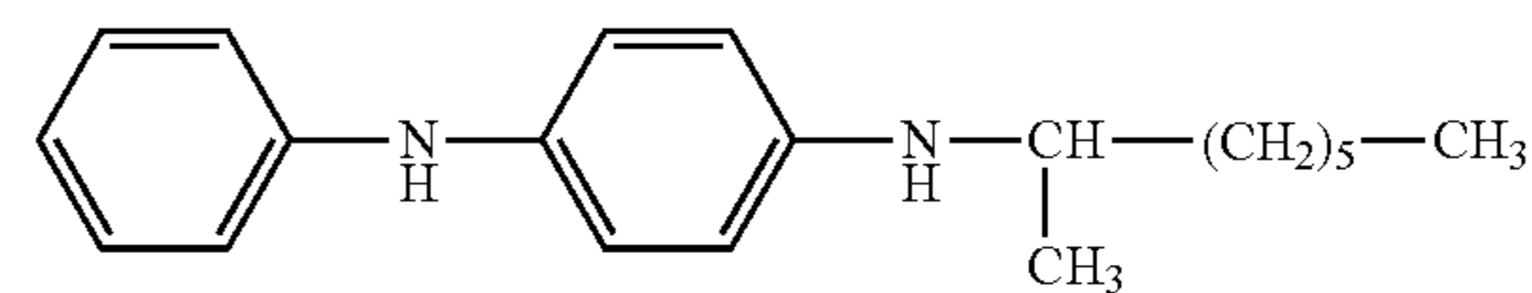
N-(1-Methylheptyl)-N'-phenyl-p-phenylenediamine (MHPPD)
