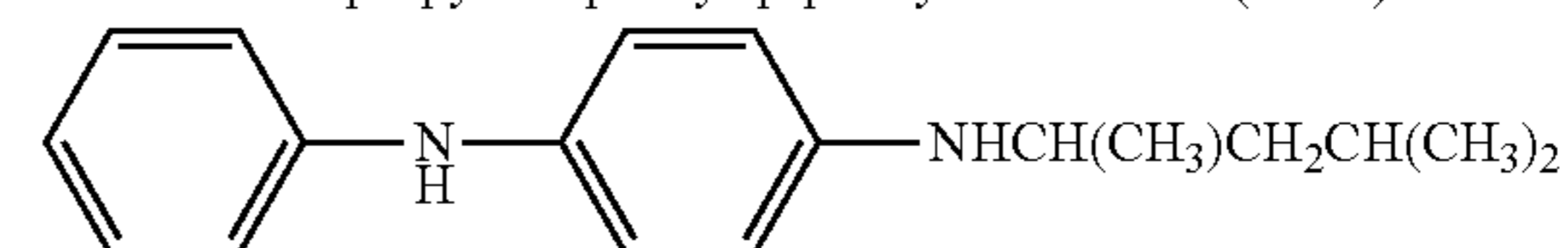
N-1,3-Dimethylbutyl-N'-phenyl-p-phenylenediamine (DMBPPD)
