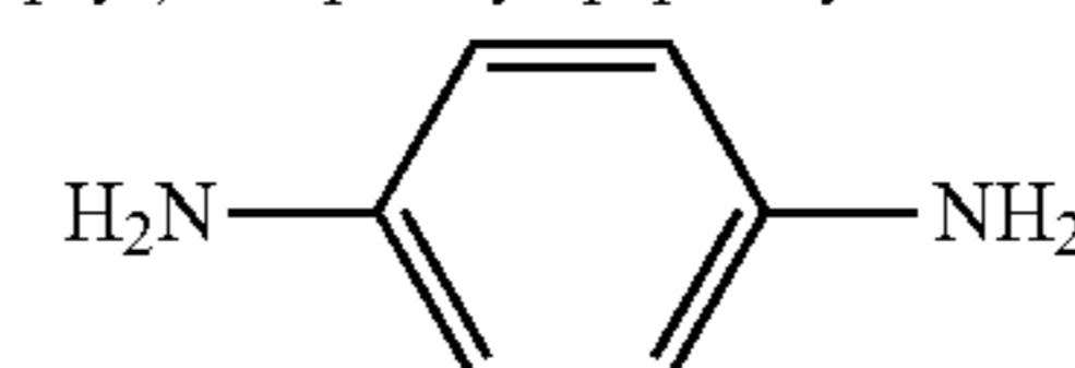
p-Phenylenediamine (PPD)
