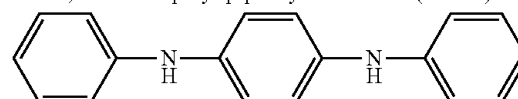
N,N'-Diphenyl-p-phenylenediamine (DPPD)
