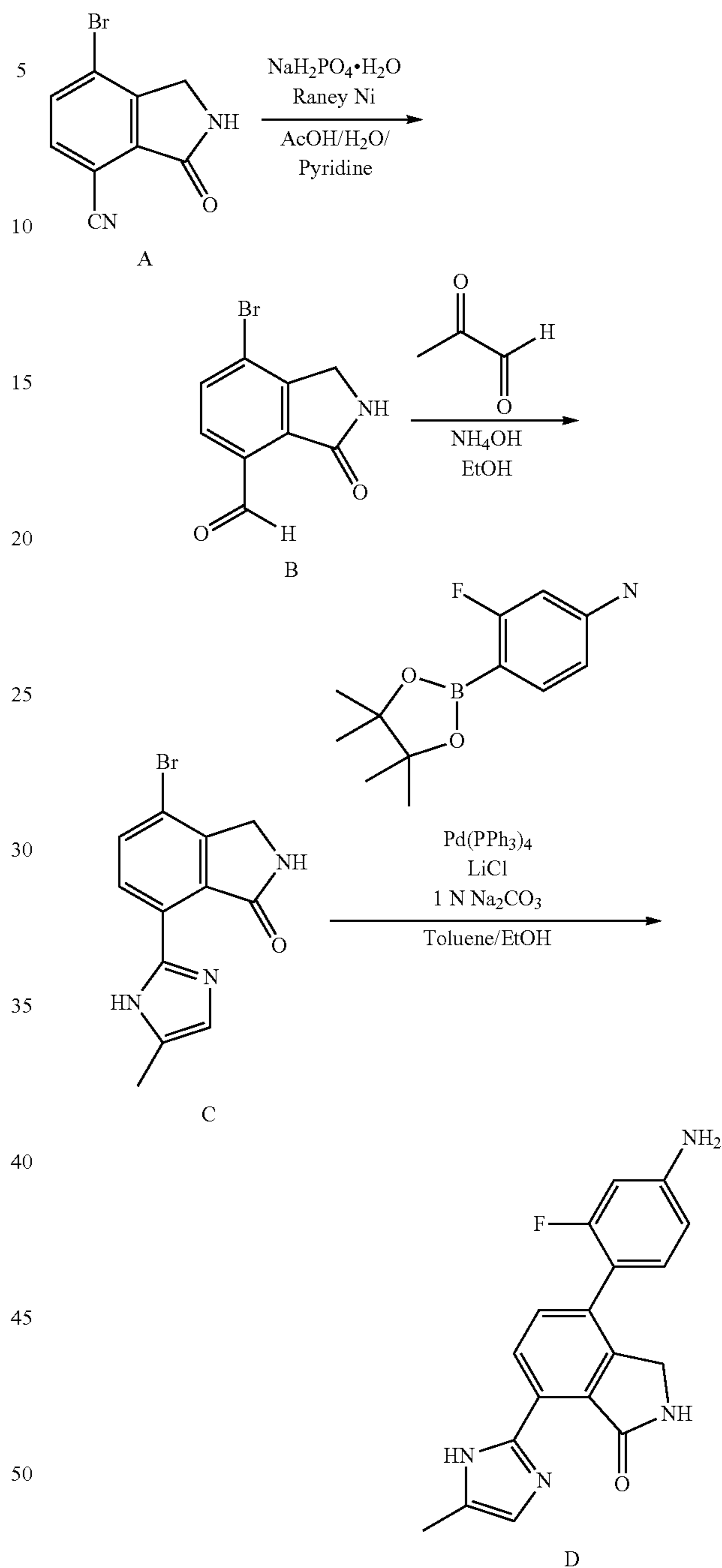
[Reaction Scheme 1]
