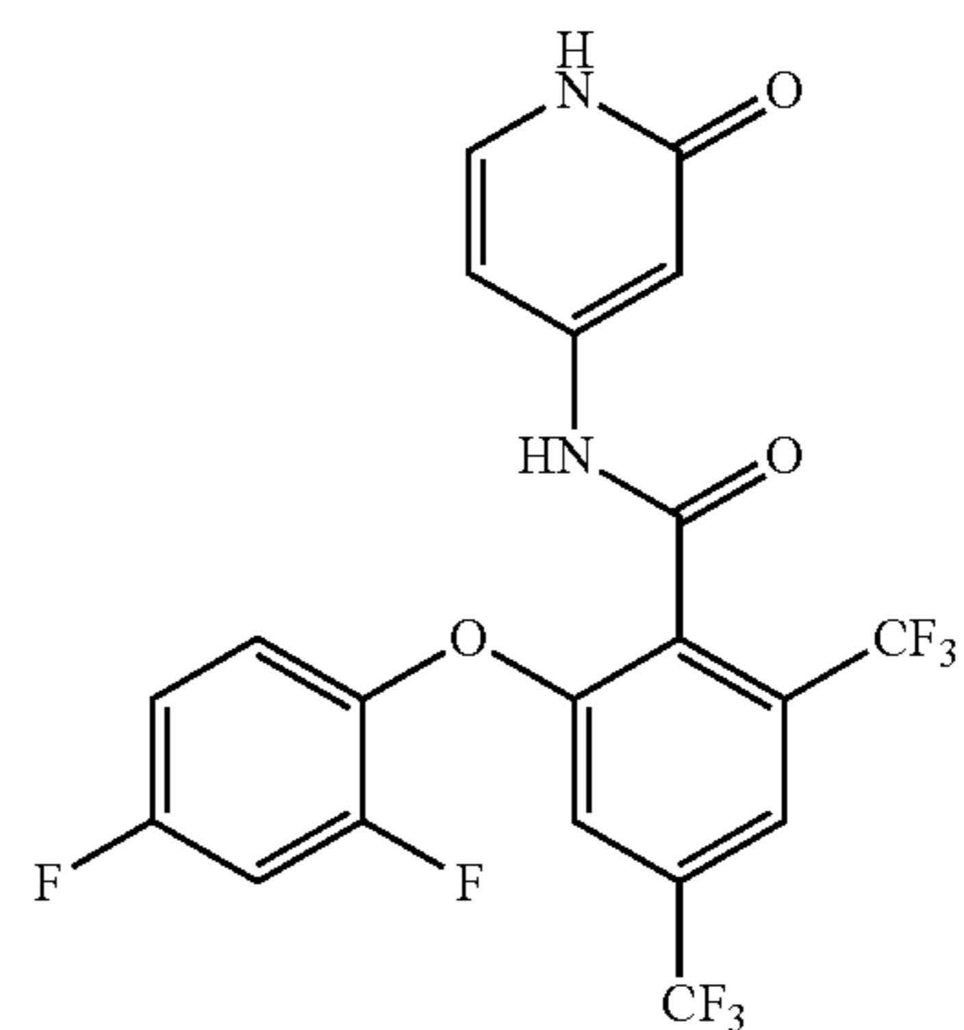
2-(2,4-difluorophenoxy)-N-(2-oxo-1,2-dihydropyridin-4-yl)-4,6-bis(trifluoromethyl)benzamide
