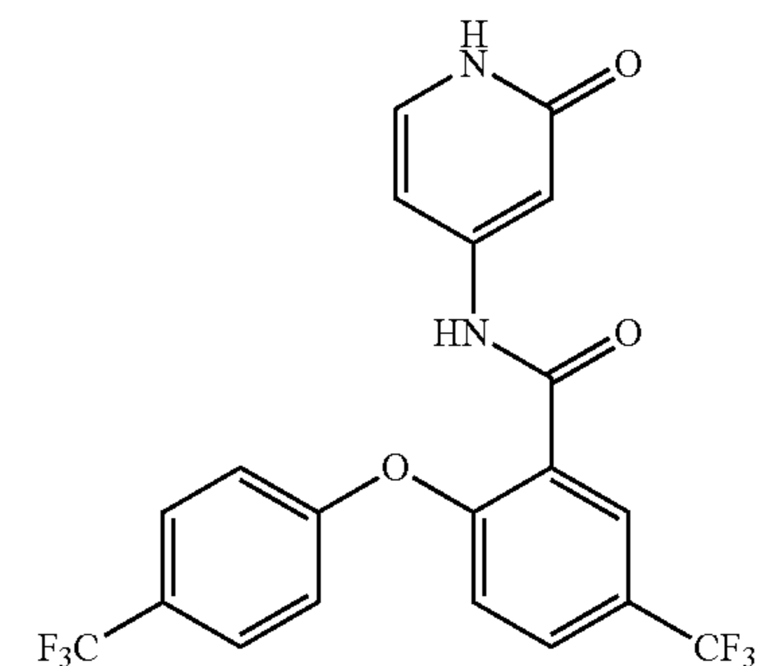
N-(2-oxo-1,2-dihydropyridin-4- yl)-5-(trifluoromethyl)-2-(4- (trifluoromethyl)phenoxy)benzamide
