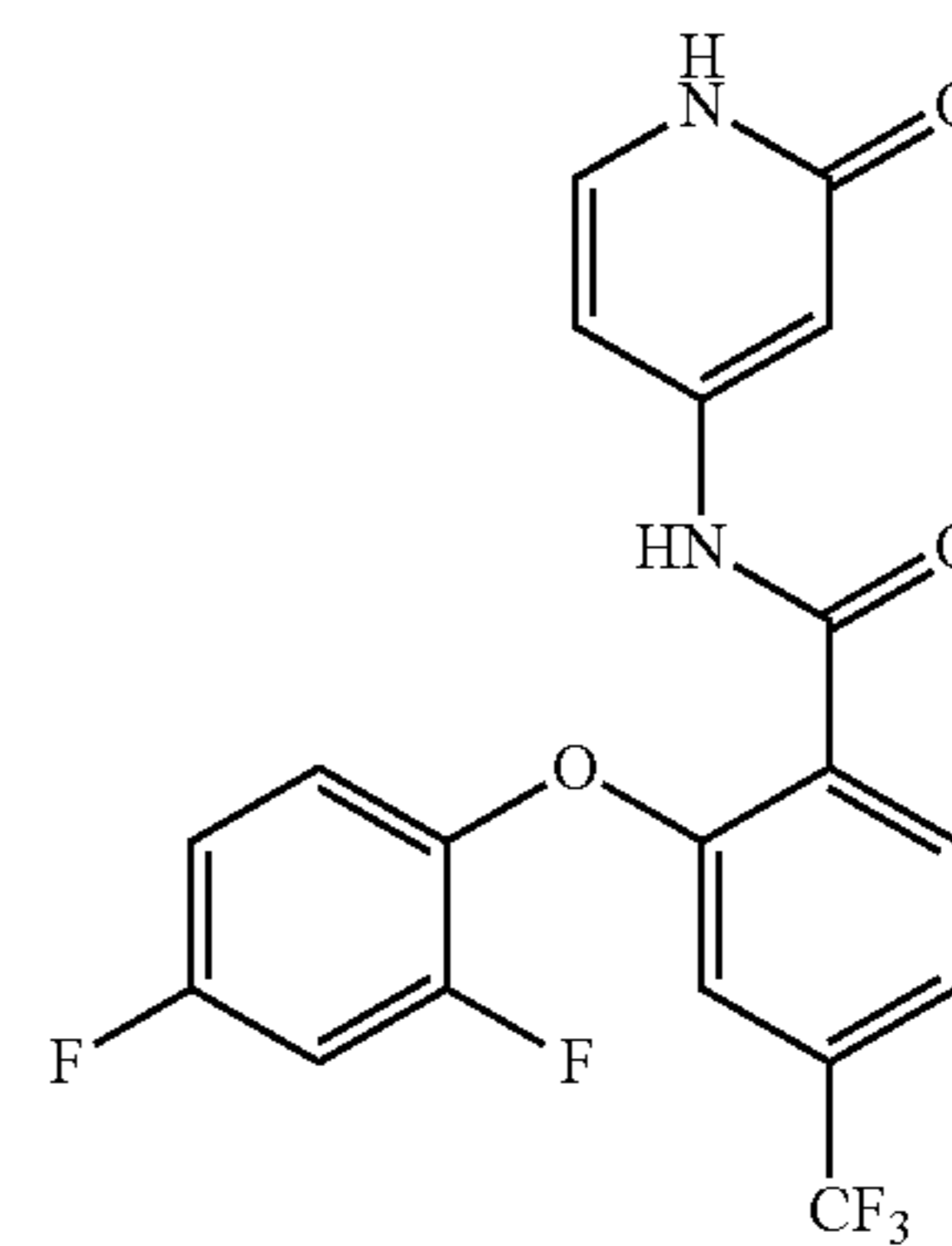
2-(2,4-difluorophenoxy)-N-(2-oxo-1,2-dihydropyridin-4-yl)-4-(trifluoromethyl)benzamide
