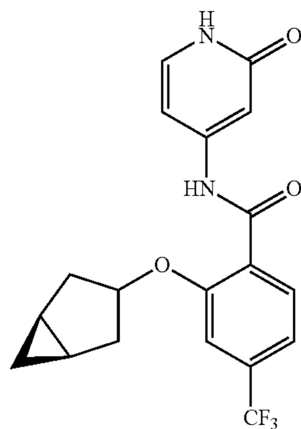
2-((1R,5S)-bicyclo[3.1.0]hexan-3-yloxy)-N-(2-oxo-1,2-dihydropyridin-4-yl)-4-(trifluoromethyl)benzamide
