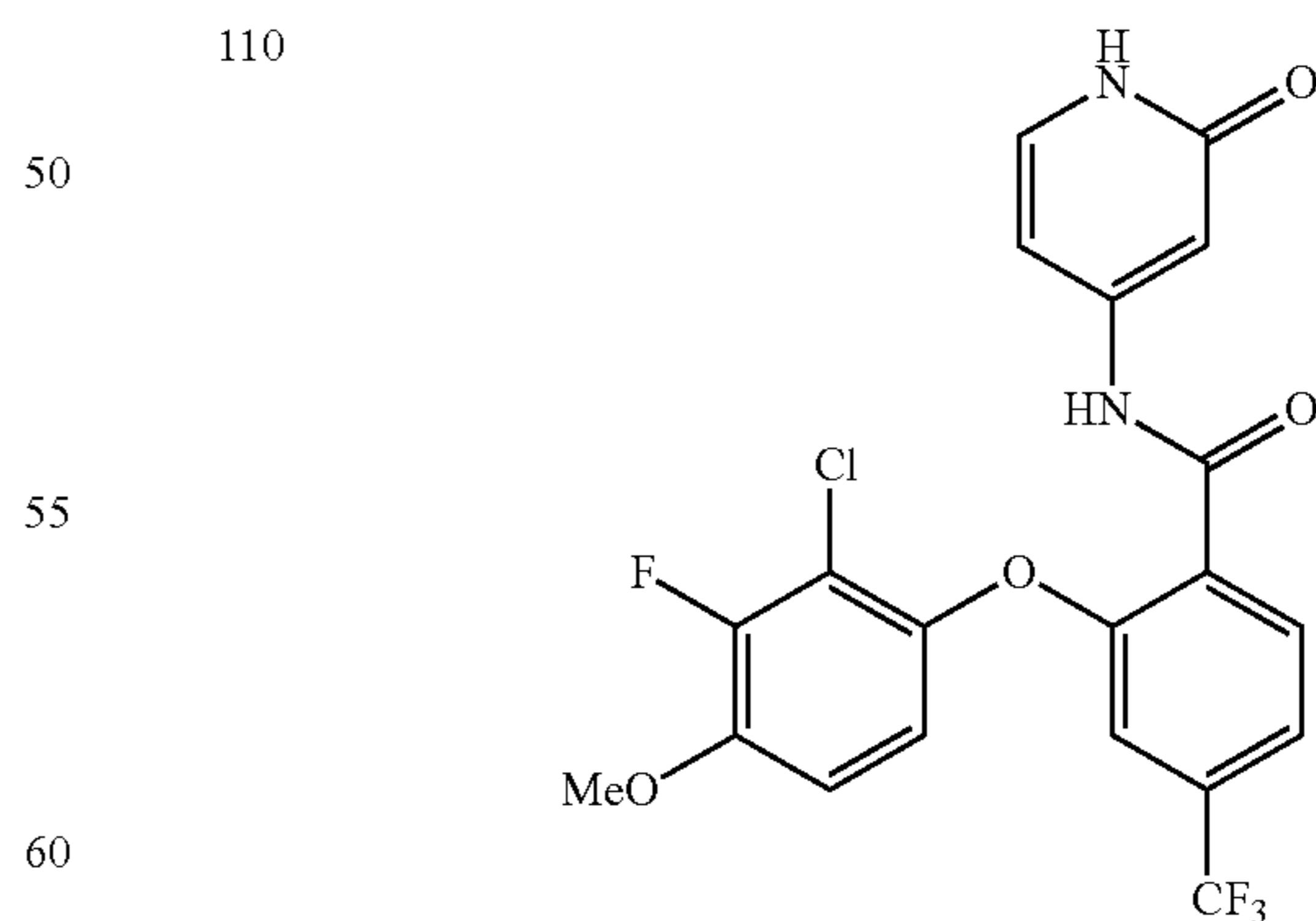
2-(2-chloro-3-fluoro-4-methoxyphenoxy)-N-(2-oxo-1,2-dihydropyridin-4-yl)-4-(trifluoromethyl)benzamide
