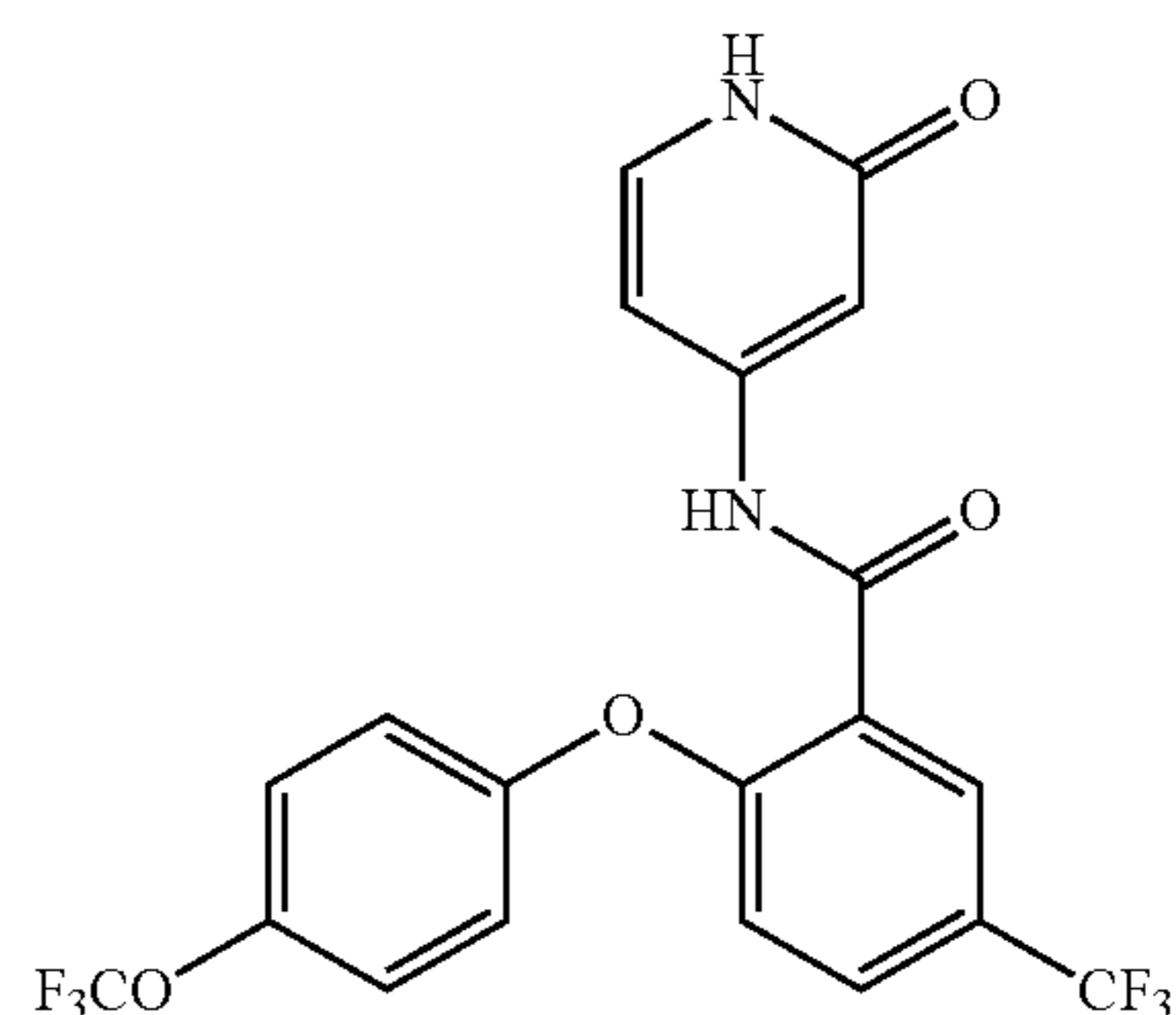
N-(2-oxo-1,2-dihydropyridin-4- yl)-2-(4- (trifluoromethoxy)phenoxy)-5- (trifluoromethyl)benzamide
