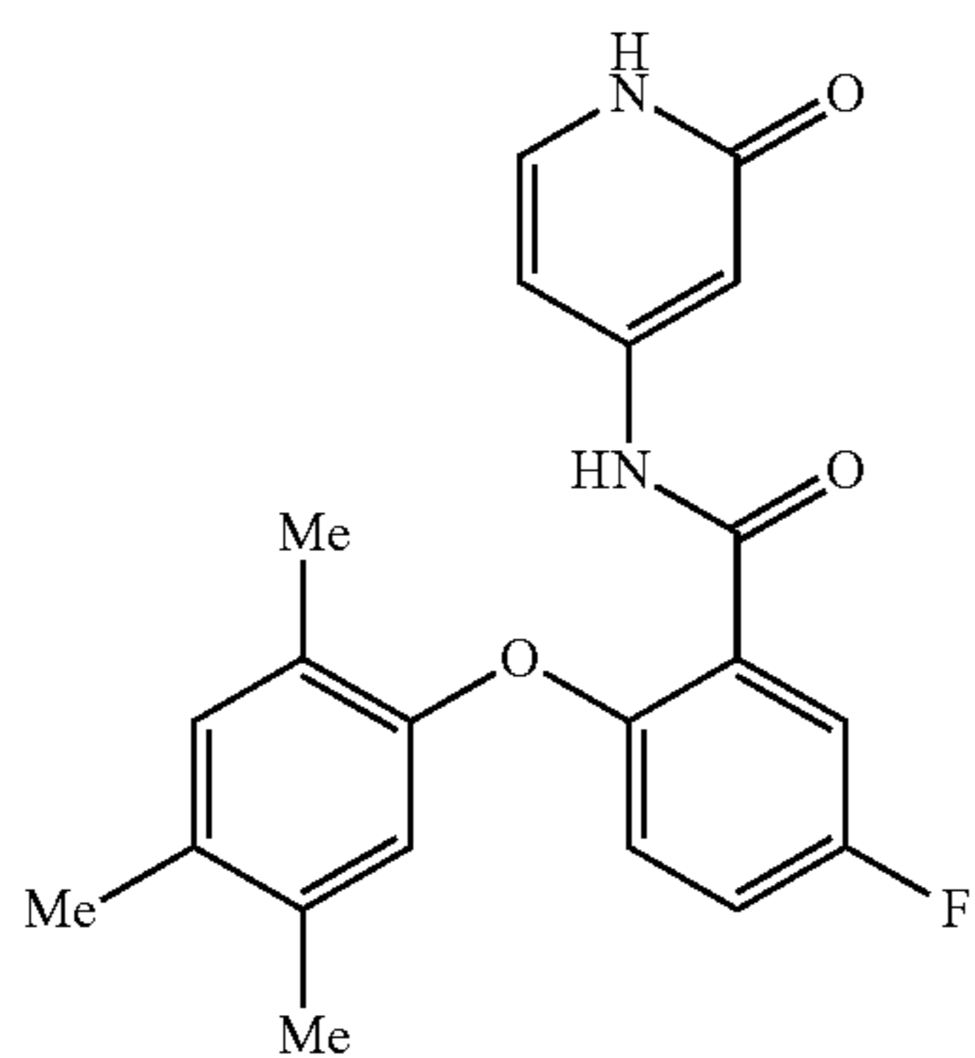
5-fluoro-N-(2-oxo-1,2-dihydropyridin-4-yl)-2-(2,4,5-trimethylphenoxy)benzamide
