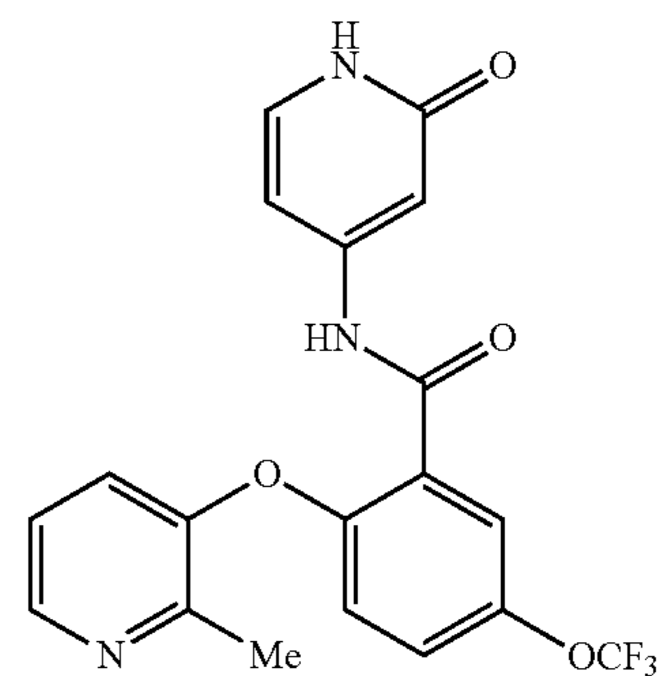
2-((2-methylpyridin-3-yl)oxy)-N-(2-oxo-1,2-dihydropyridin-4-yl)-5-(trifluoromethoxy)benzamide
