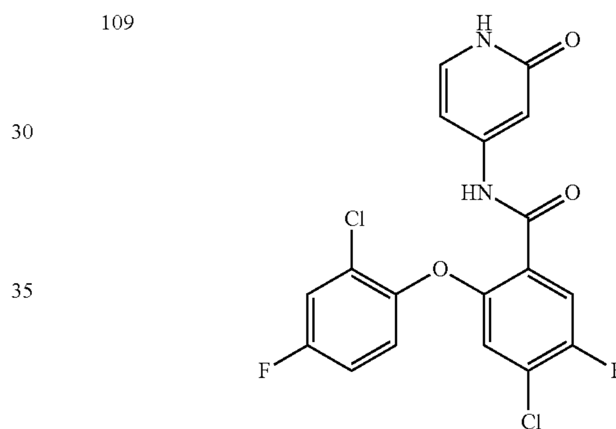
4-chloro-2-(2-chloro-4-fluorophenoxy)-5-fluoro-N-(2-oxo-1,2-dihydropyridin-4-yl)benzamide
