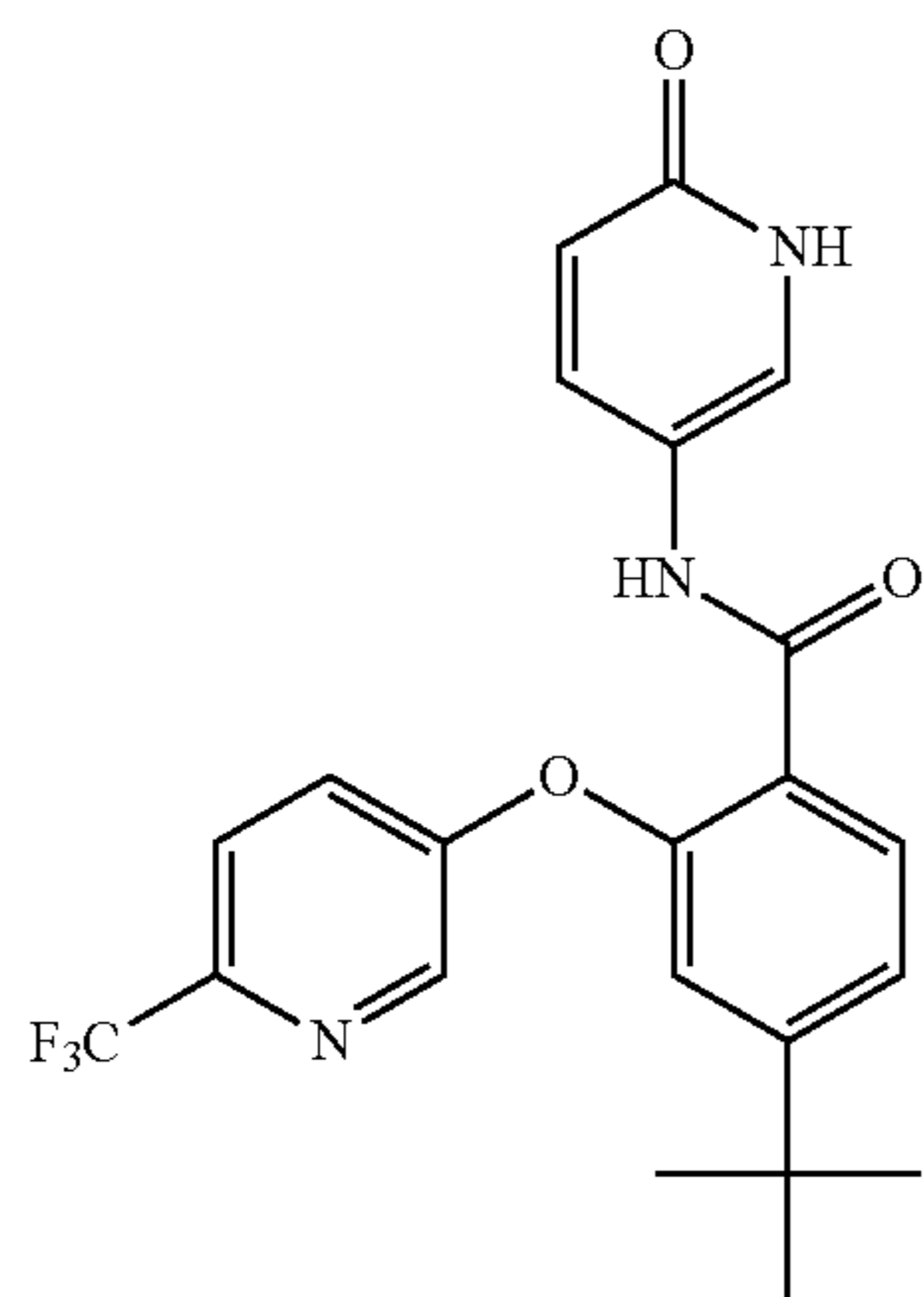
4-(tert-butyl)-N-(6-oxo-1,6-dihydropyridin-3-yl)-2-((6-(trifluoromethyl)pyridin-3-yl)oxy)benzamide
