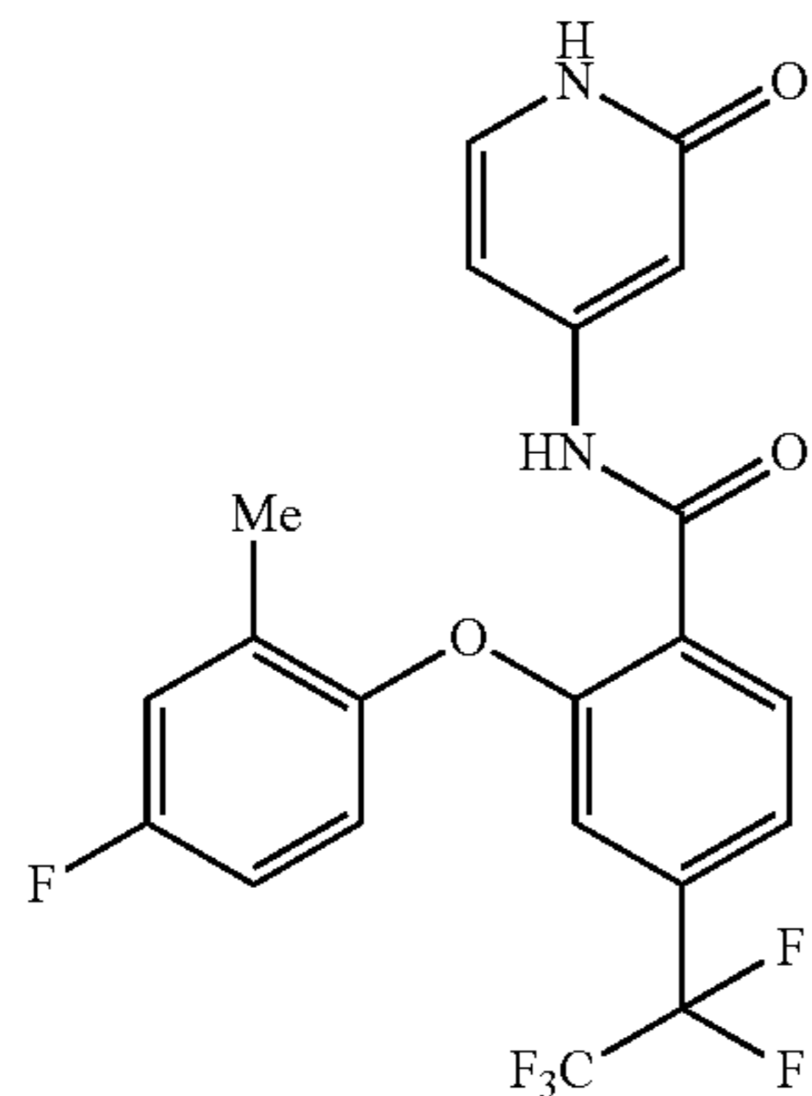
2-(4-fluoro-2-methylphenoxy)-N-(2-oxo-1,2-dihydropyridin-4-yl)-4-(perfluoroethyl)benzamide
