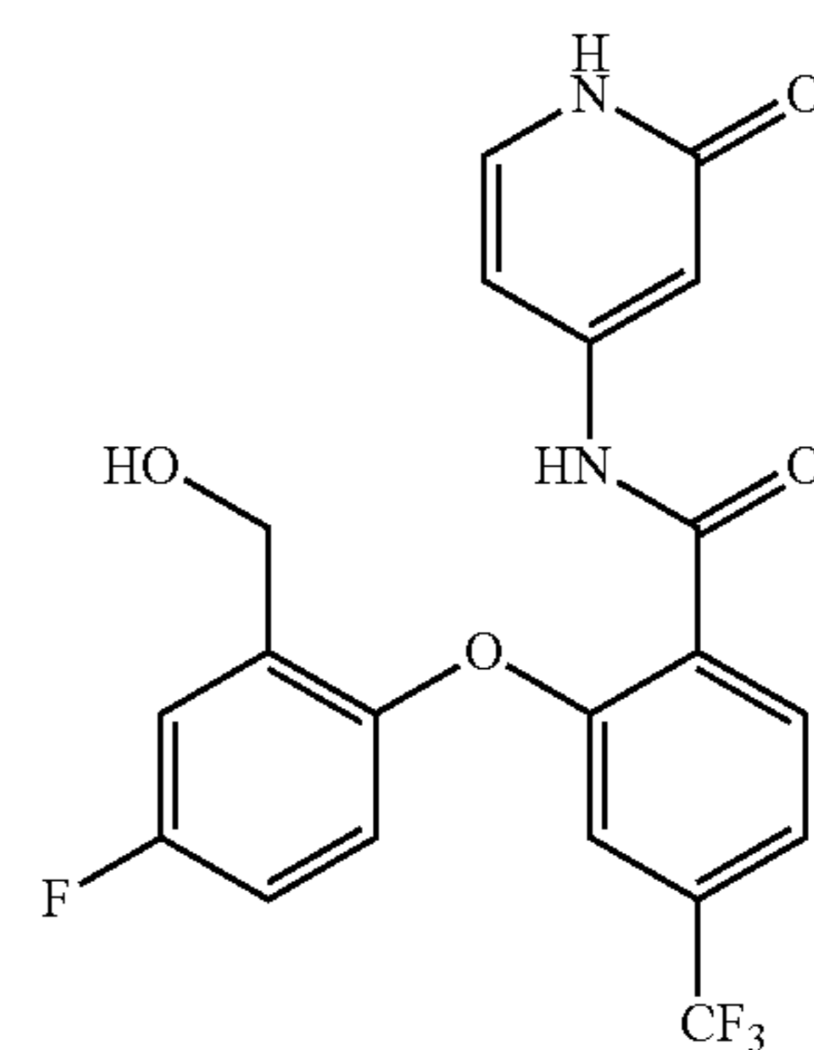
2-(4-fluoro-2-(hydroxymethyl)phenoxy)-N-(2-oxo-1,2-dihydropyridin-4-yl)-4,6-bis(trifluoromethyl)benzamide
