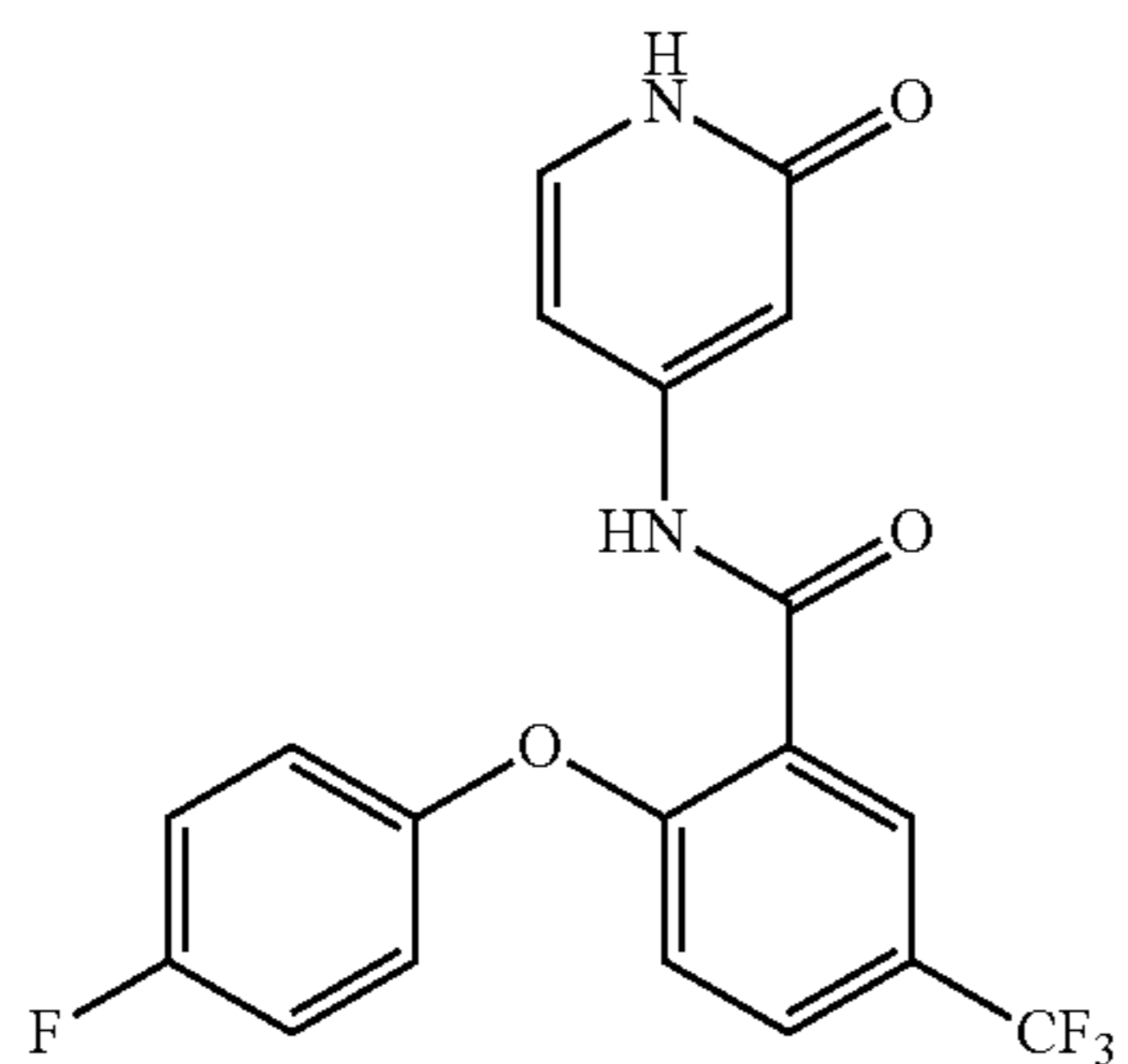
2-(4-fluorophenoxy)-N-(2-oxo-1,2-dihydropyridin-4-yl)-5-(trifluoromethyl)benzamide
