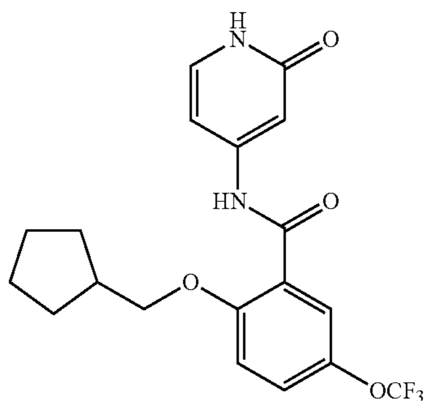
2-(cyclopentylmethoxy)-N-(2-oxo-1,2-dihydropyridin-4-yl)-5-(trifluoromethoxy)benzamide
