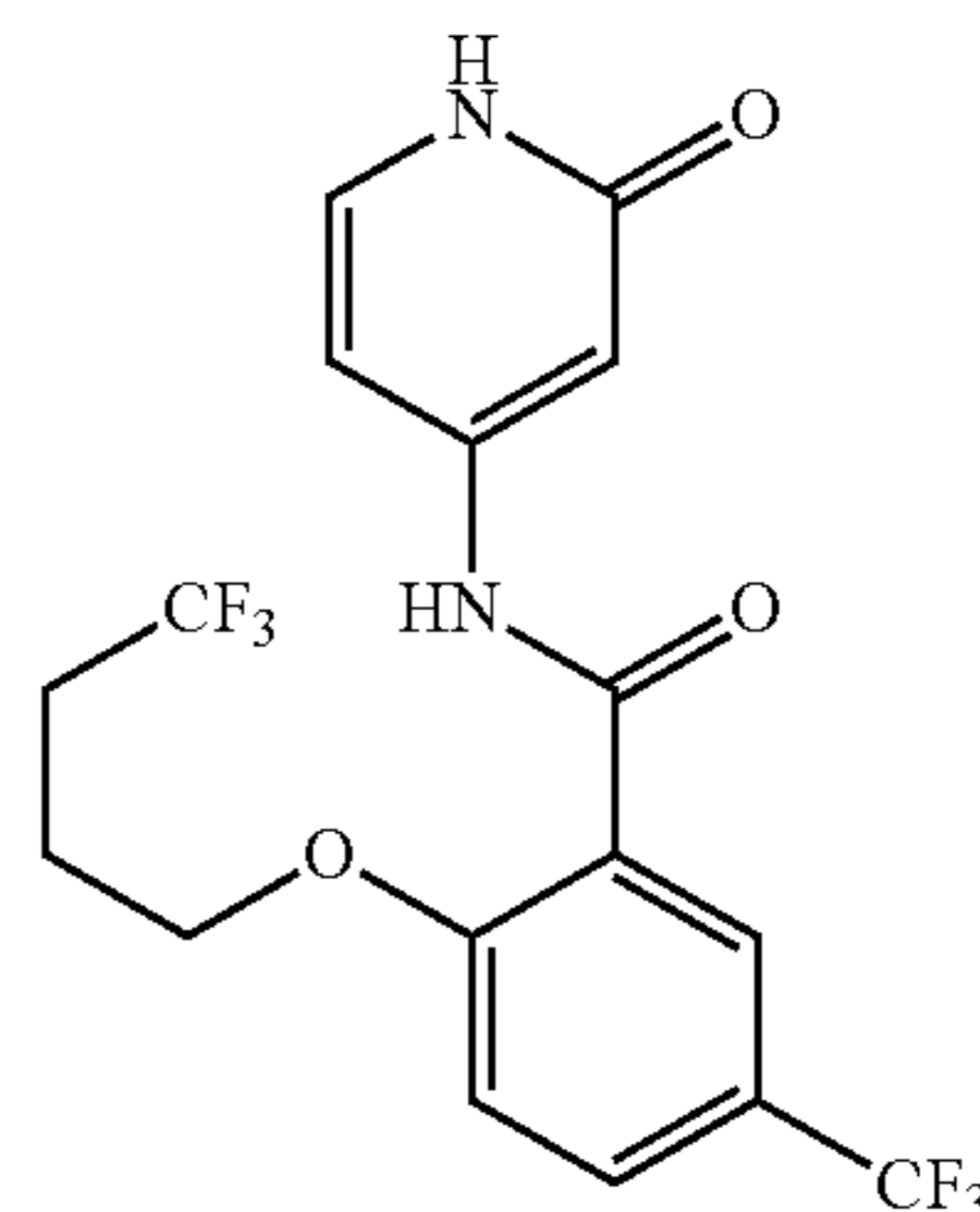
N-(2-oxo-1,2-dihydropyridin-4-yl)-2-(4,4,4-trifluorobutoxy)-5-(trifluoromethyl)benzamide
