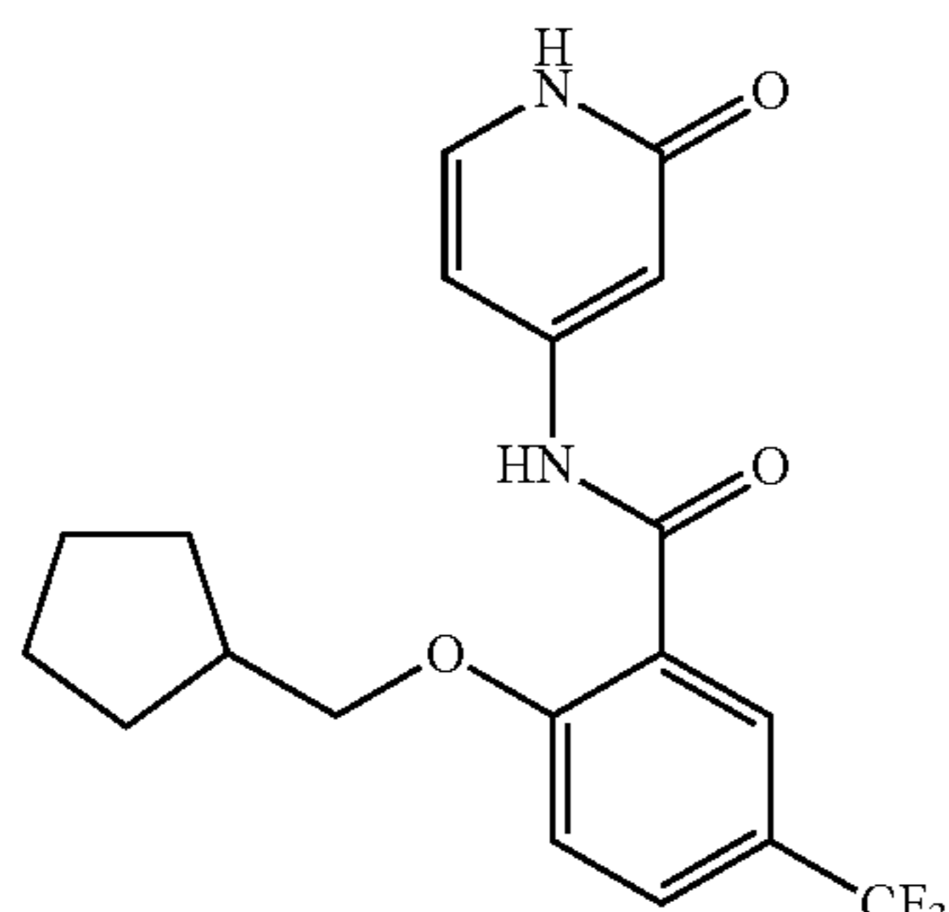
2-(cyclopentylmethoxy)-N-(2-oxo-1,2-dihydropyridin-4-yl)-5-(trifluoromethyl)benzamide
