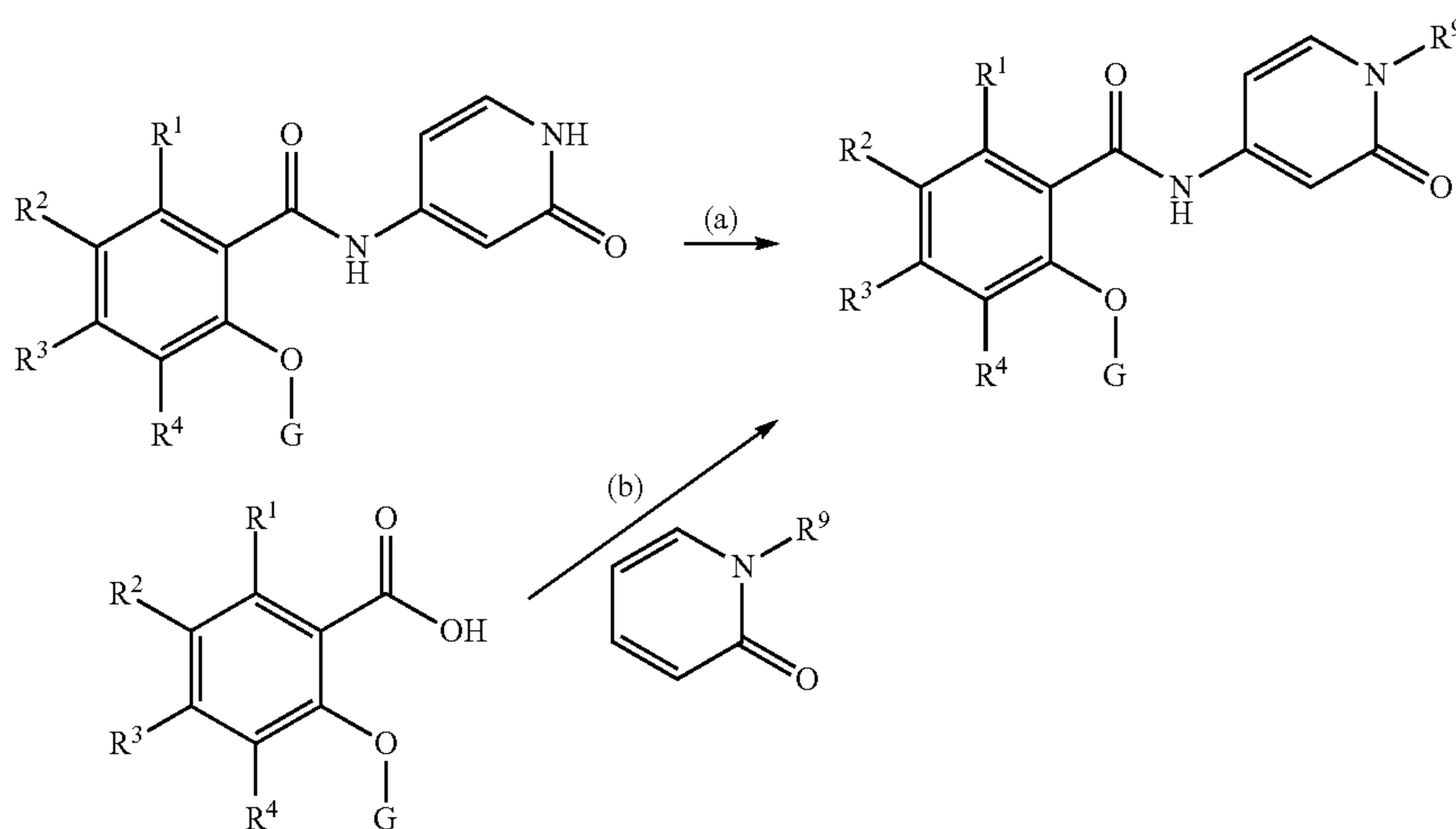
Scheme 3: General Preparation of Compounds of Formula I
