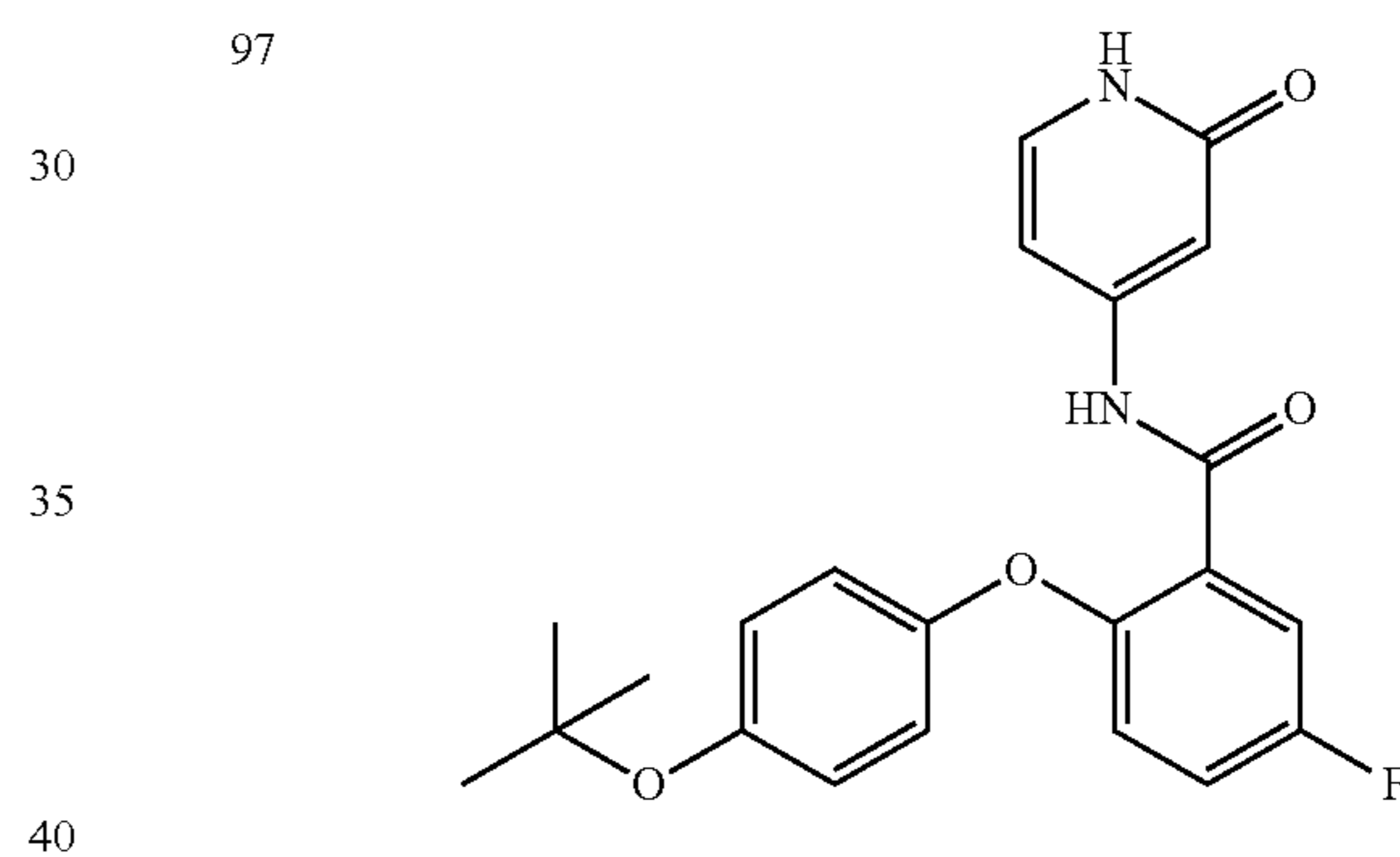
2-(4-(tert-butoxy)phenoxy)-5-fluoro-N-(2-oxo-1,2-dihydropyridin-4-yl)benzamide
