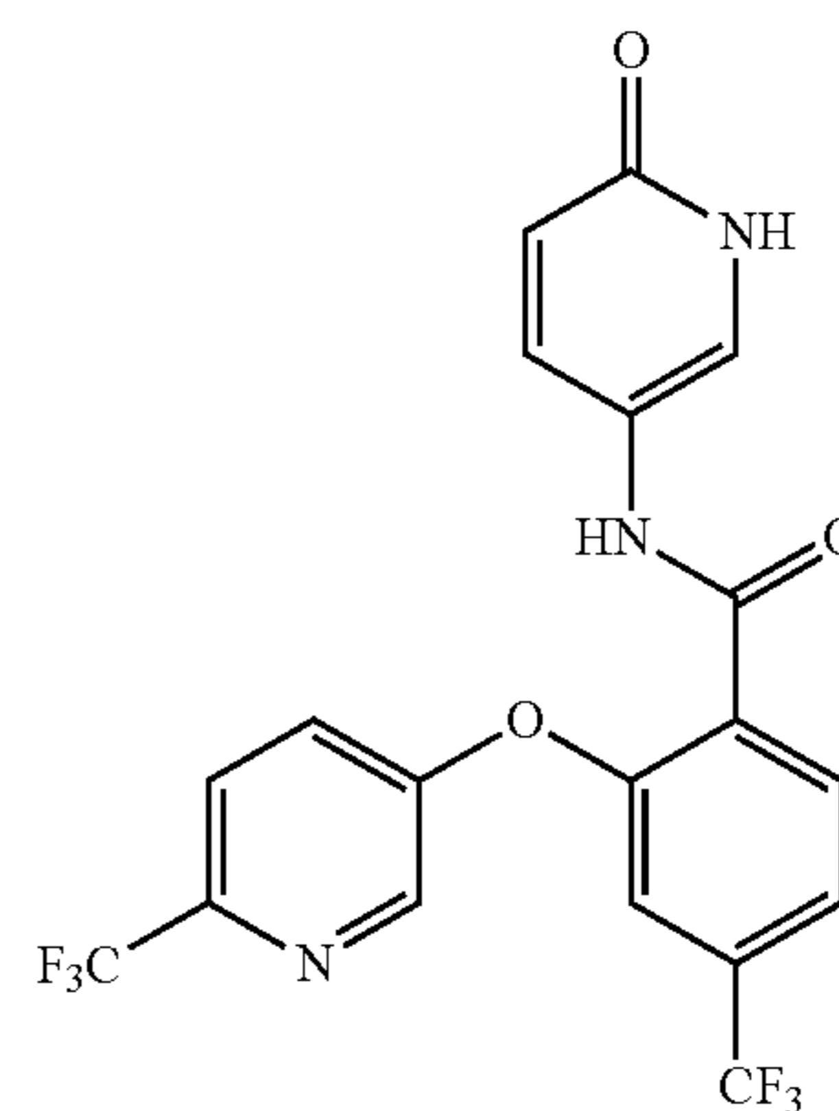
N-(6-oxo-1,6-dihydropyridin-3-yl)-4-(trifluoromethyl)-2-((6-(trifluoromethyl)pyridin-3-yl)oxy)benzamide
