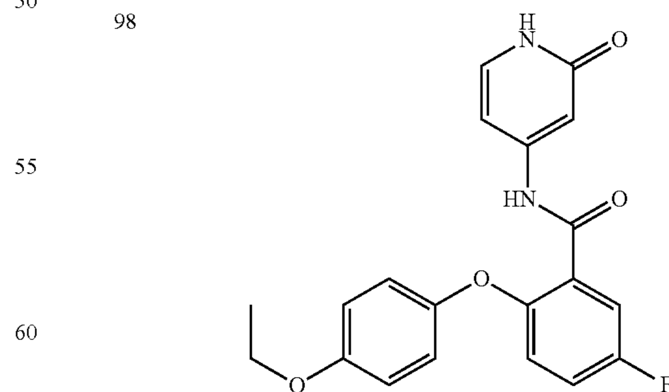
2-(4-ethoxyphenoxy)-5-fluoro-N-(2-oxo-1,2-dihydropyridin-4-yl)benzamide
