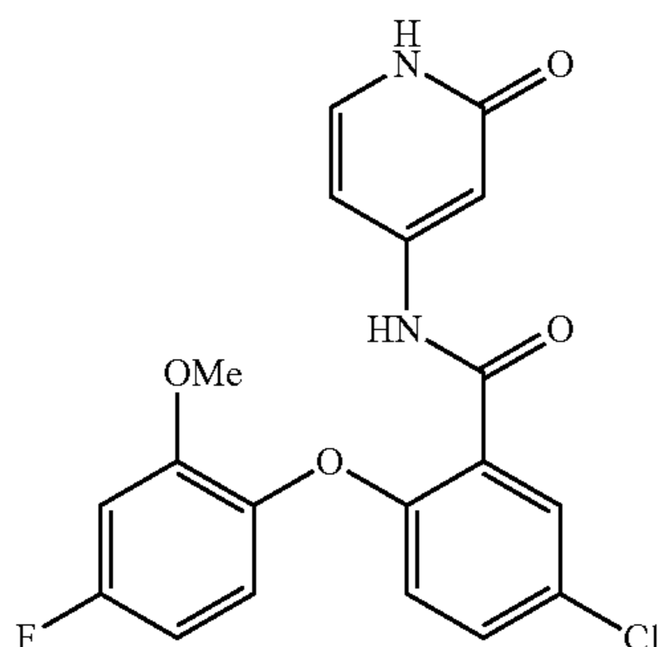
5-chloro-2-(4-fluoro-2- methoxyphenoxy)-N-(2-oxo-1,2- dihydropyridin-4-yl)benzamide
