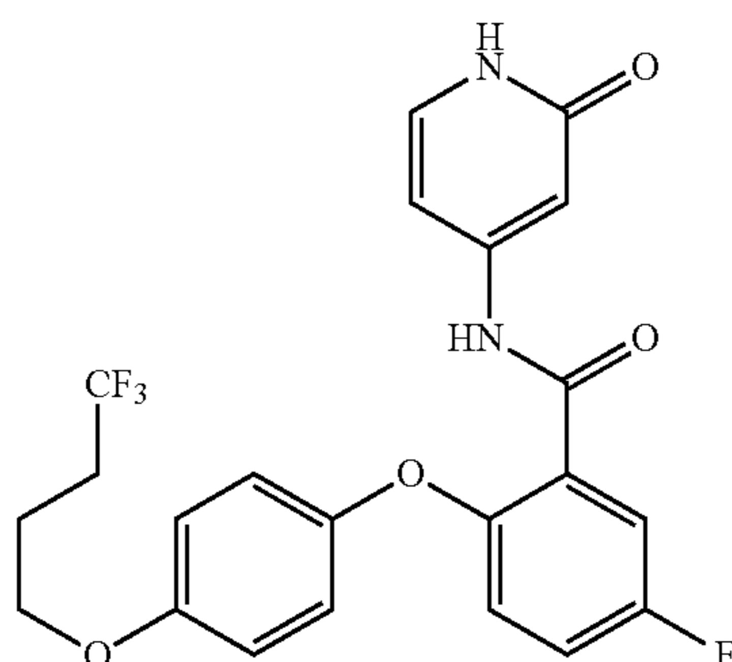
5-fluoro-N-(2-oxo-1,2-dihydropyridin-4-yl)-2-(4-(4,4,4-trifluorobutoxy)phenoxy)benzamide
