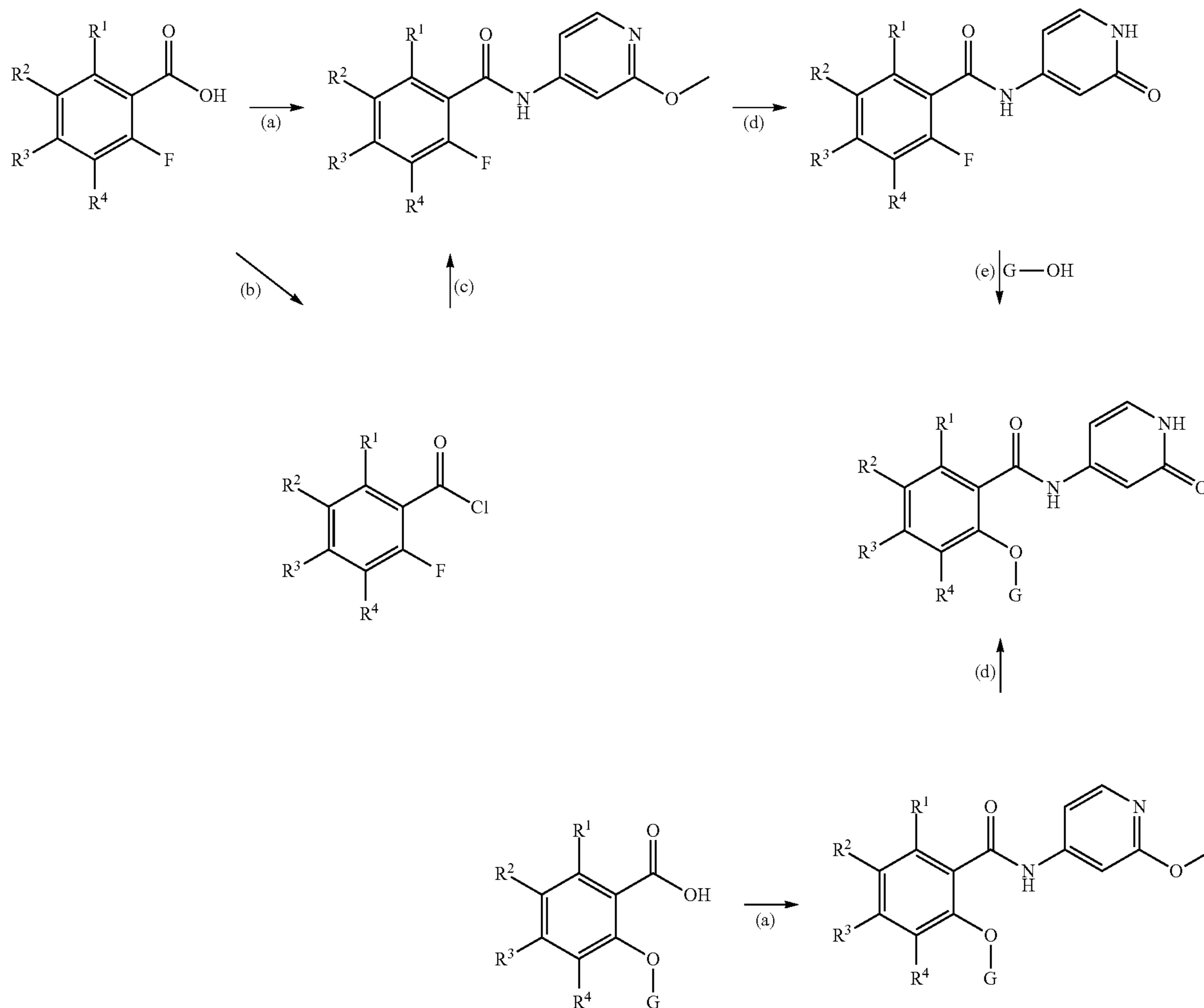
Scheme 1: General Preparation of Compounds of Formula I
