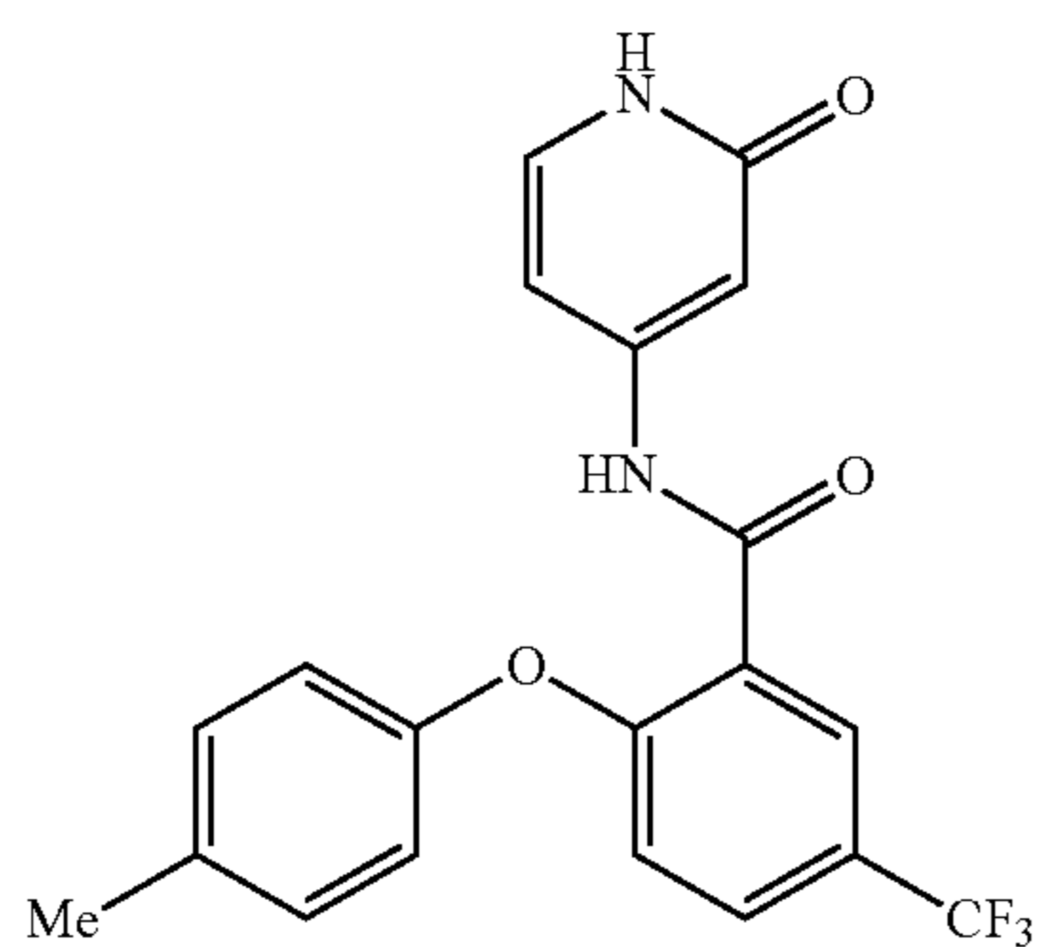
N-(2-oxo-1,2-dihydropyridin-4-yl)-2-(p-tolyloxy)-5-(trifluoromethyl)benzamide
