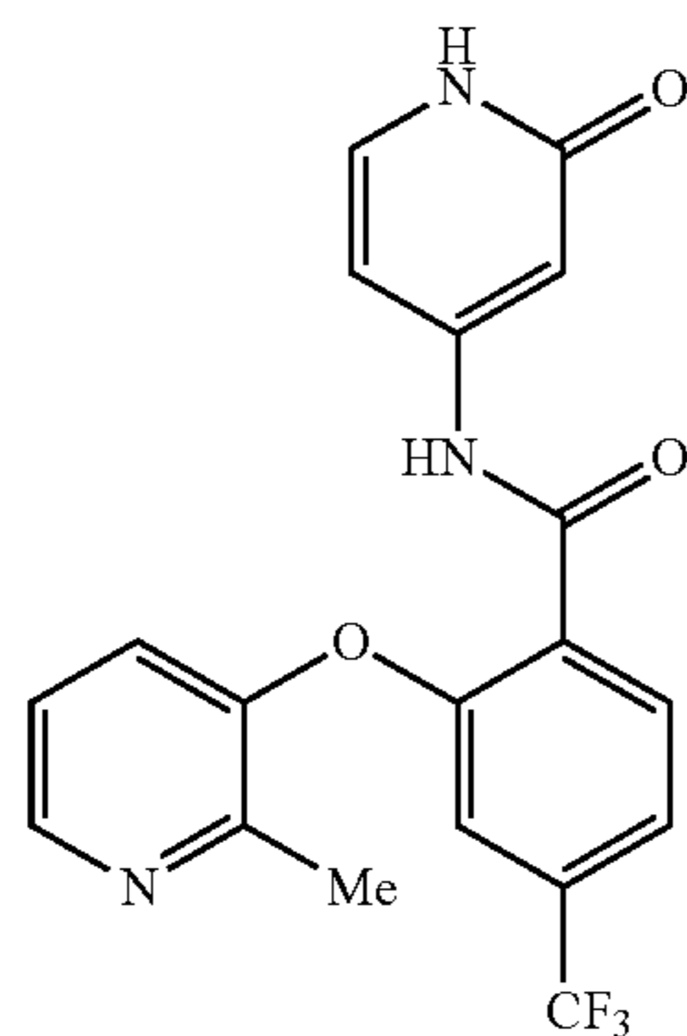
2-((2-methylpyridin-3-yl)oxy)-N-(2-oxo-1,2-dihydropyridin-4-yl)-4-(trifluoromethyl)benzamide
