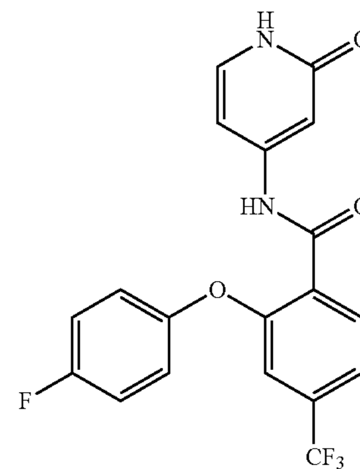
2-(4-fluorophenoxy)-N-(2-oxo-1,2-dihydropyridin-4-yl)-4-(trifluoromethyl)benzamide
