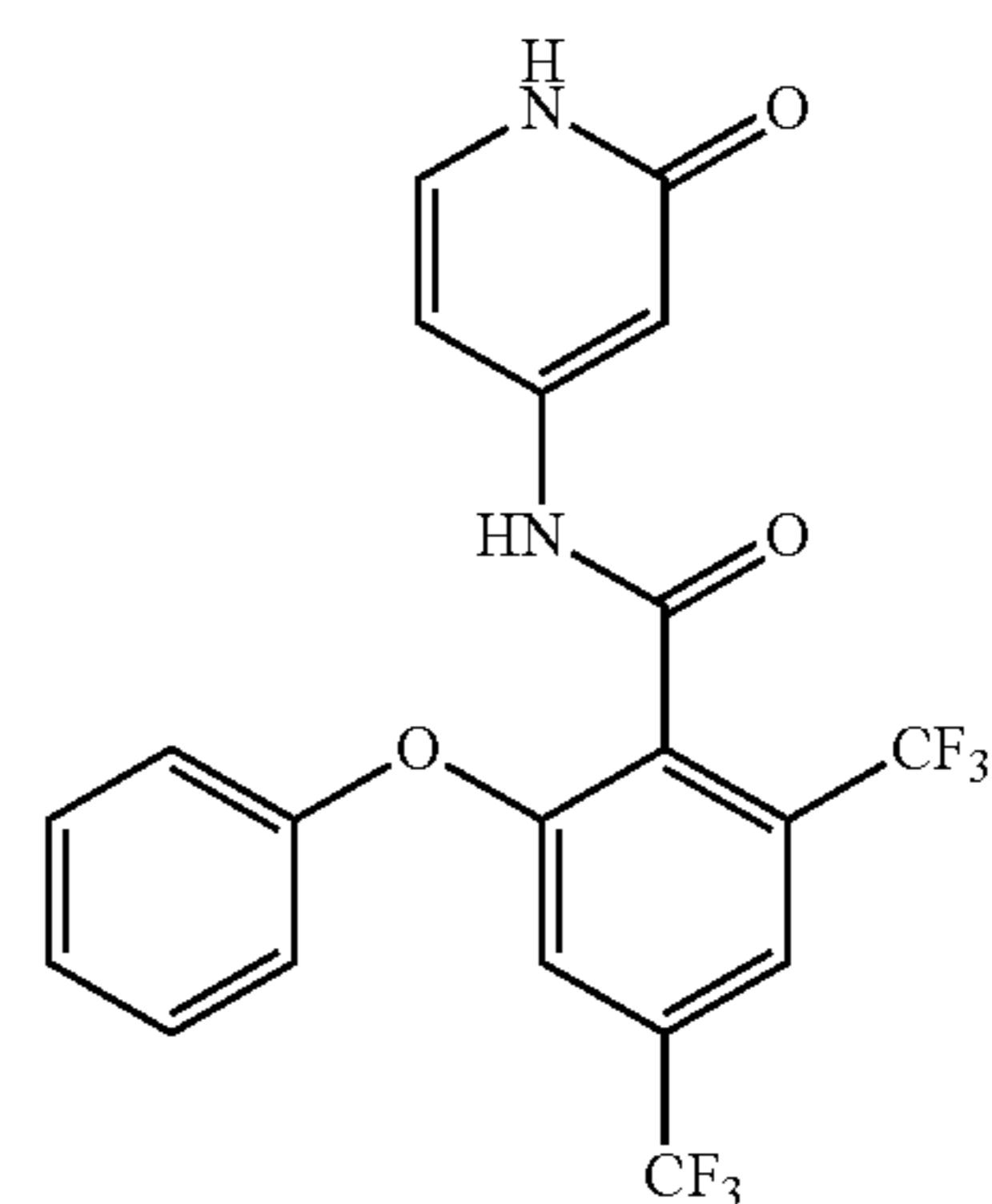
N-(2-oxo-1,2-dihydropyridin-4-yl)-2-phenoxy-4,6-bis(trifluoromethyl)benzamide
