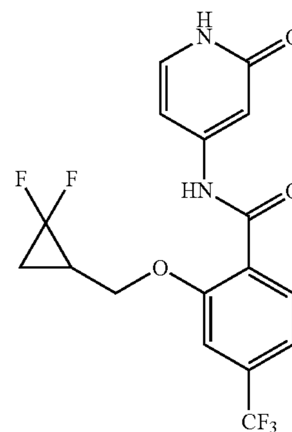
2-((2,2-difluorocyclopropyl)methoxy)-N-(2-oxo-1,2-dihydropyridin-4-yl)-4-(trifluoromethyl)benzamide
