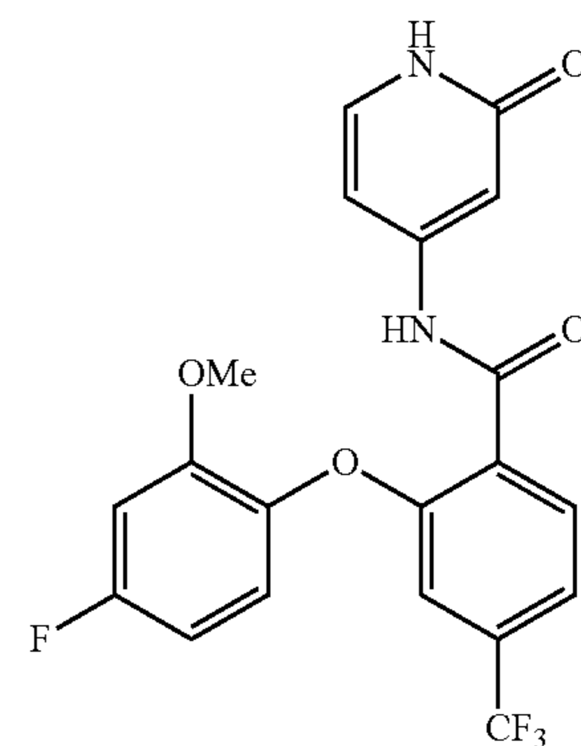
2-(4-fluoro-2-methoxyphenoxy)-N-(2-oxo-1,2-dihydropyridin-4-yl)-4,6-bis(trifluoromethyl)benzamide
