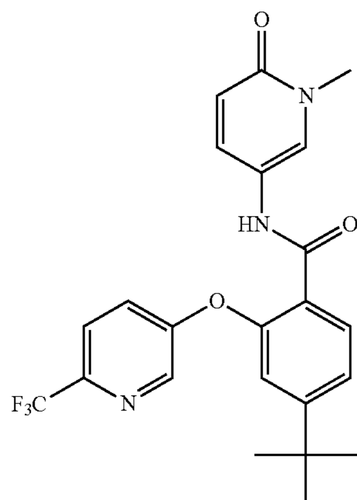
4-(tert-butyl)-N-(1-methyl-6-oxo-1,6-dihydropyridin-3-yl)-2-((6-(trifluoromethyl)pyridin-3-yl)oxy)benzamide
