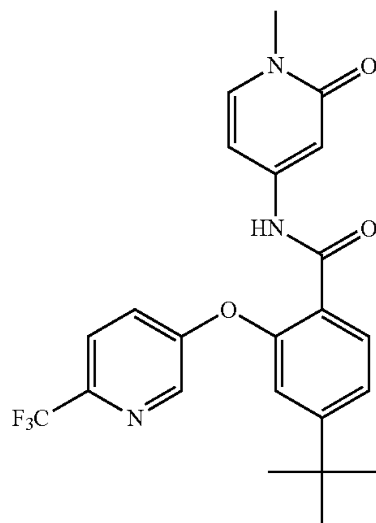
4-(tert-butyl)-N-(1-methyl-2-oxo-1,2-dihydropyridin-4-yl)-2-((6-(trifluoromethyl)pyridin-3-yl)oxy)benzamide
