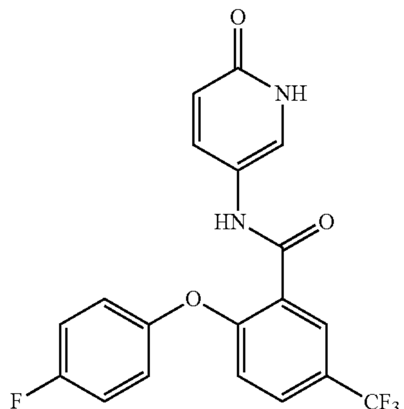
2-(4-fluorophenoxy)-N-(6-oxo-1,6-dihydropyridin-3-yl)-5-(trifluoromethyl)benzamide
