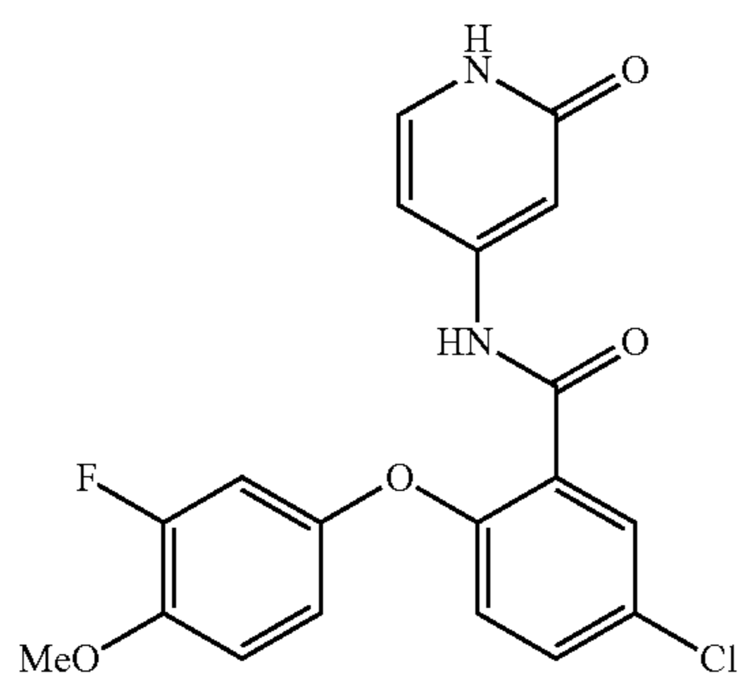
5-chloro-2-(3-fluoro-4- methoxyphenoxy)-N-(2-oxo-1,2- dihydropyridin-4-yl)benzamide
