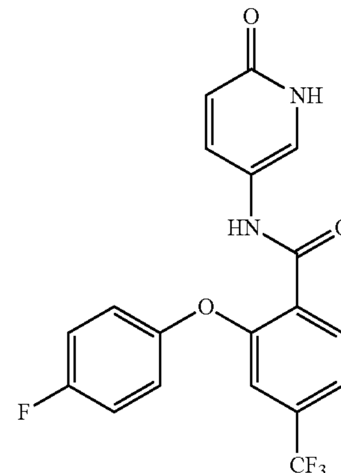
2-(4-fluorophenoxy)-N-(6-oxo-1,6-dihydropyridin-3-yl)-4-(trifluoromethyl)benzamide
