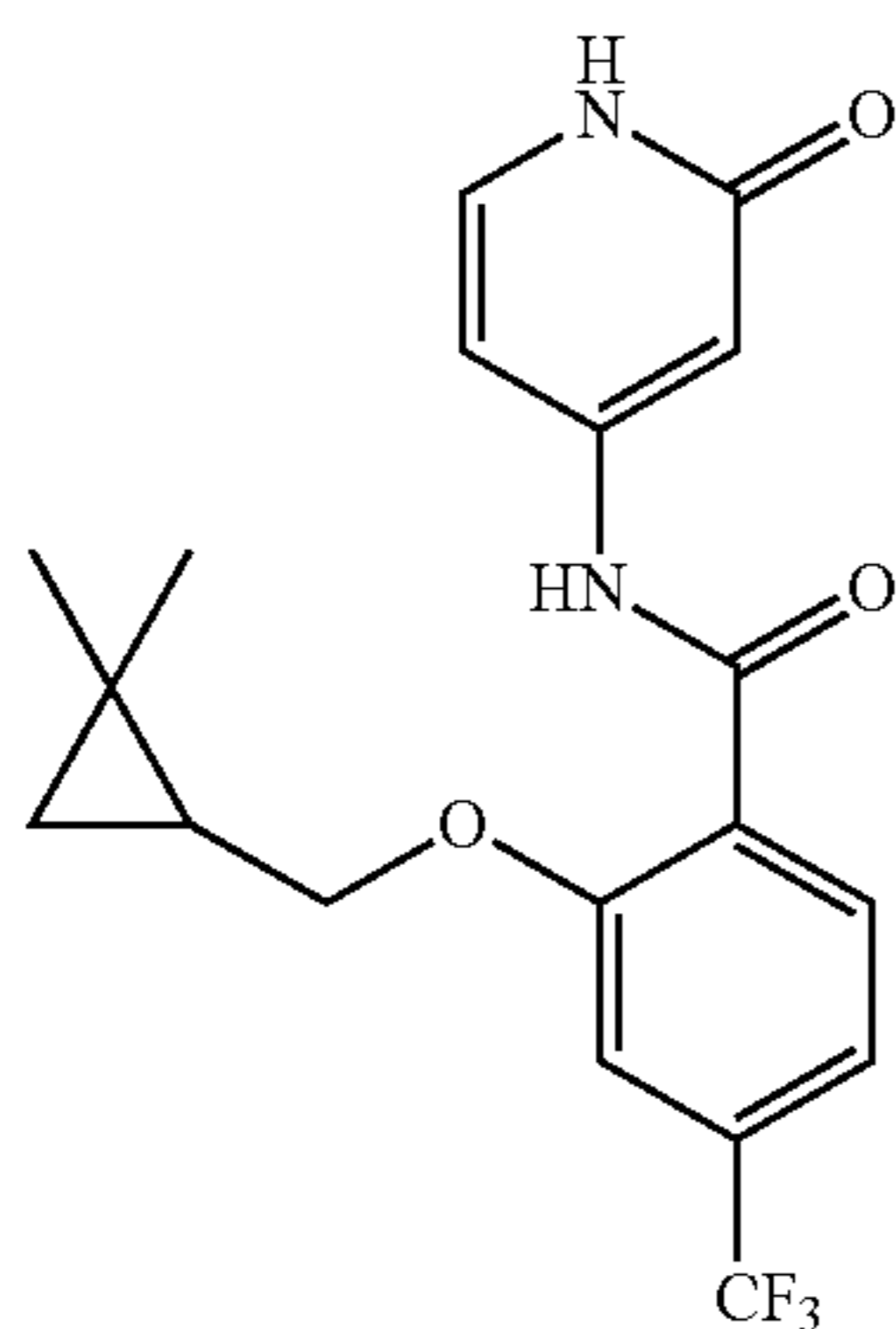
2-((2,2-dimethylcyclopropyl)methoxy)-N-(2-oxo-1,2-dihydropyridin-4-yl)-4-(trifluoromethyl)benzamide
