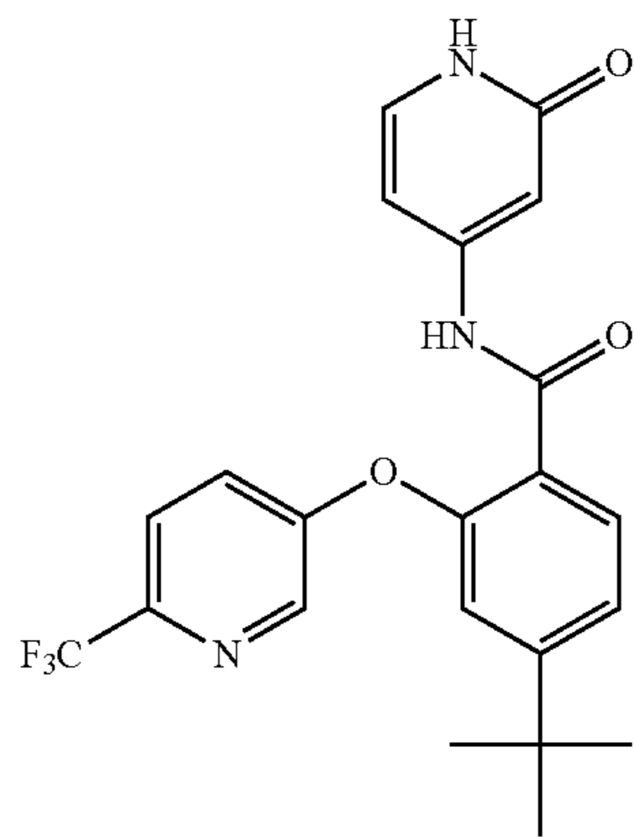
4-(tert-butyl)-N-(2-oxo-1,2-dihydropyridin-4-yl)-2-((6-(trifluoromethyl)pyridin-3-yl)oxy)benzamide
