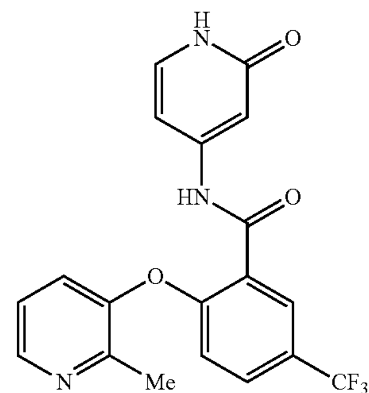
2-((2-methylpyridin-3-yl)oxy)-N-(2-oxo-1,2-dihydropyridin-4-yl)-5-(trifluoromethyl)benzamide
