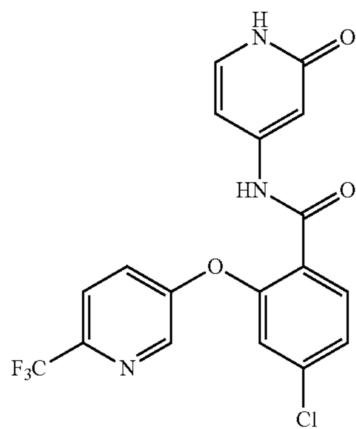
4-chloro-N-(2-oxo-1,2-dihydropyridin-4-yl)-2-((6-(trifluoromethyl)pyridin-3-yl)oxy)benzamide
