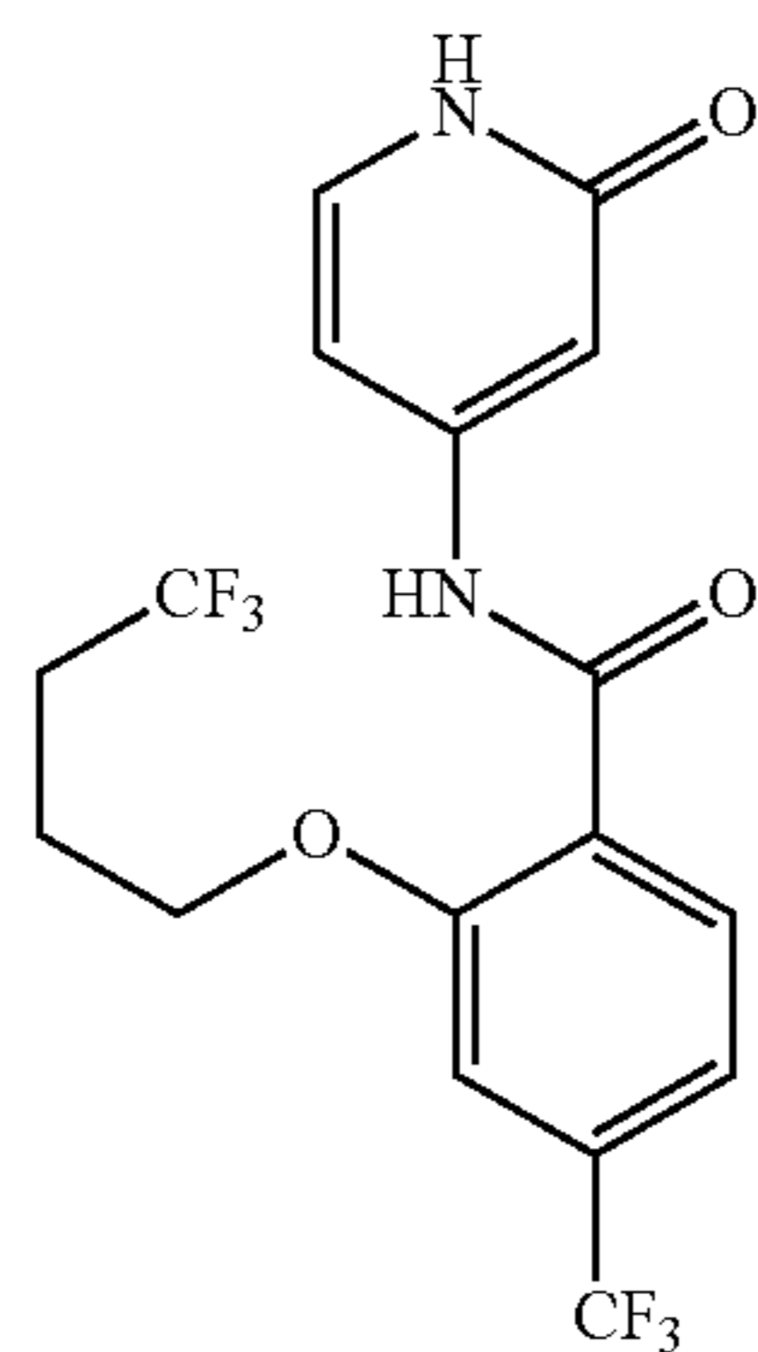
N-(2-oxo-1,2-dihydropyridin-4-yl)-2-(4,4,4-trifluorobutoxy)-4-(trifluoromethyl)benzamide
