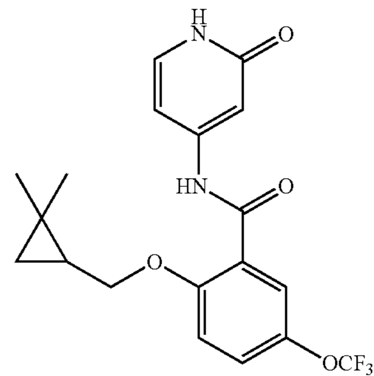
2-((2,2-dimethylcyclopropyl)methoxy)-N-(2-oxo-1,2-dihydropyridin-4-yl)-5-(trifluoromethoxy)benzamide
