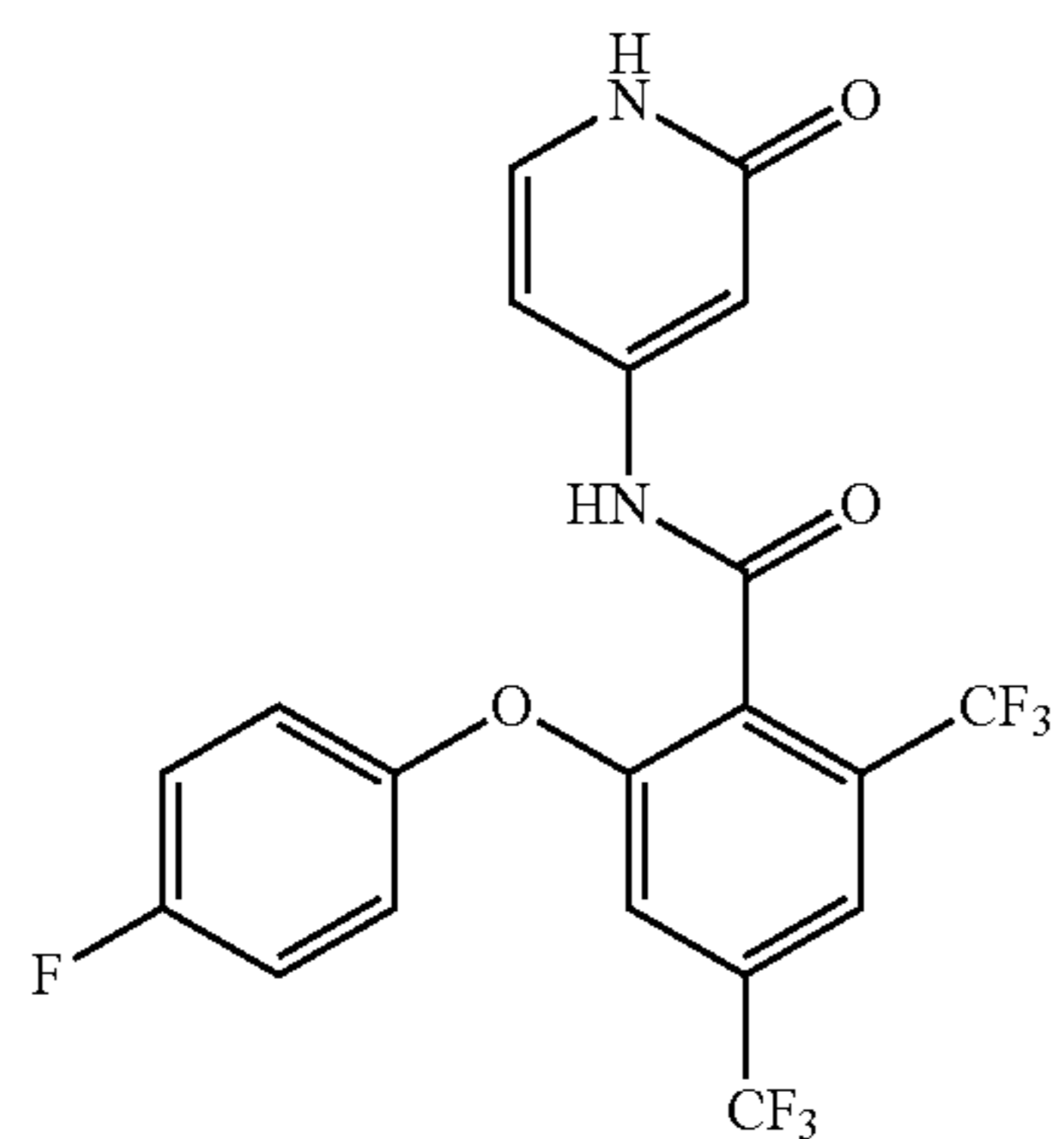
2-(4-fluorophenoxy)-N-(2-oxo-1,2-dihydropyridin-4-yl)-4,6-bis(trifluoromethyl)benzamide
