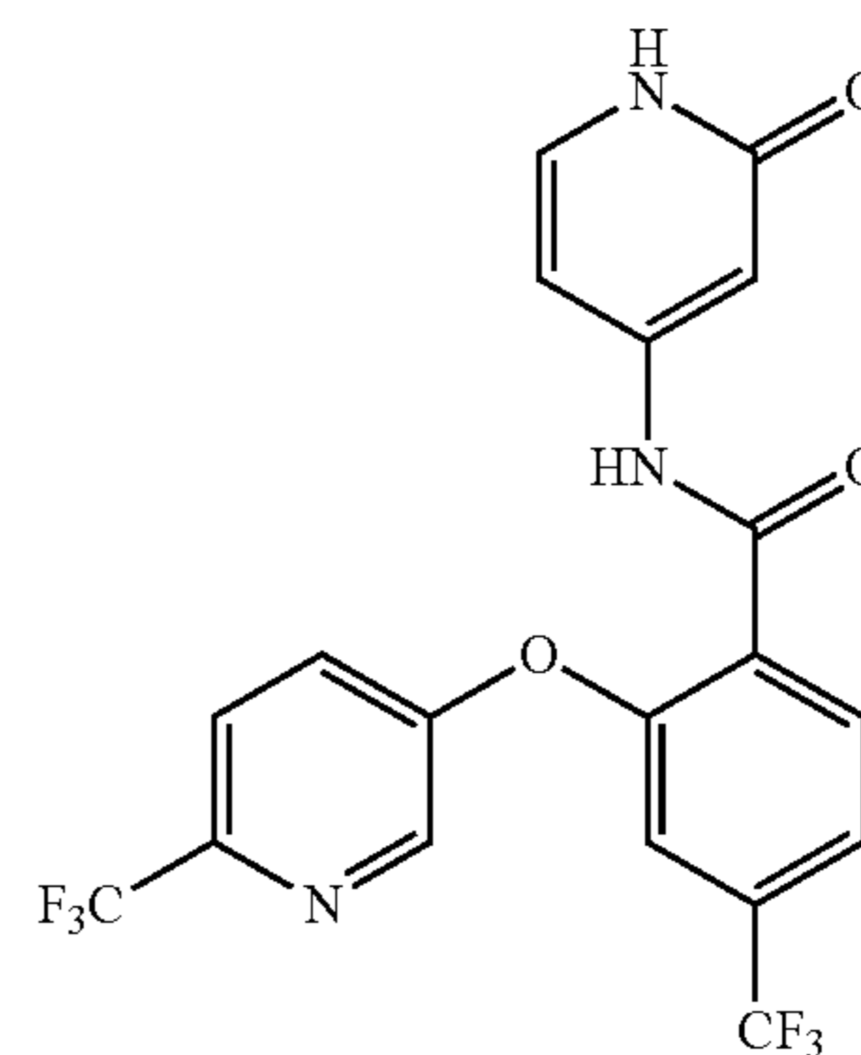
N-(2-oxo-1,2-dihydropyridin-4-yl)-4-(trifluoromethyl)-2-((6-(trifluoromethyl)pyridin-3-yl)oxy)benzamide
