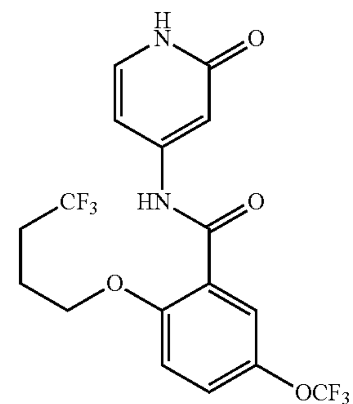
N-(2-oxo-1,2-dihydropyridin-4-yl)-2-(4,4,4-trifluorobutoxy)-5-(trifluoromethoxy)benzamide
