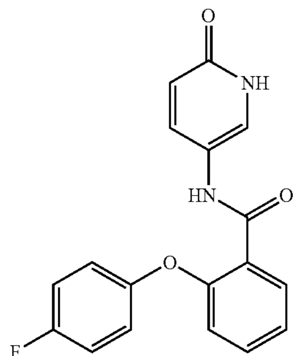
2-(4-fluorophenoxy)-N-(6-oxo-1,6-dihydropyridin-3-yl)benzamide
