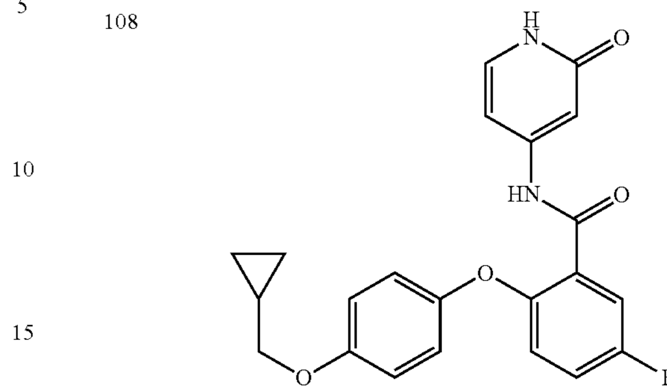
2-(4-(cyclopropylmethoxy)phenoxy)-5-fluoro-N-(2-oxo-1,2-dihydropyridin-4-yl)benzamide
