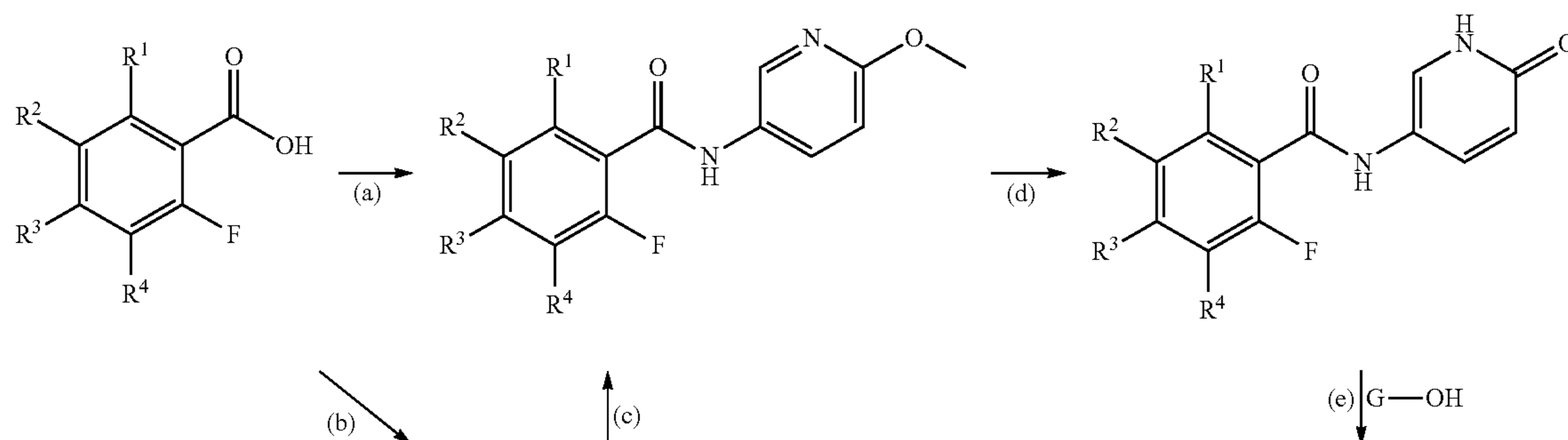
Scheme 2: General Preparation of Compounds of Formula I'
