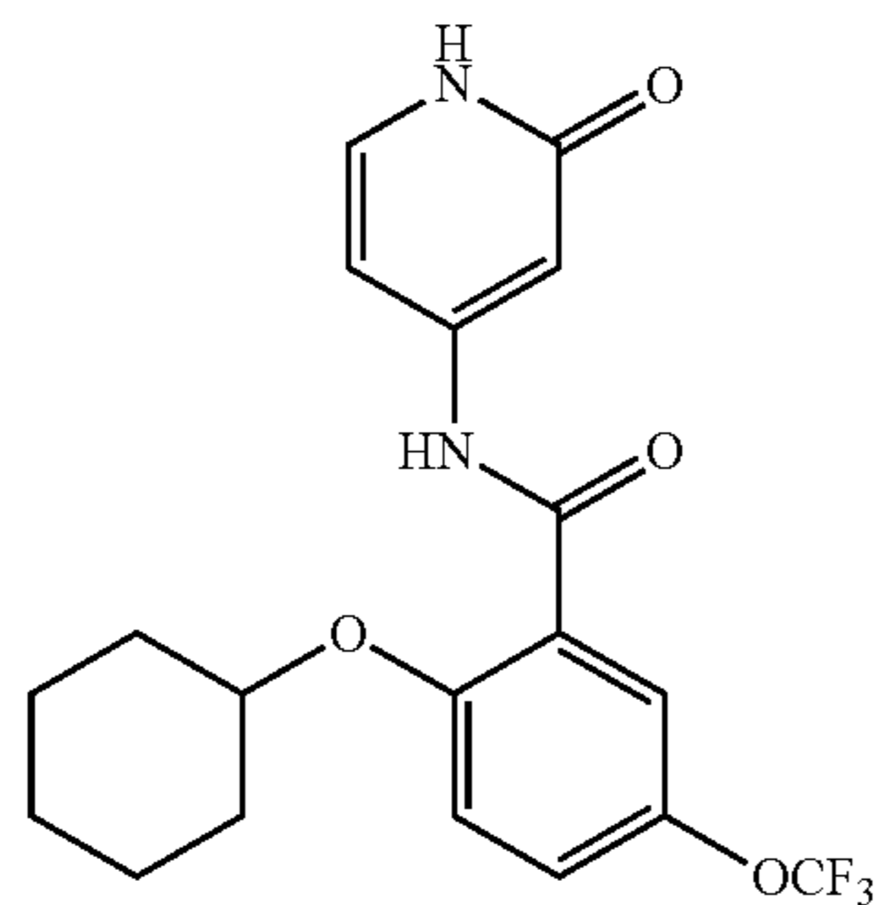
2-(cyclohexyloxy)-N-(2-oxo-1,2-dihydropyridin-4-yl)-5-(trifluoromethoxy)benzamide
