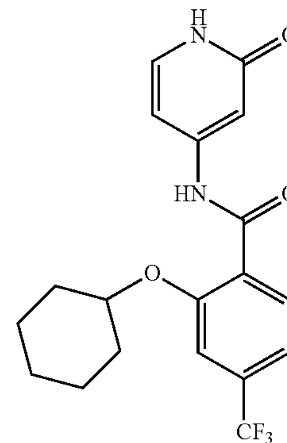
2-(cyclohexyloxy)-N-(2-oxo-1,2-dihydropyridin-4-yl)-4-(trifluoromethyl)benzamide
