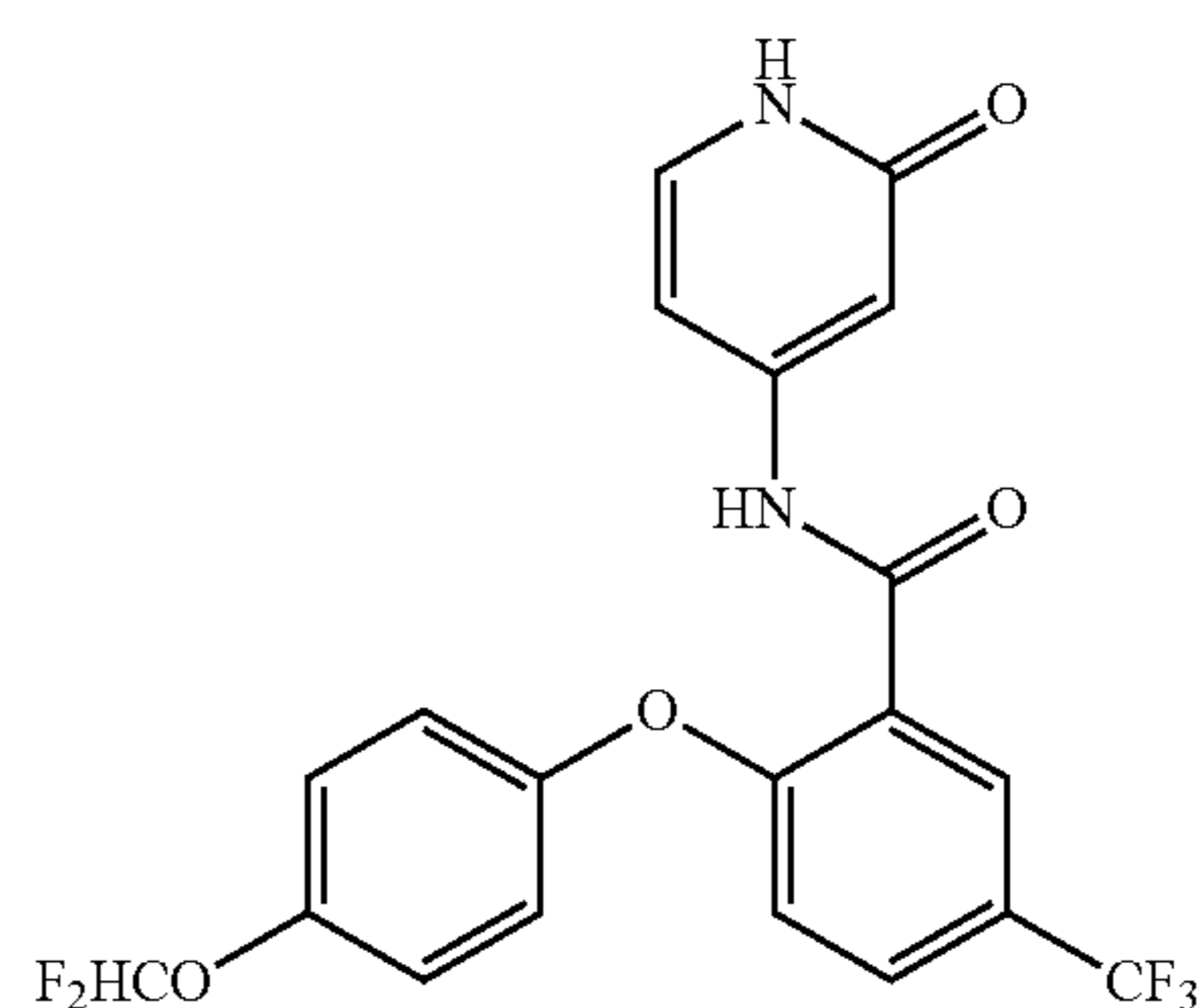
2-(4-(difluoromethoxy)phenoxy)- N-(2-oxo-1,2-dihydropyridin-4- yl)-5-(trifluoromethyl)benzamide
