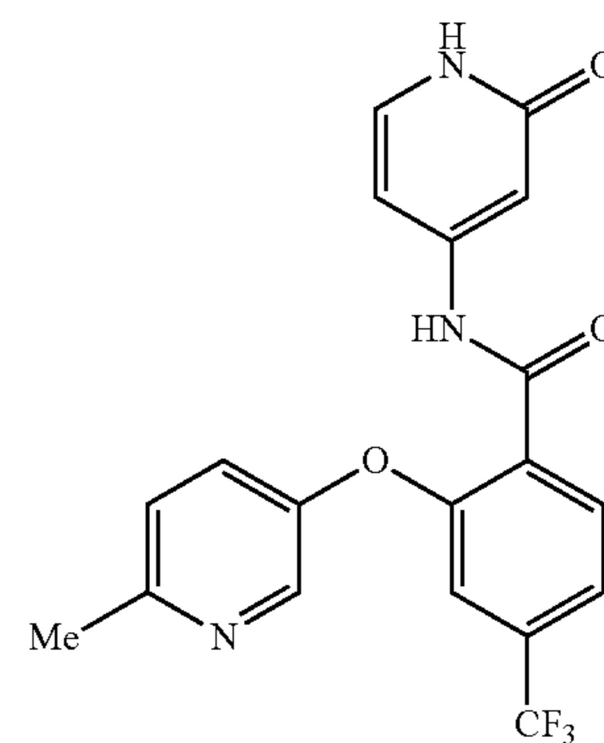
2-((6-methylpyridin-3-yl)oxy)-N-(2-oxo-1,2-dihydropyridin-4-yl)-4-(trifluoromethyl)benzamide
