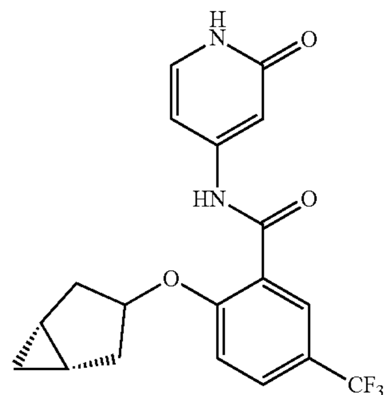
2-((1R,5S)-bicyclo[3.1.0]hexan-3-ylmethoxy)-N-(2-oxo-1,2-dihydropyridin-4-yl)-5-(trifluoromethyl)benzamide
