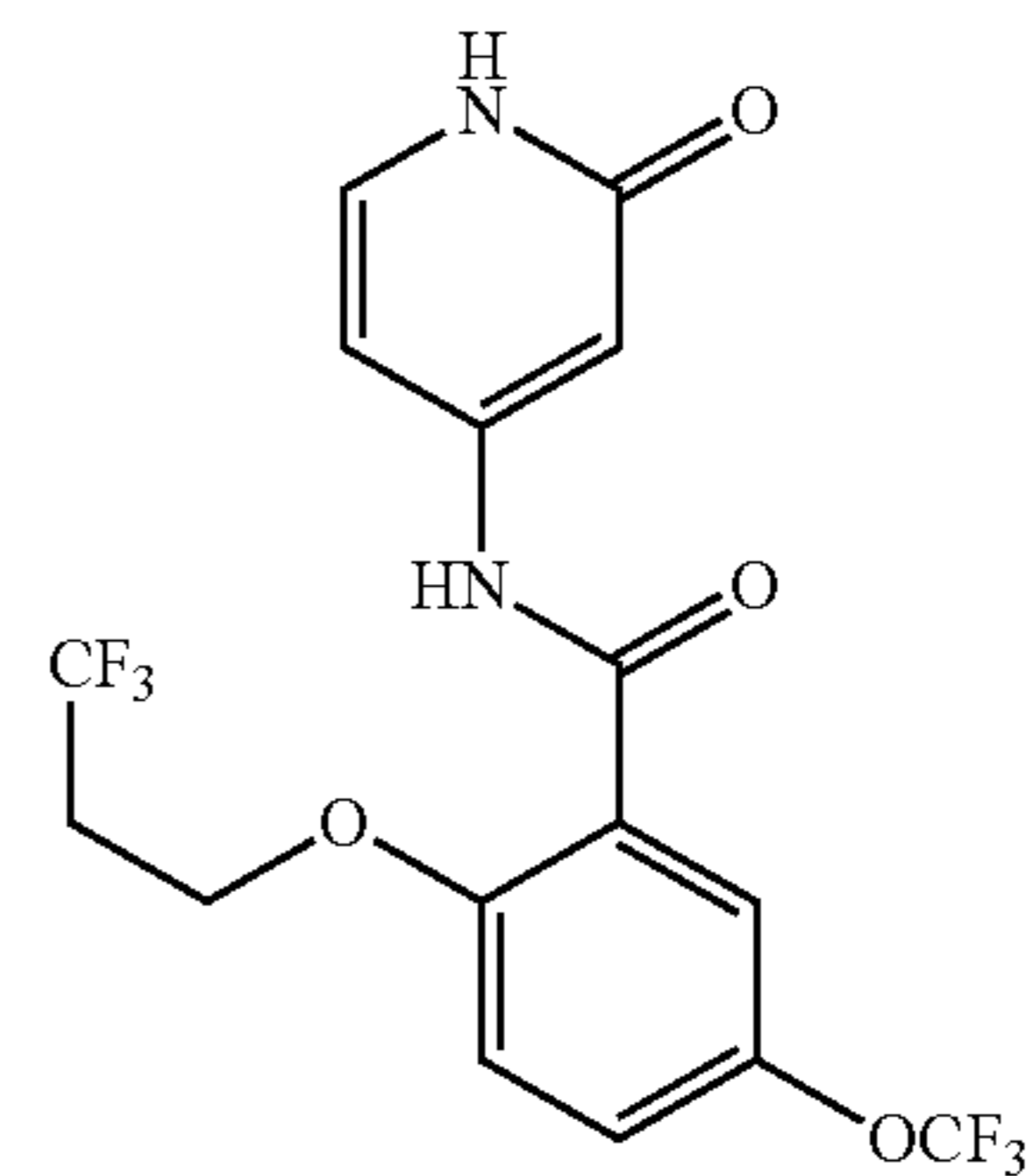
N-(2-oxo-1,2-dihydropyridin-4-yl)-5-(trifluoromethoxy)-2-(3,3,3-trifluoropropoxy)benzamide
