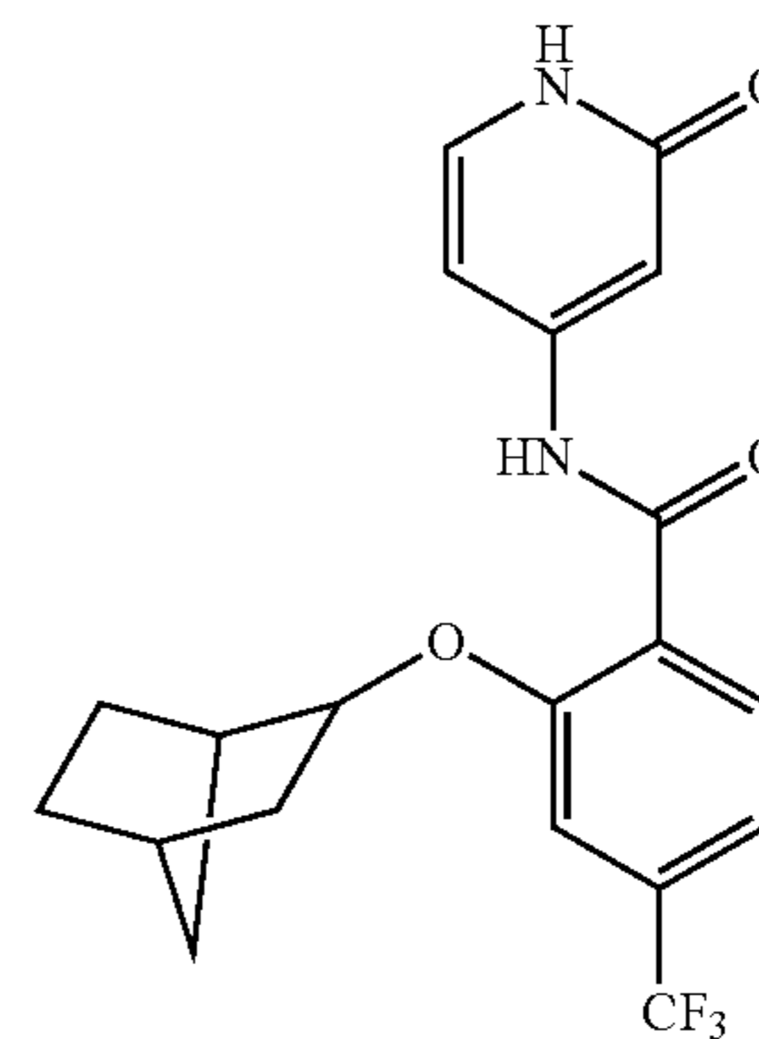
2-(bicyclo[2.2.1]heptan-2-yloxy)-N-(2-oxo-1,2-dihydropyridin-4-yl)-4-(trifluoromethyl)benzamide
