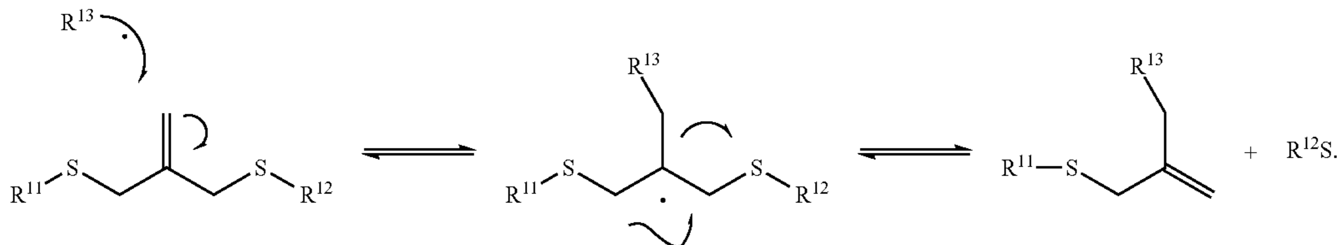
Scheme 1
