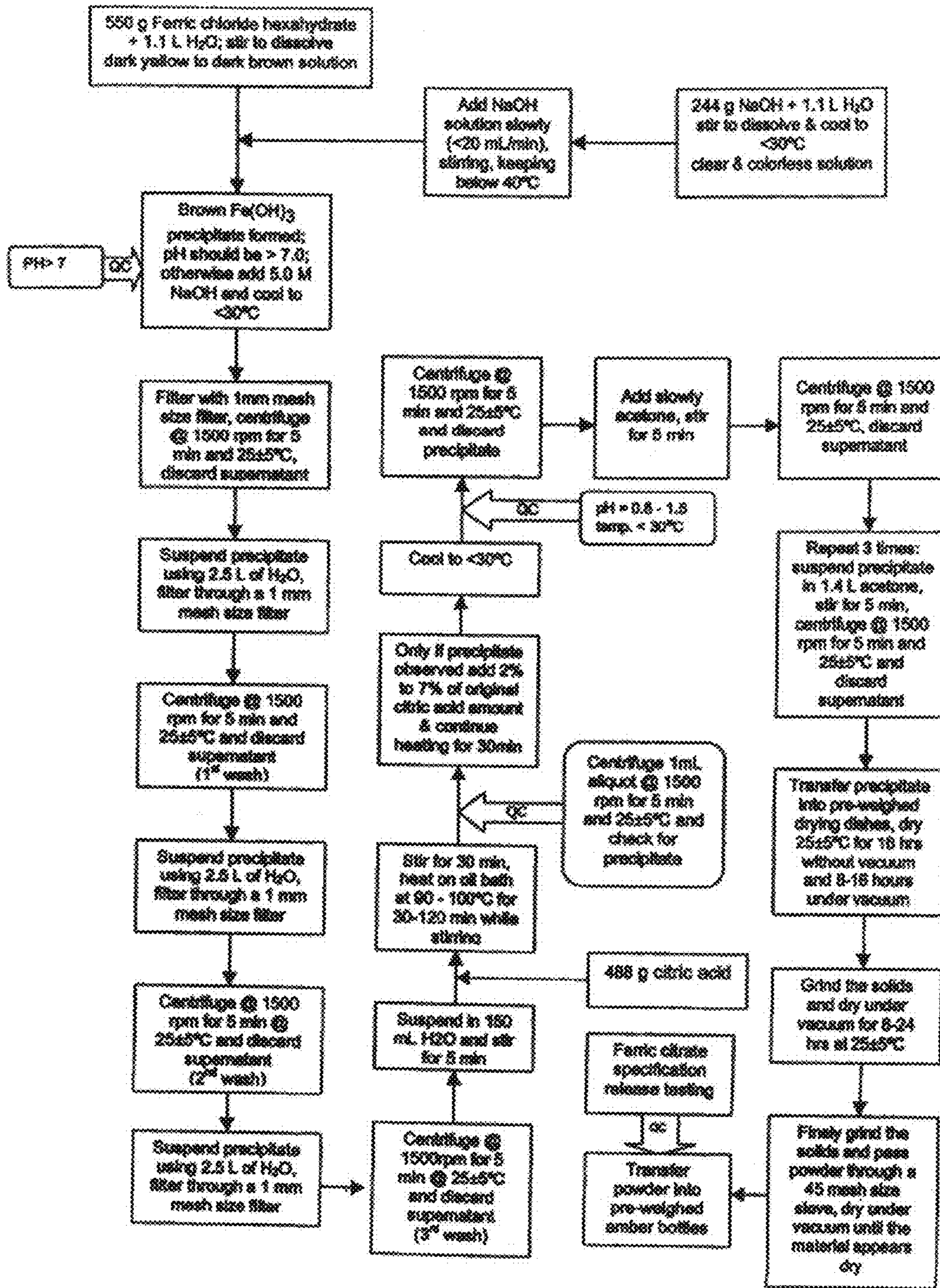
Figure 2 Pharmaceutical-Grade Ferric Citrate Manufacture Flow Chart
