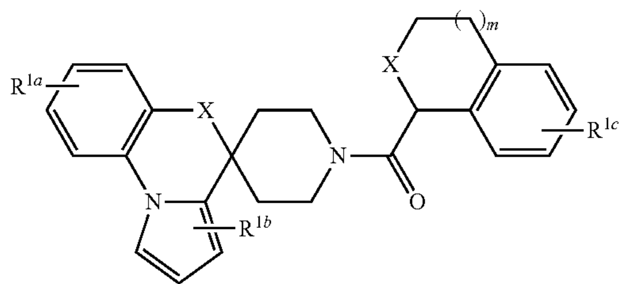
Formula VII
