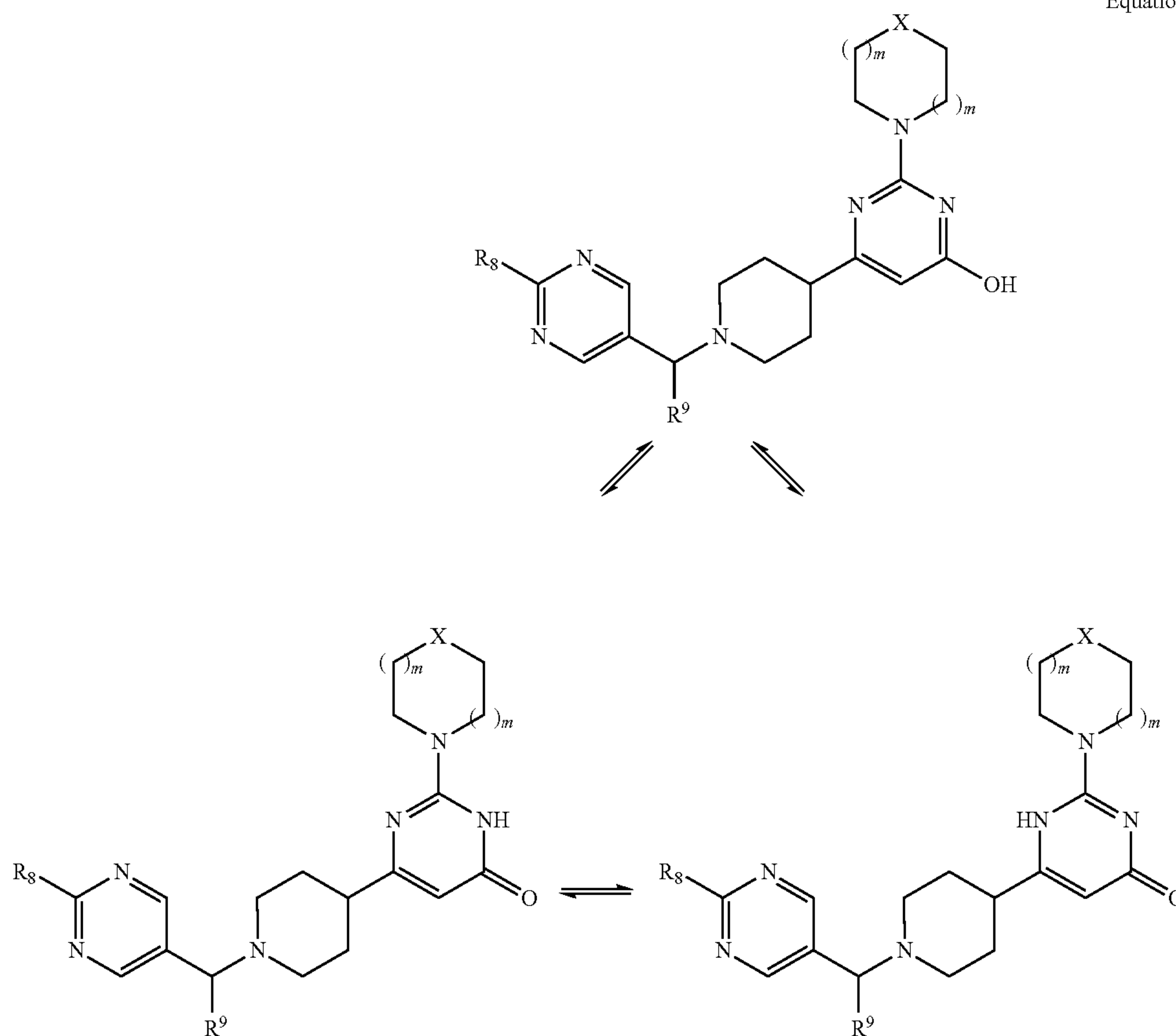
Equation II
