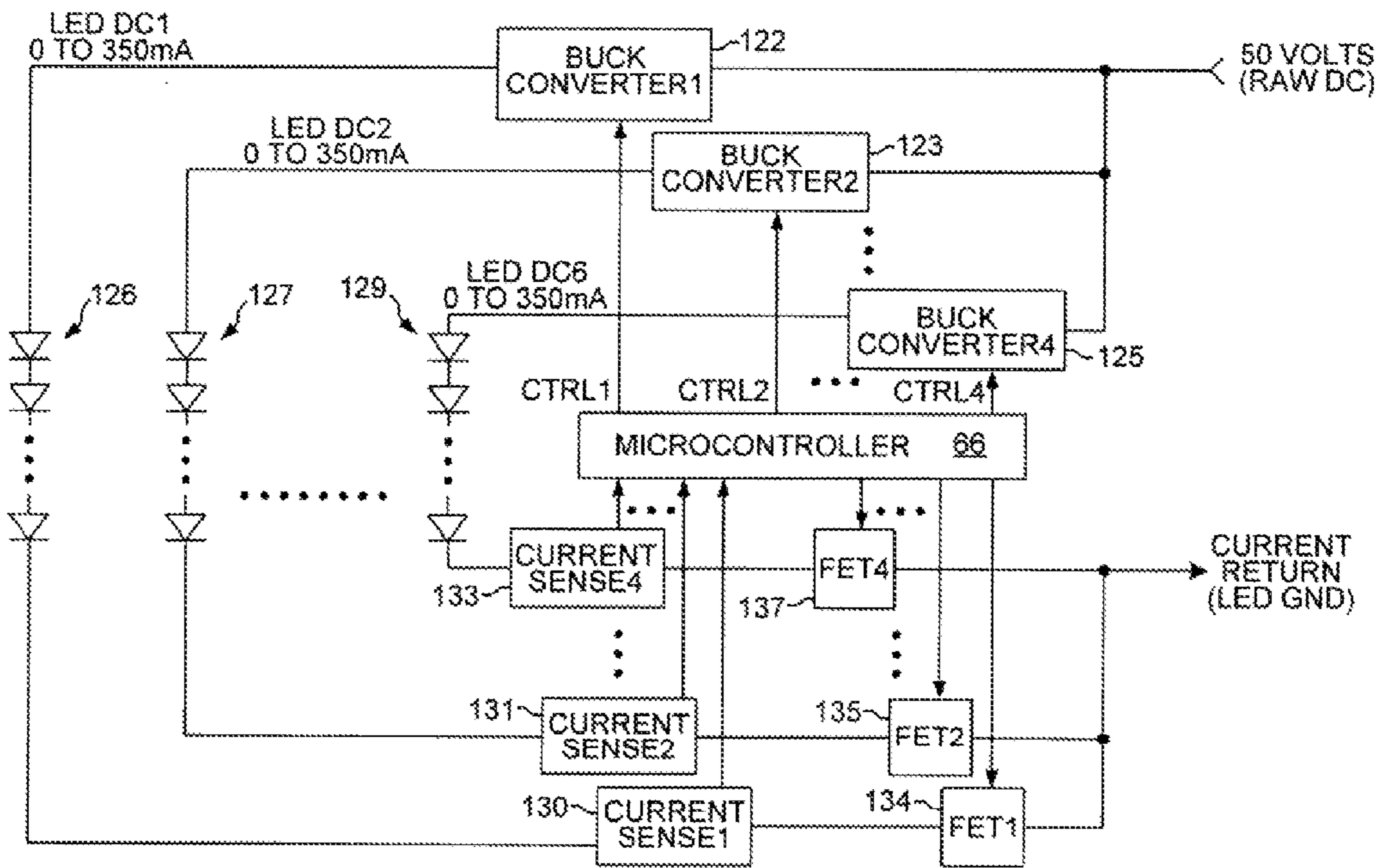
ANOTHER WAY TO DRIVE MULTIPLE STRINGS OF LED JUNCTIONS WITH MULTIPLE BUCK CONVERTERS
