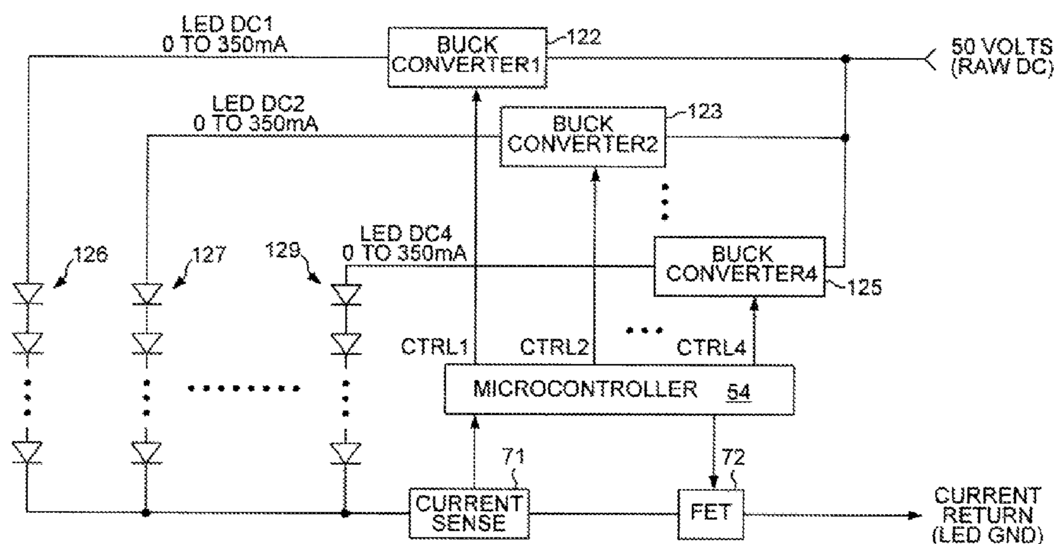
ONE WAY TO DRIVE MULTIPLE STRINGS OF LED JUNCTIONS WITH MULTIPLE BUCK CONVERTERS
