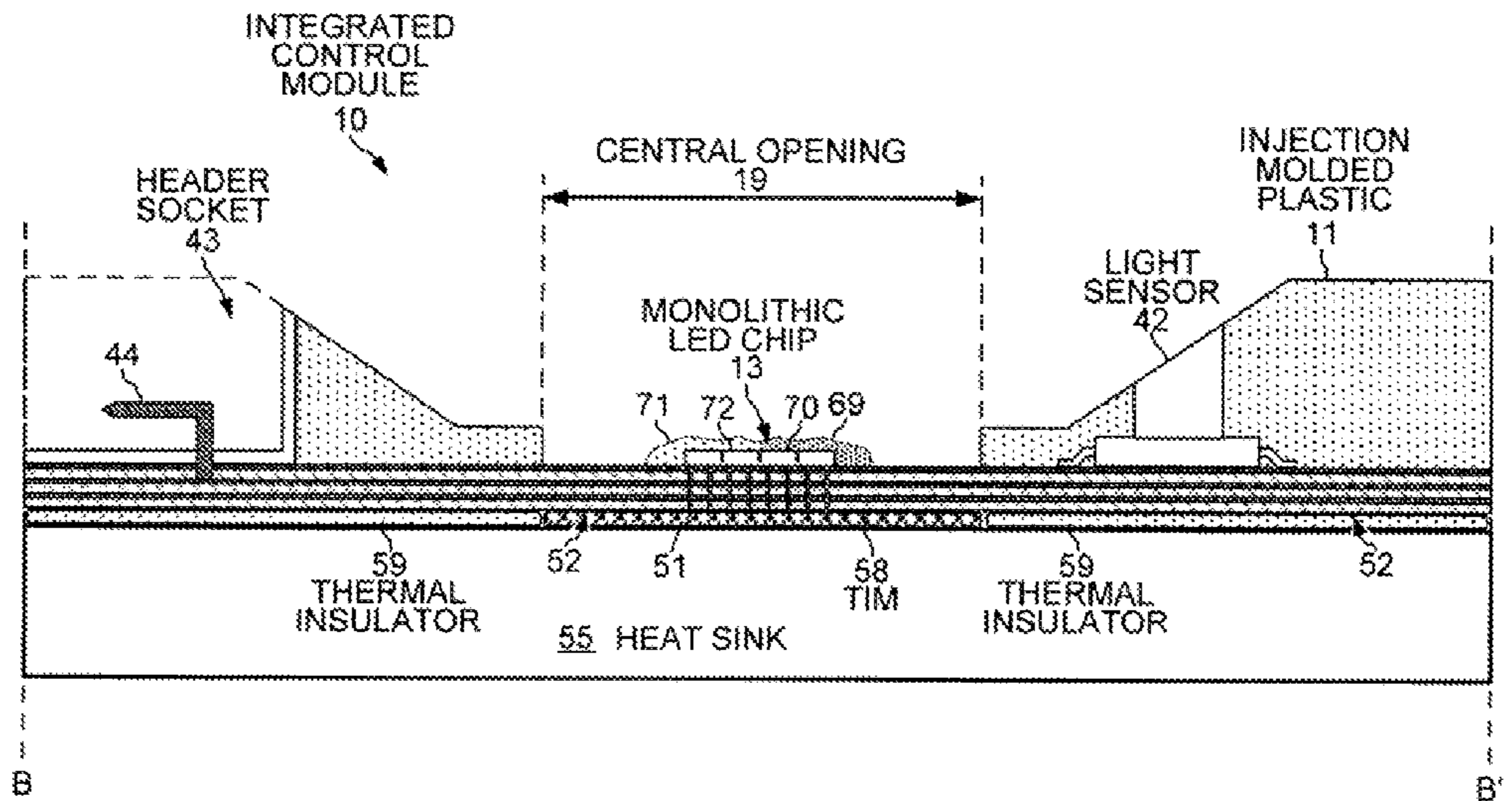
CROSS-SECTIONAL VIEW TAKEN ALONG LINE B-B' (SHOWN ON A HEAT SINK)
