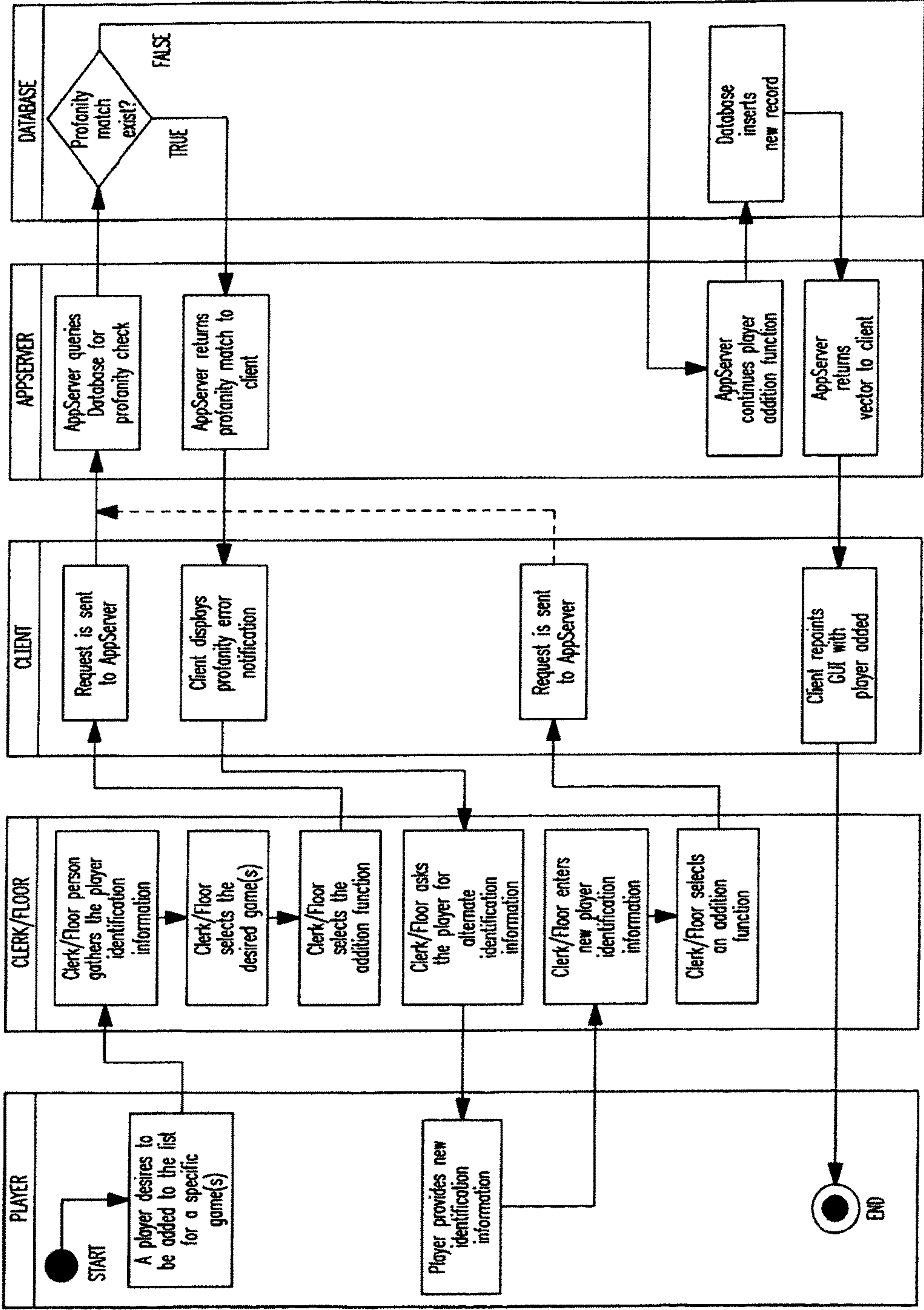
Activity Diagram
