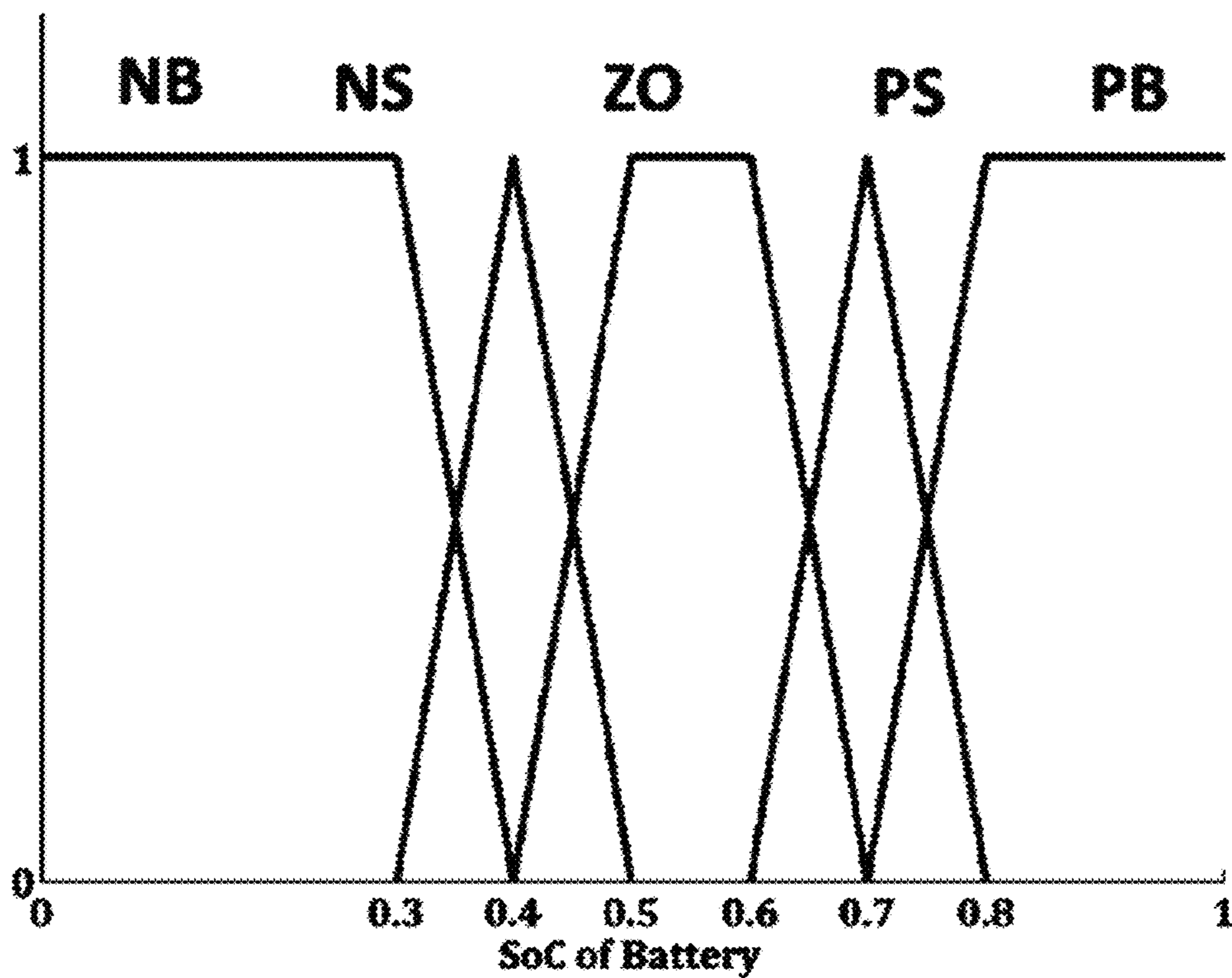
MEMBERSHIP FUNCTION FOR STATE OF CHARGE FOR THE BATTERY (SOC_BE)
