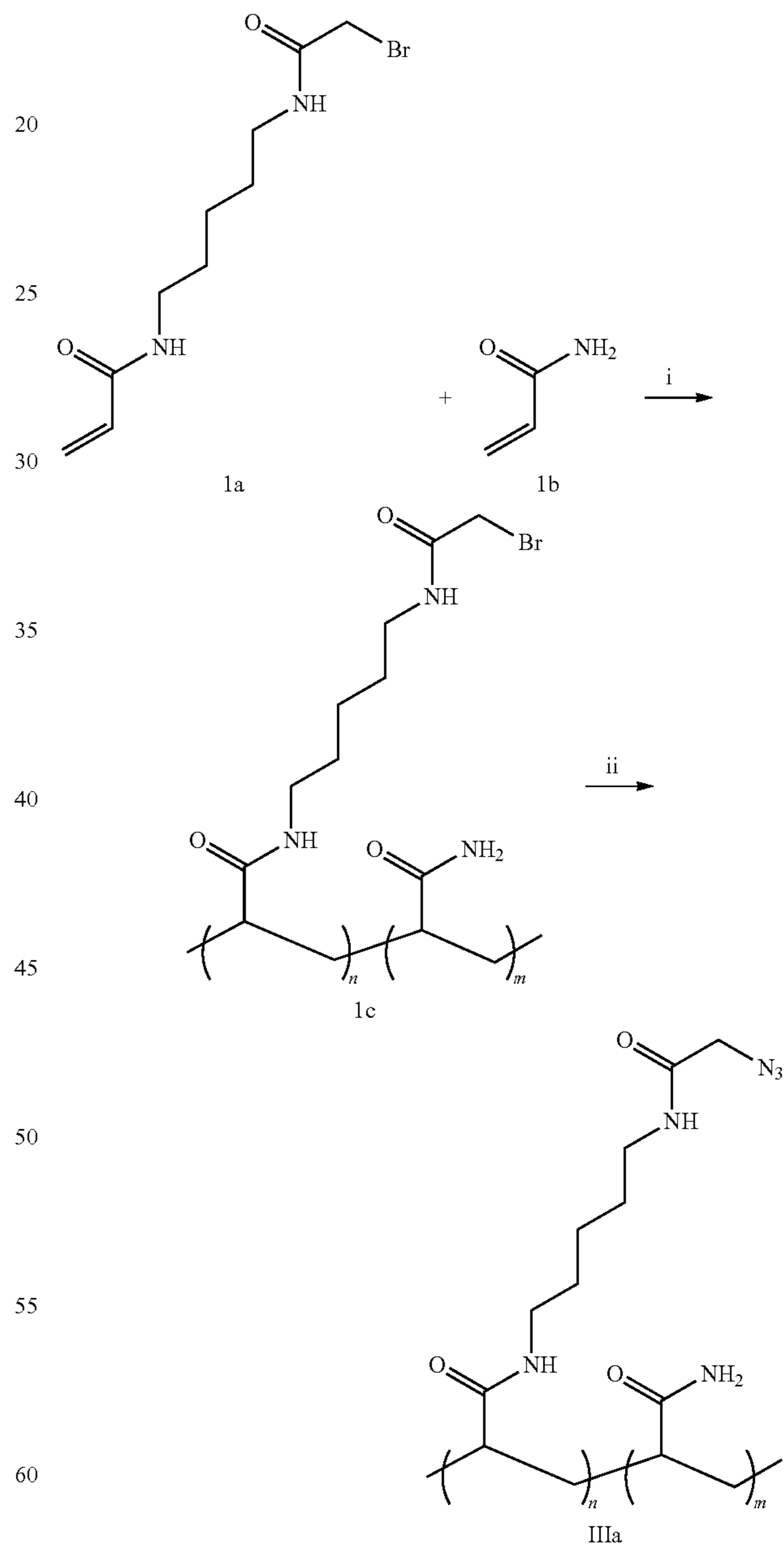
Scheme 1A. Synthesis of a solution-state PAZAM mixture
