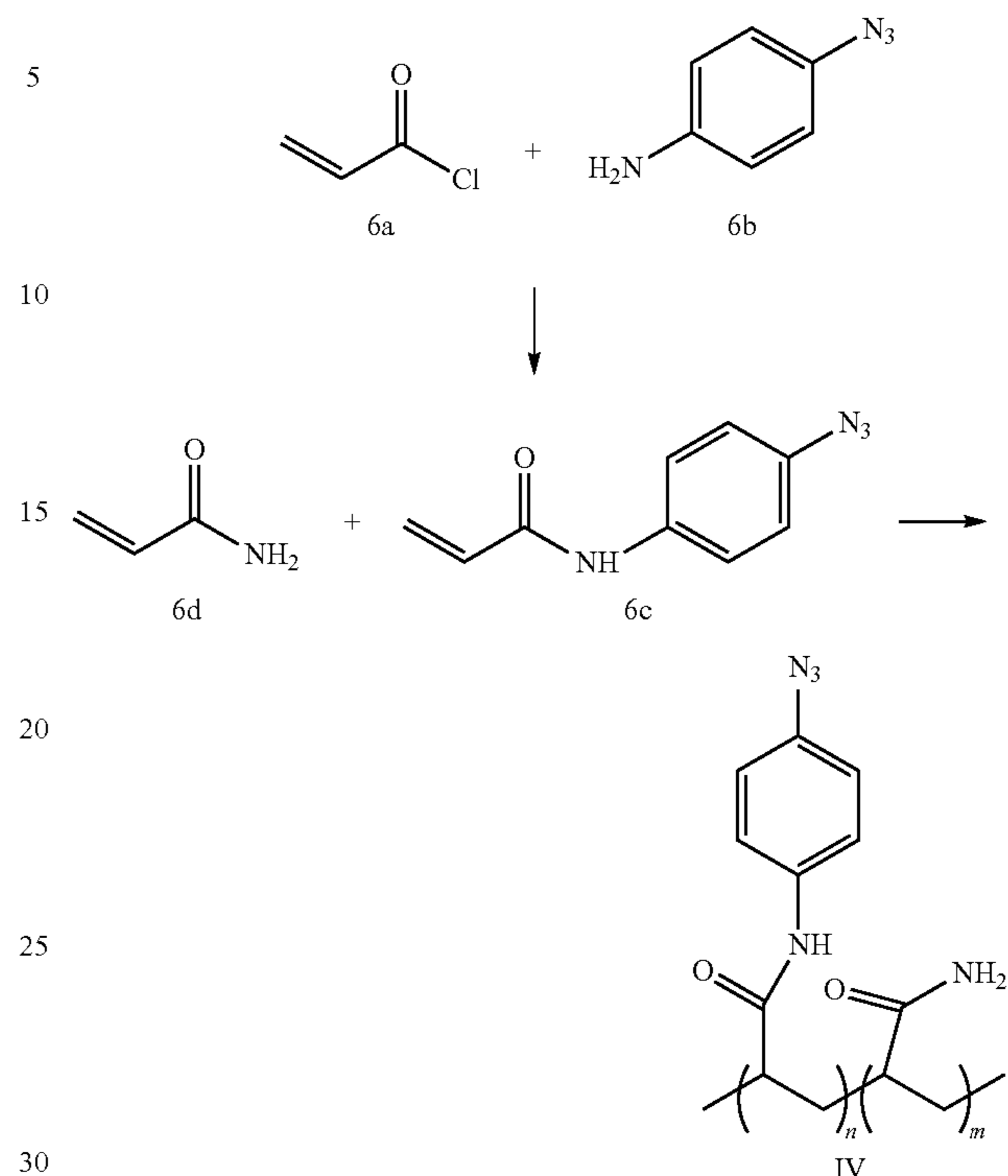
Scheme 6. Synthesis of a Photoactive Linear Polymer
