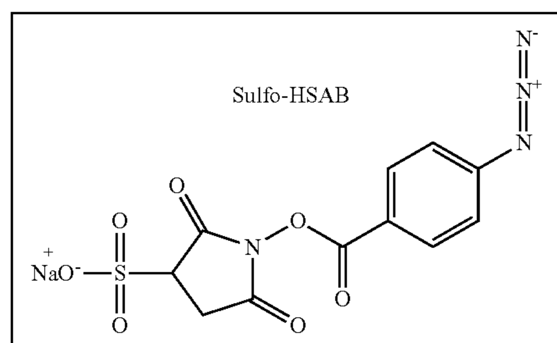
Scheme 4. Pathway Used to Generate a Photoactive Surface
