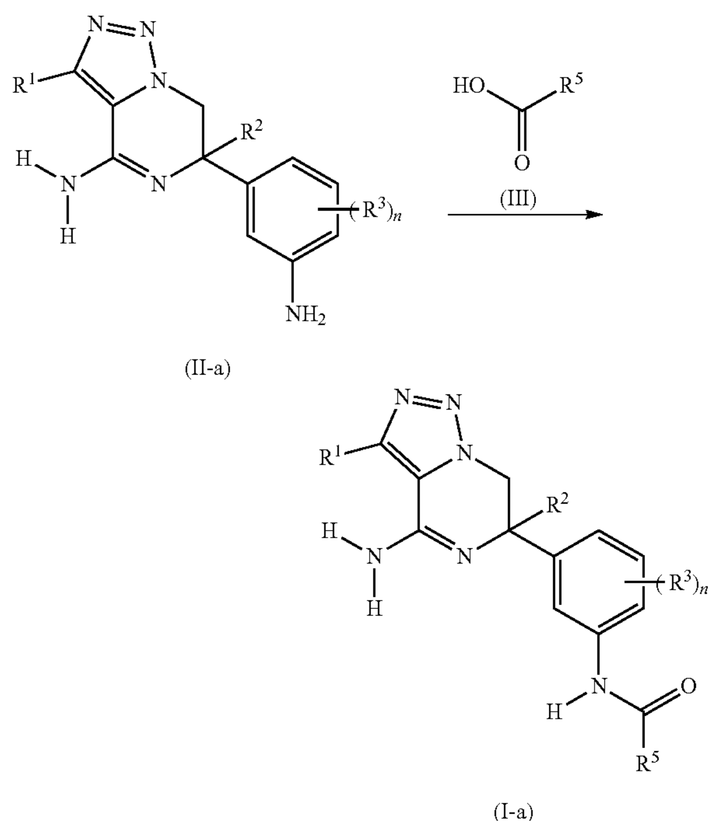
Reaction Scheme 1
