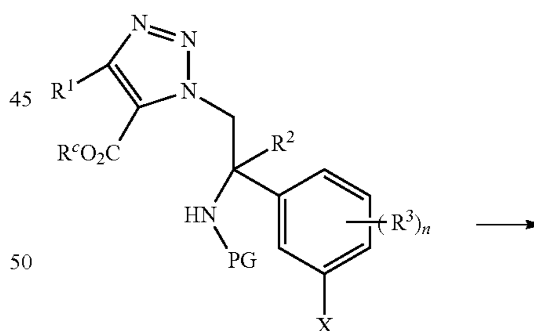
Reaction Scheme 6a
