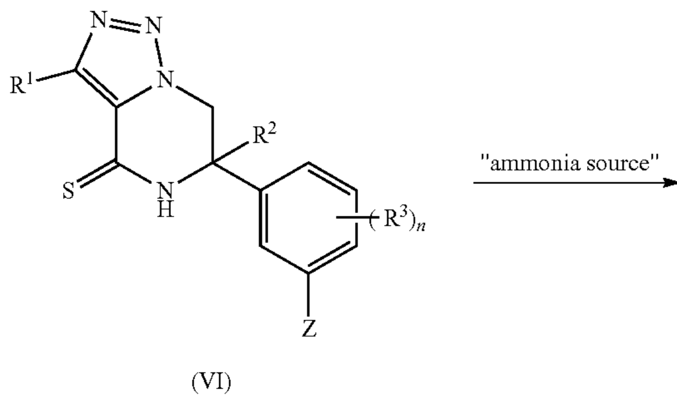
Reaction Scheme 4
