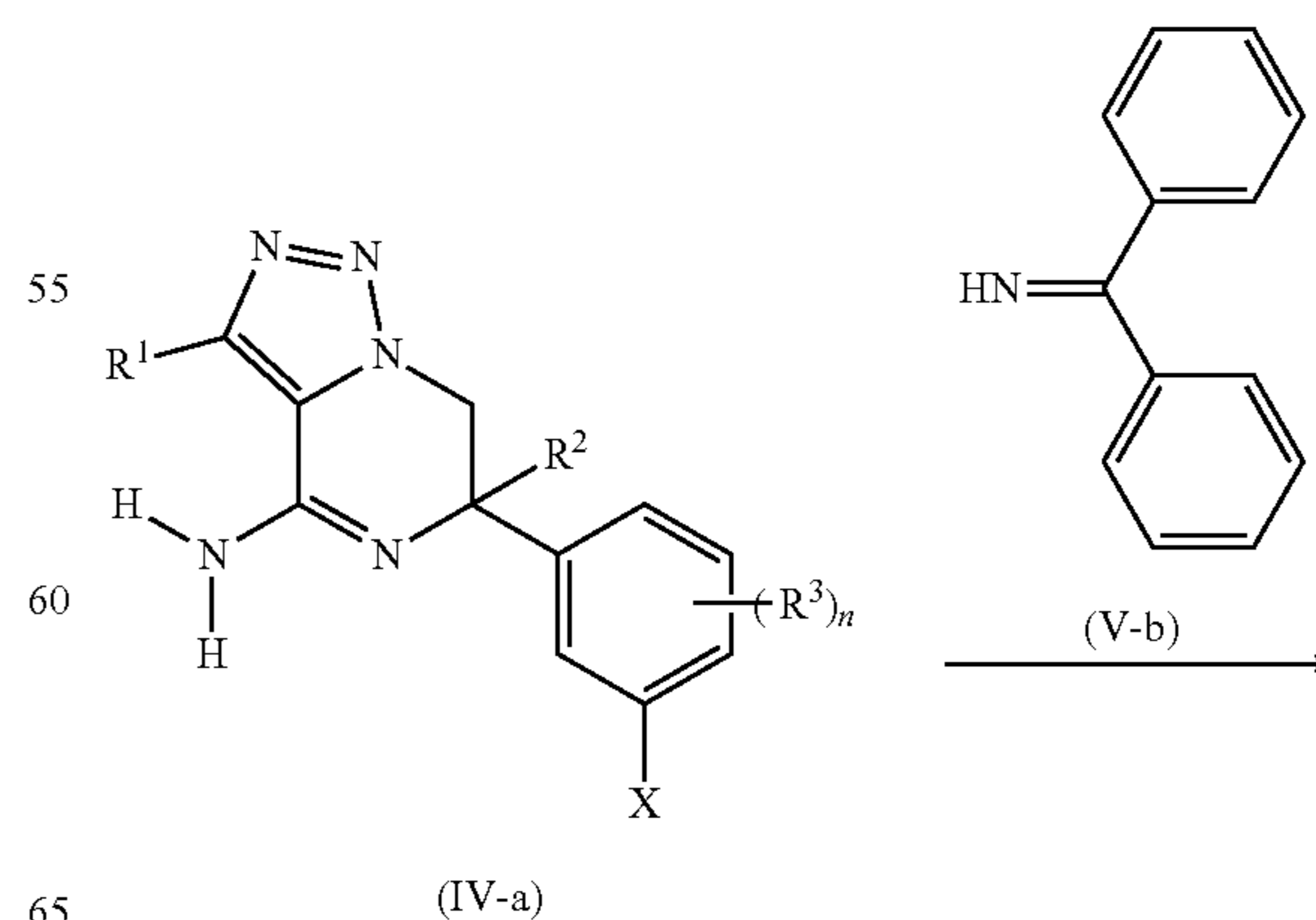
Reaction Scheme 3b
