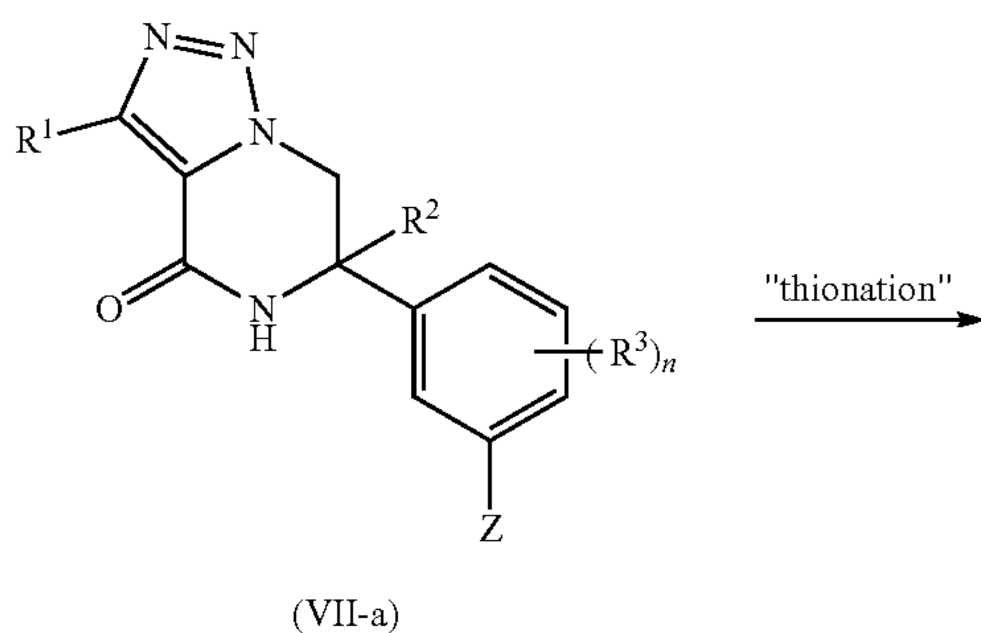
Reaction Scheme 5
