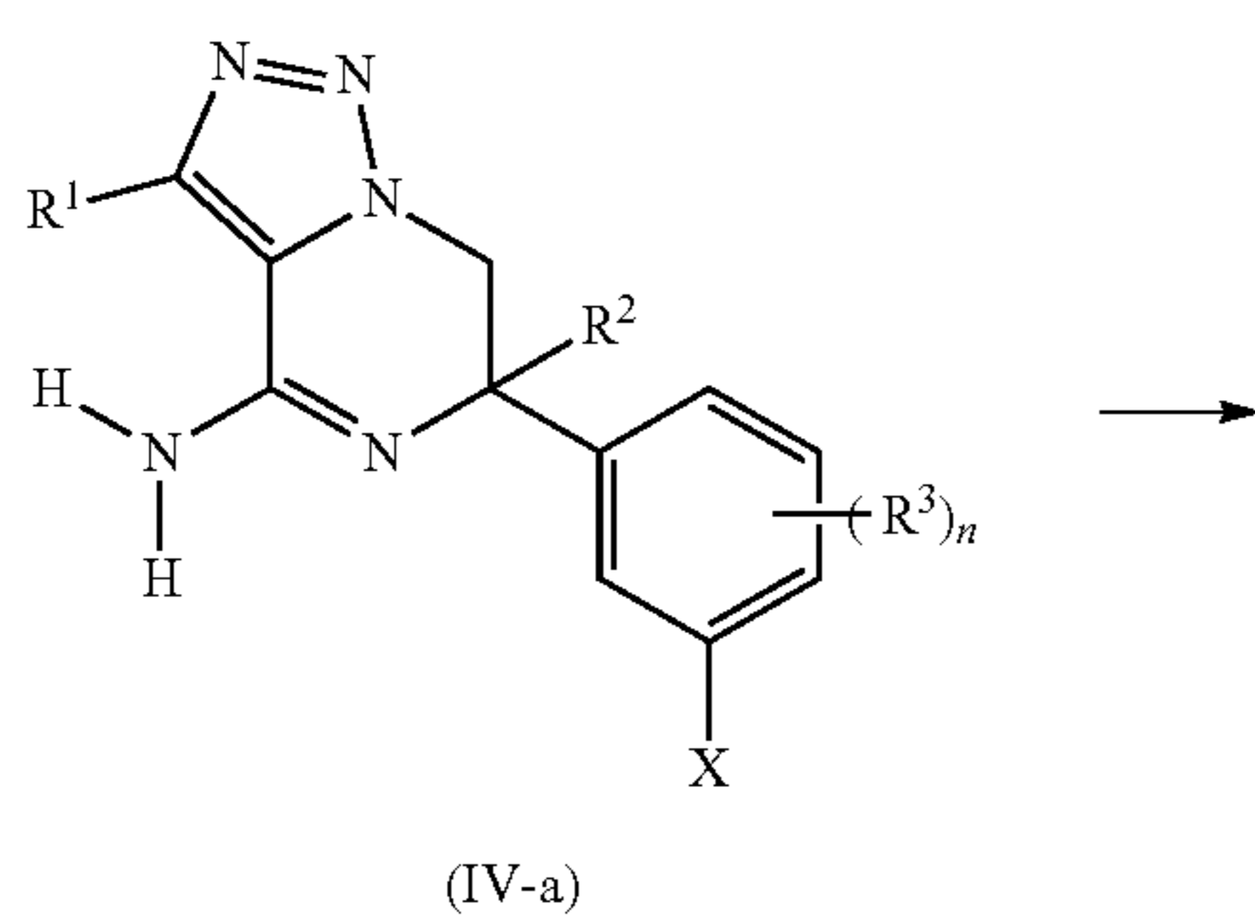
Reaction Scheme 3a
