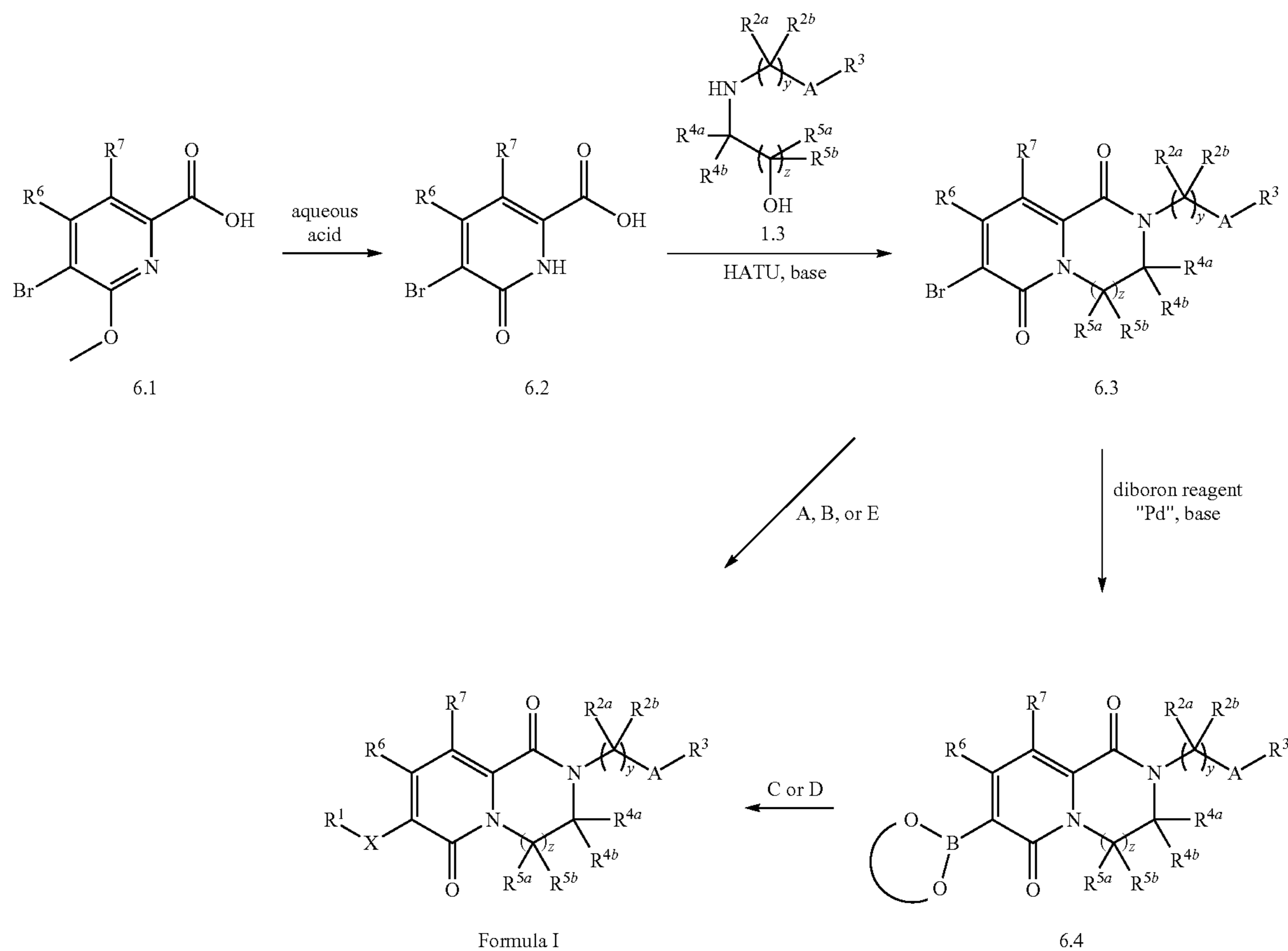
Scheme 6
