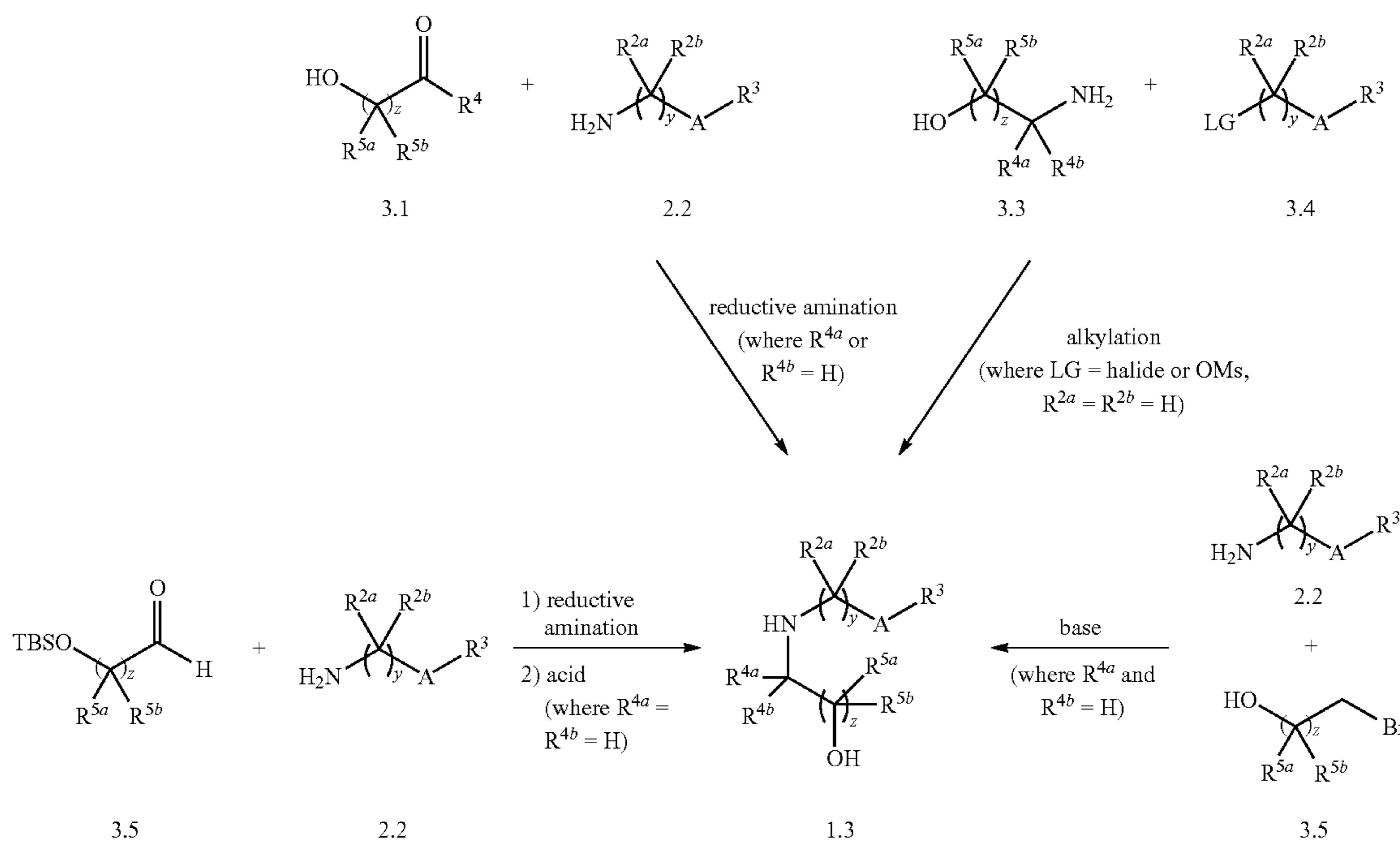
Scheme 3
