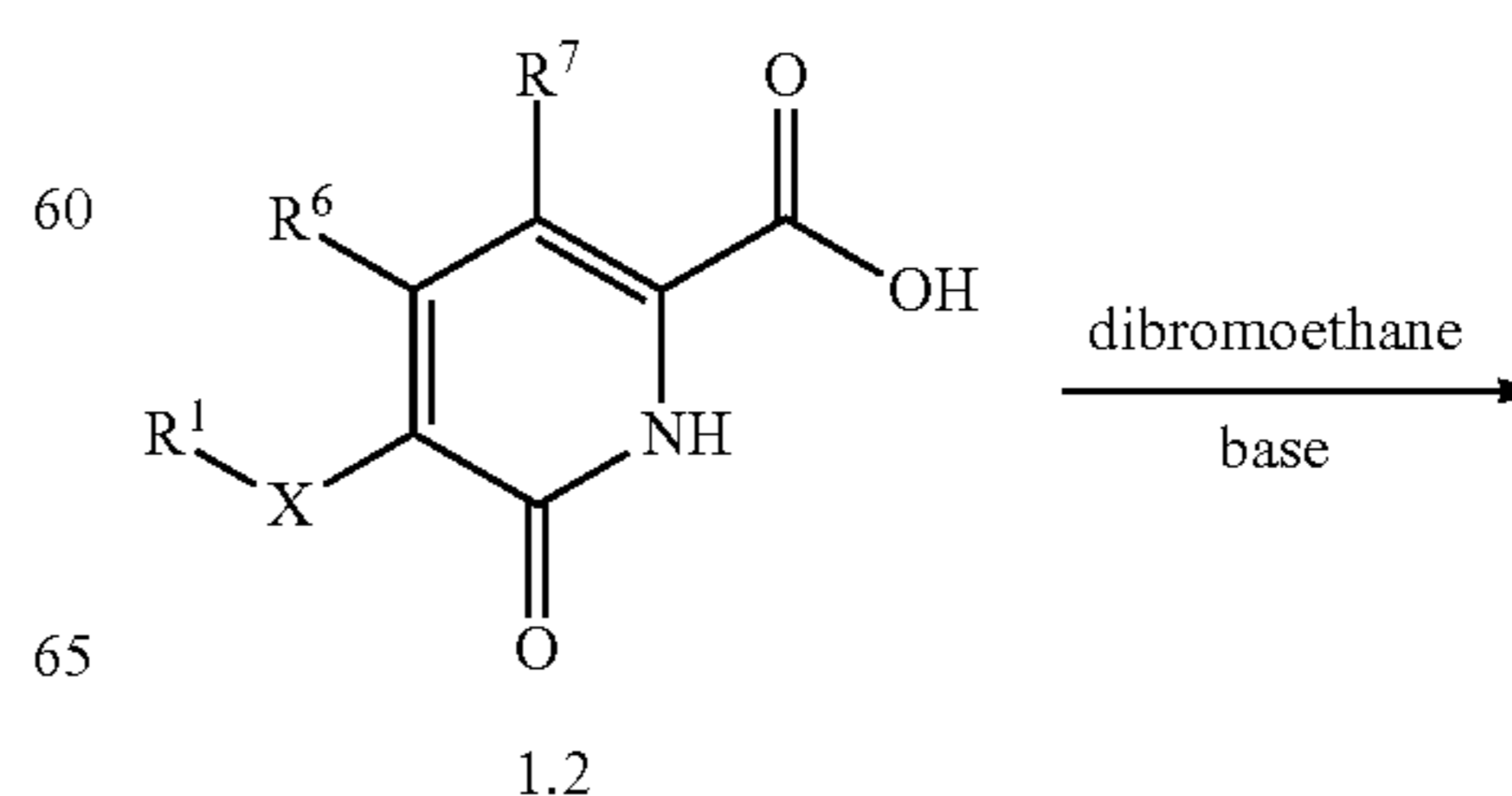
Scheme 7
