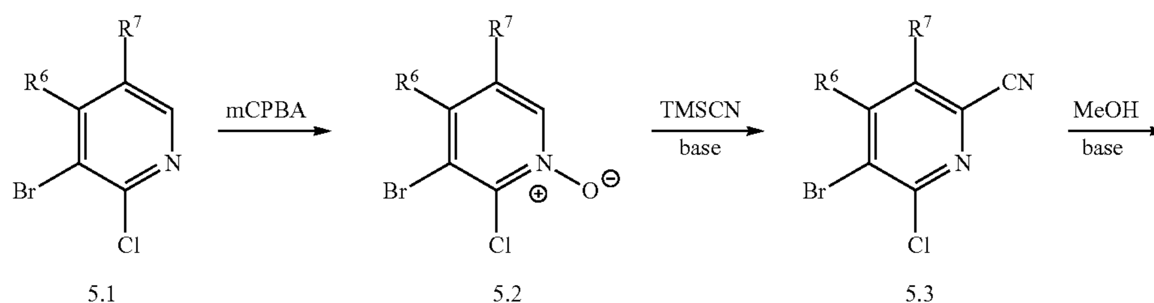
Scheme 5
