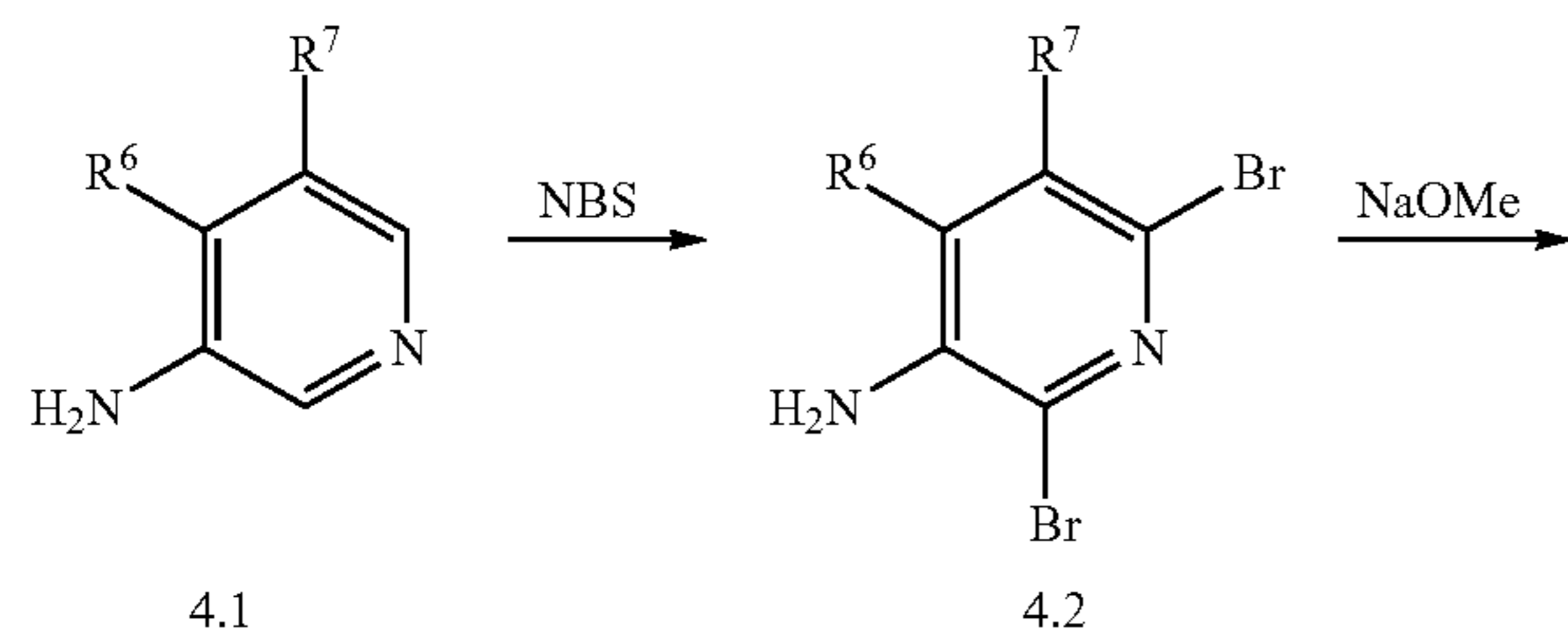
Scheme 4
