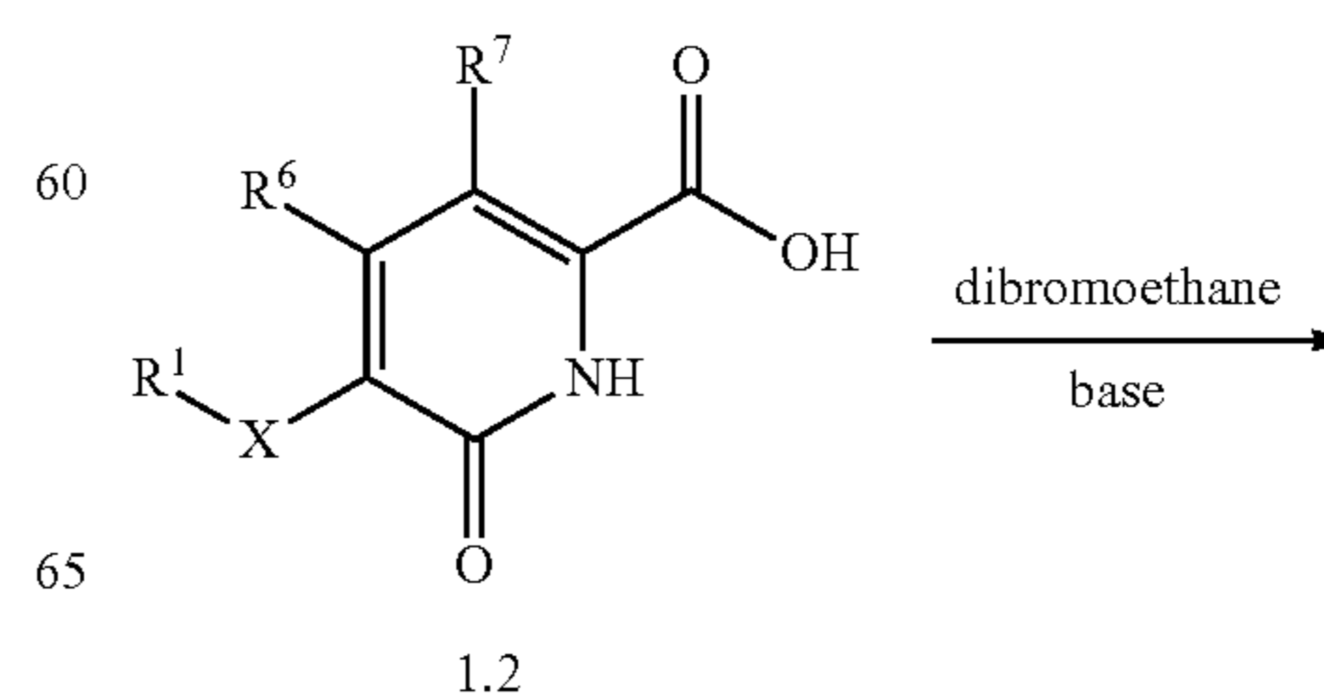
Scheme 7
