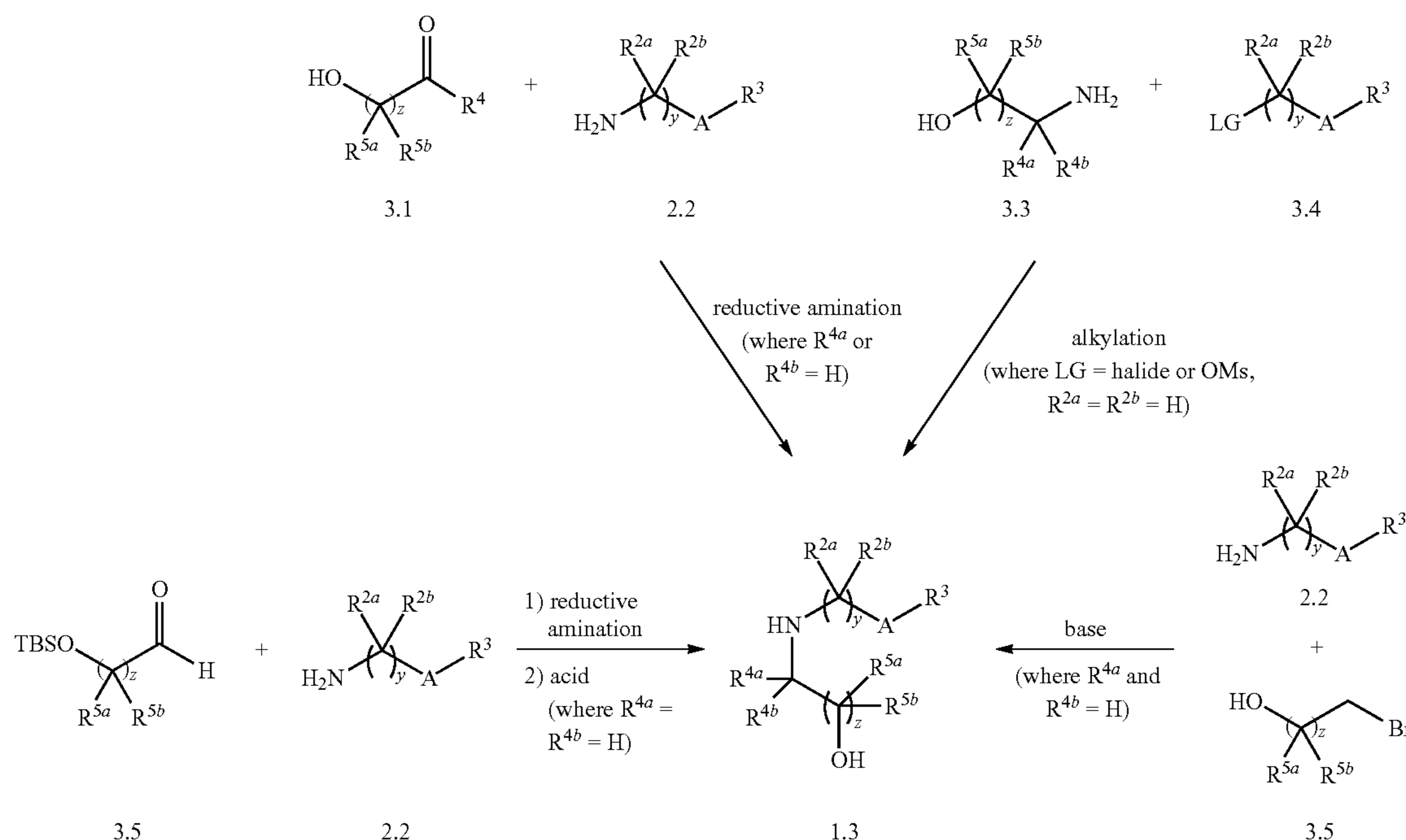
Scheme 3
