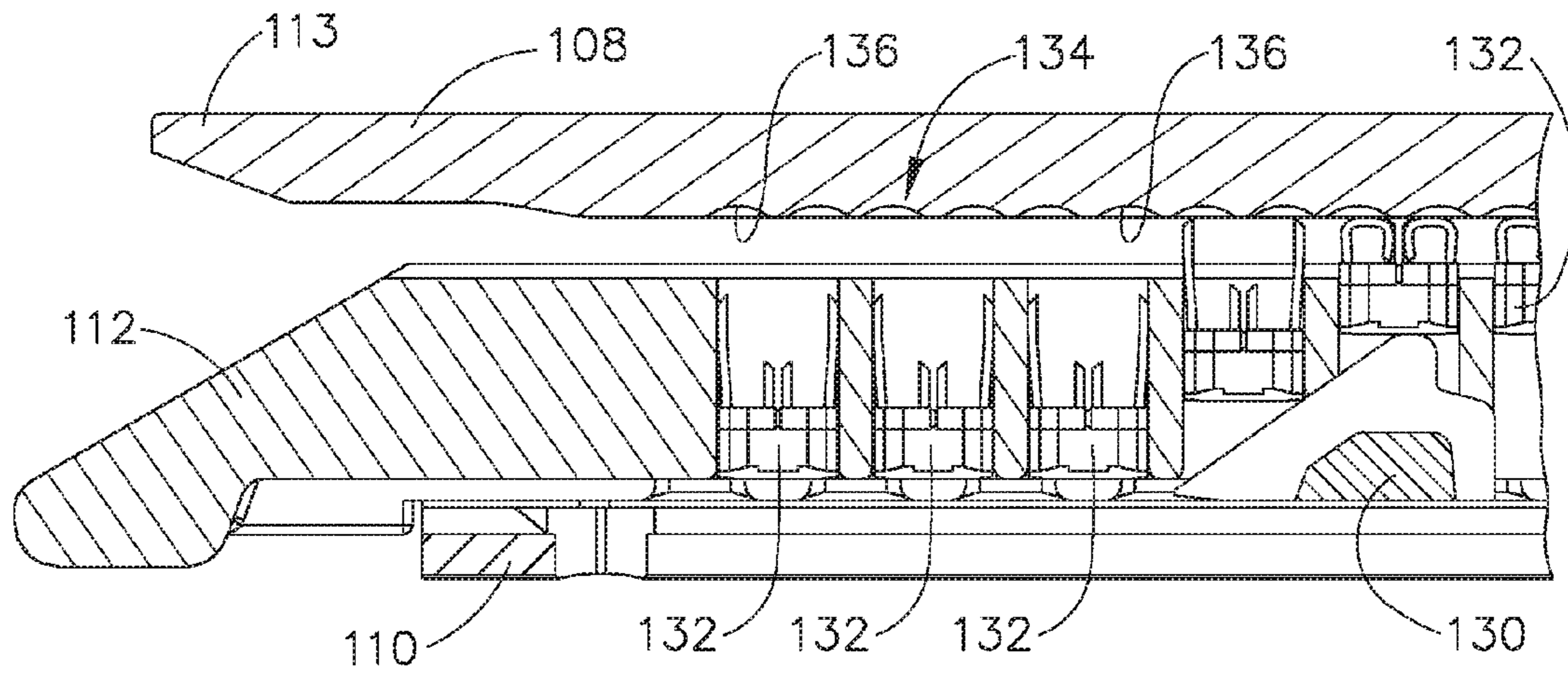
FIG. 6 (PRIOR ART)
