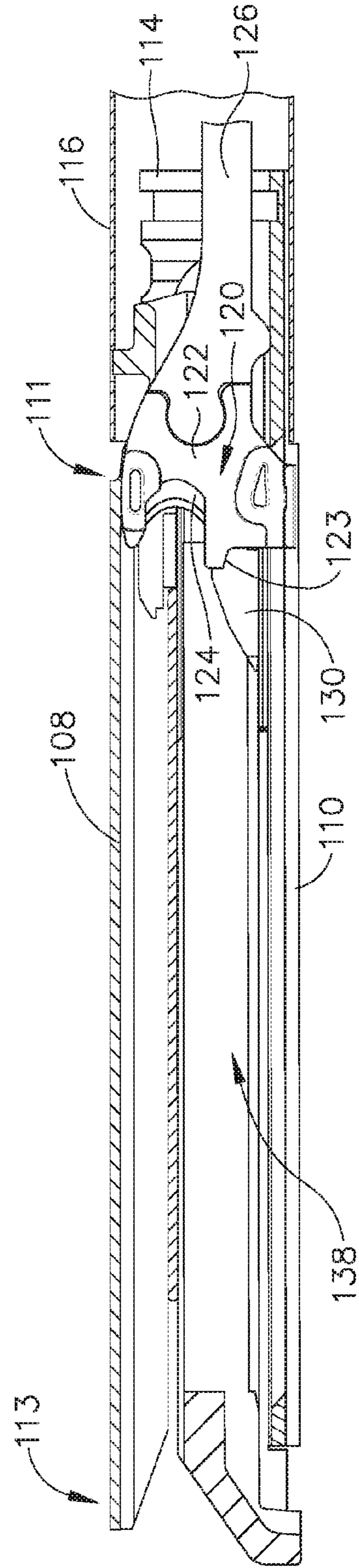
FIG. 3 (PRIOR ART)
