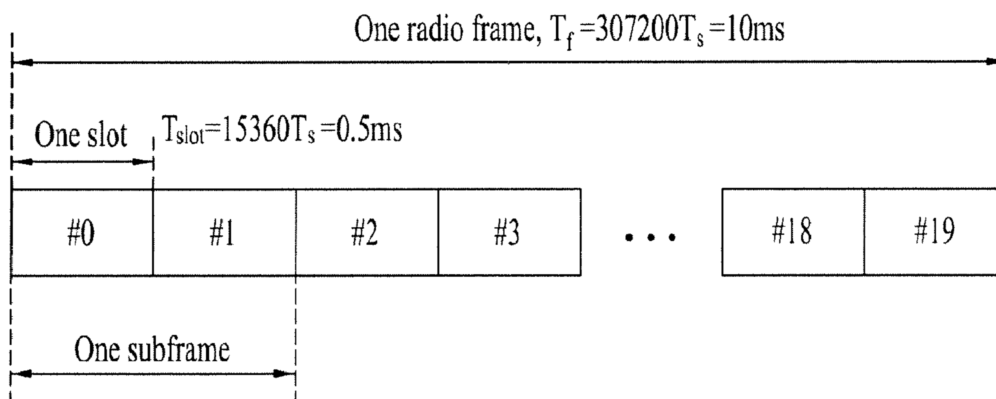
<Frame structure type 1>
