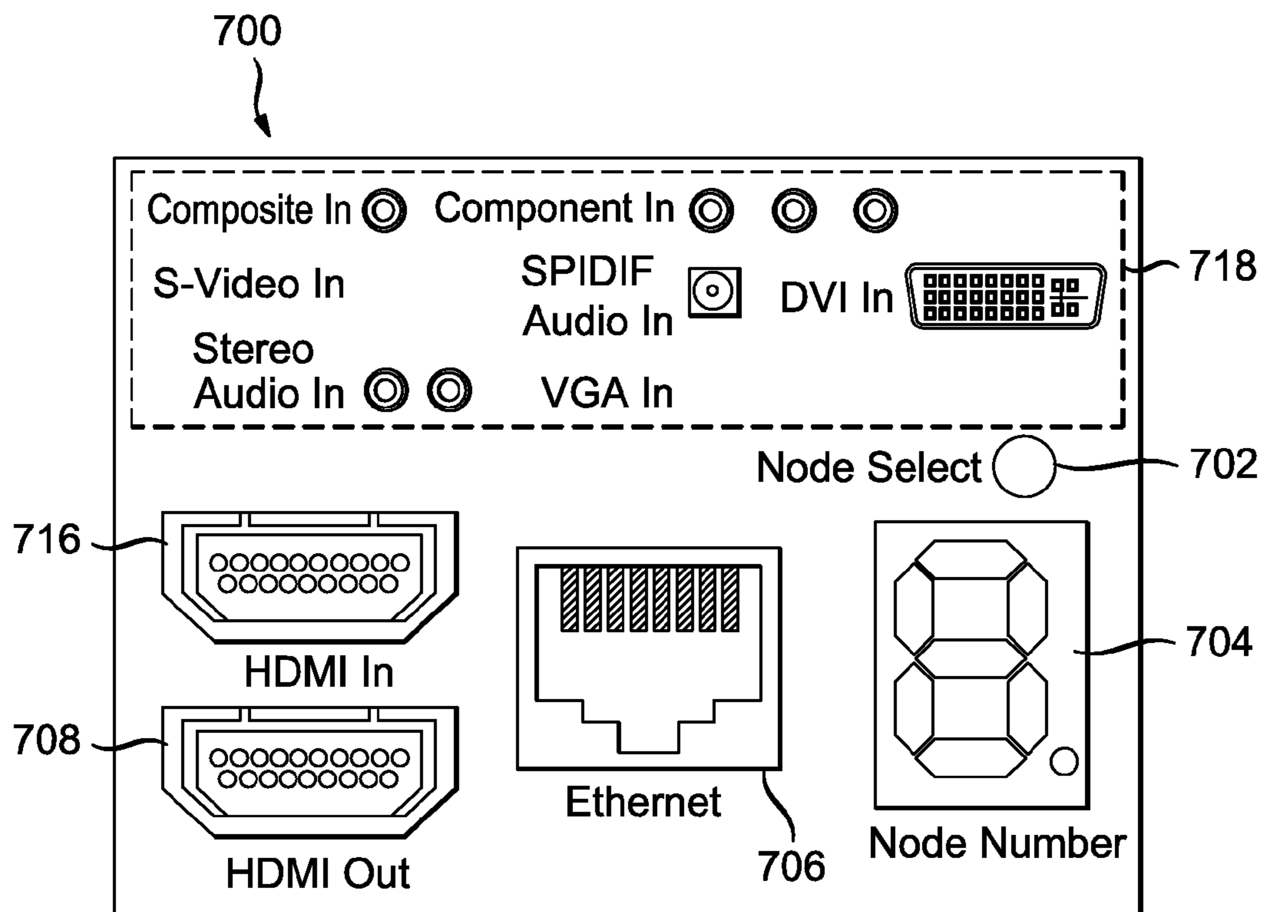
Complex AV Server Device Back Panel with Varied Inputs
