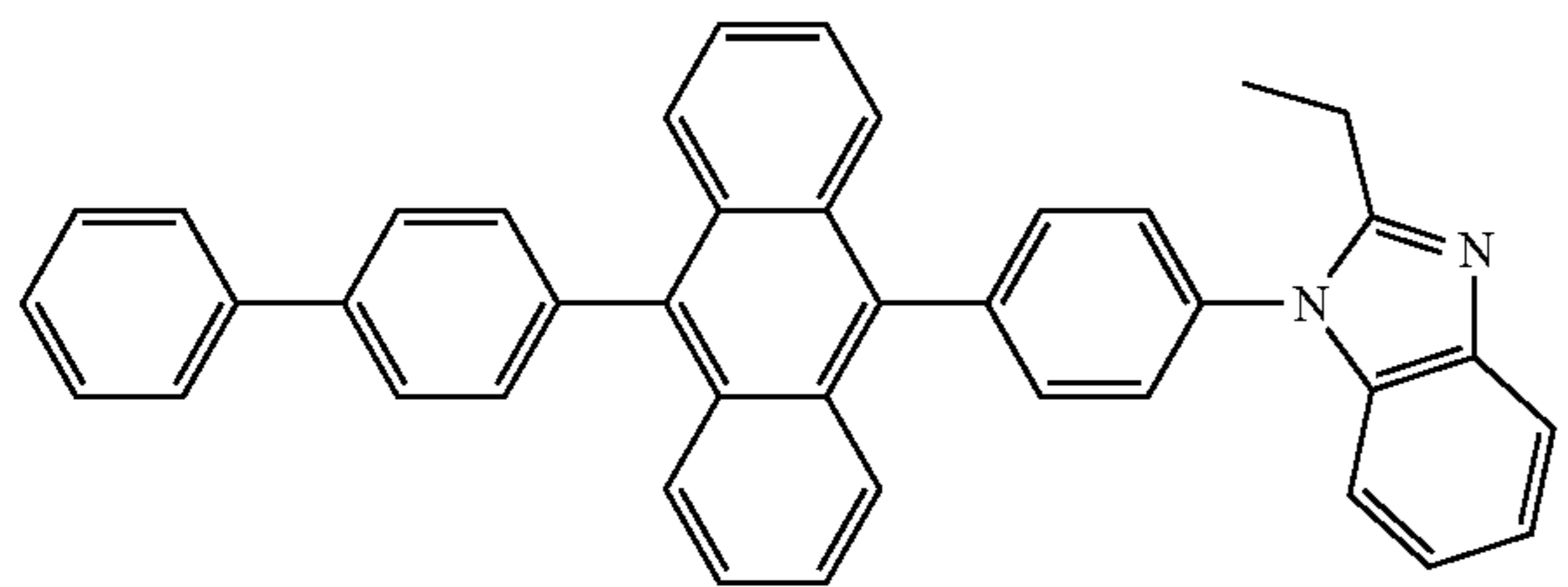
Compound 1
