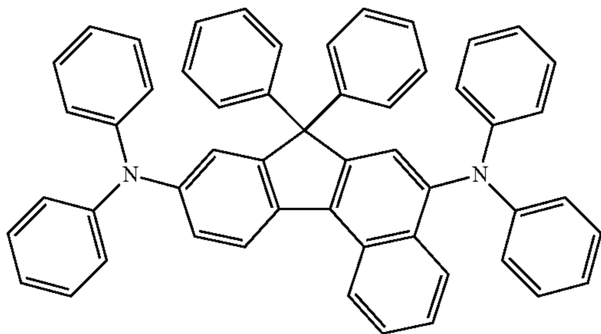
Comparative Compound
