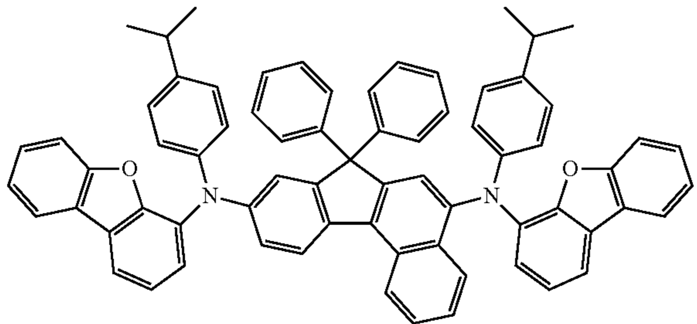
Compound 1
