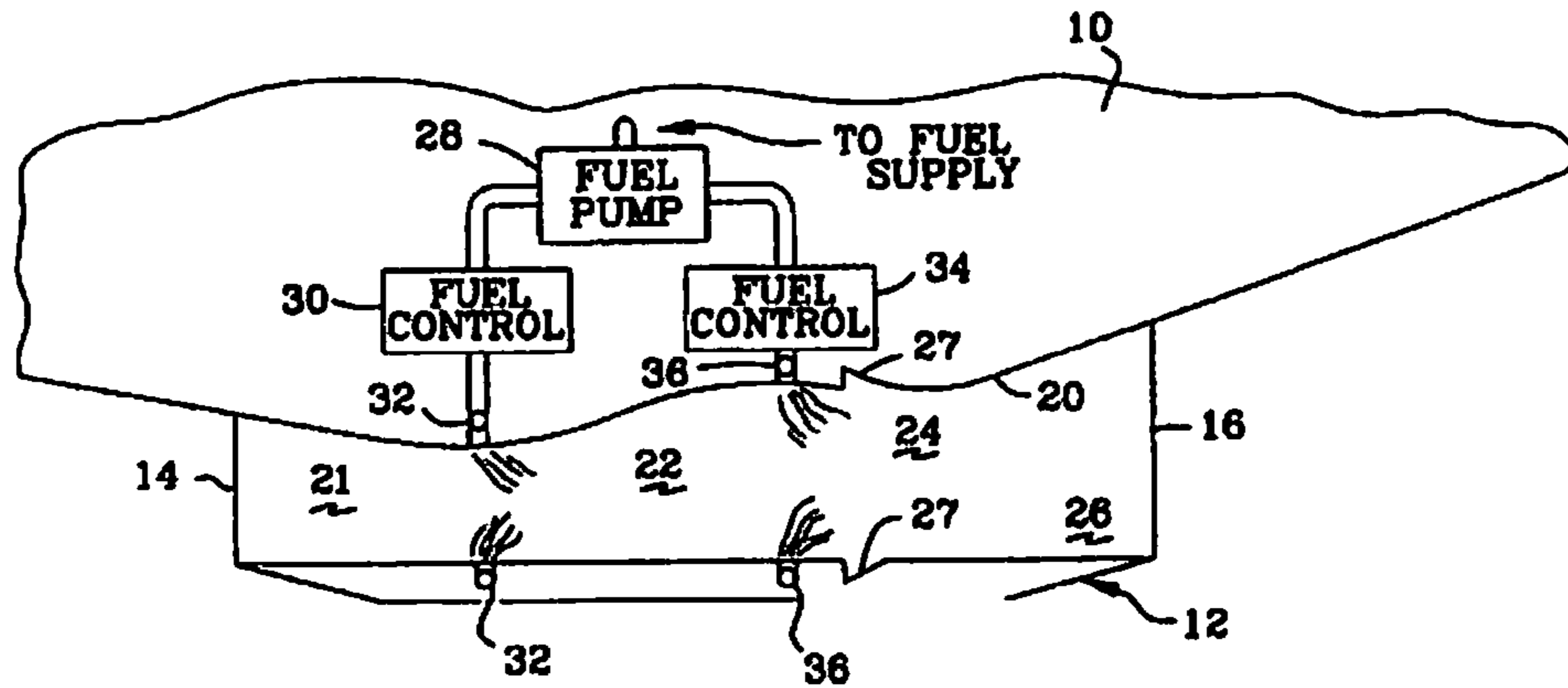
FIG. 1 (Prior Art)
