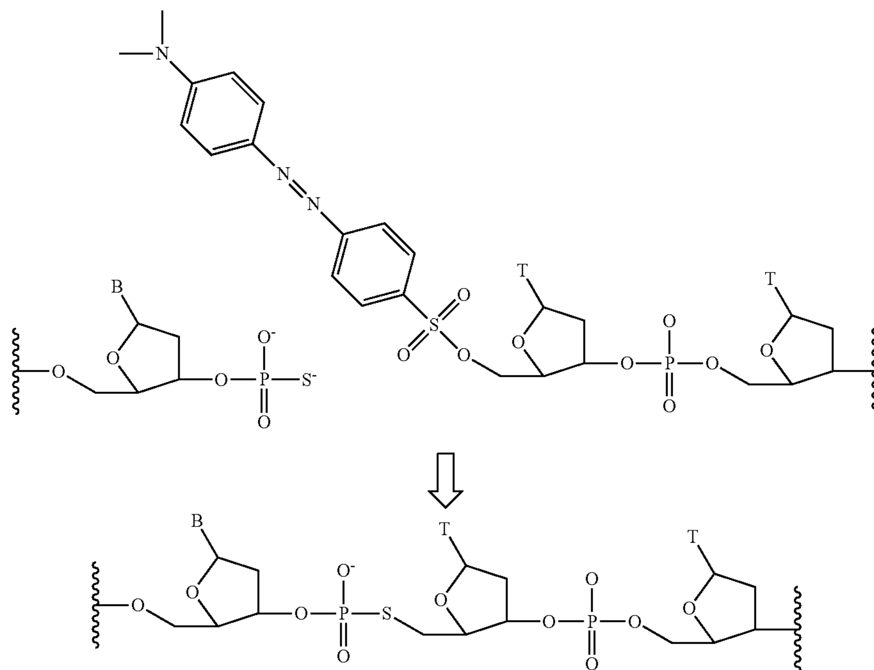
Scheme 1: Chemical ligation reaction between a 3' phosphorothioate oligonucleotide (S-probe) and a 5' DABSYL modified oligonucleotide (L-probe).
