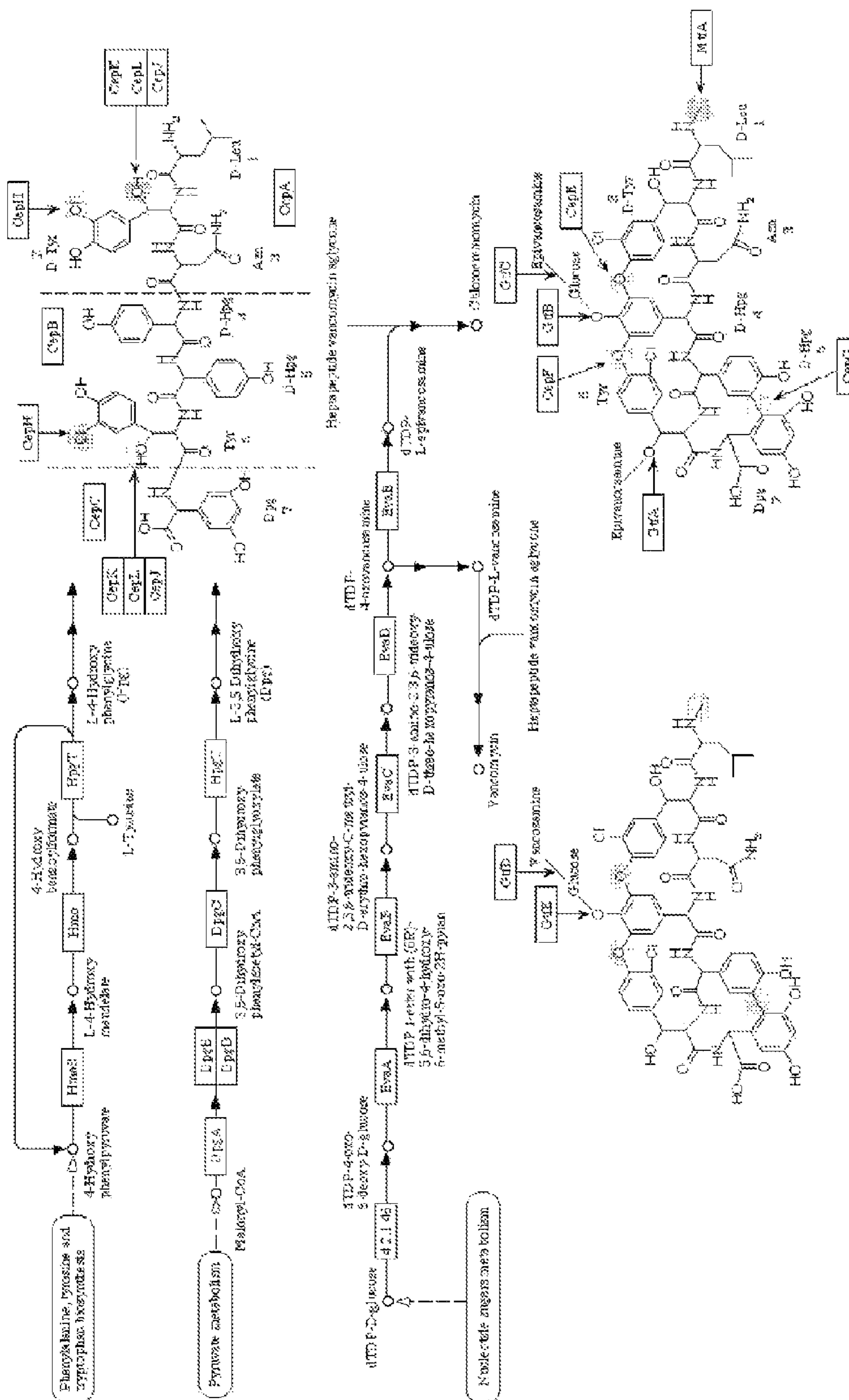
Biosynthesis of Vancomycin
