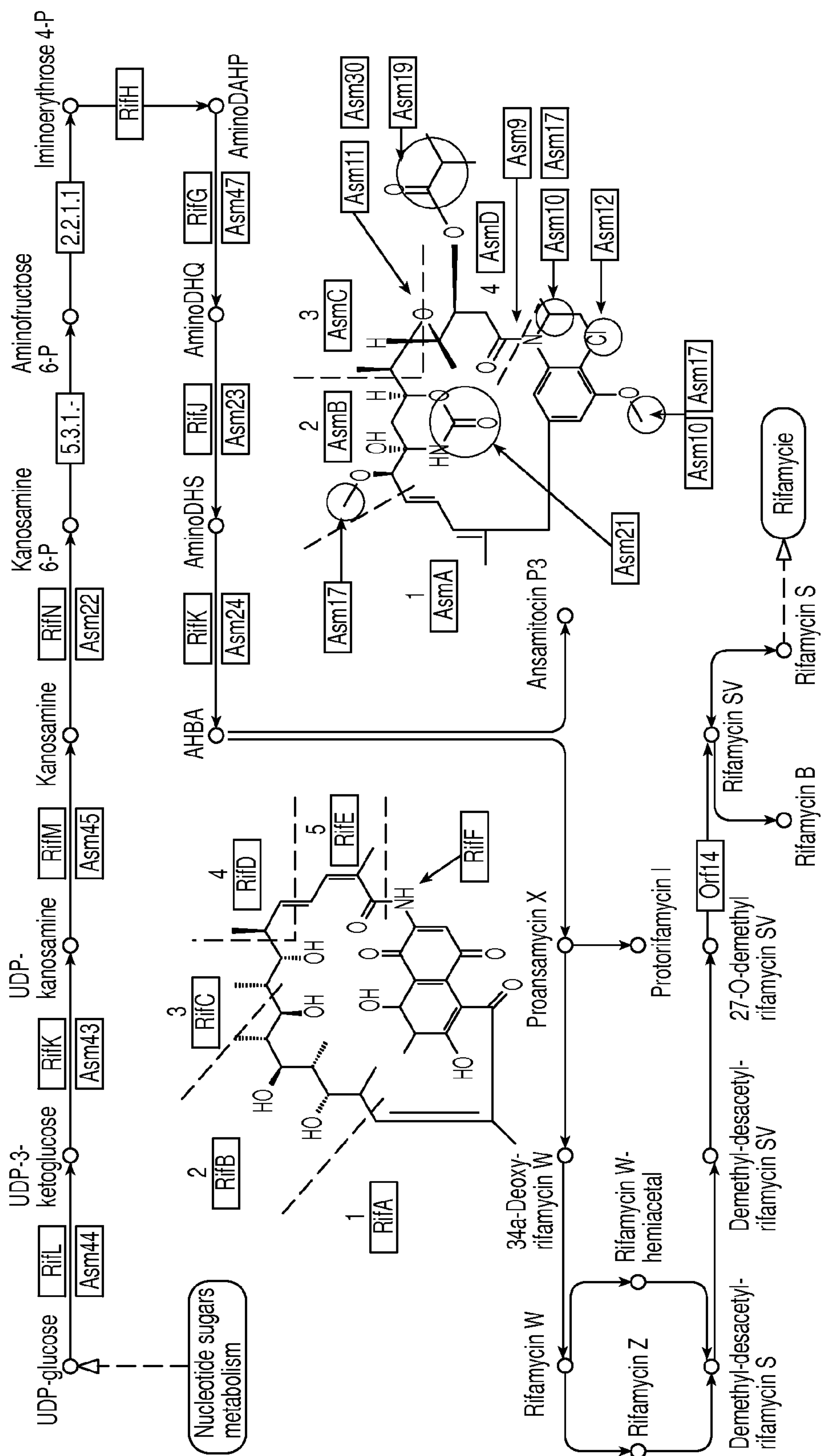
Ansamycin Biosynthesis
