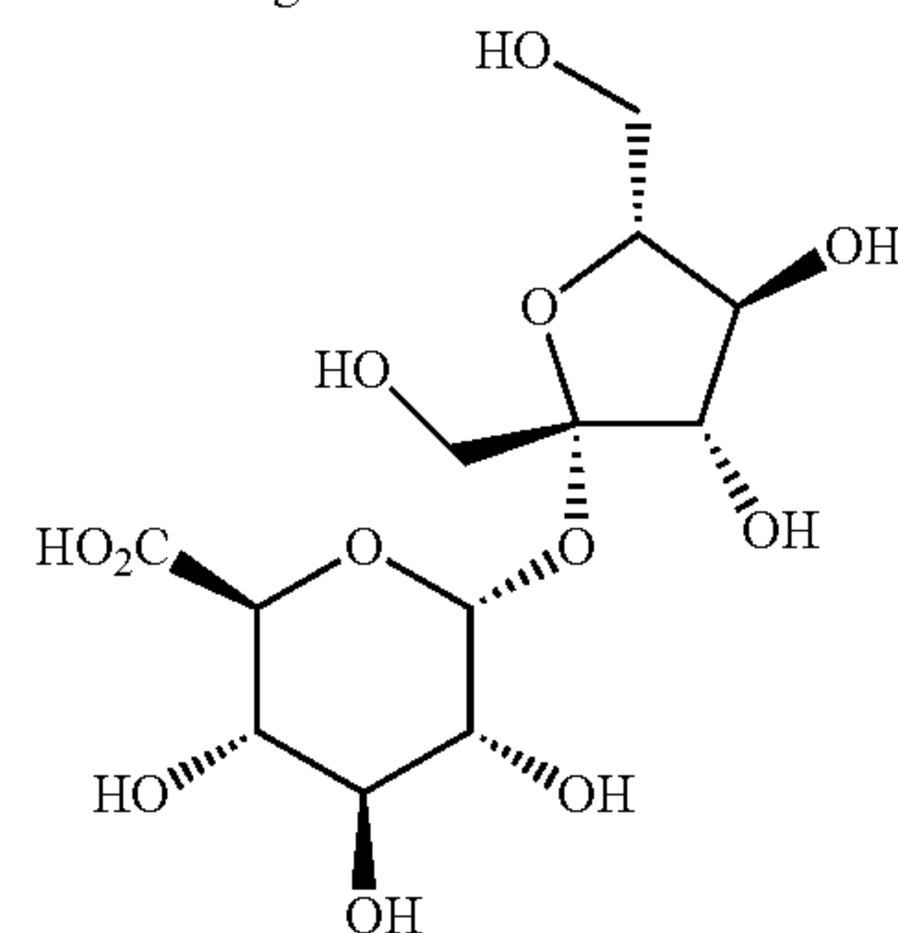
6-MAS 6-monoacid of sucrose
