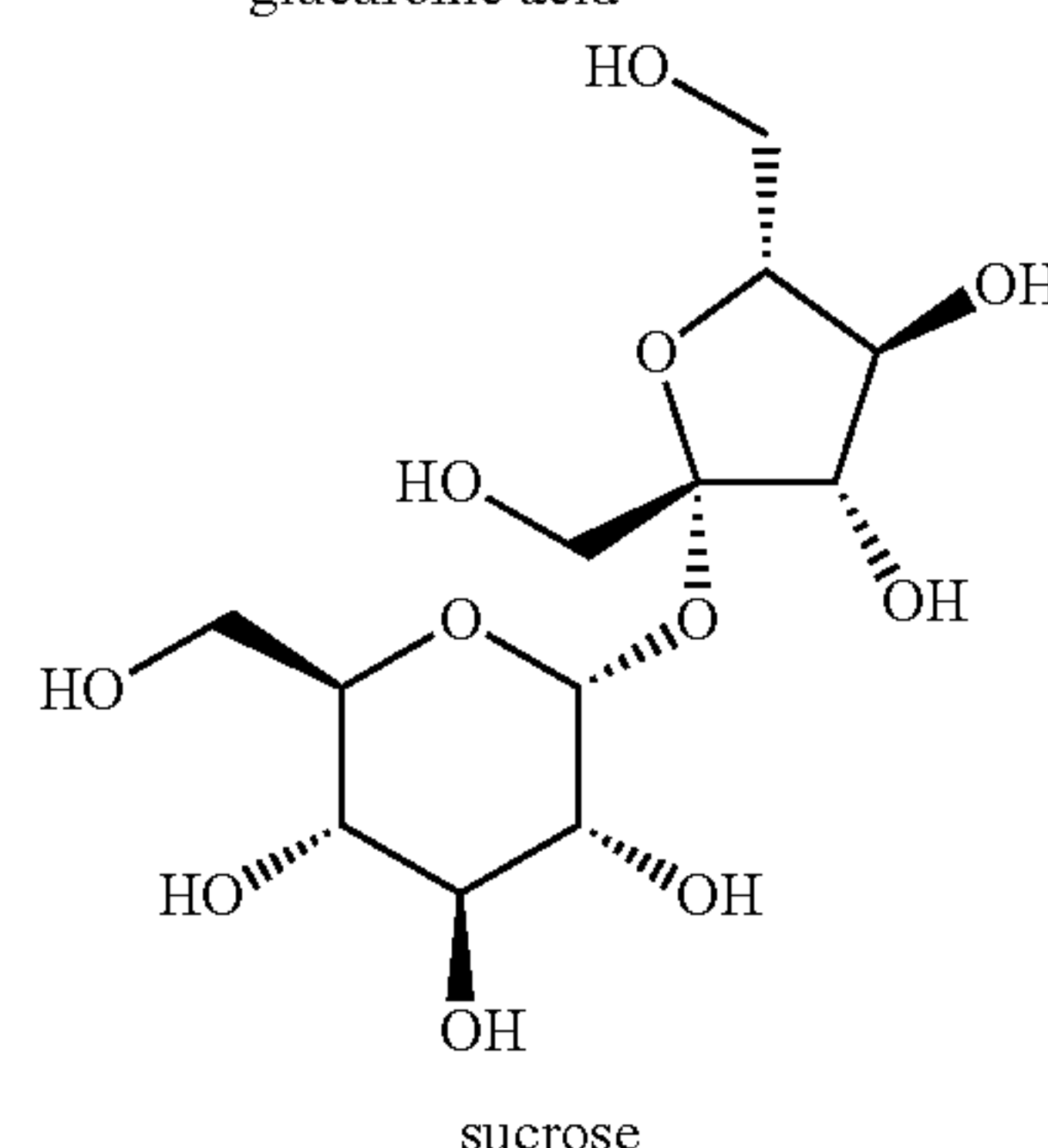
sucrose
