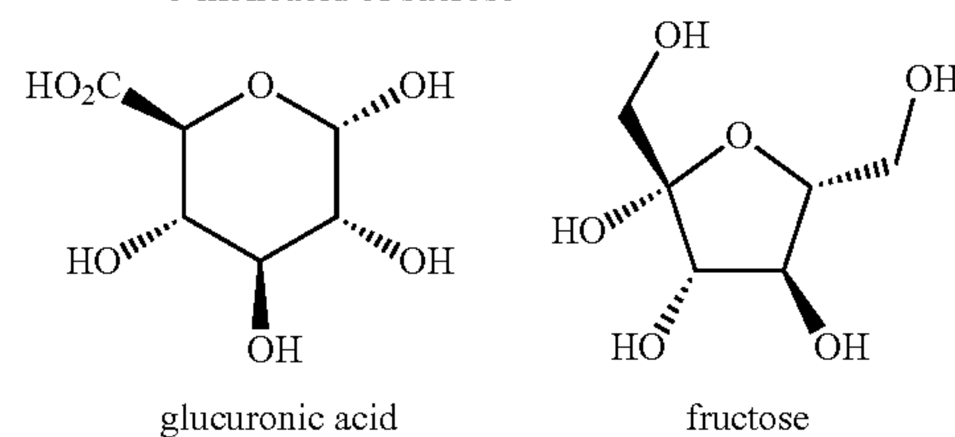
6-MAS 6-monoacid of sucrose
