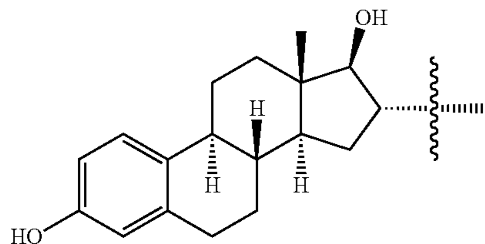
16-substituted estriol
