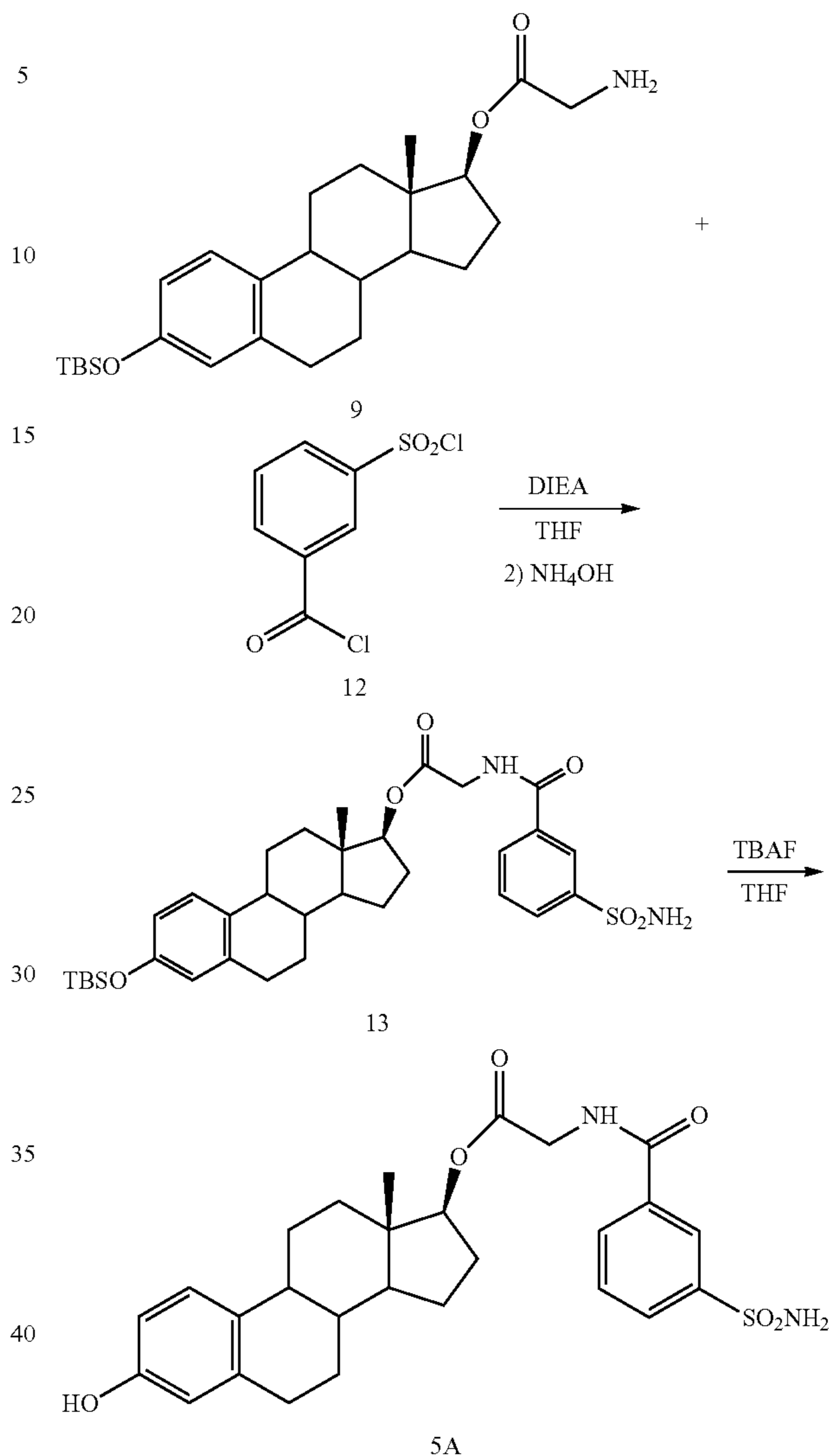
Scheme 6
