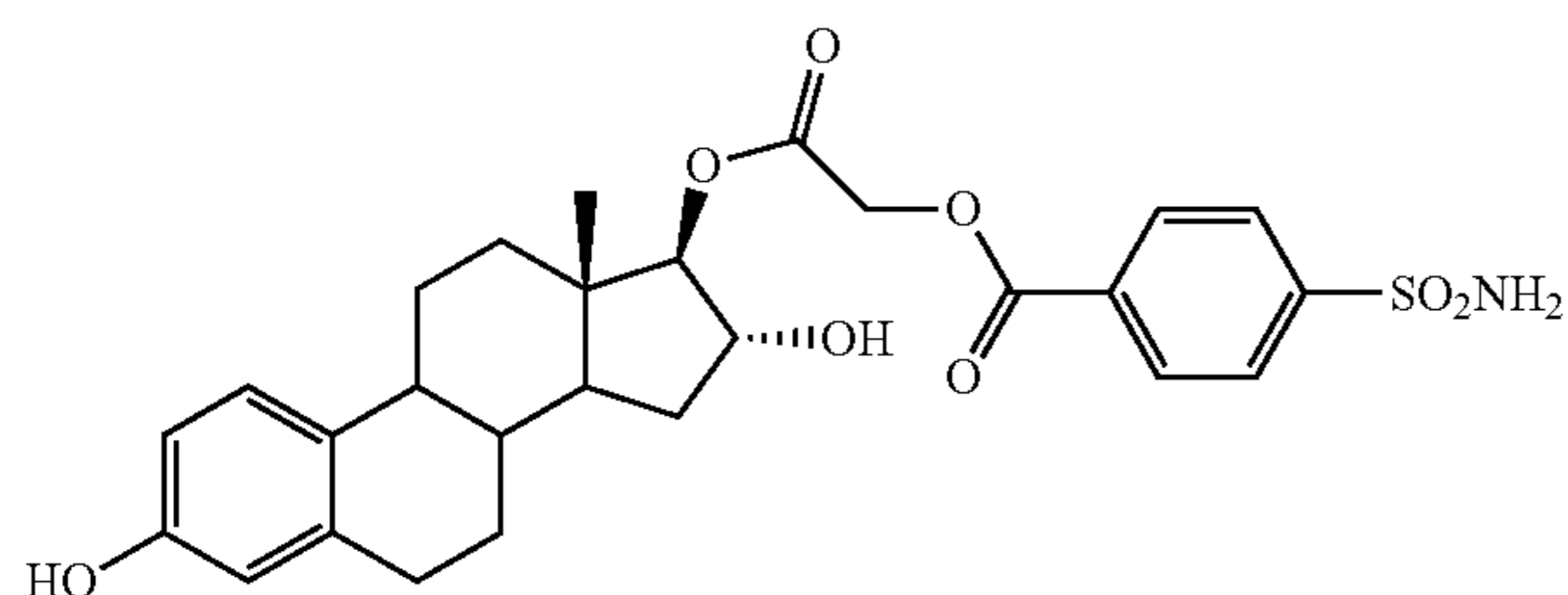
2-((13S,16R,17R)-3,16-dihydroxy-13-methyl-7,8,9,11,12,13,14,15,16,17-decahydro-6H-cyclopenta[a]phenanthren-17-yloxy)-2-oxoethyl 4-sulfamoylbenzoate
