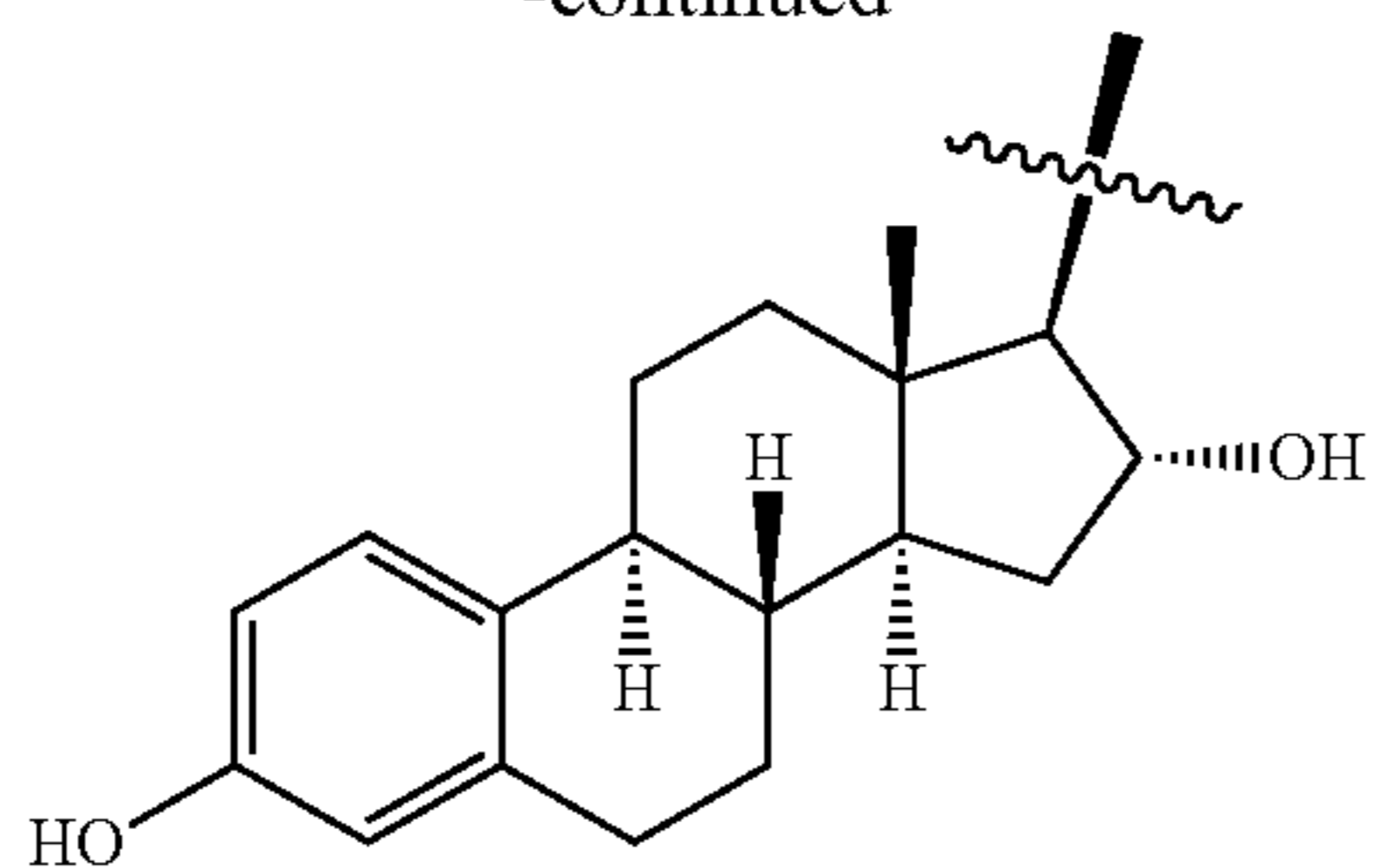
17-substituted estriol
