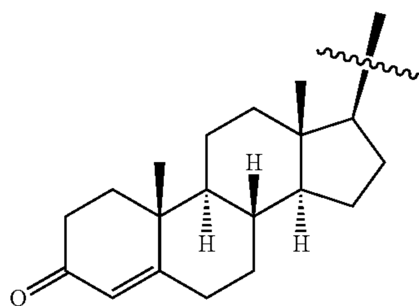
testosterone
