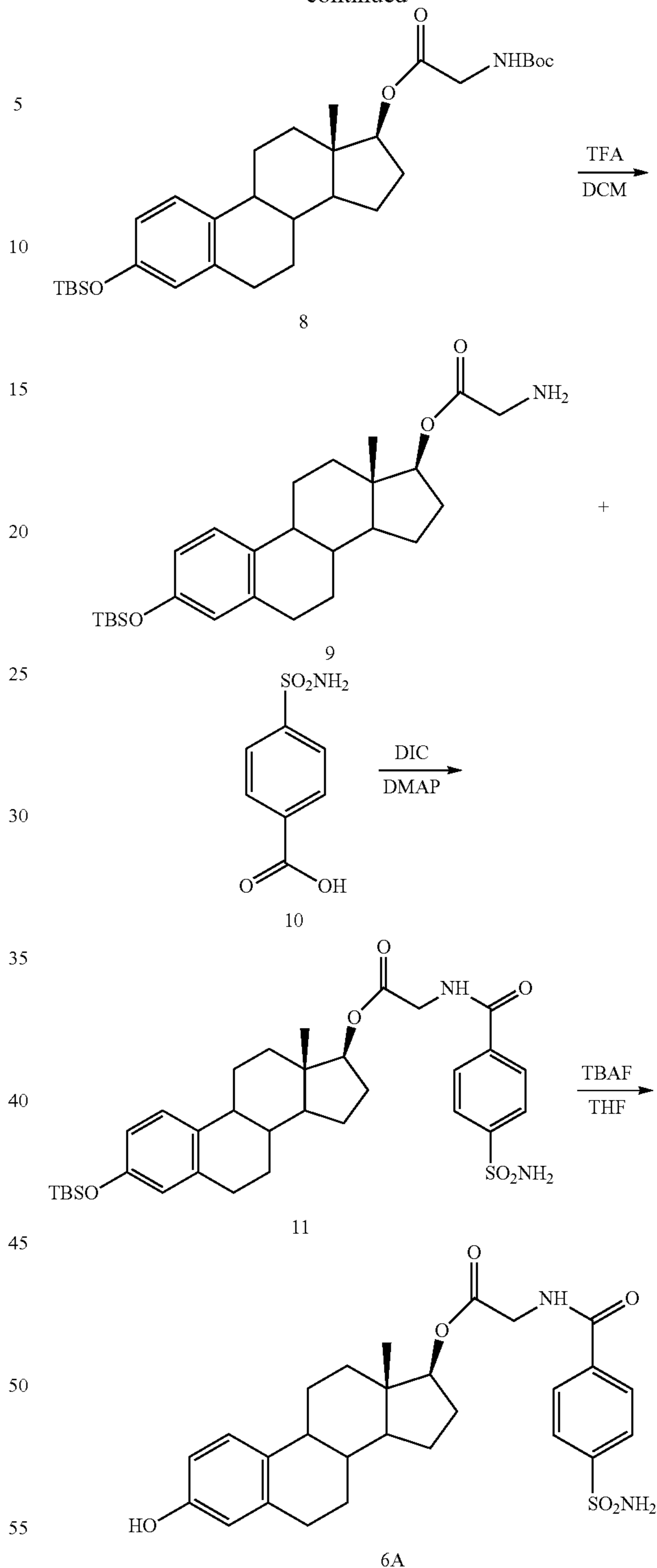
2-((13S,16R,17R)-3,16-dihydroxy-13-methyl-7,8,9,11,12,13,14,15,16,17-decahydro-6H-cyclopenta[a]phenanthren-17-yloxy)-2-oxoethyl 4-sulfamoylbenzoate
