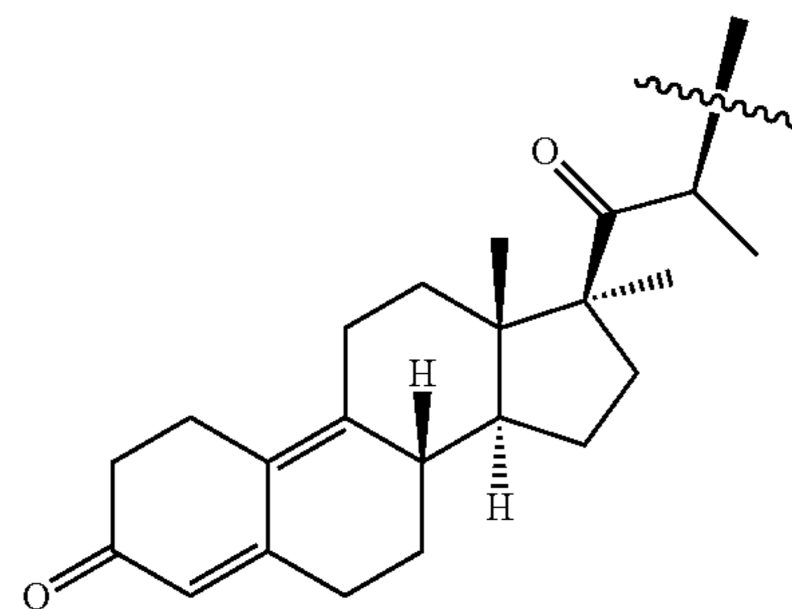
trimegestone
