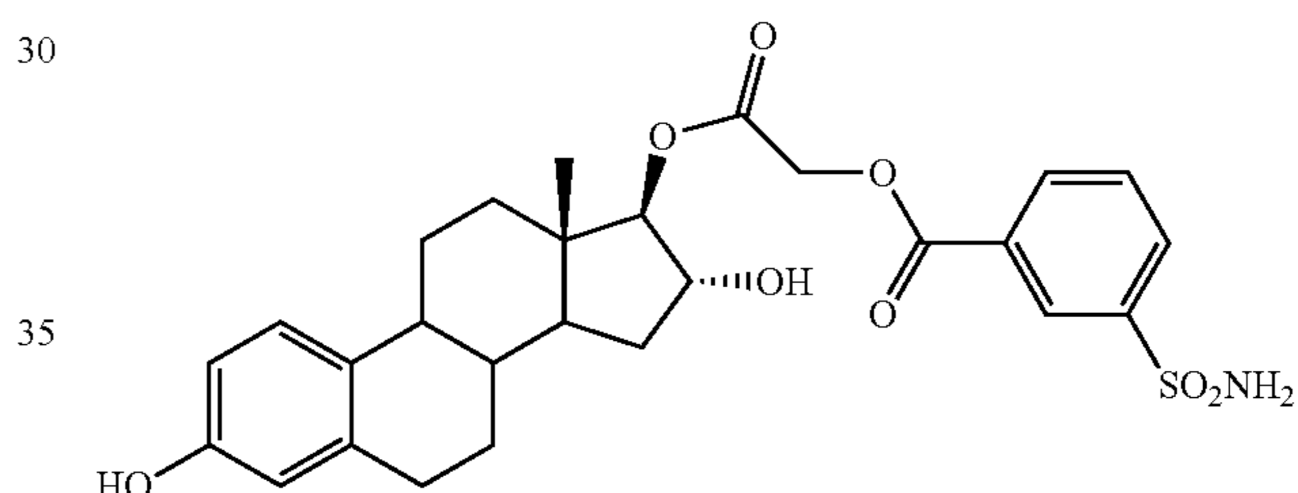
2-((13S,16R,17R)-3,16-dihydroxy-13-methyl-7,8,9,11,12,13,14,15,16,17-decahydro-6H-cyclopenta[a]phenanthren-17-yloxy)-2-oxoethyl 3-sulfamoylbenzoate
