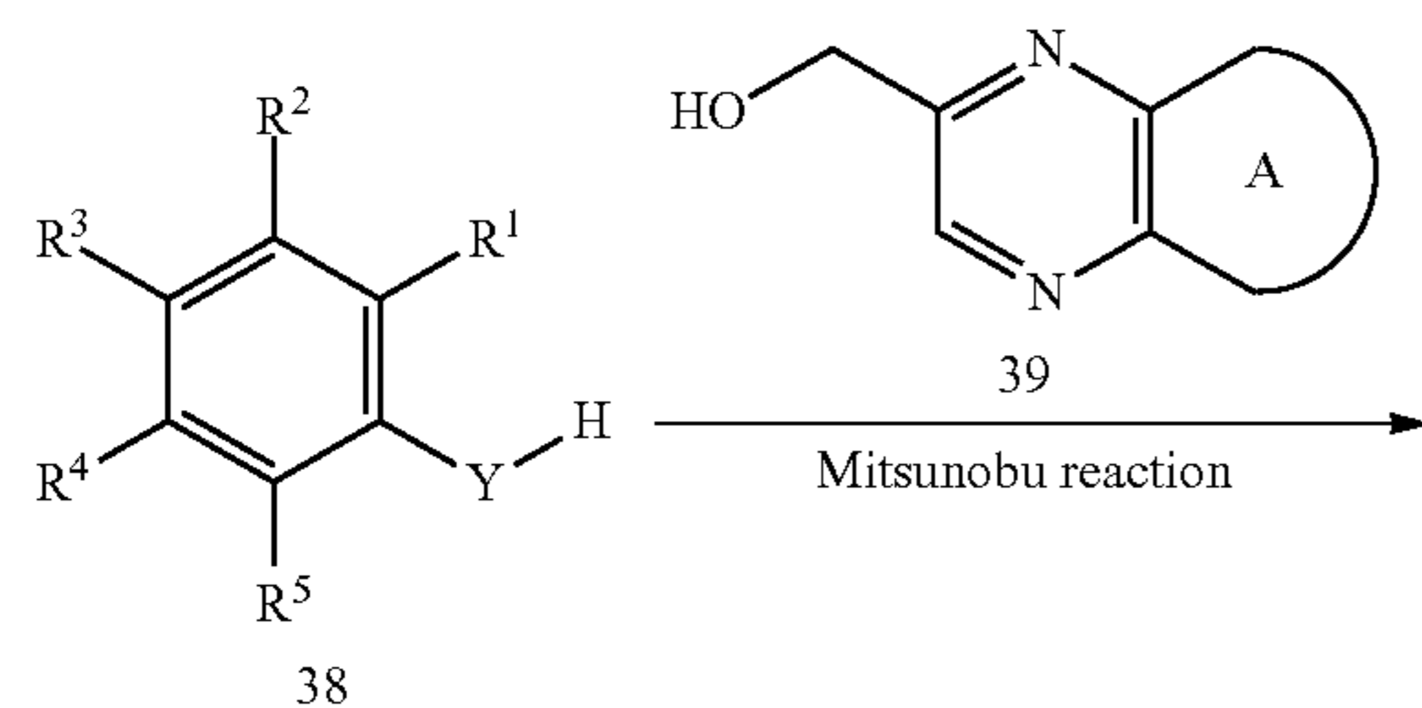
Scheme 13
