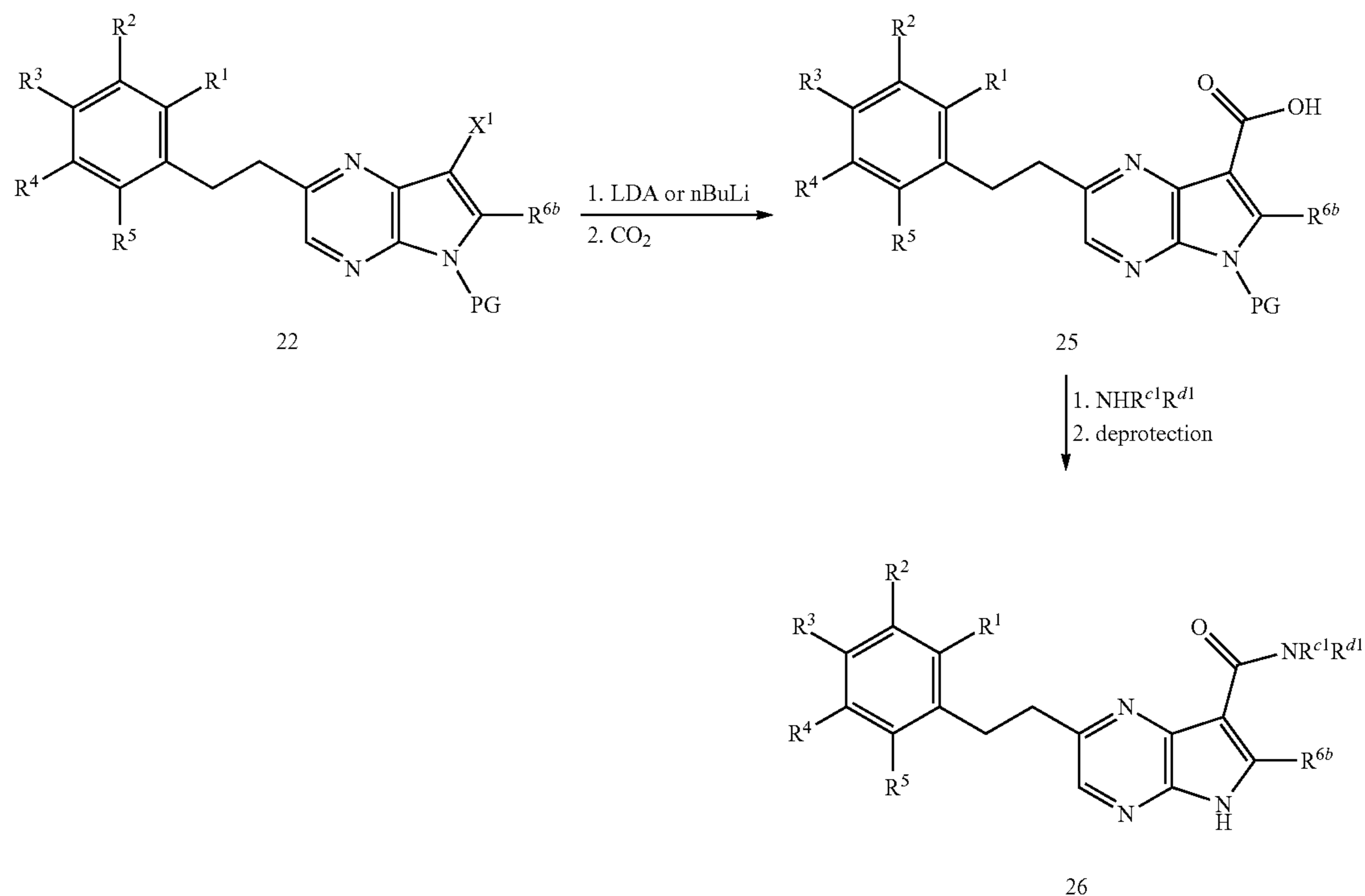
Scheme 8
