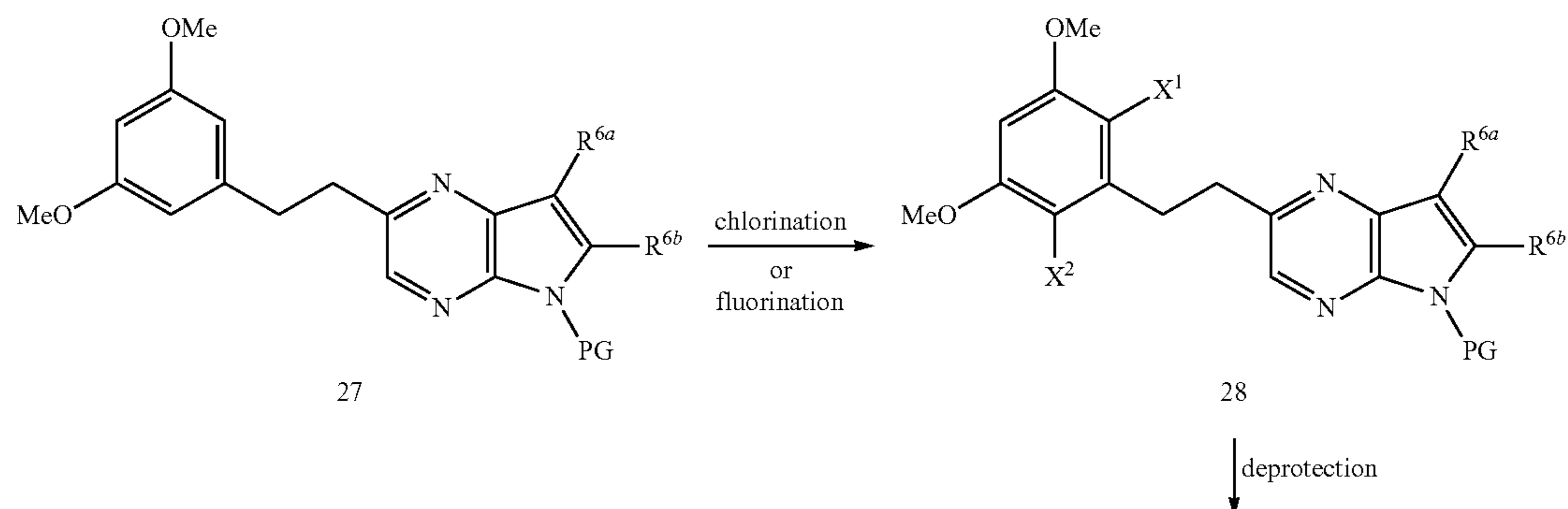
Scheme 9
