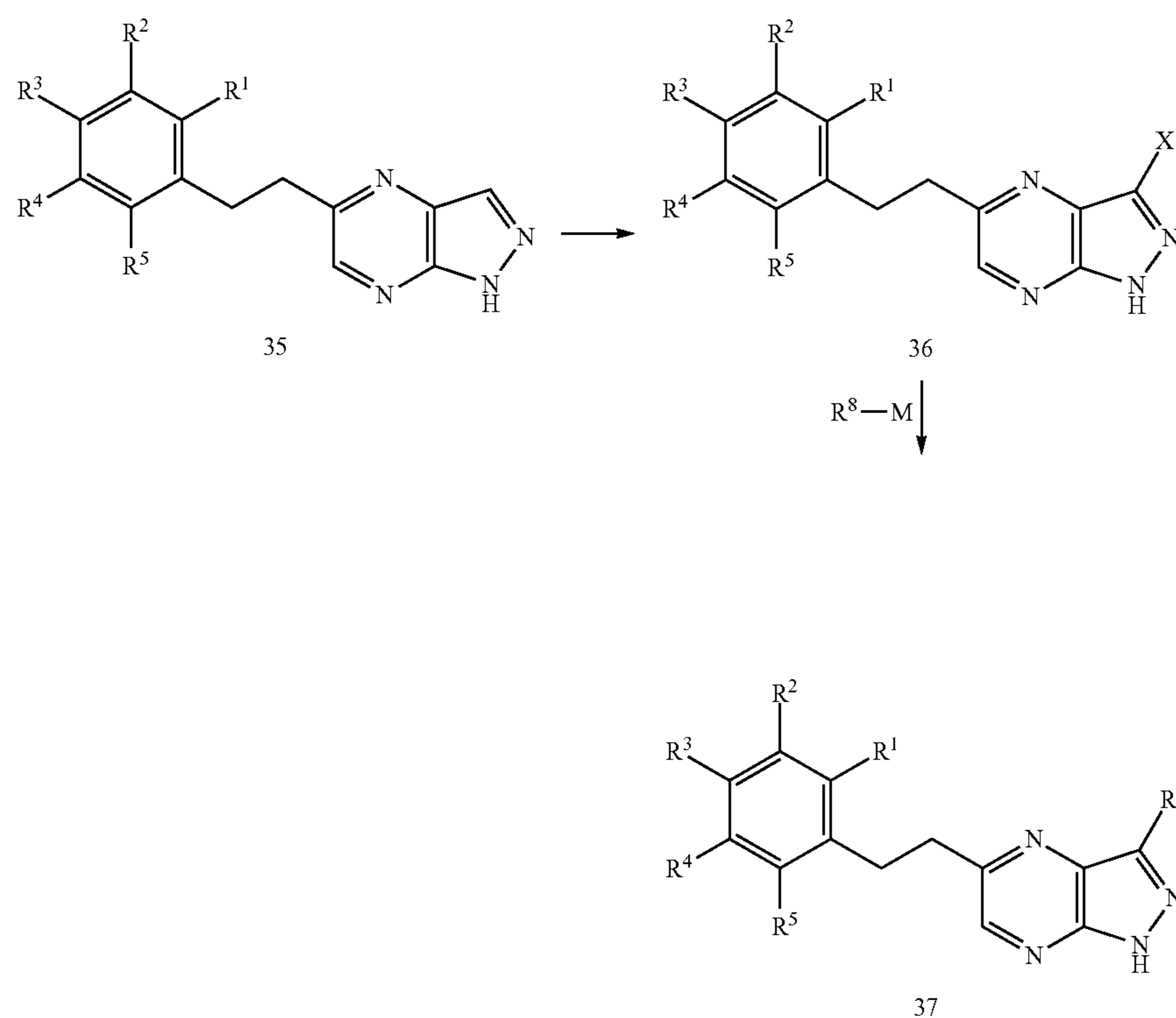
Scheme 12
