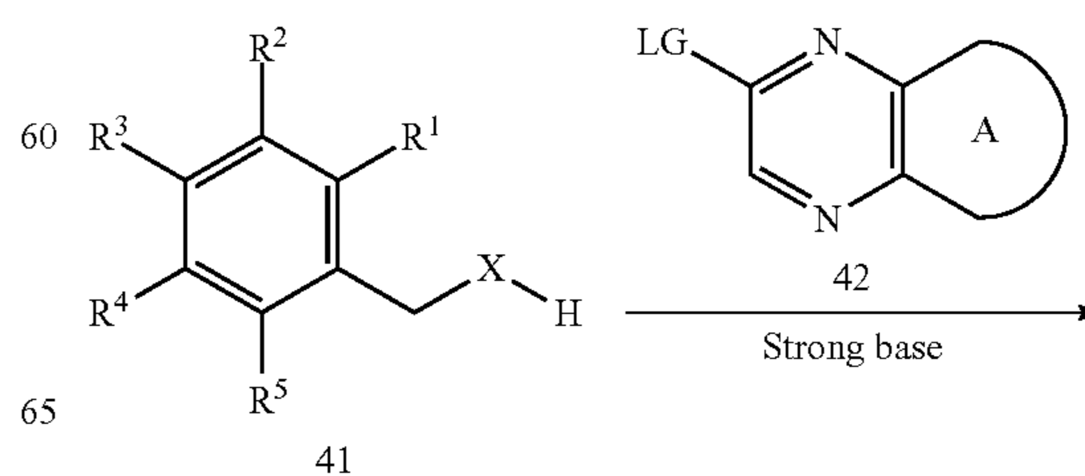
Scheme 14
