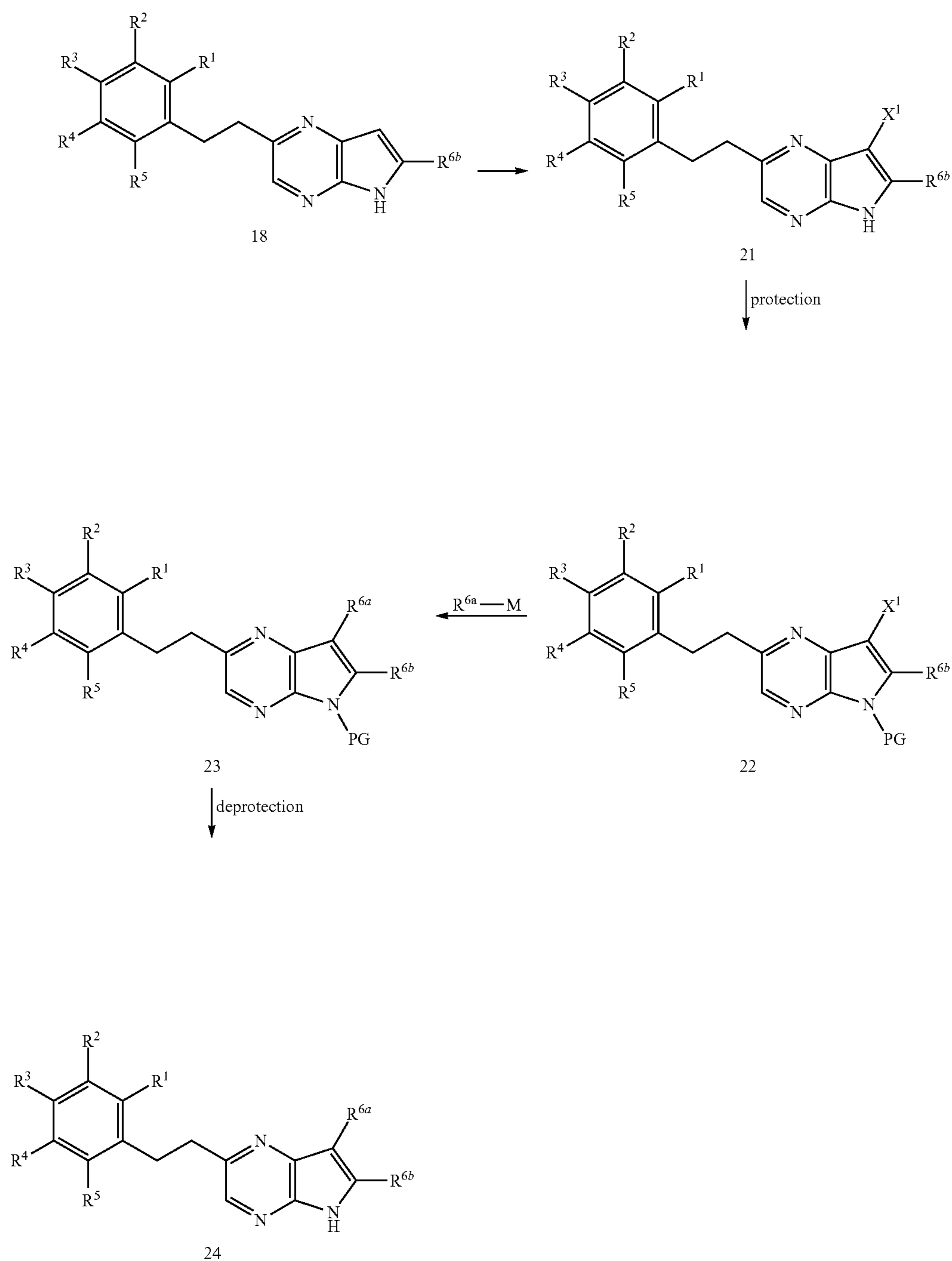
Scheme 7
