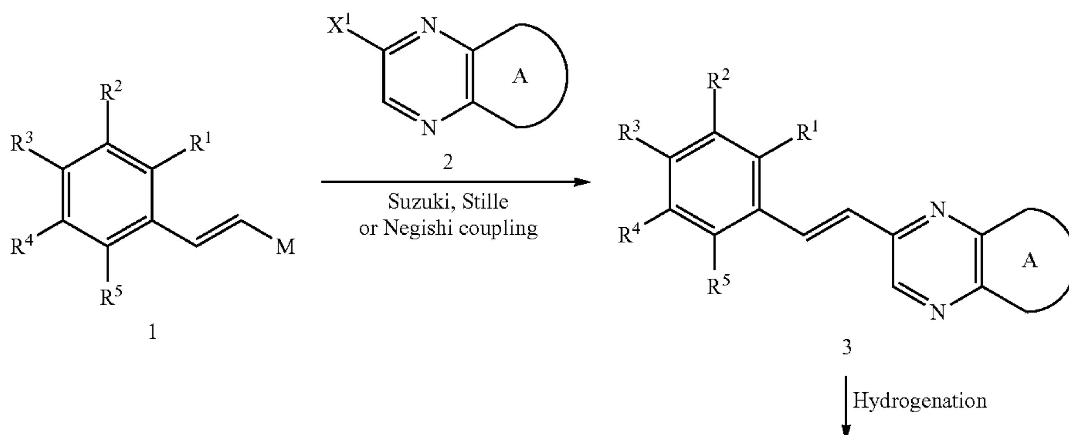
Scheme 1
