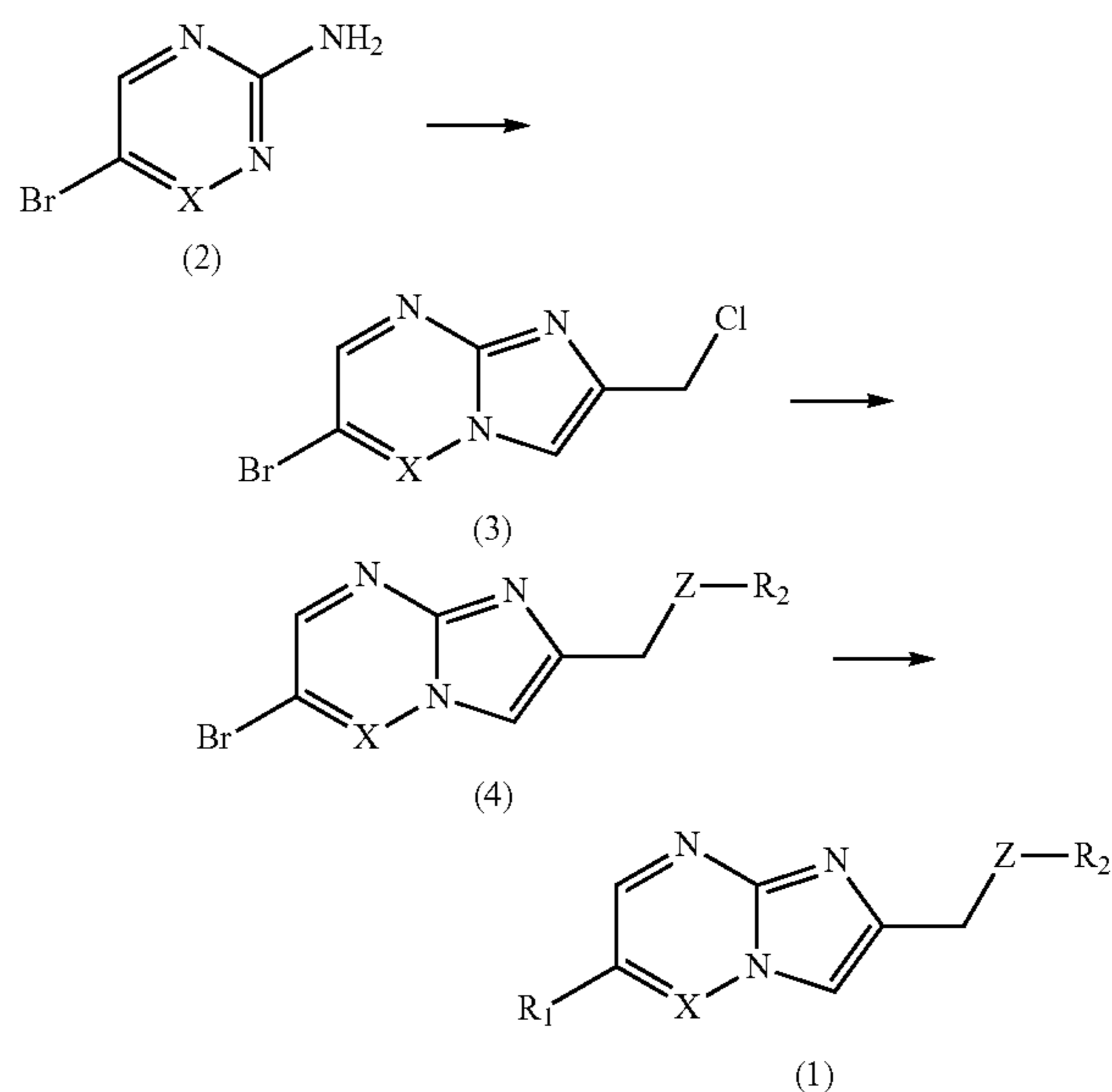
[Reaction Scheme 1]
