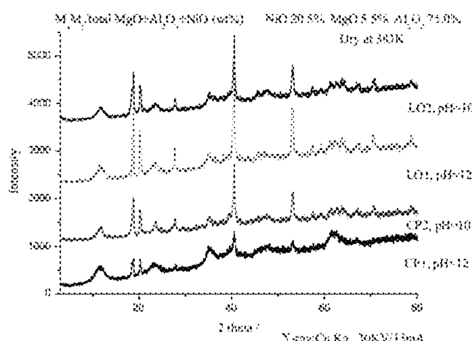
XRD patterns of LDH uncalined materials: Comparison for coprecipitation and impregnation techniques
