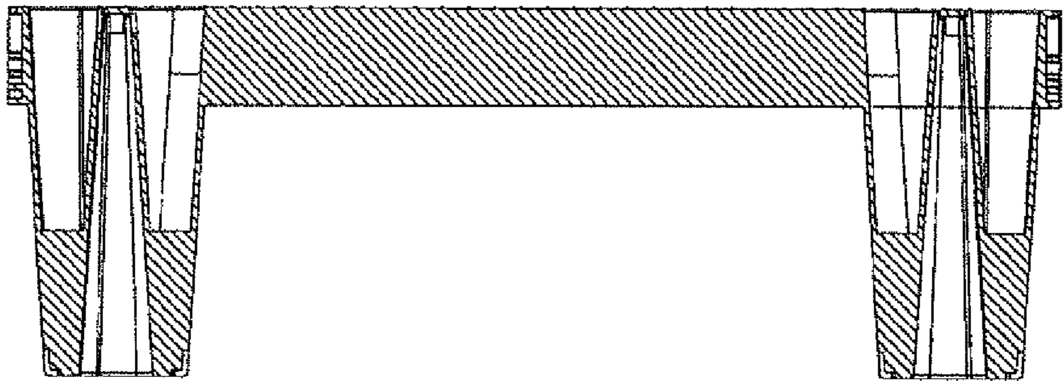
Fig. 82 Section C-C
