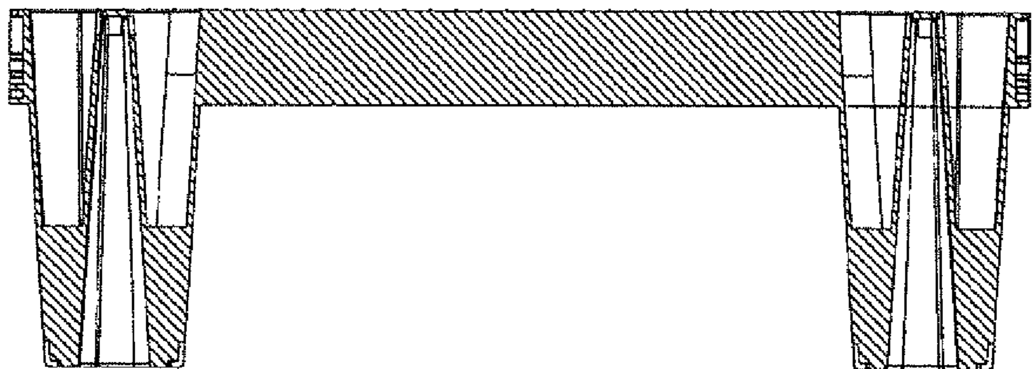
Fig. 82 Section C-C
