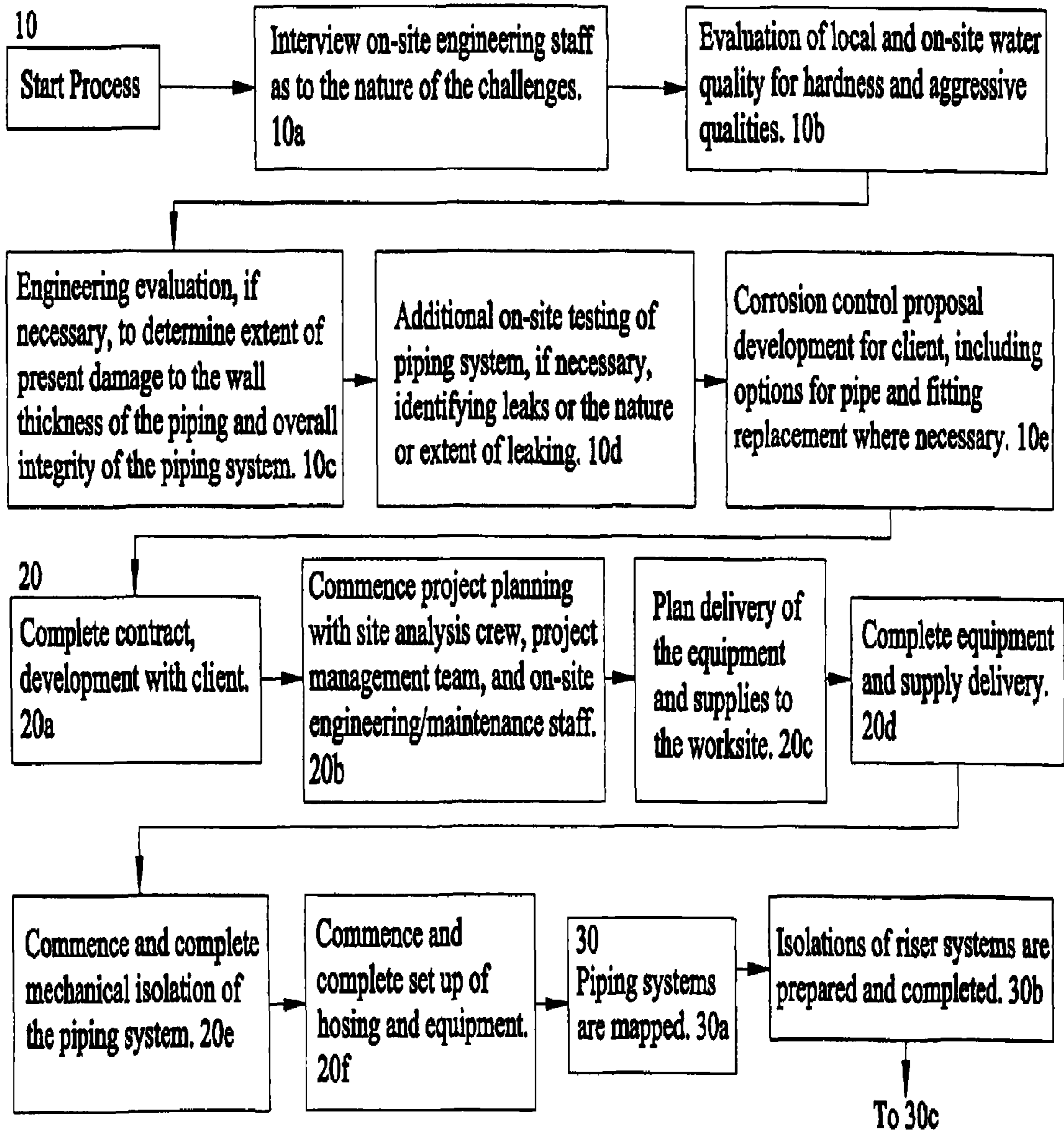
Fig. 2A PROCESS FLOWCHART
