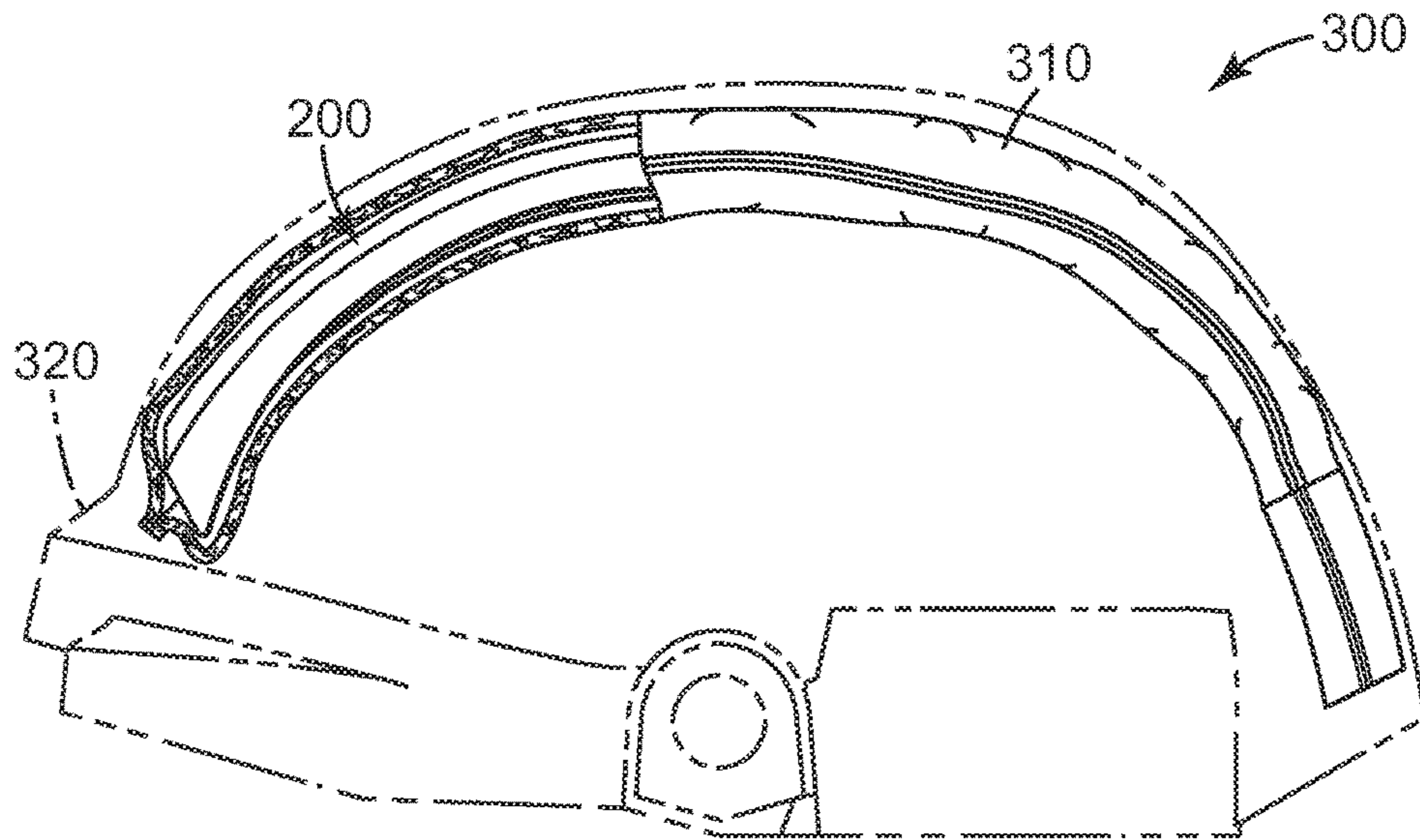
Fig. 3 PRIOR ART
