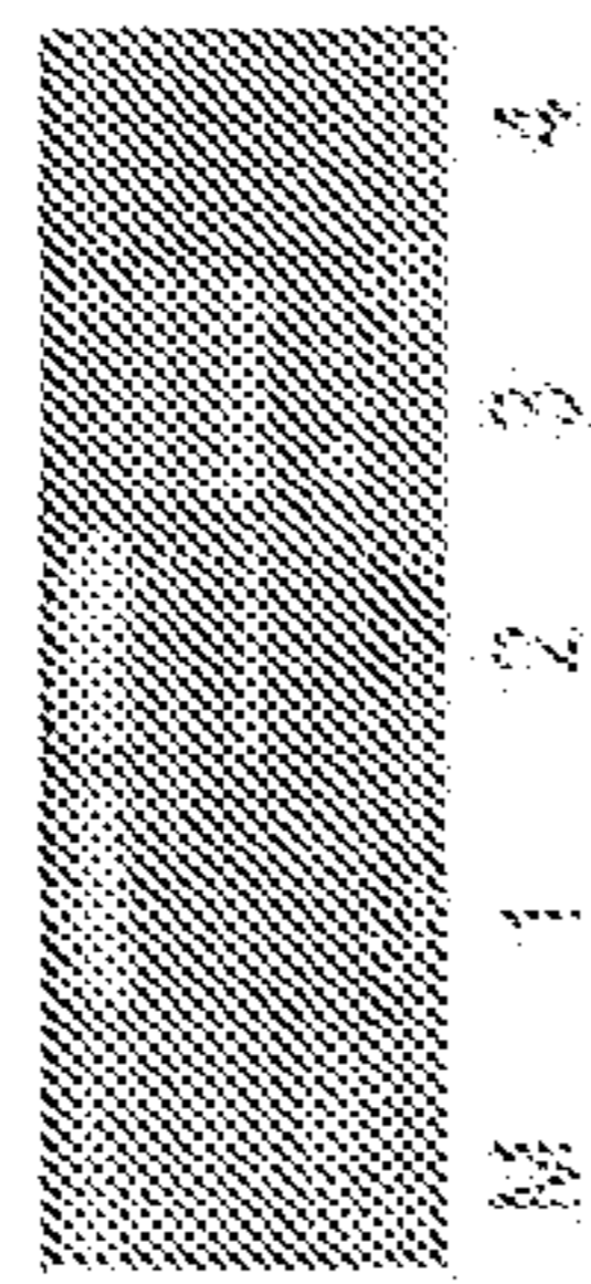
M: MARKER; 1: AAV; 2: AAV/GFP 3: PCR FOR AAV/GFP; 4: NO TEMPLATE
