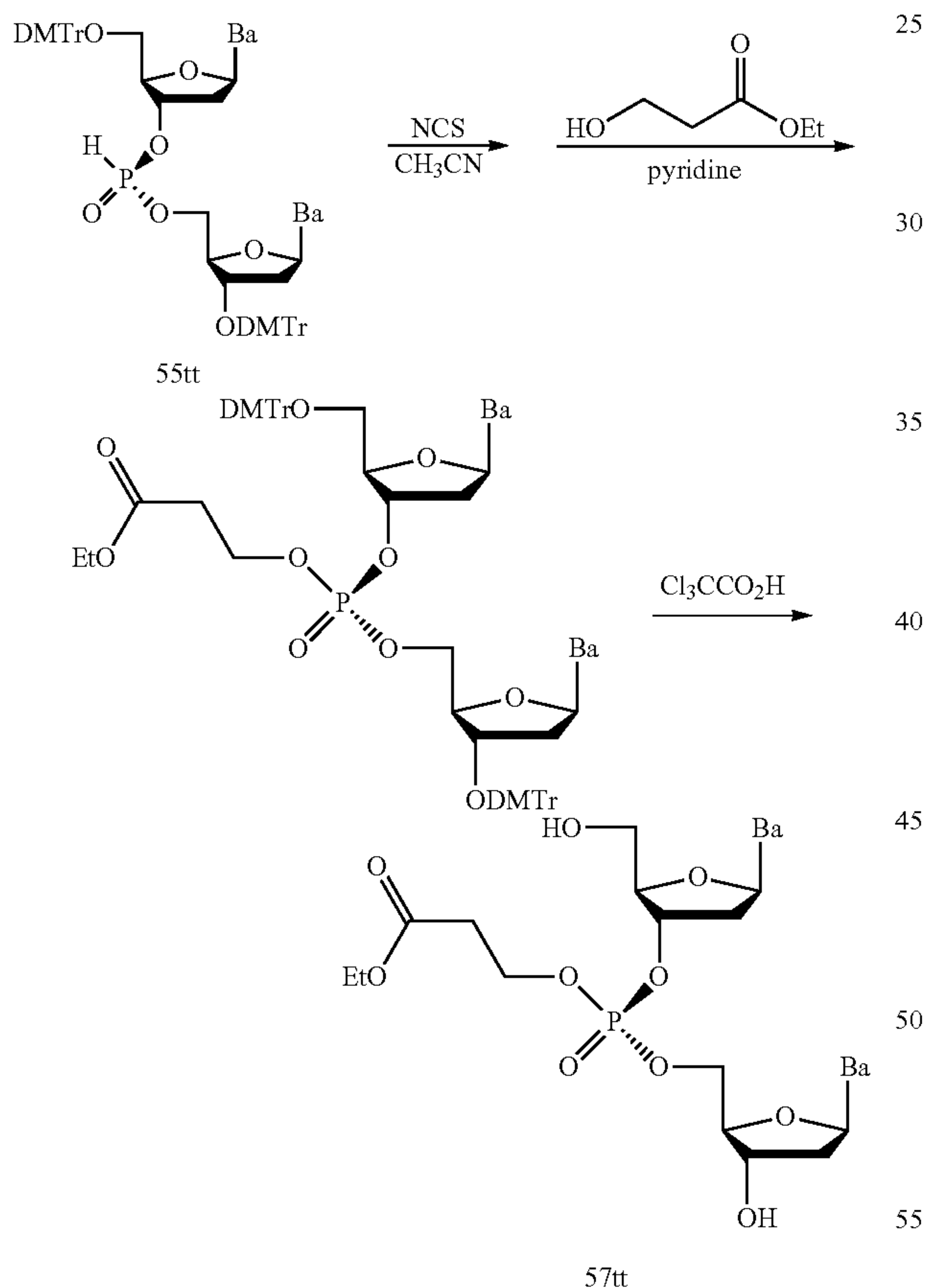
Scheme Y: Synthesis of 2-carboethoxyethyl nucleic acid prodrugs.
