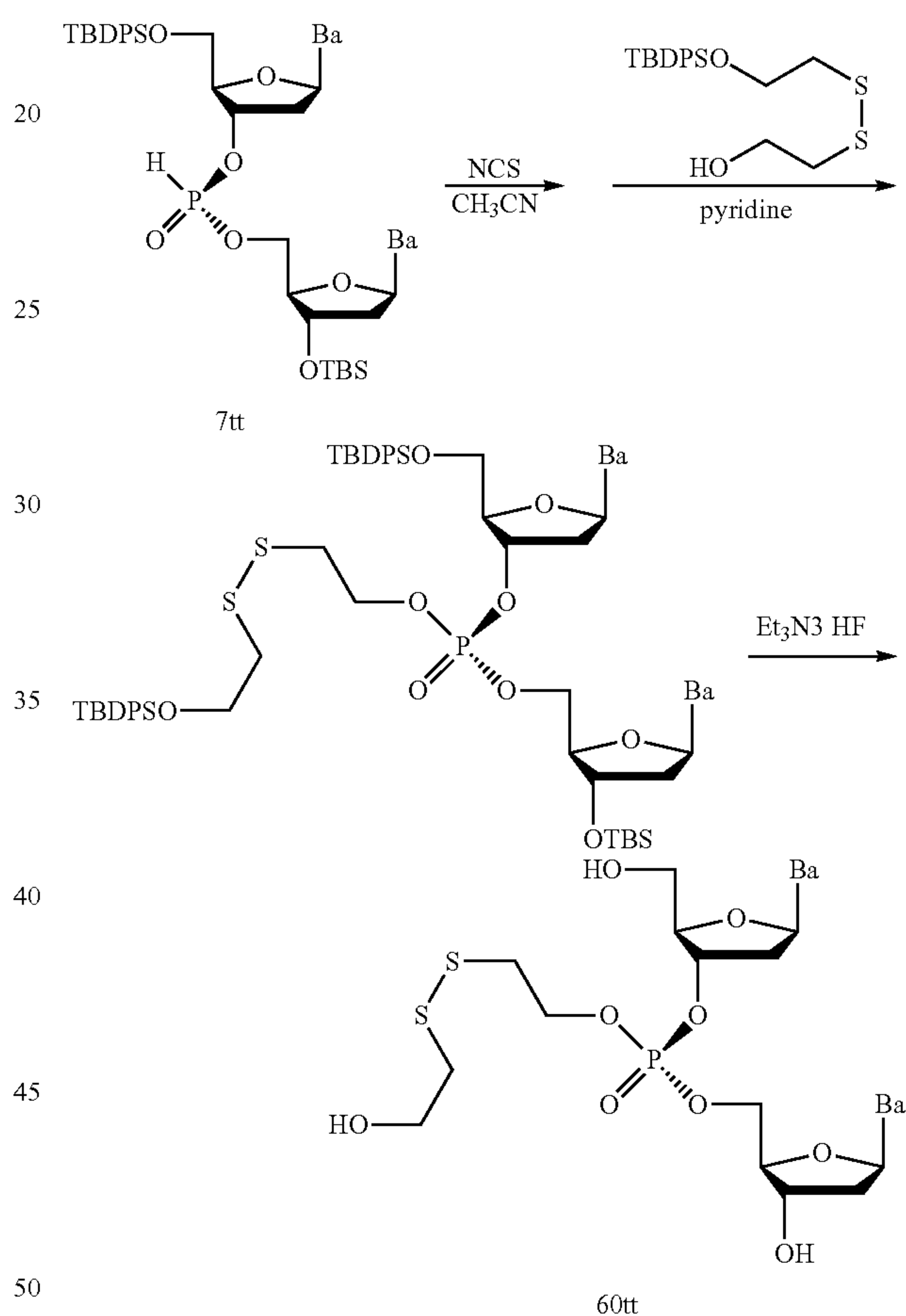
Scheme BB: Synthesis of 2-((2-hydroxyethyl)disulfide)ethyl nucleic acid prodrugs.
