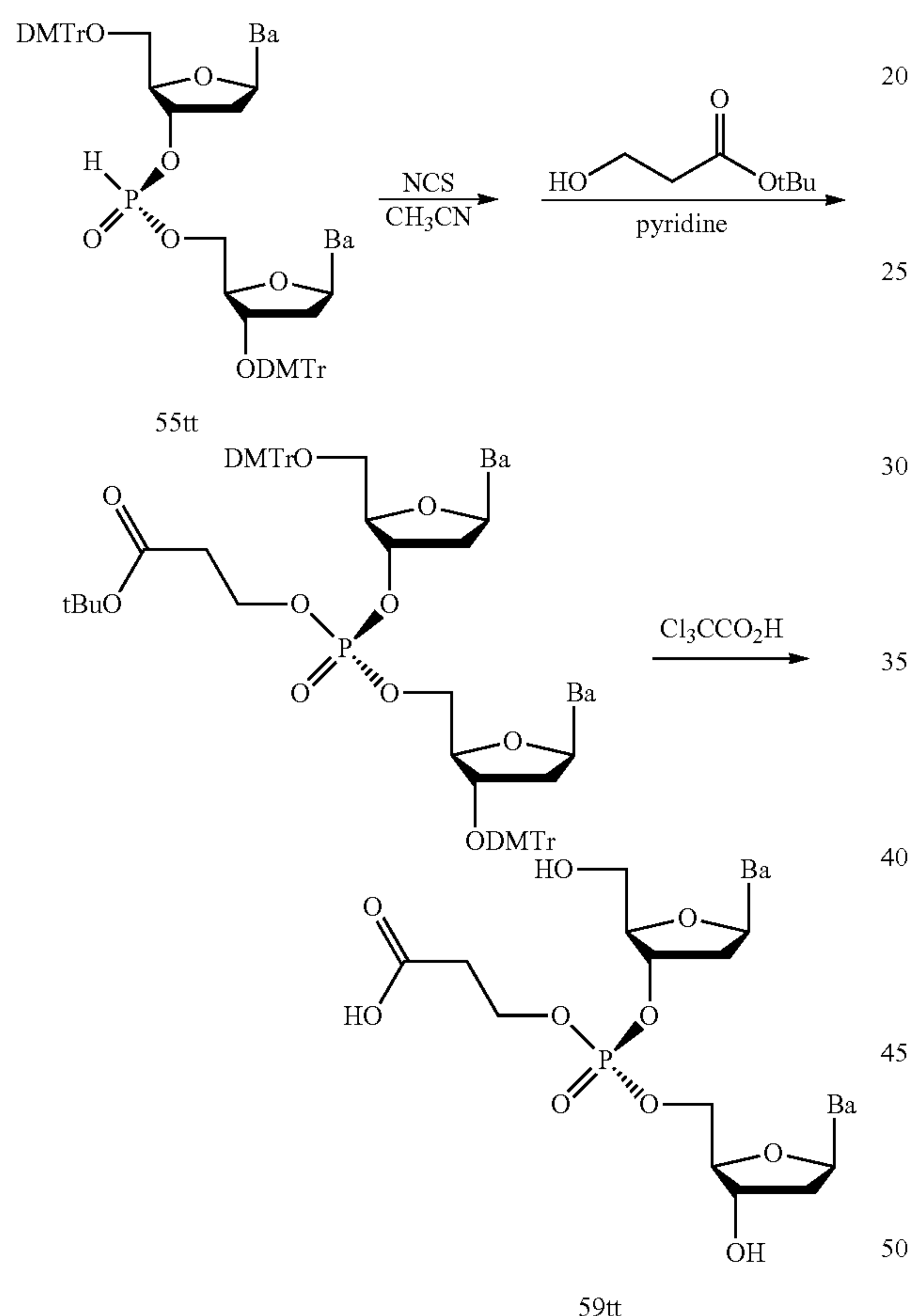
Scheme AA: Synthesis of 2-carboxyethyl nucleic acid prodrugs.
