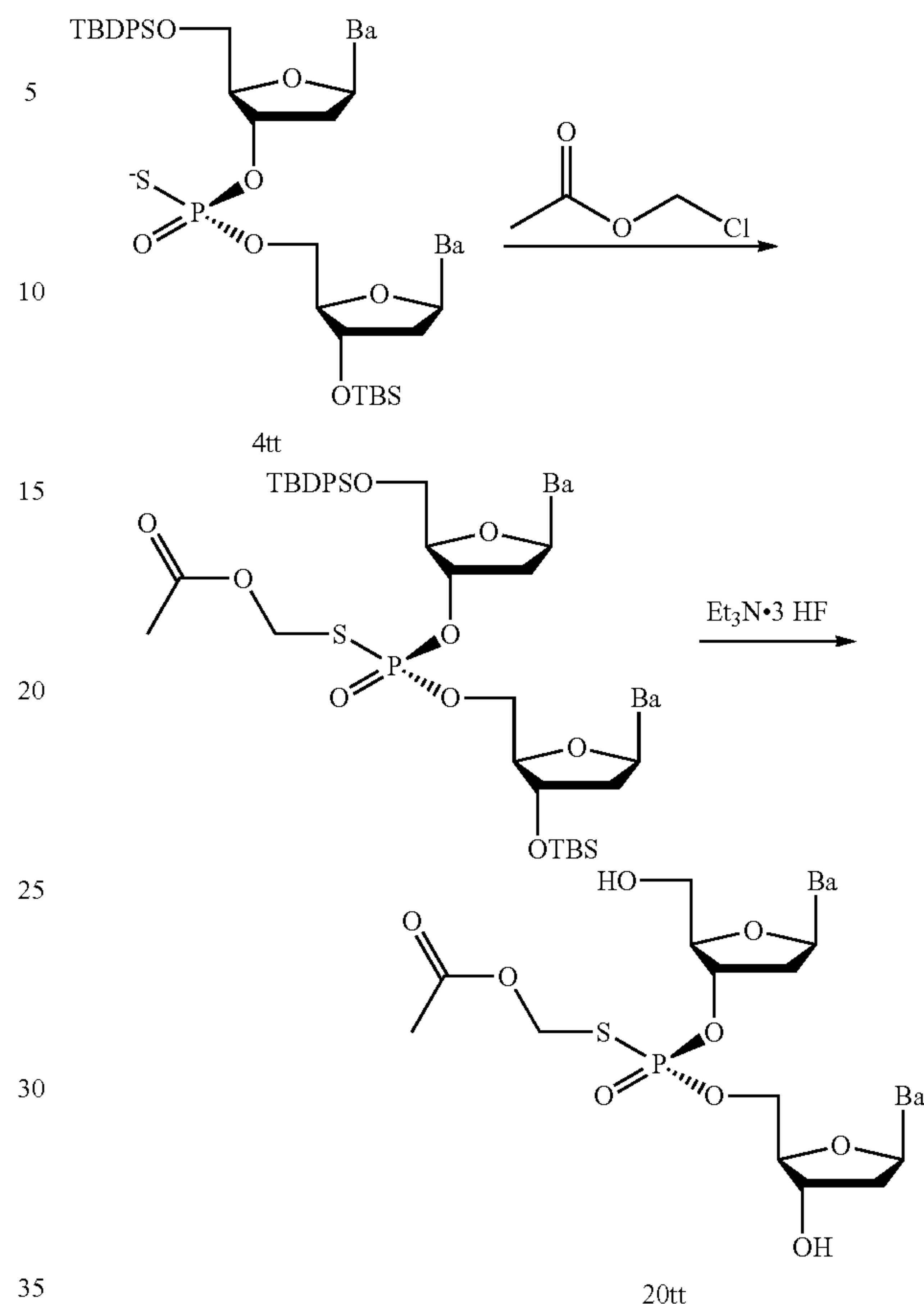
Scheme I: Synthesis of thioacyloxy pronucleotides.
