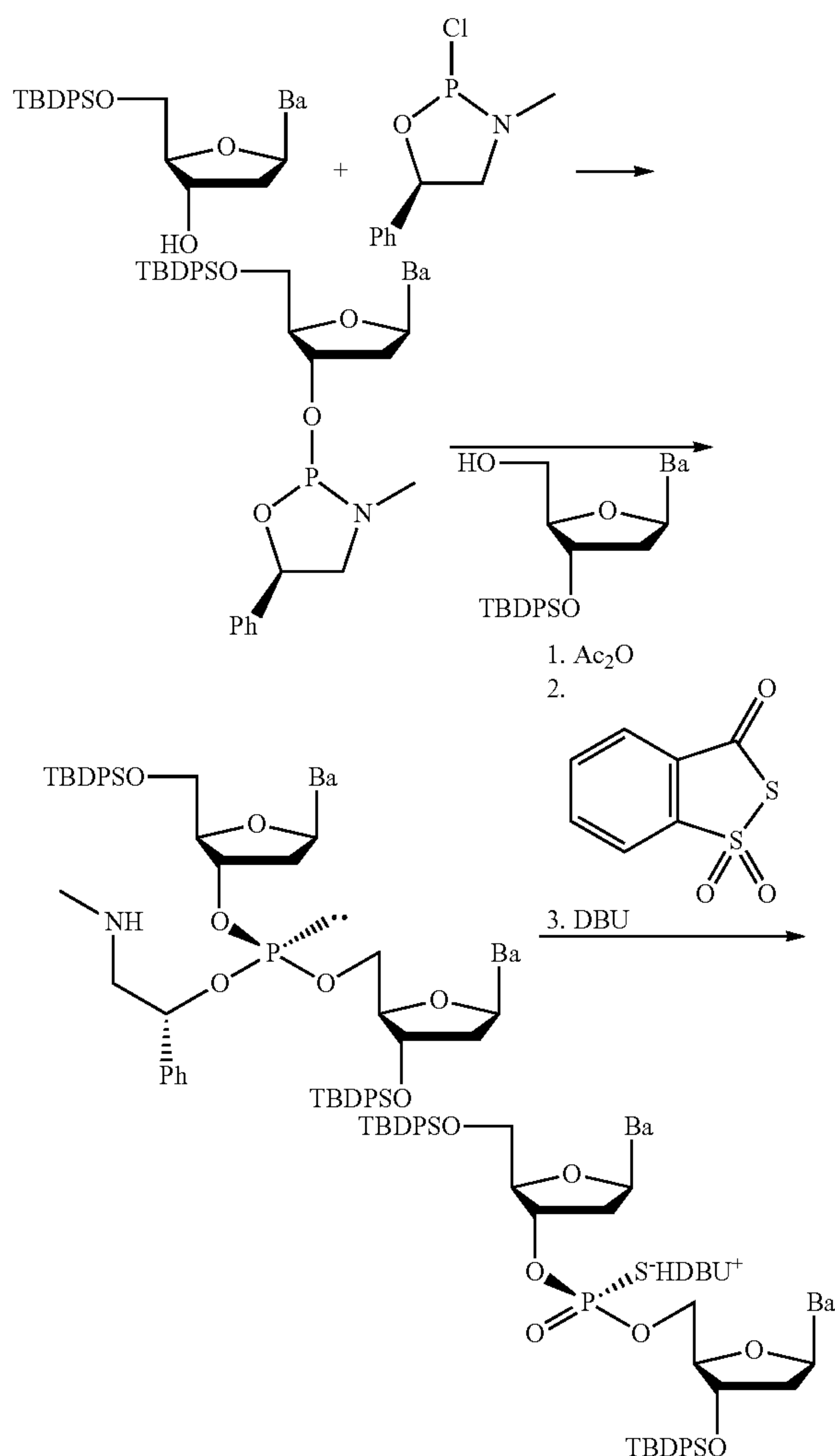
Scheme 11. Synthesis of a chiral dinucleoside phosphorothioate by stereoselective synthesis.
