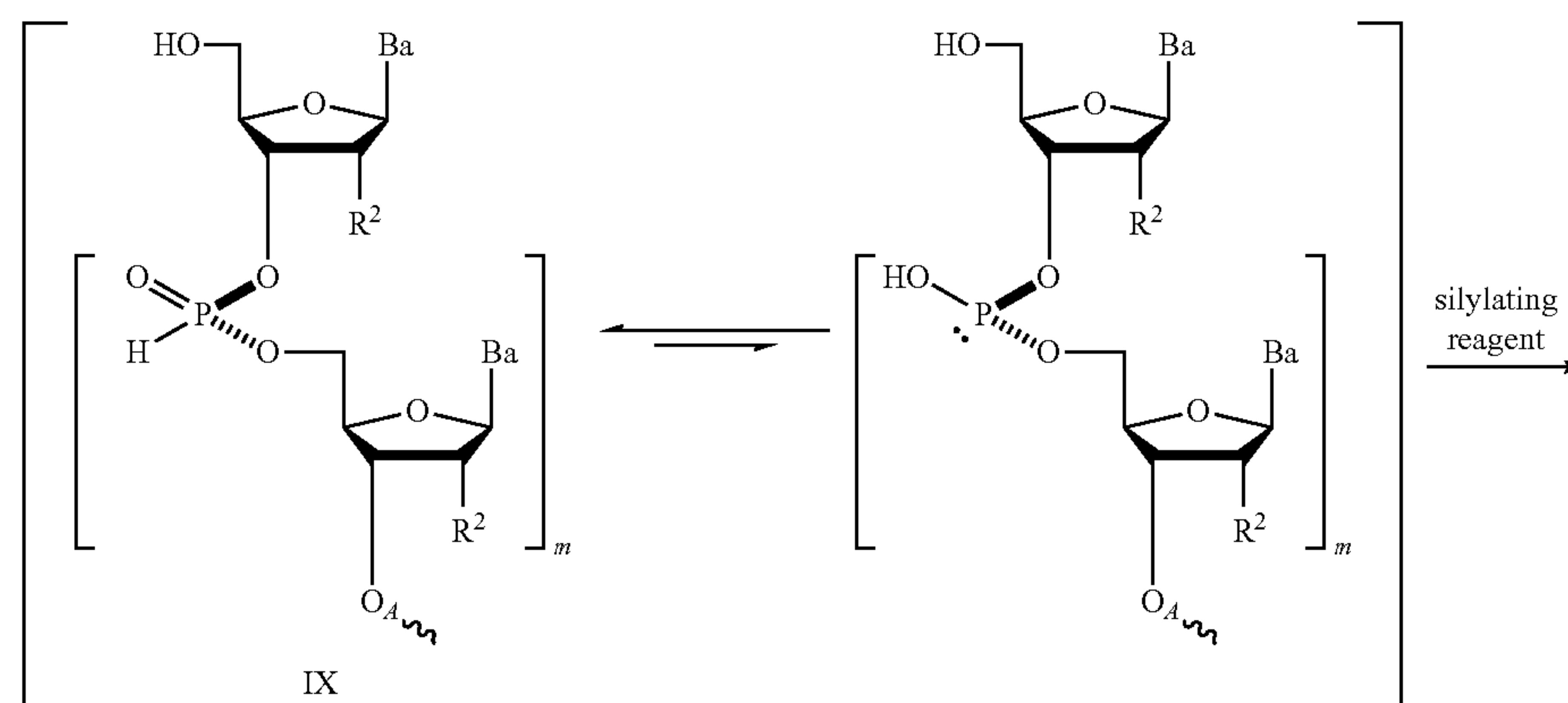
Reaction Scheme 10b.
