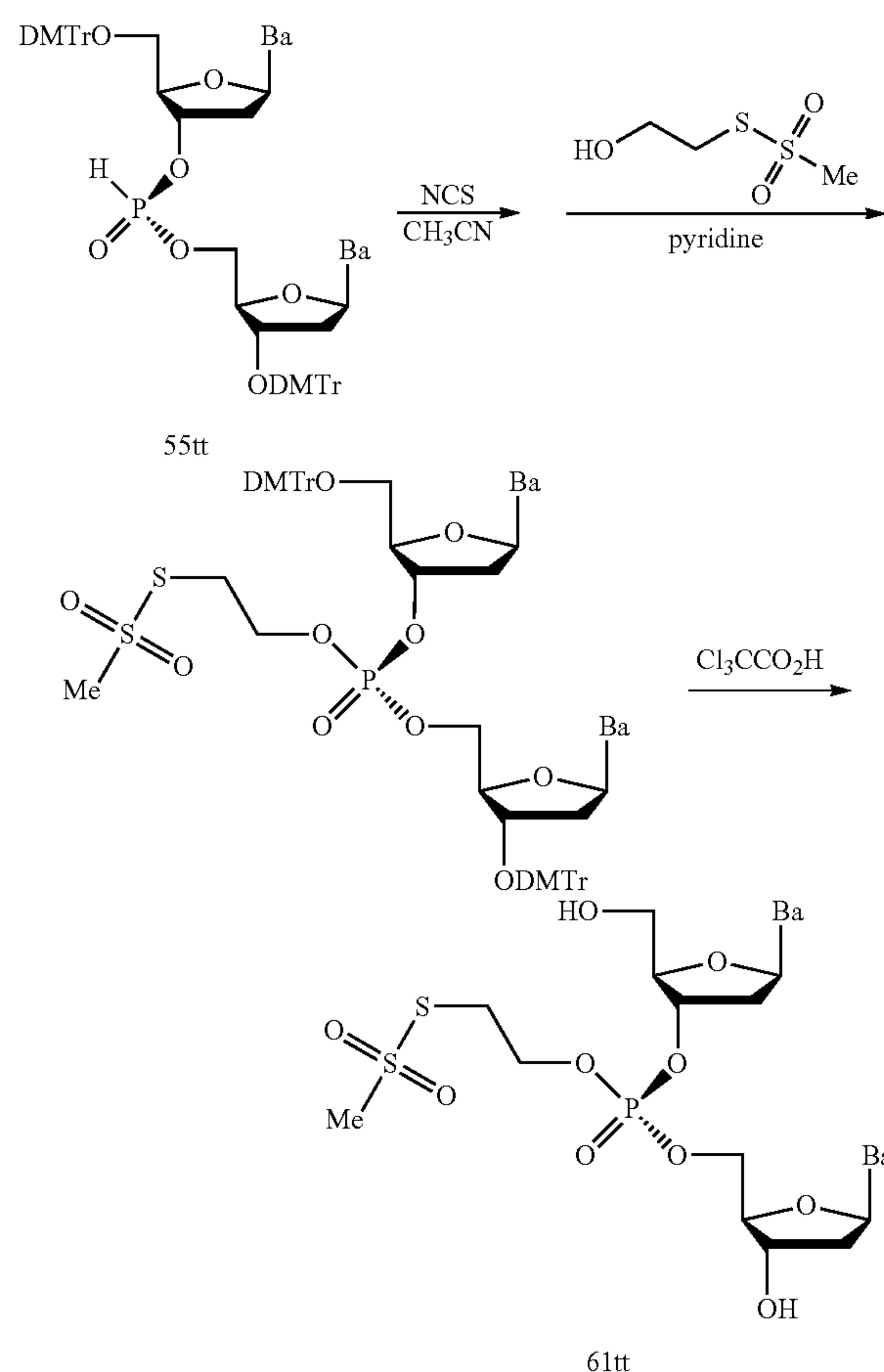
Scheme CC: Synthesis of 2-(methanesulfonylthio)ethyl nucleic acid prodrugs.
