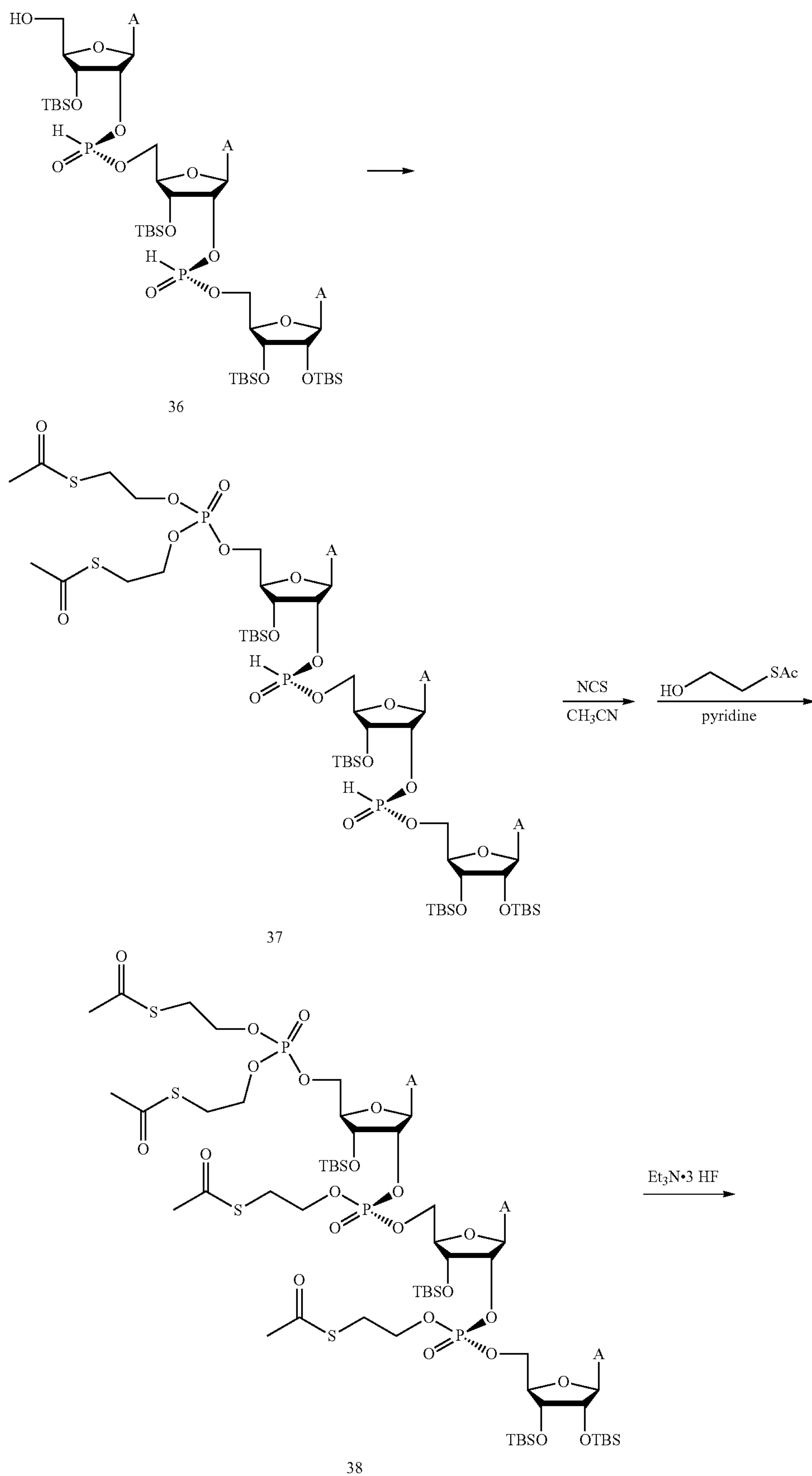
Scheme O-b: Synthesis of a 2'-5'-A 3 S-acetyl-2-thioethyl pronucleotide
