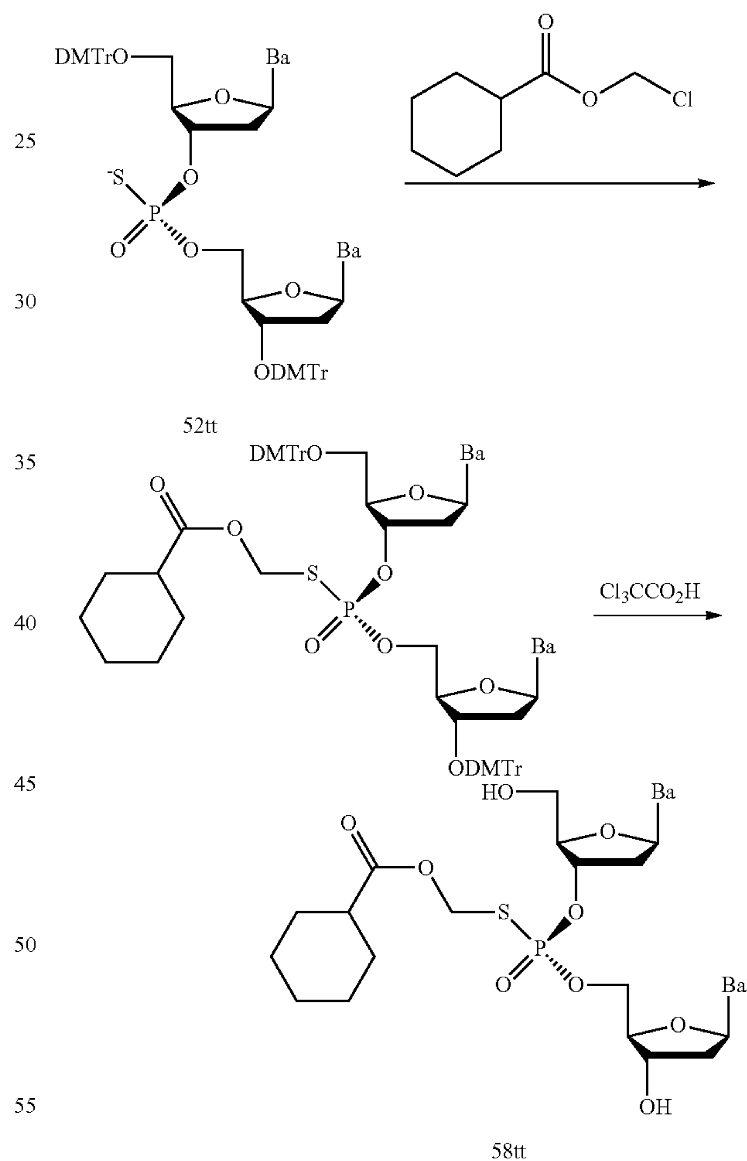
Scheme Z: Synthesis of thio(cyclohexyl)acyloxy pronucleotides
