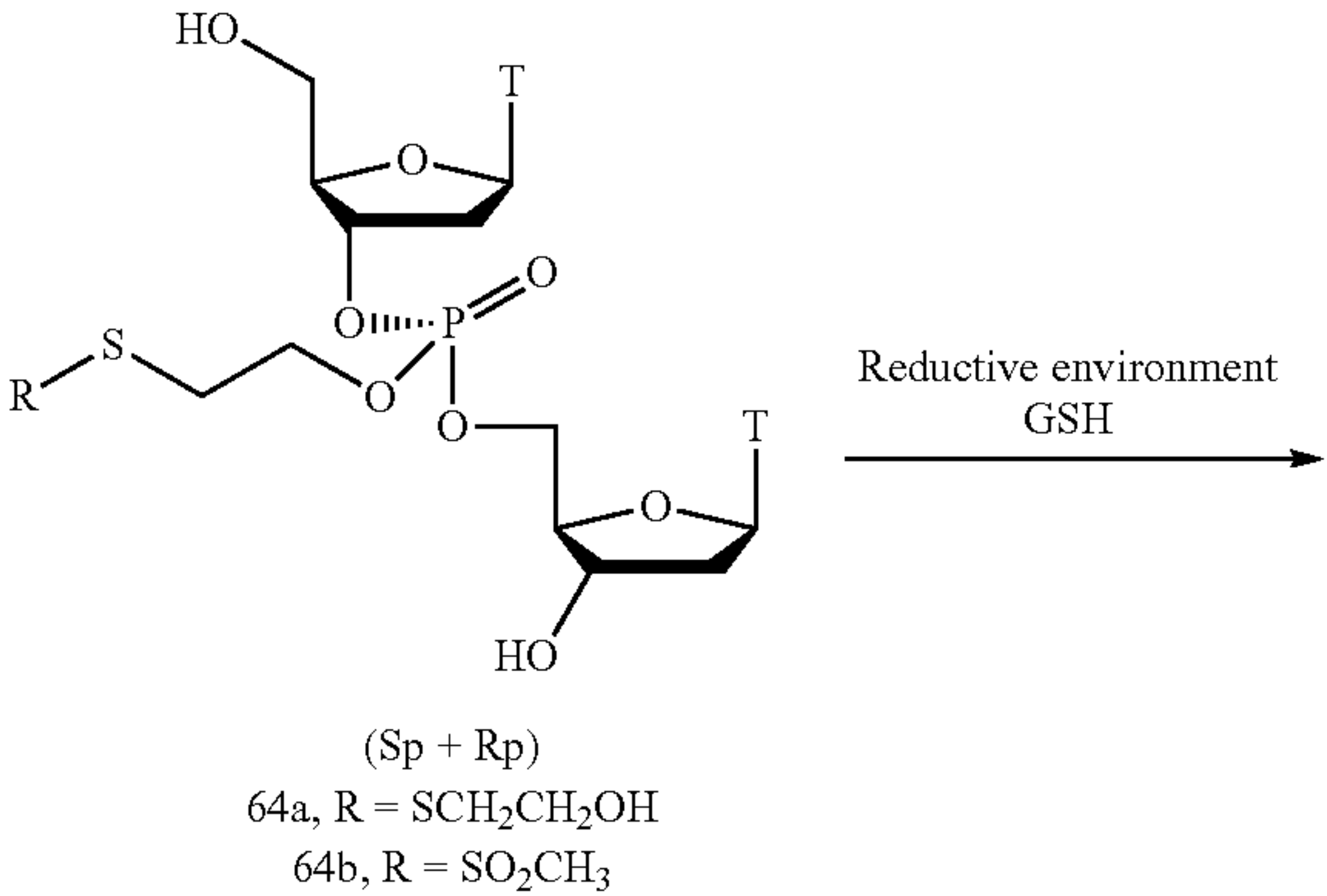
Scheme EE: Mechanism of Glutathione Cleavage
