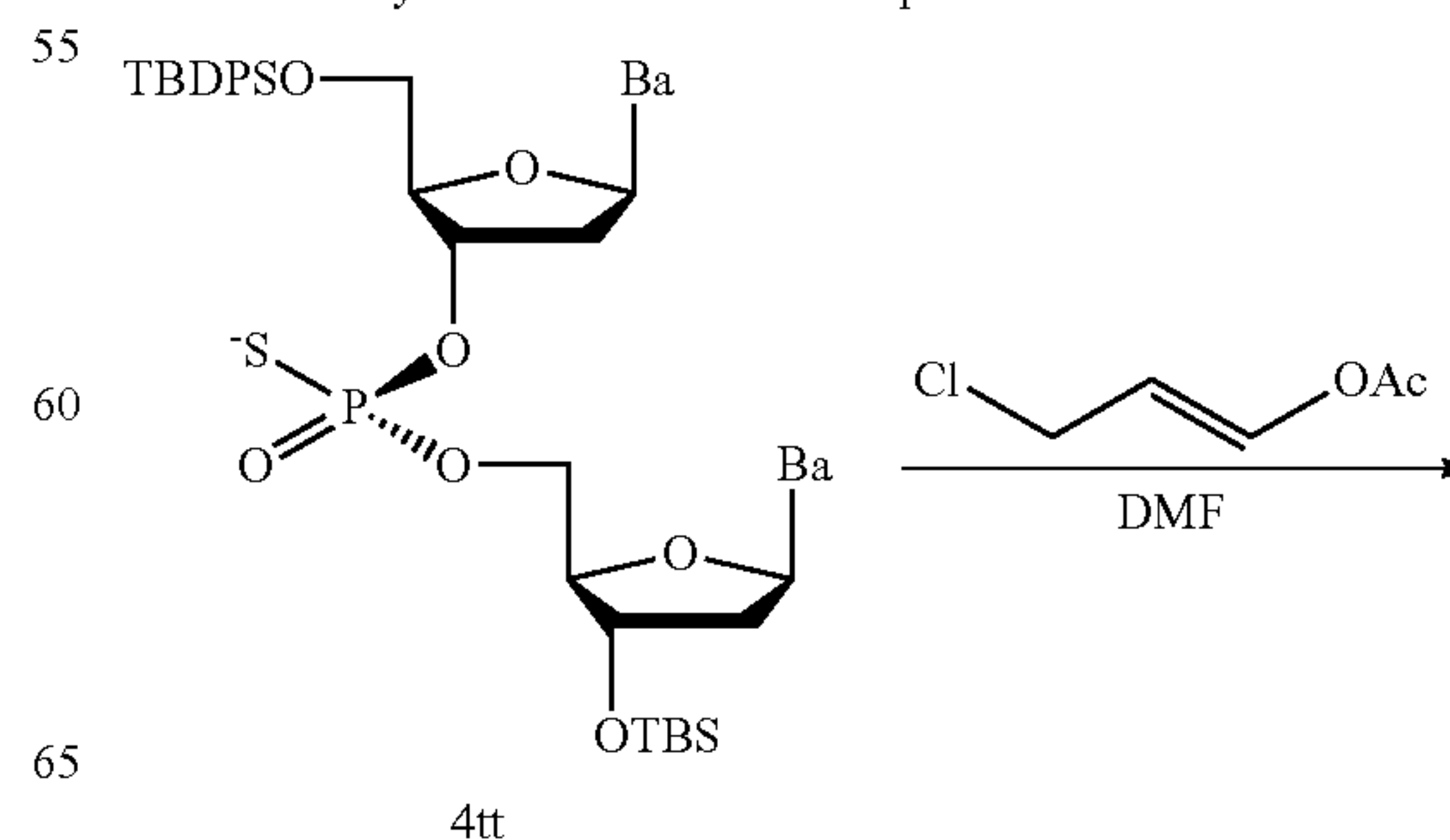
Scheme M: Synthesis of C3 enol ester pronucleotides.
