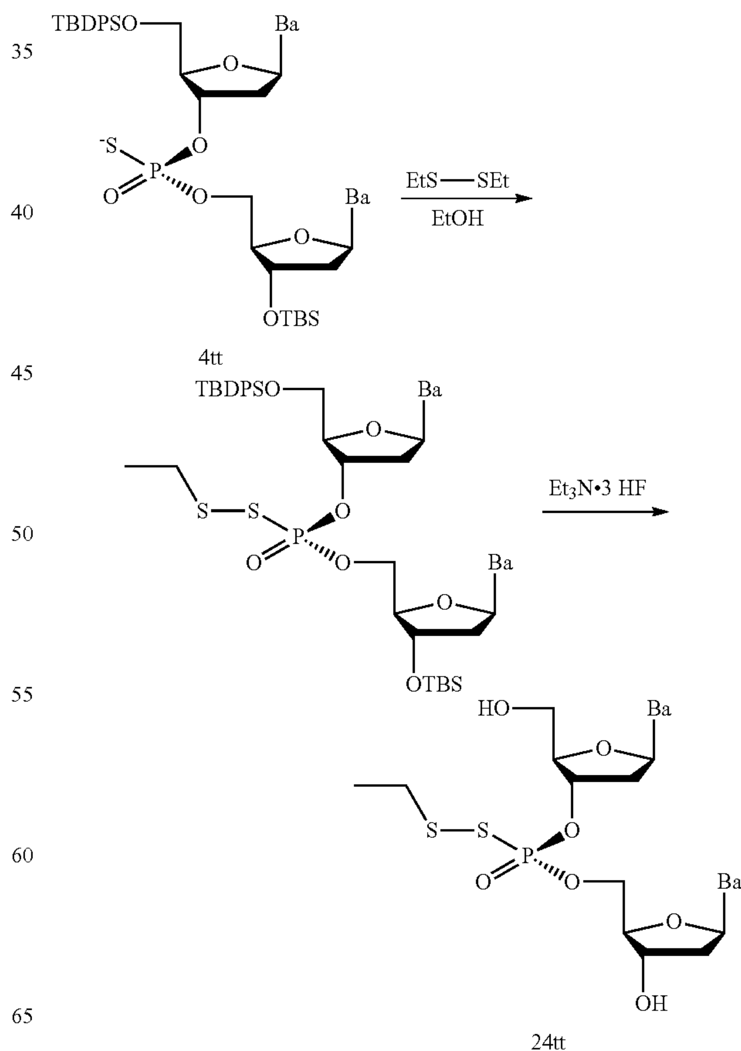
Scheme K: Synthesis of disulfide pronucleotides.
