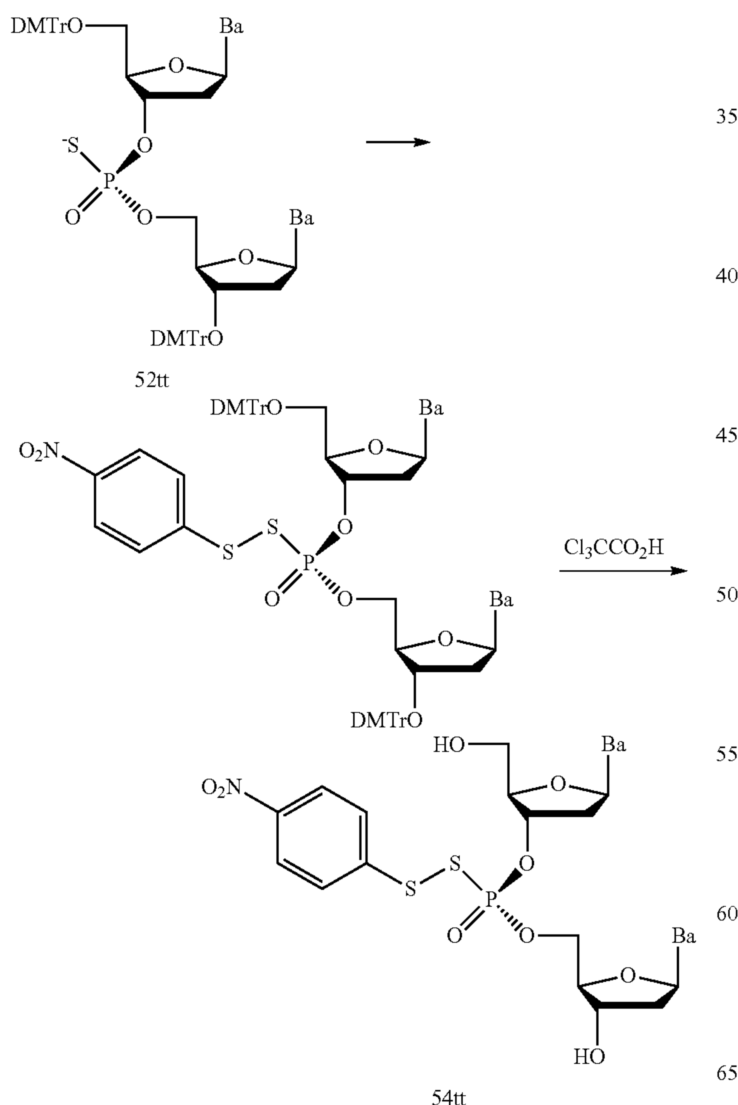
Scheme W: Synthesis of thiotrialkylammoniummethyl pronucleotides
