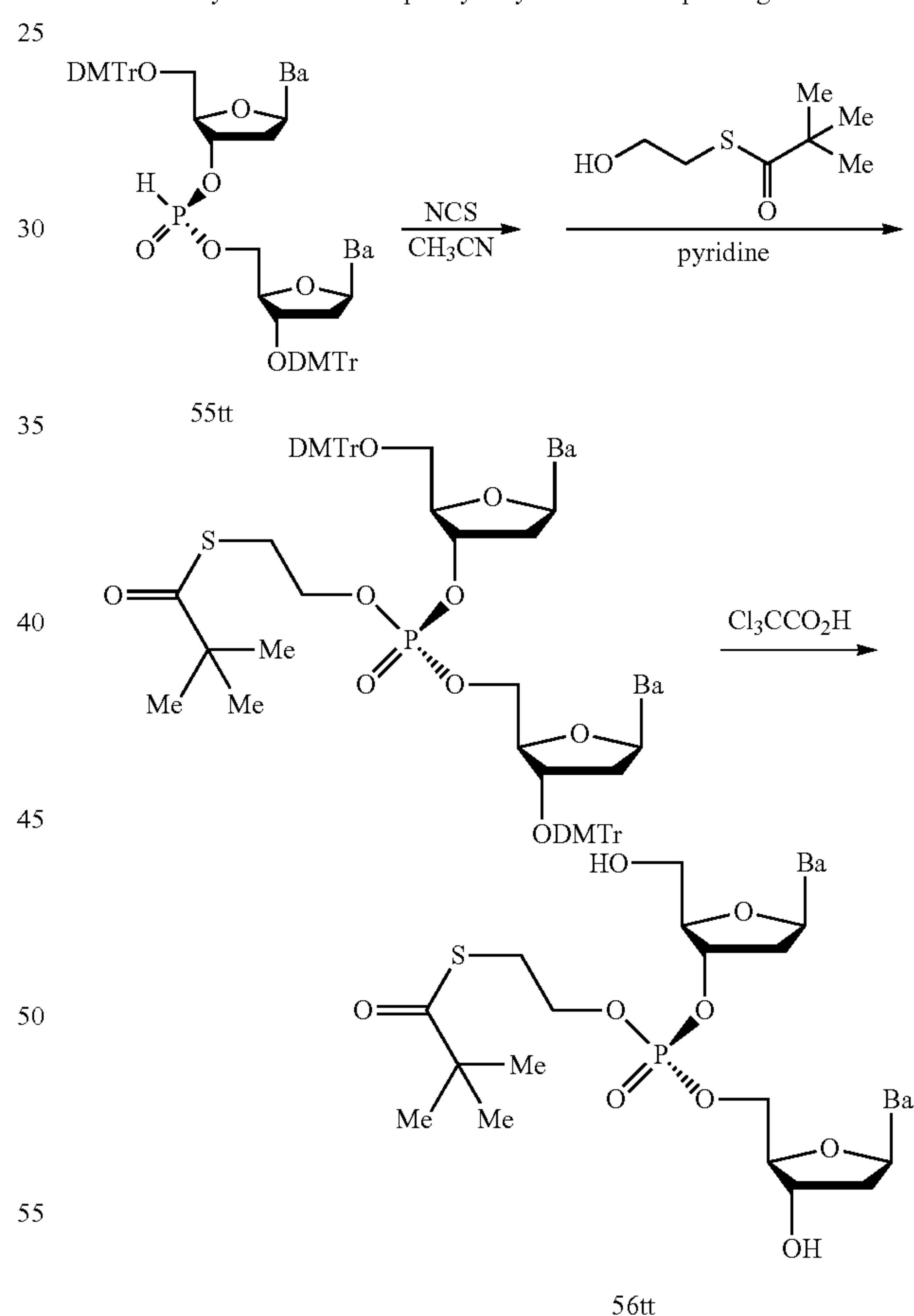
Scheme X: Synthesis of 2-thiopivalylethyl nucleic acid prodrugs.
