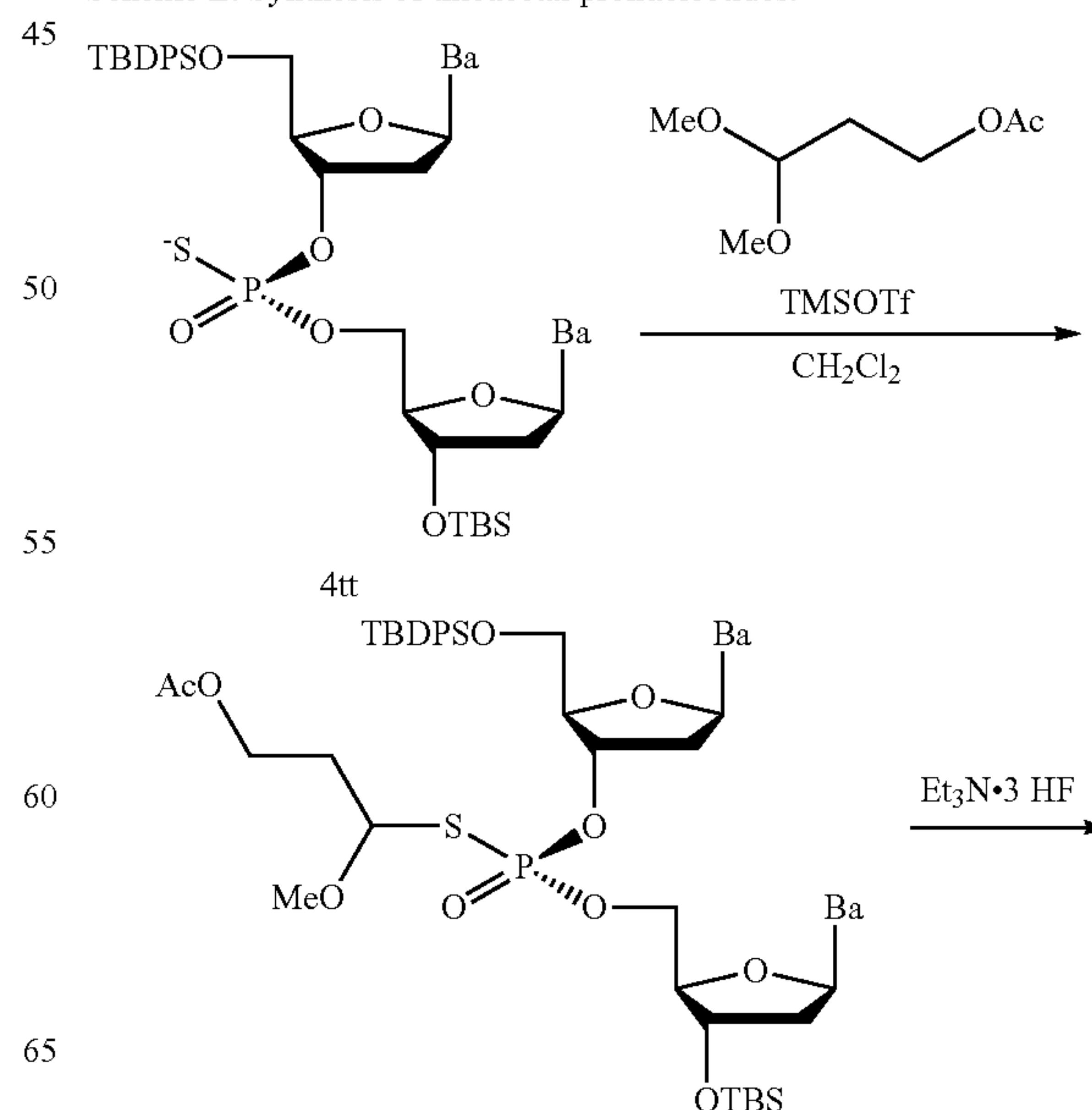
Scheme L: Synthesis of thioacetal pronucleotides.
