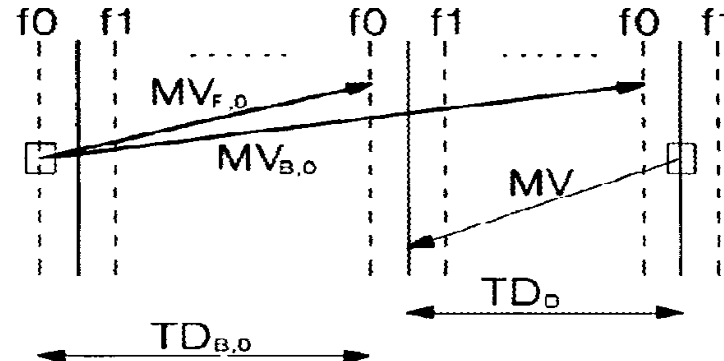
FIG. 8(C) current B List 0 reference List 1 reference
