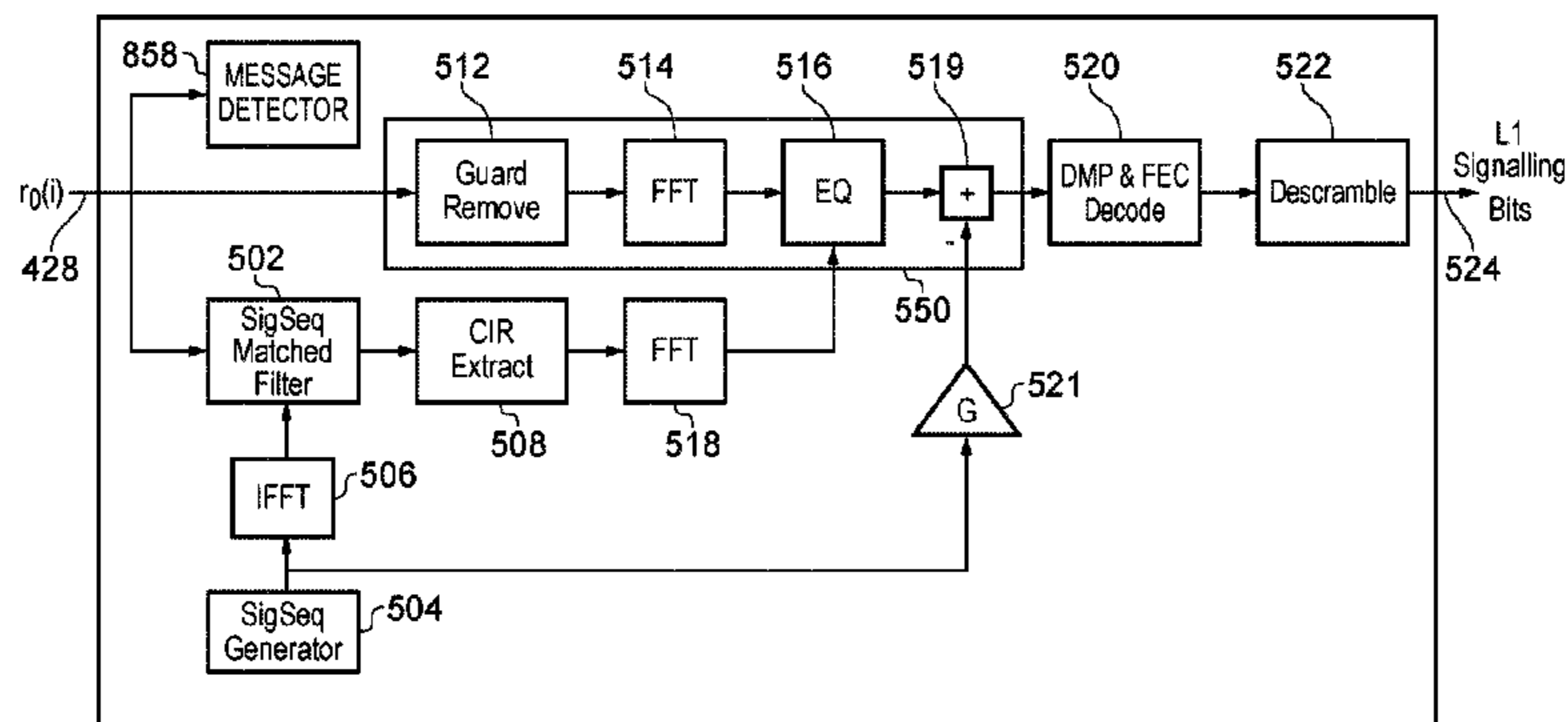
Frequency domain SigSeq removal • r_0(i) is output of frequency offset corrector
