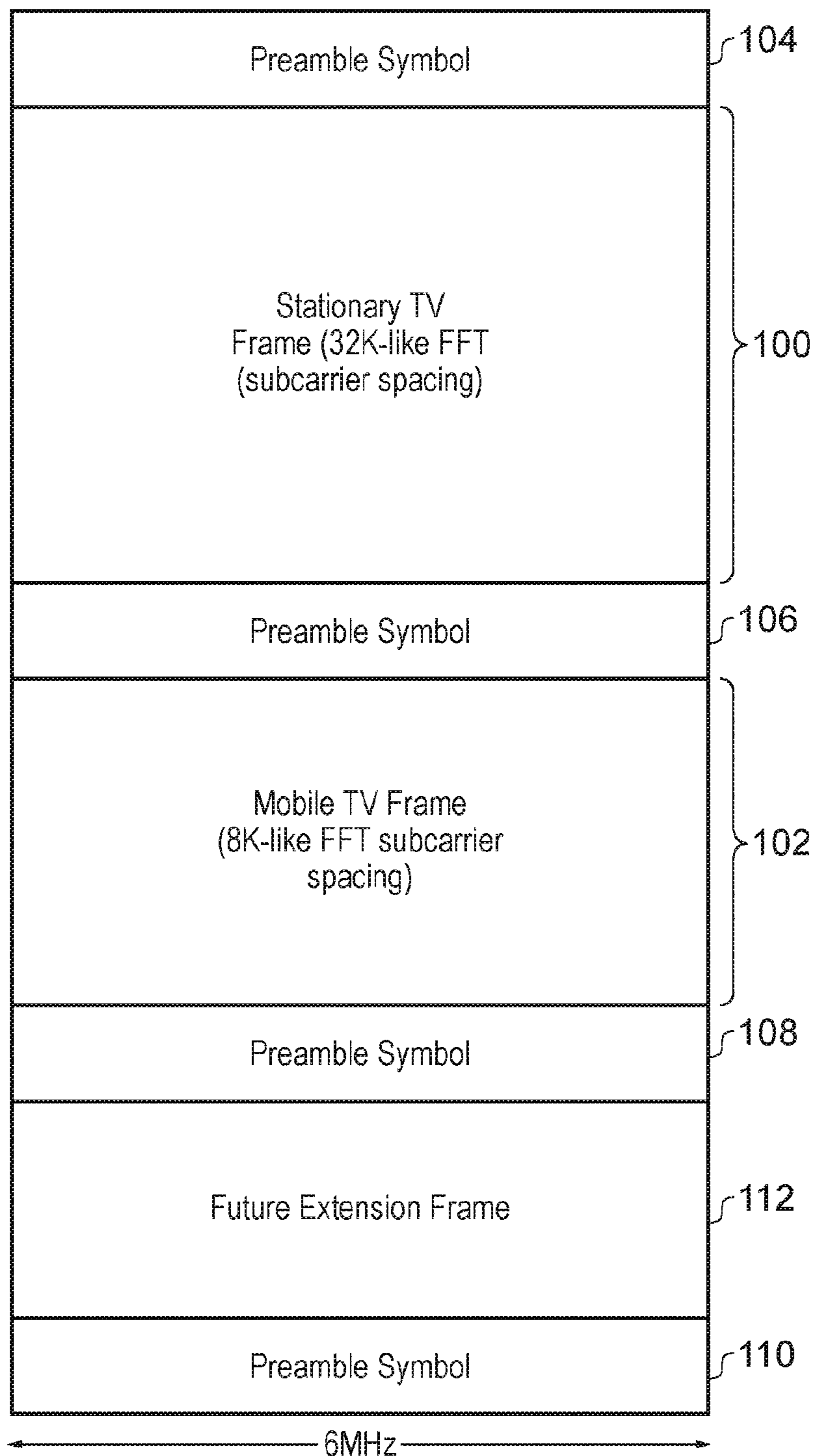
Framing concept for ATSC3-0
