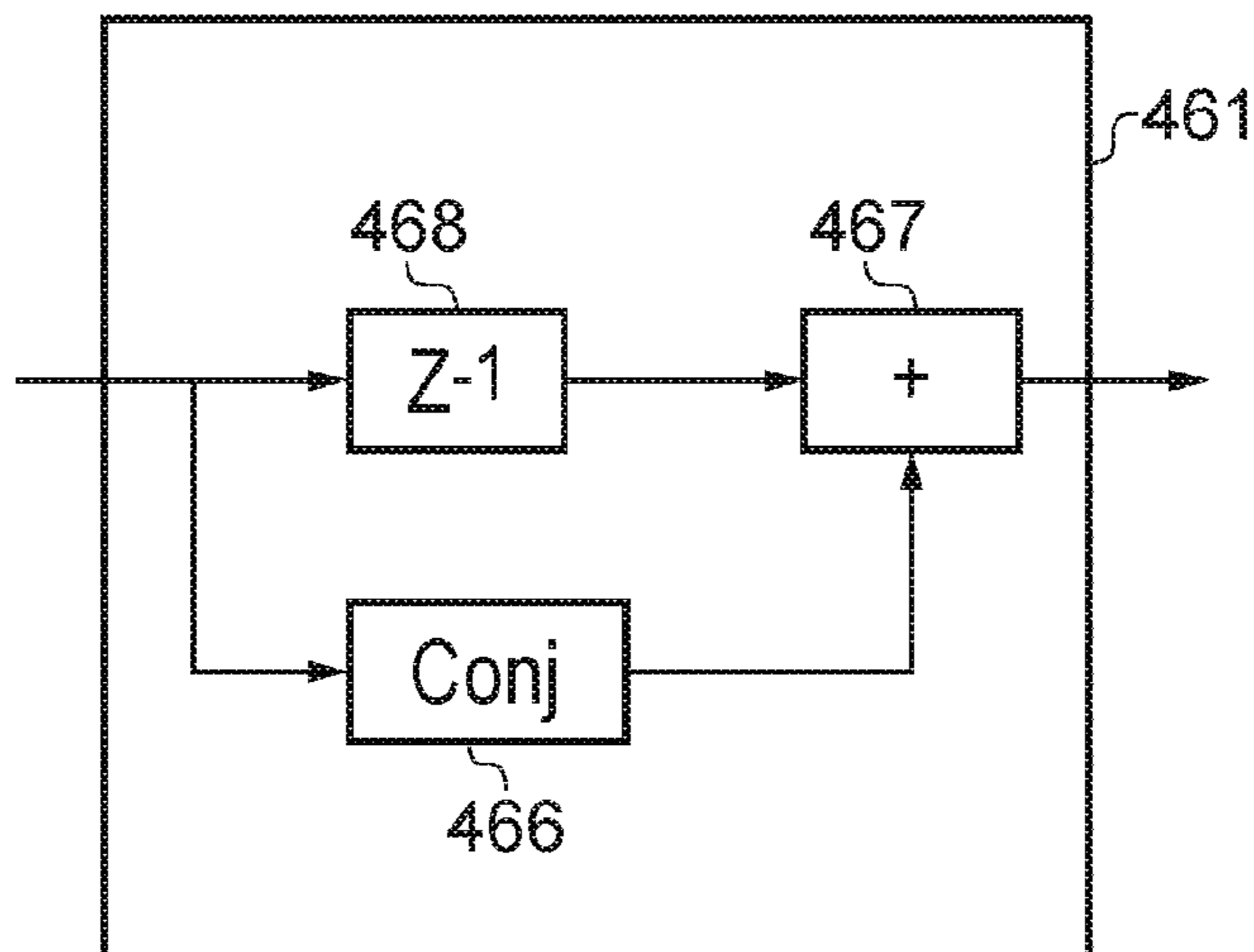
Differential Encoder
