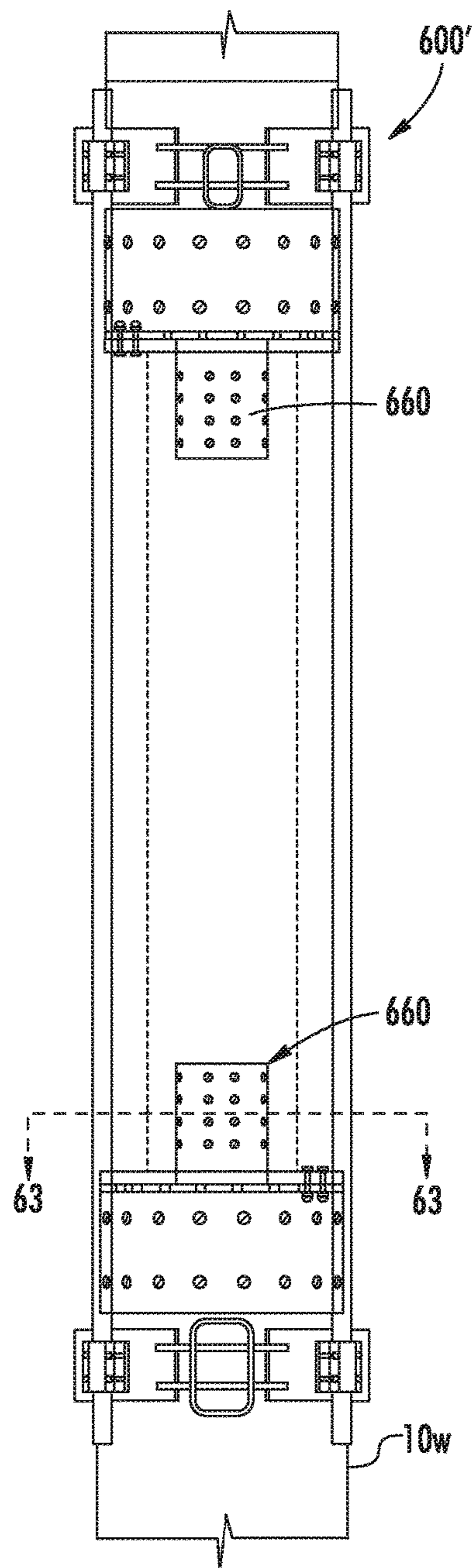
INSTALL LOWER INNER SLEEVE STEP 6
