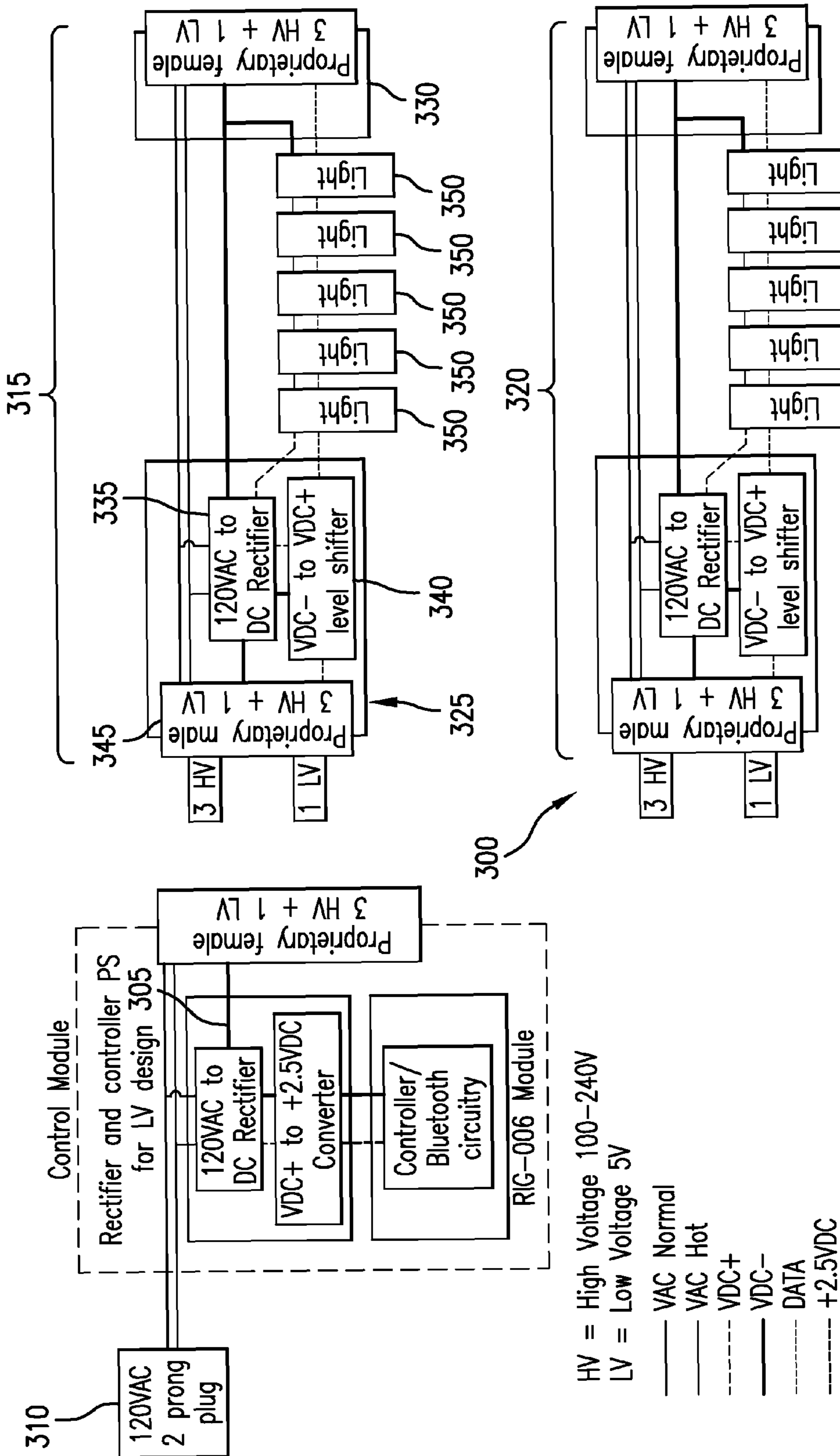
Configuration 1: 120V AC rectifier and level shifter at each string with separate control module
