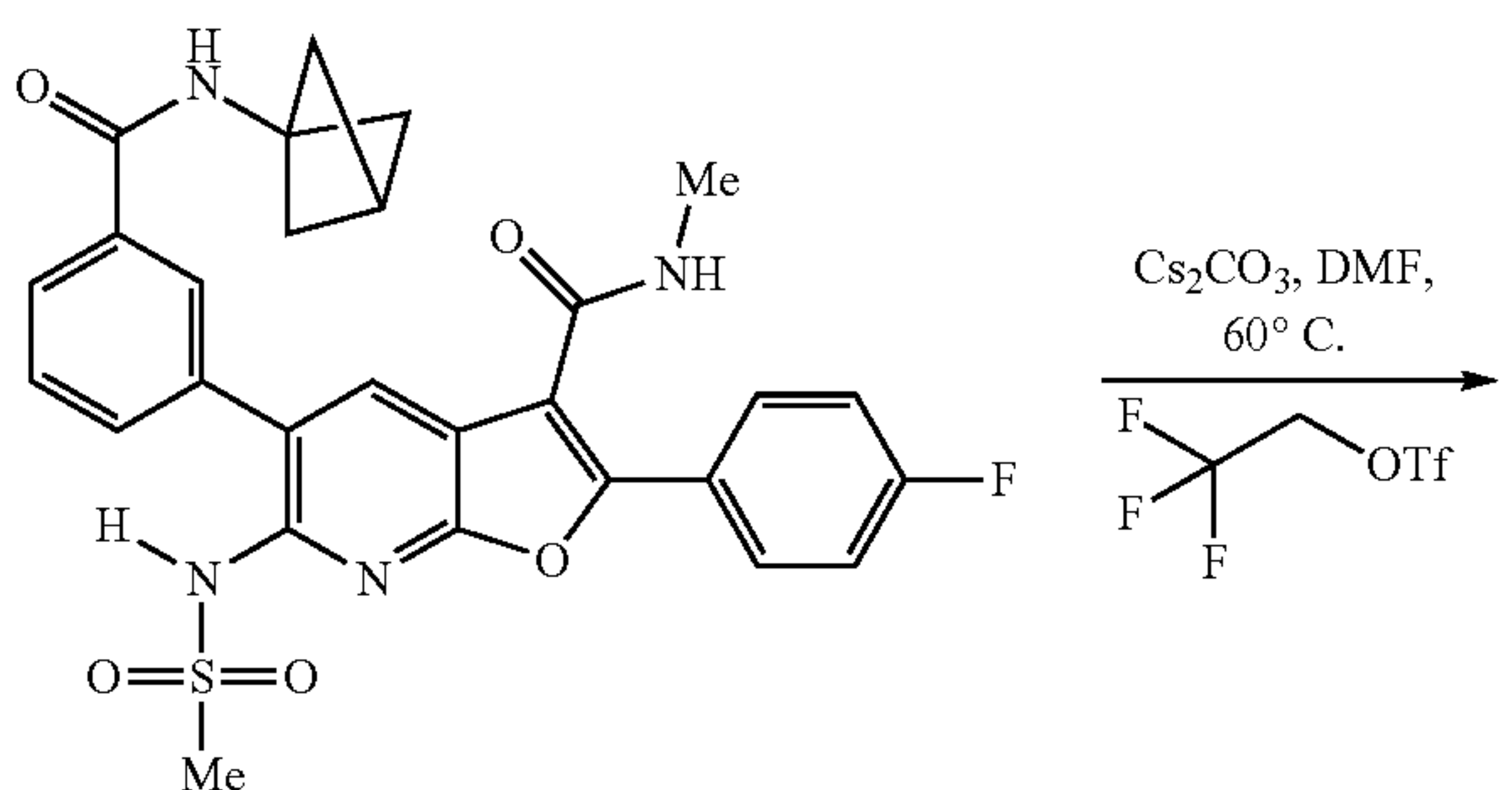
Azaindole Scheme 16
