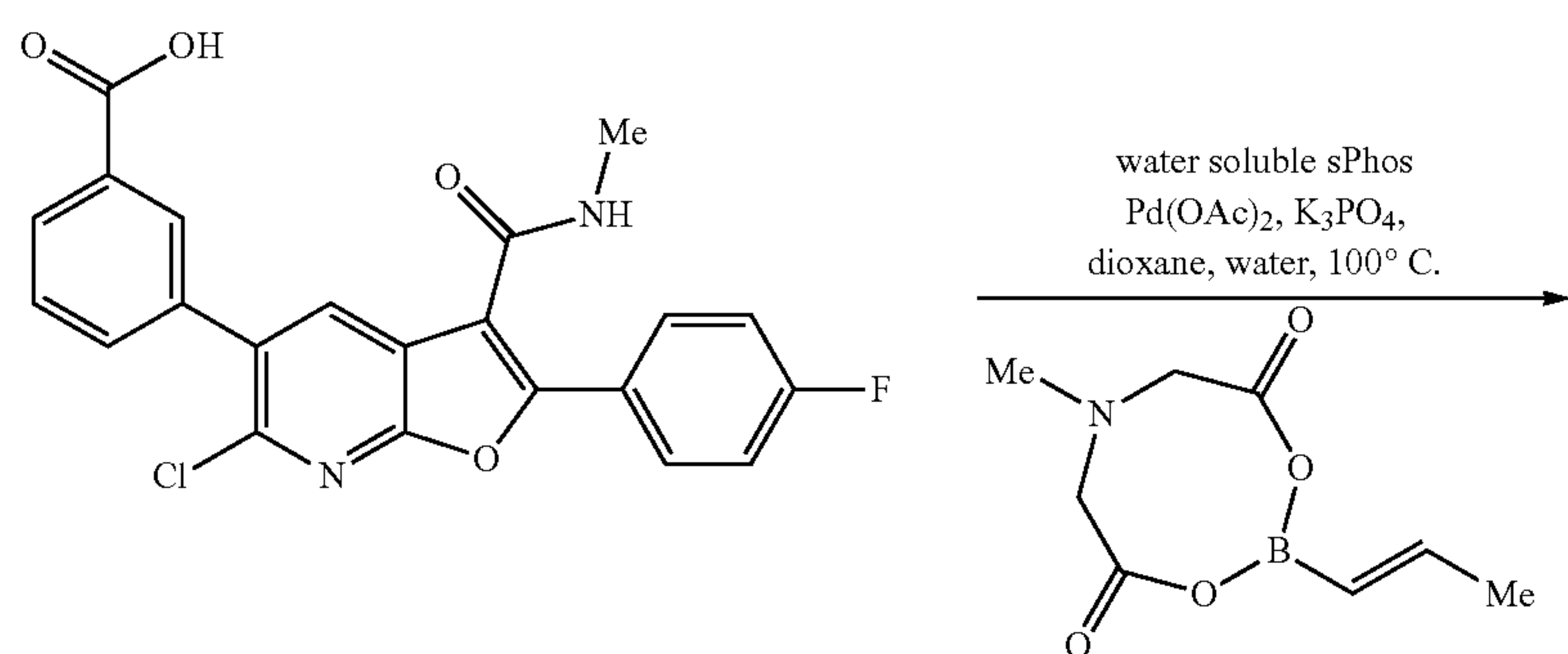
Azaindole Scheme 7
