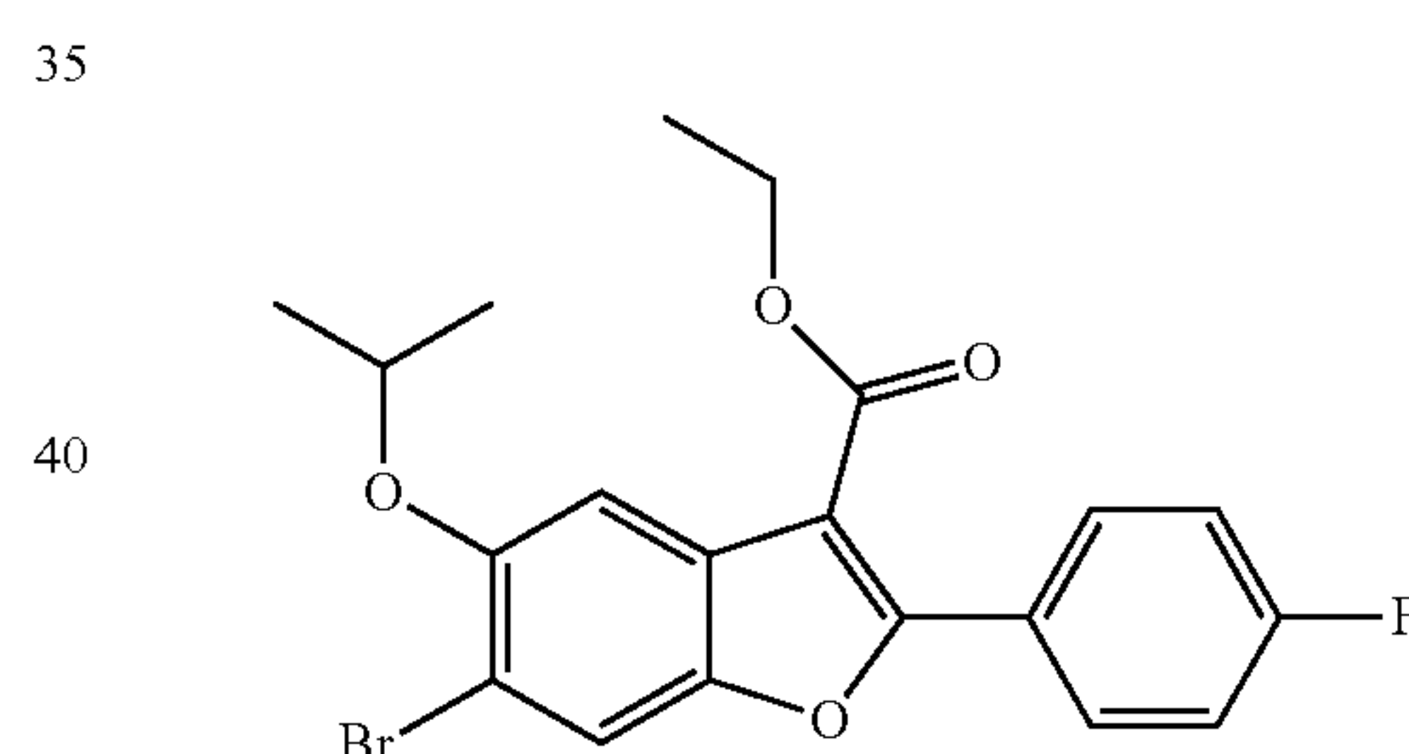
Ethyl 6-bromo-2-(4-fluorophenyl)-5-isopropoxybenzofuran-3-carboxylate
