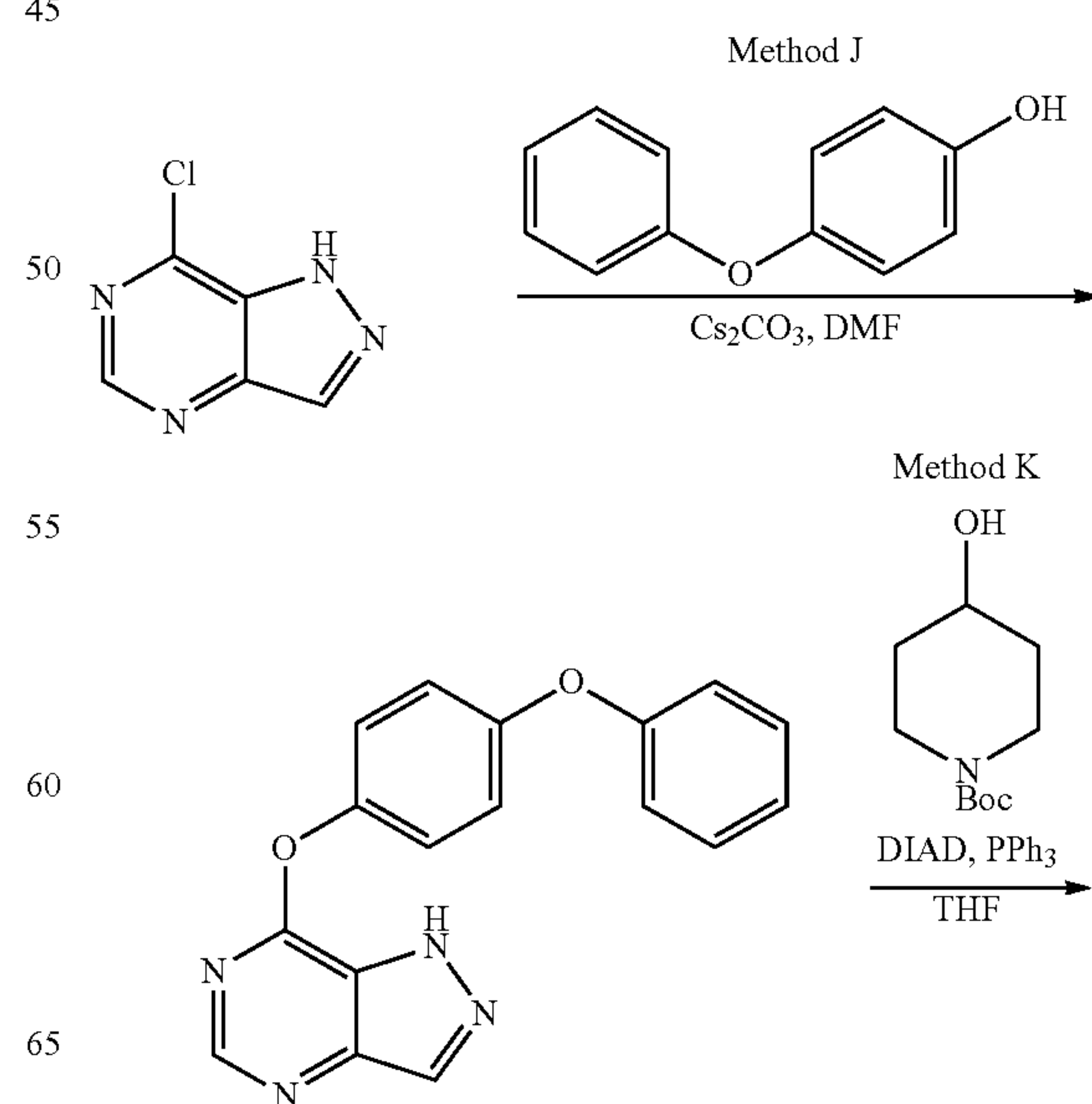
Scheme 3
