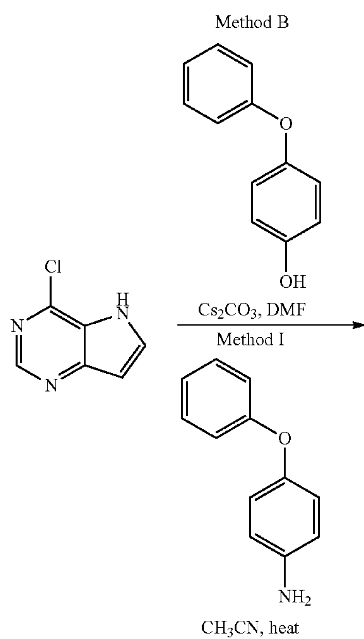
Scheme 2
