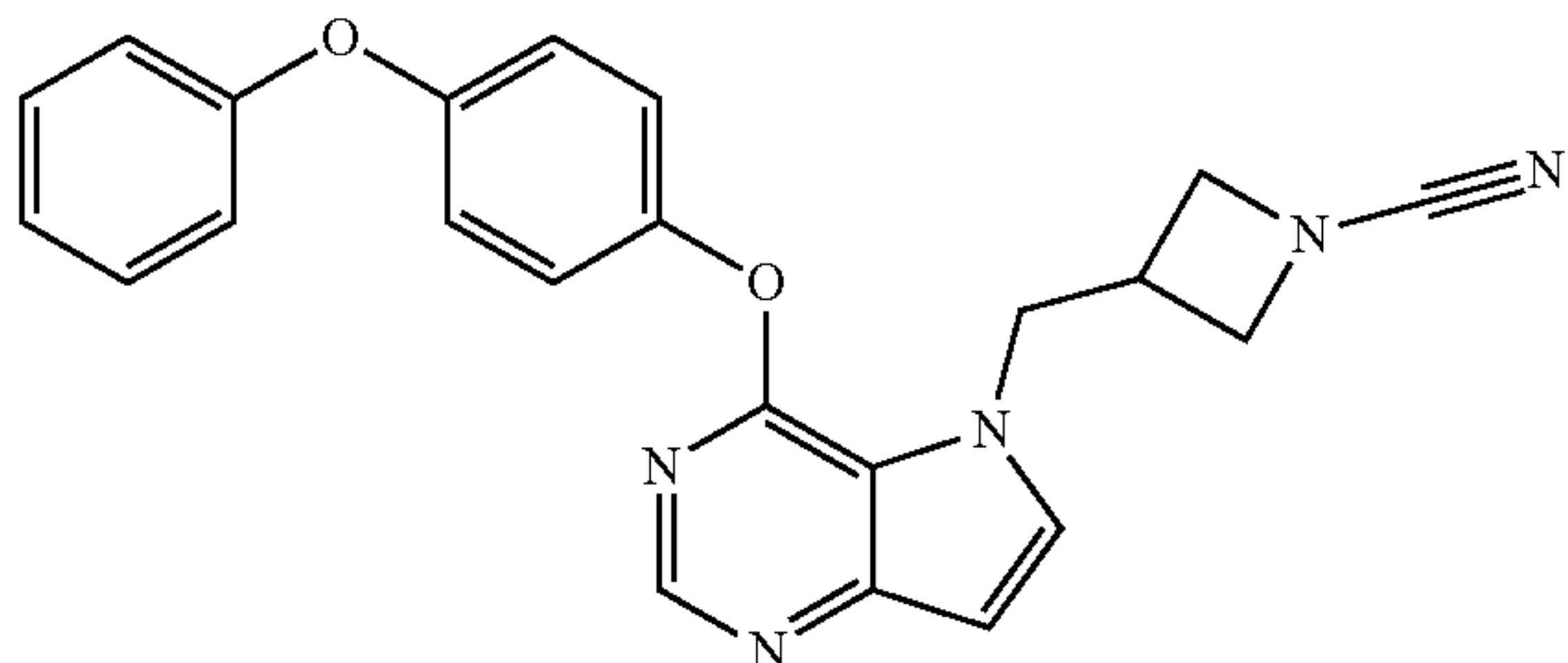
3-[[4-(4-phenoxy)oxy]-5H-pyrrolo[3,2-d]pyrimidin-5-yl]methyl]azetidine-1-carbonitrile (66)
