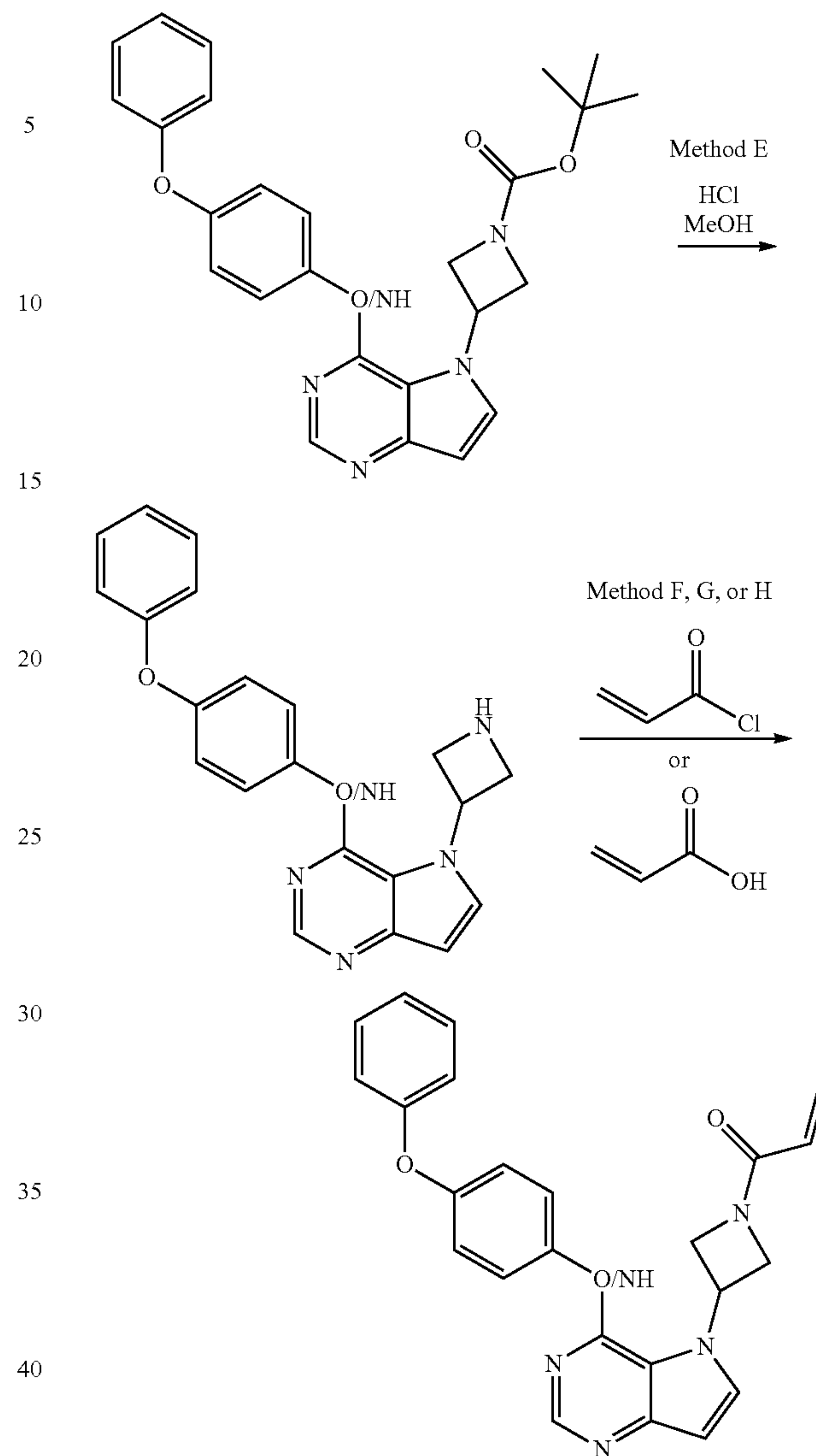
Scheme 3
