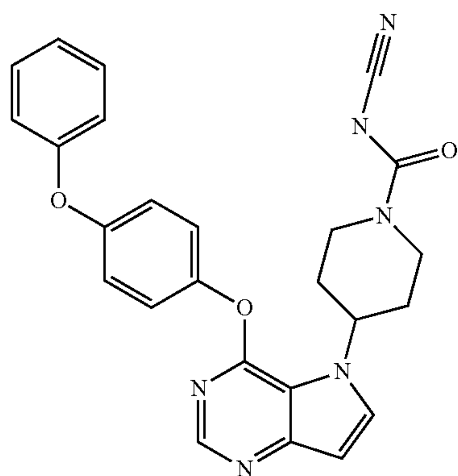
N-cyano-4-(4-(4-phenoxyphenoxy)-5H-pyrrolo[3,2-d]pyrimidin-5-yl)piperidine-1-carboxamide (57)
