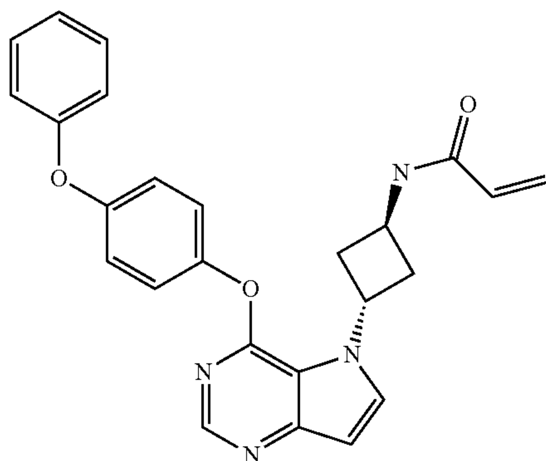
N-(trans-3-(4-(4-phenoxyphenoxy)-5H-pyrrolo[3,2-d]pyrimidin-5-yl)cyclobutyl)acrylamide (8)
