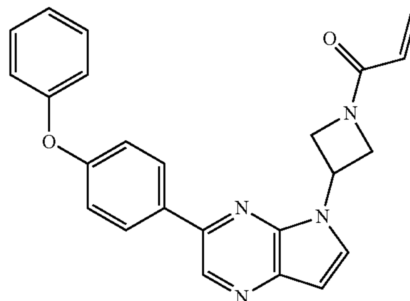
1-(3-(3-(4-phenoxyphenyl)-5H-pyrrolo[2,3-b]pyrazin-5-yl)azetidin-1-yl)prop-2-en-1-one (7)
