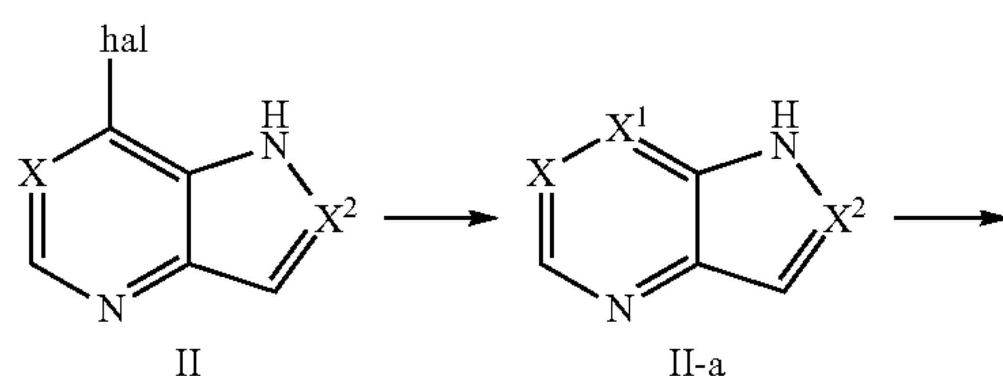
Scheme A
