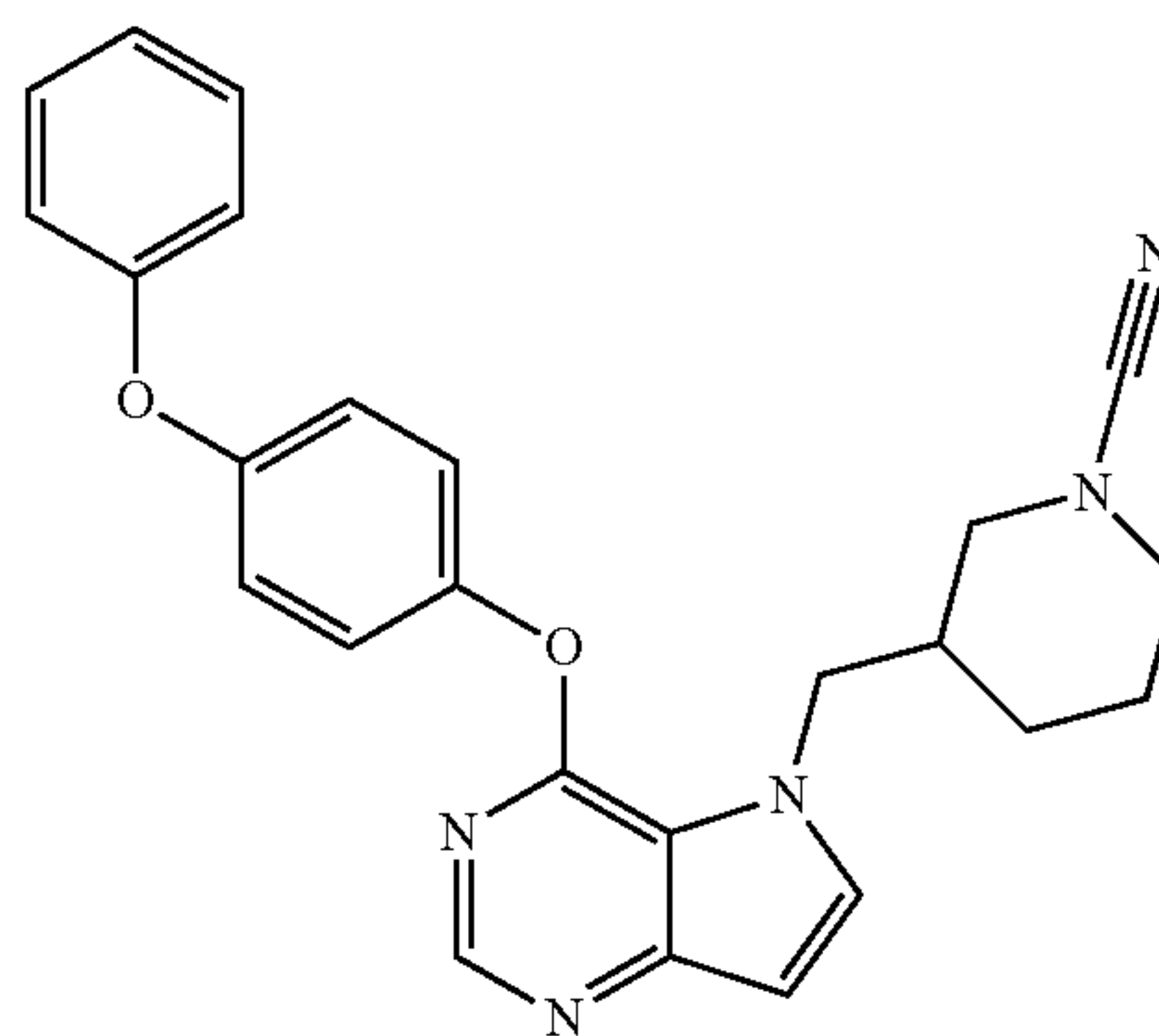
3-[[4-(4-phenoxyphenoxy)-5H-pyrrolo[3,2-d]pyrimidin-5-yl]methyl]piperidine-1-carbonitrile (63)
