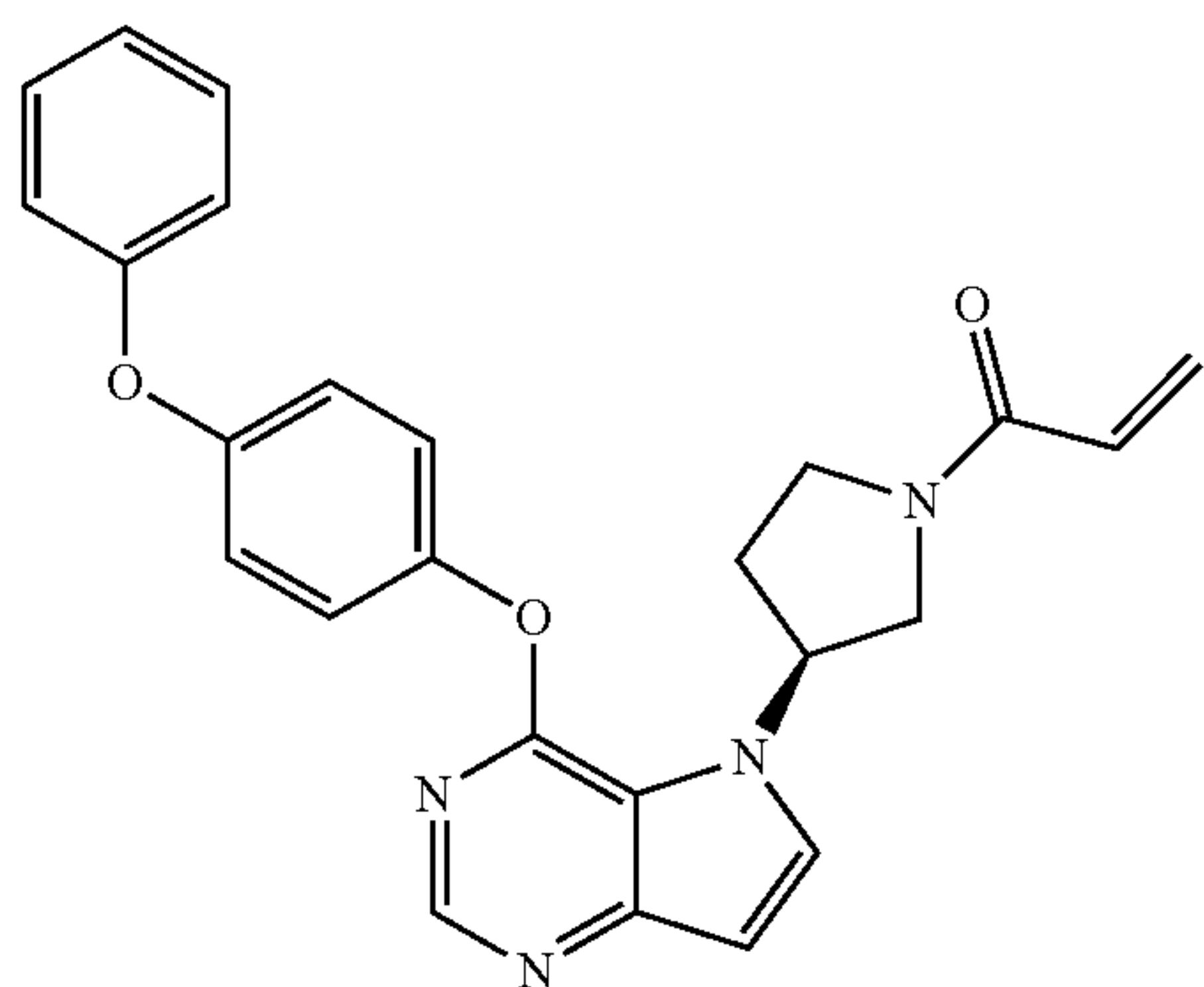
(S)-1-(3-(4-(4-phenoxyphenoxy)-5H-pyrrolo[3,2-d]pyrimidin-5-yl)pyrrolidin-1-yl)prop-2-en-1-one (5)
