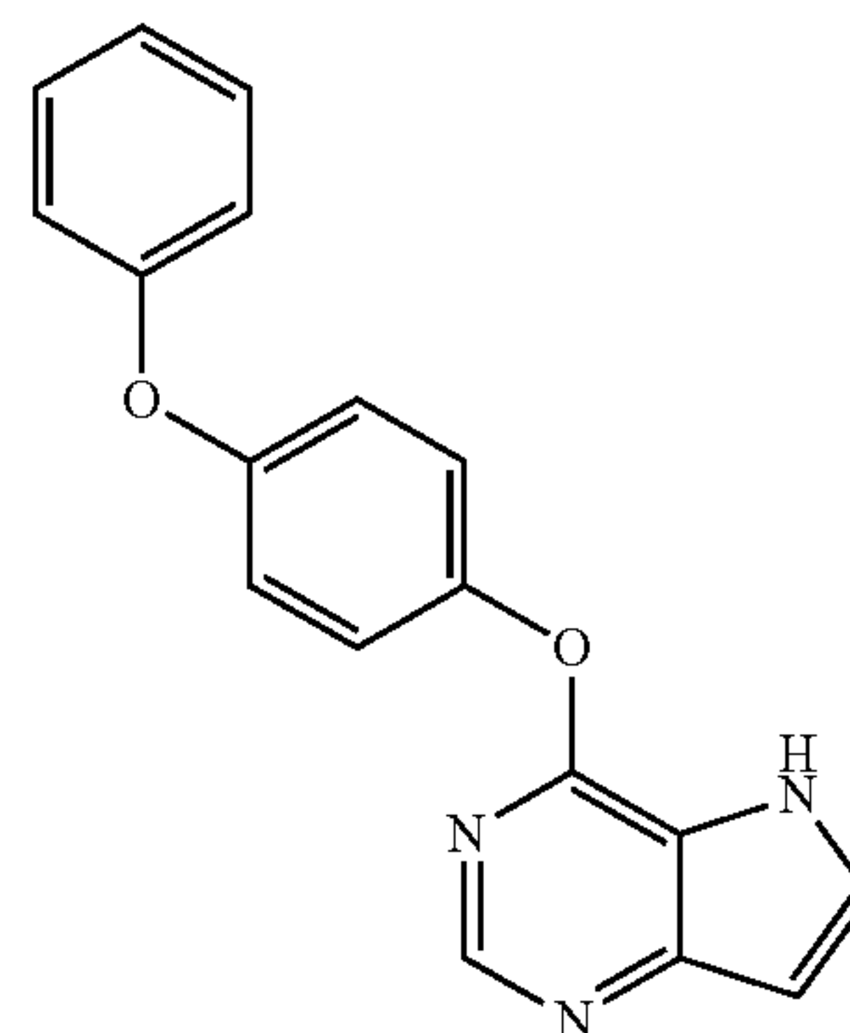
4-(4-phenoxyphenoxy)-5H-pyrrolo[3,2-d]pyrimidine (Method B)
