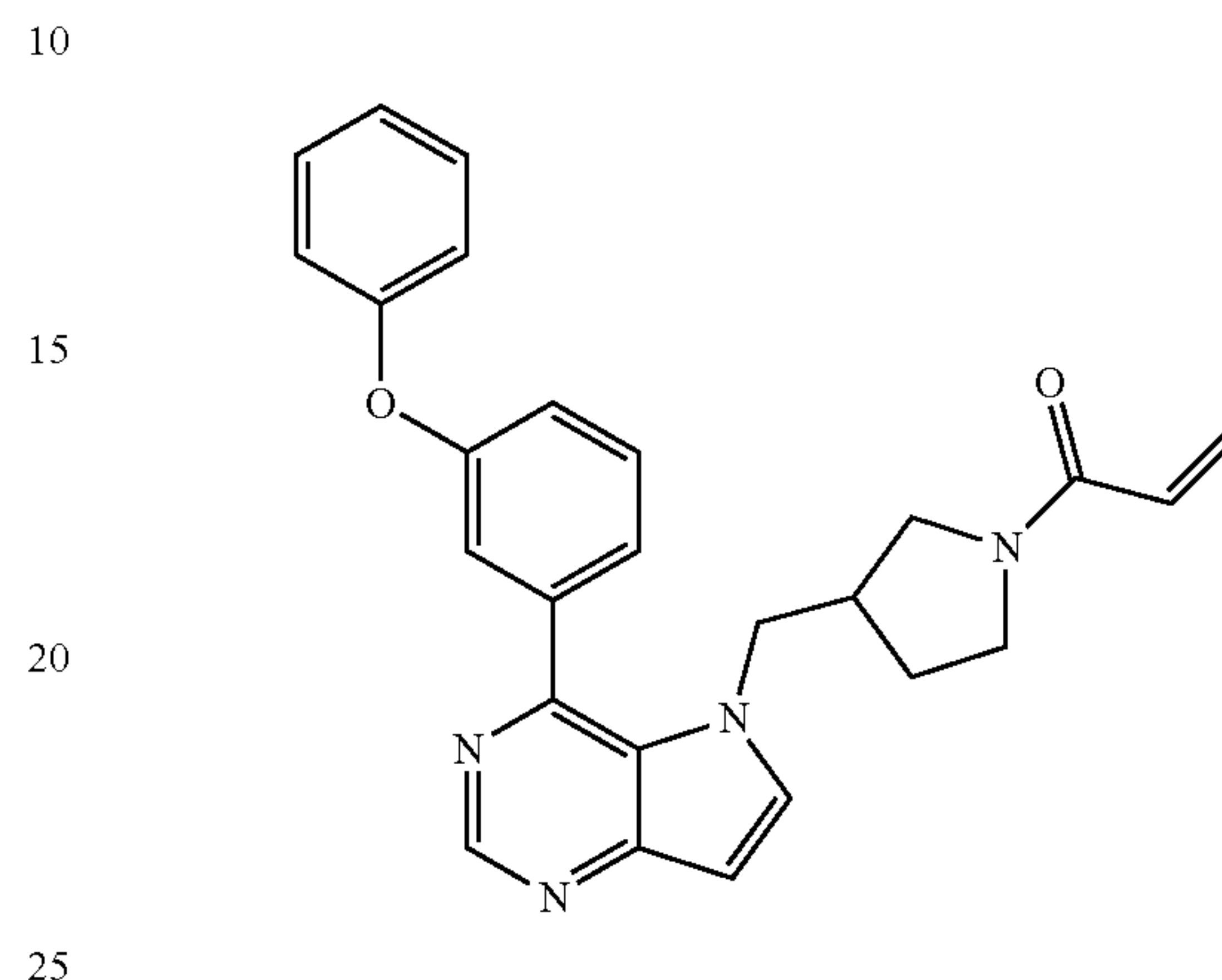
1-(3-((4-(3-phenoxyphenyl)-5H-pyrrolo[3,2-d]pyrimidin-5-yl)methyl)pyrrolidin-1-yl)prop-2-en-1-one (40)
