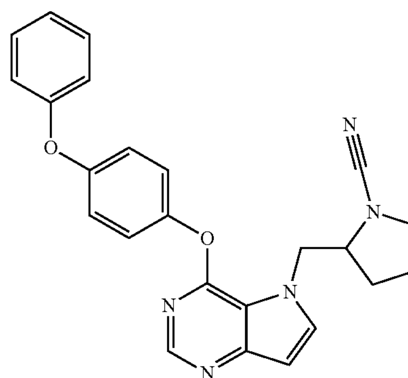
2-[[4-(4-phenoxyphenoxy)-5H-pyrrolo[3,2-d]pyrimidin-5-yl]methyl]pyrrolidine-1-carbonitrile (61)
