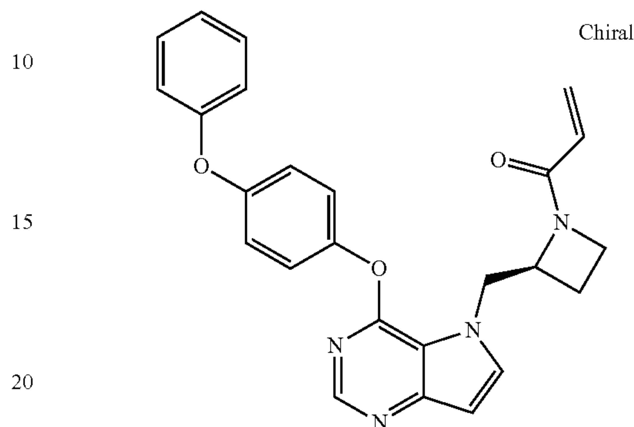
(S)-1-(2-((4-(4-phenoxyphenoxy)-5H-pyrrolo[3,2-d]pyrimidin-5-yl)methyl)azetidin-1-yl)prop-2-en-1-one (25)
