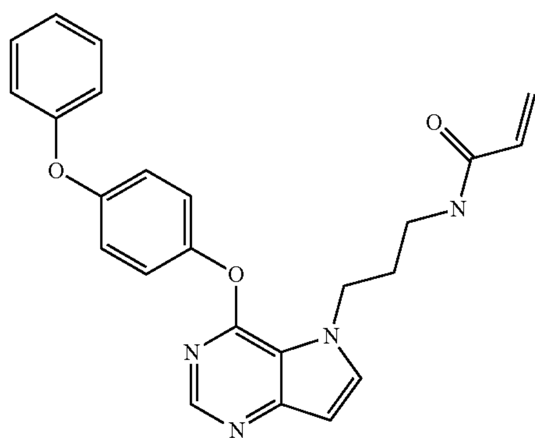
N-(3-(4-(4-phenoxyphenoxy)-5H-pyrrolo[3,2-d]pyrimidin-5-yl)propyl)acrylamide (26)
