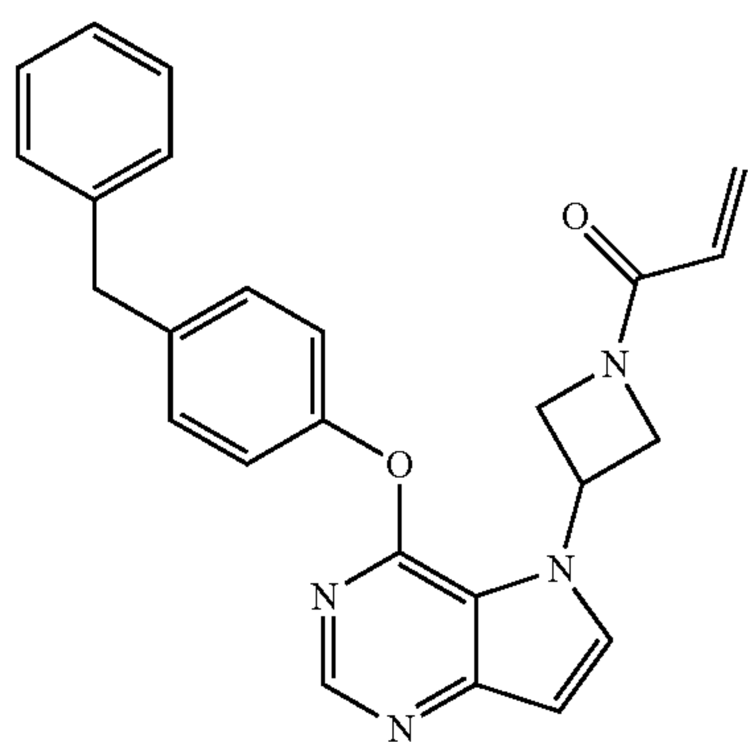
1-(3-(4-(4-benzylphenoxy)-5H-pyrrolo[3,2-d]pyrimidin-5-yl)azetidin-1-yl)prop-2-en-1-one (17)
