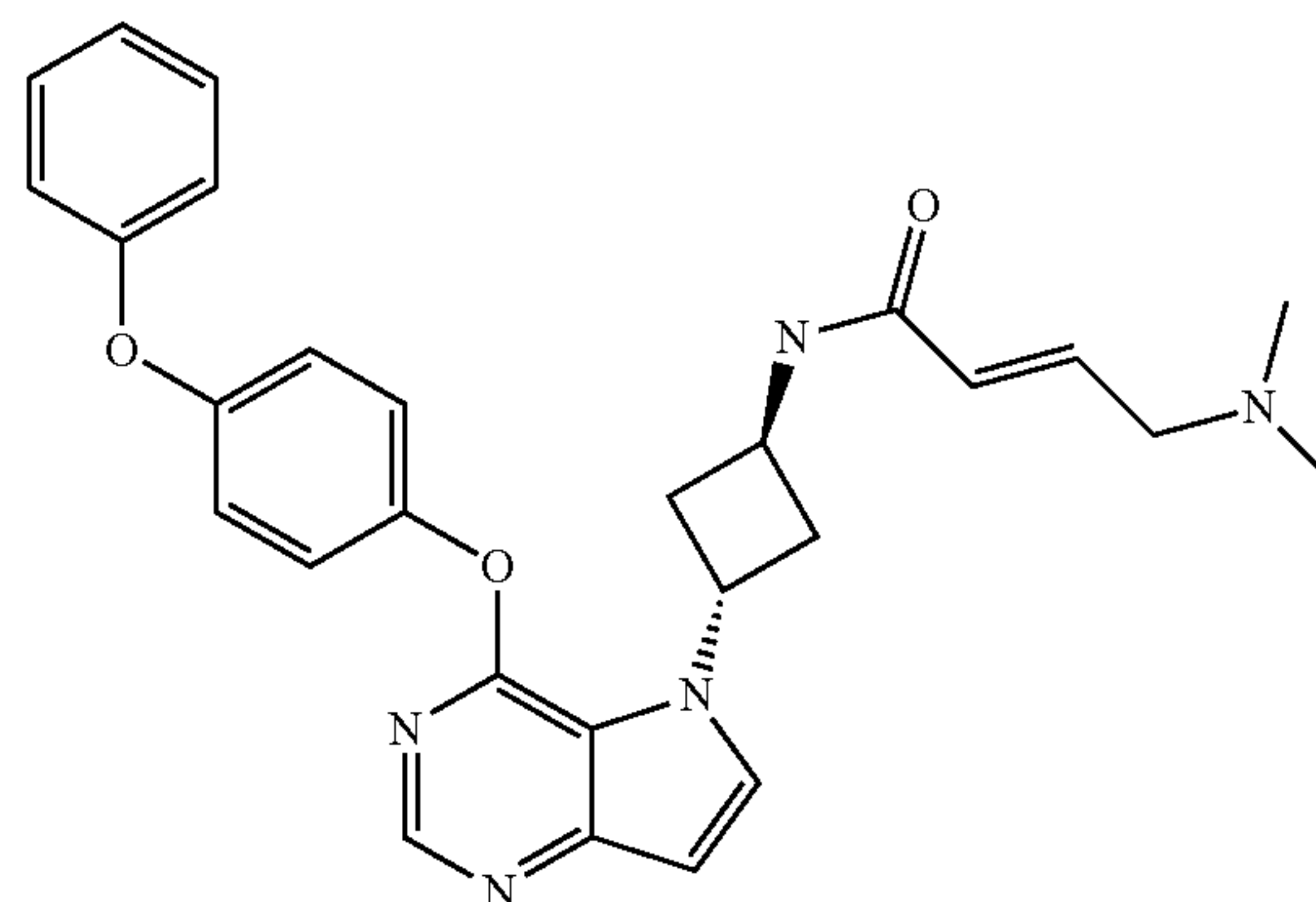
(E)-4-(dimethylamino)-N-(trans-3-(4-(4-phenoxyphenoxy)-5H-pyrrolo[3,2-d]pyrimidin-5-yl)cyclobutyl)but-2-enamide (33)
