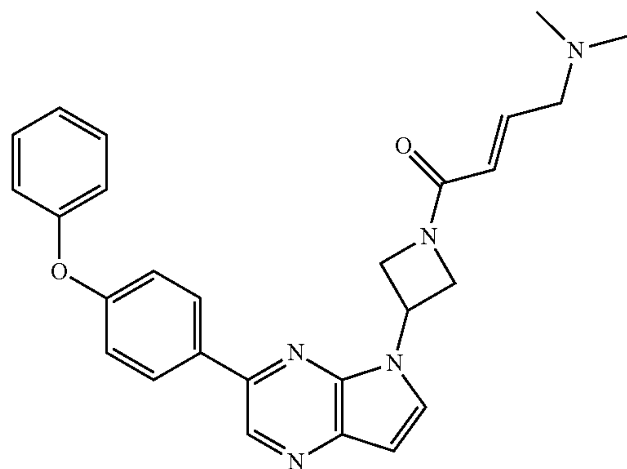
(E)-4-(dimethylamino)-1-(3-(3-(4-phenoxyphenyl)-5H-pyrrolo[2,3-b]pyrazin-5-yl)azetidin-1-yl)but-2-en-1-one (24)
