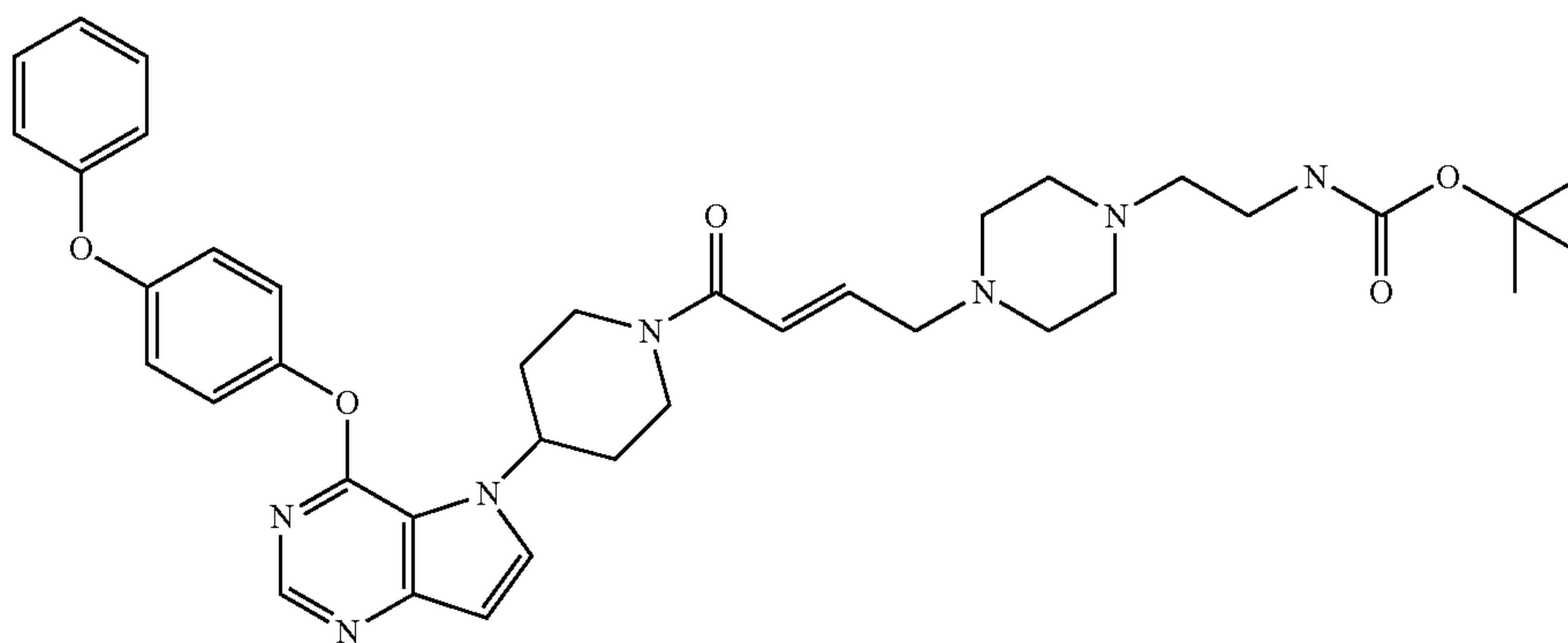
tert-butyl (E)-(2-(4-(4-oxo-4-(4-(4-(4-phenoxyphenoxy)-5H-pyrrolo[3,2-d]pyrimidin-5-yl)piperidin-1-yl)but-2-en-1-yl)piperazin-1-yl)ethyl)carbamate
