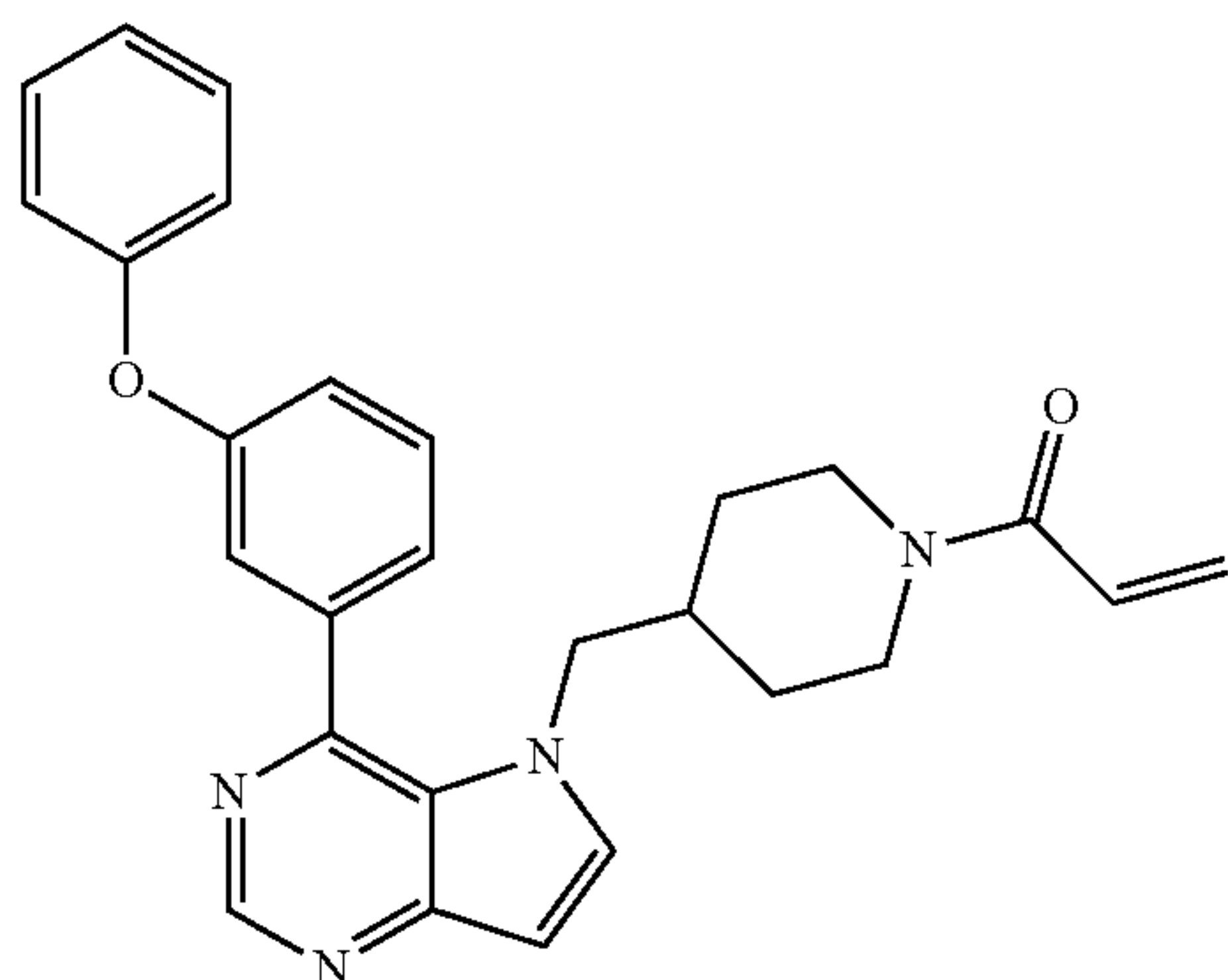
1-(4-((4-(3-phenoxyphenyl)-5H-pyrrolo[3,2-d]pyrimidin-5-yl)methyl)piperidin-1-yl)prop-2-en-1-one (45)
