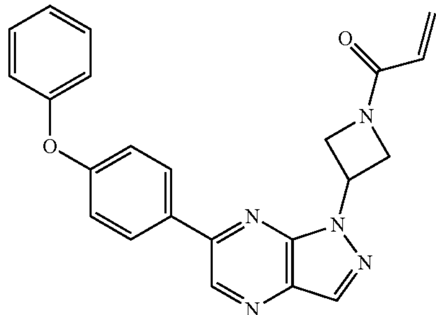
1-(3-(6-(4-phenoxyphenyl)-1H-pyrazolo[3,4-b]pyrazin-1-yl)azetidin-1-yl)prop-2-en-1-one (23)
