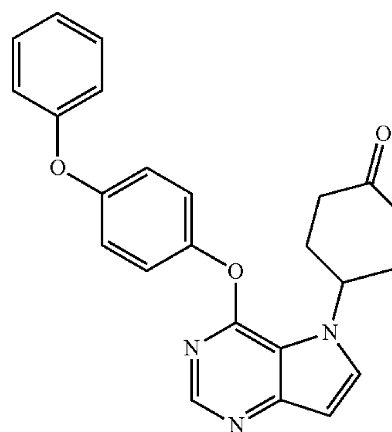
4-[4-(4-phenoxyphenoxy)-5H-pyrrolo[3,2-d]pyrimidin-5-yl]cyclohexan-1-one
