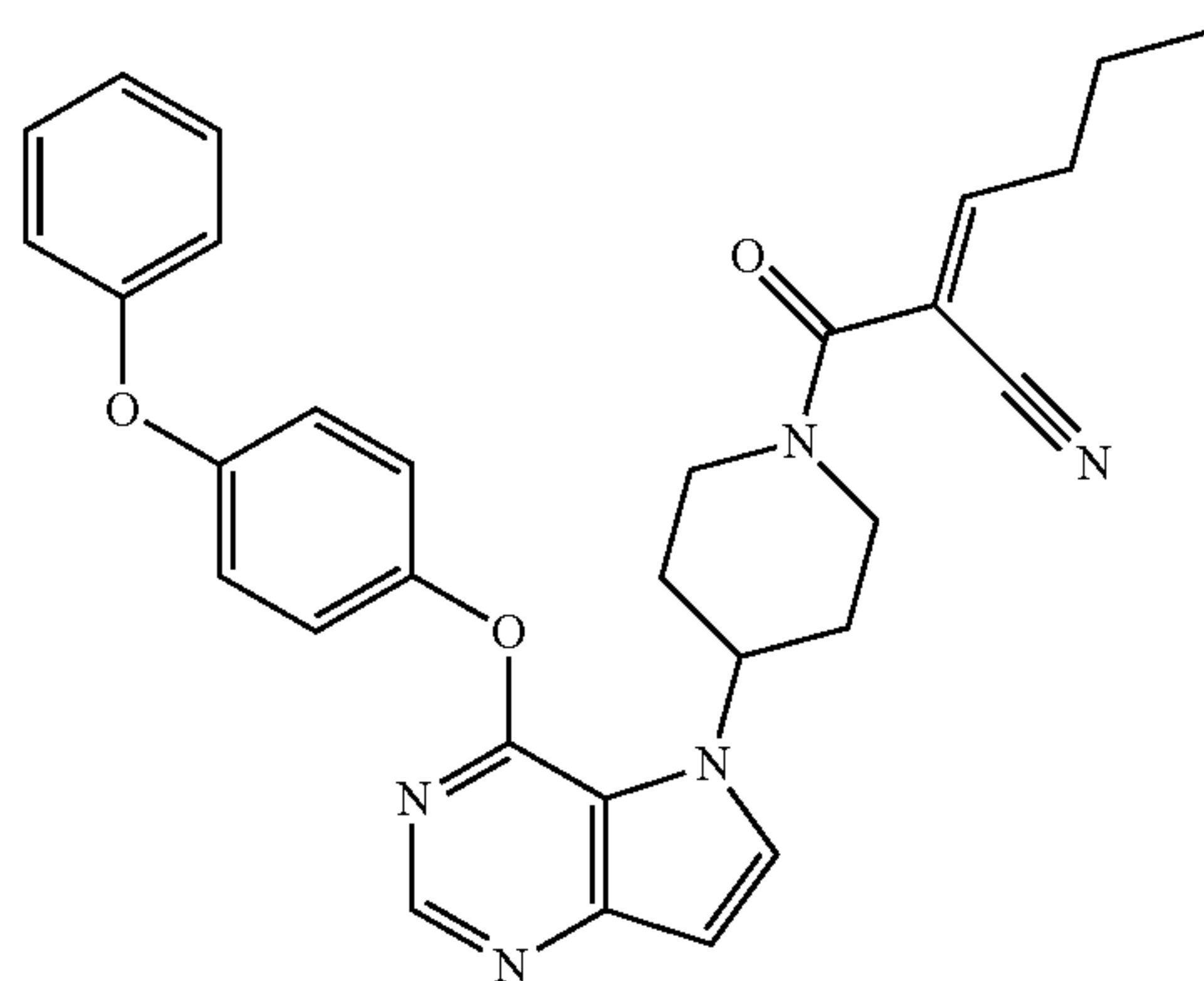
(E)-2-(4-(4-(4-phenoxyphenoxy)-5H-pyrrolo[3,2-d]pyrimidin-5-yl)piperidine-1-carbonyl)hex-2-enenitrile (55)
