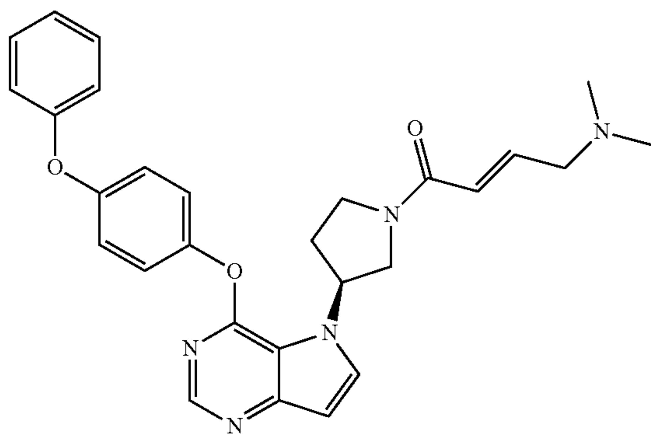
(S,E)-4-(dimethylamino)-1-(3-(4-(4-phenoxyphenoxy)-5H-pyrrolo[3,2-d]pyrimidin-5-yl)pyrrolidin-1-yl)but-2-en-1-one (18)
