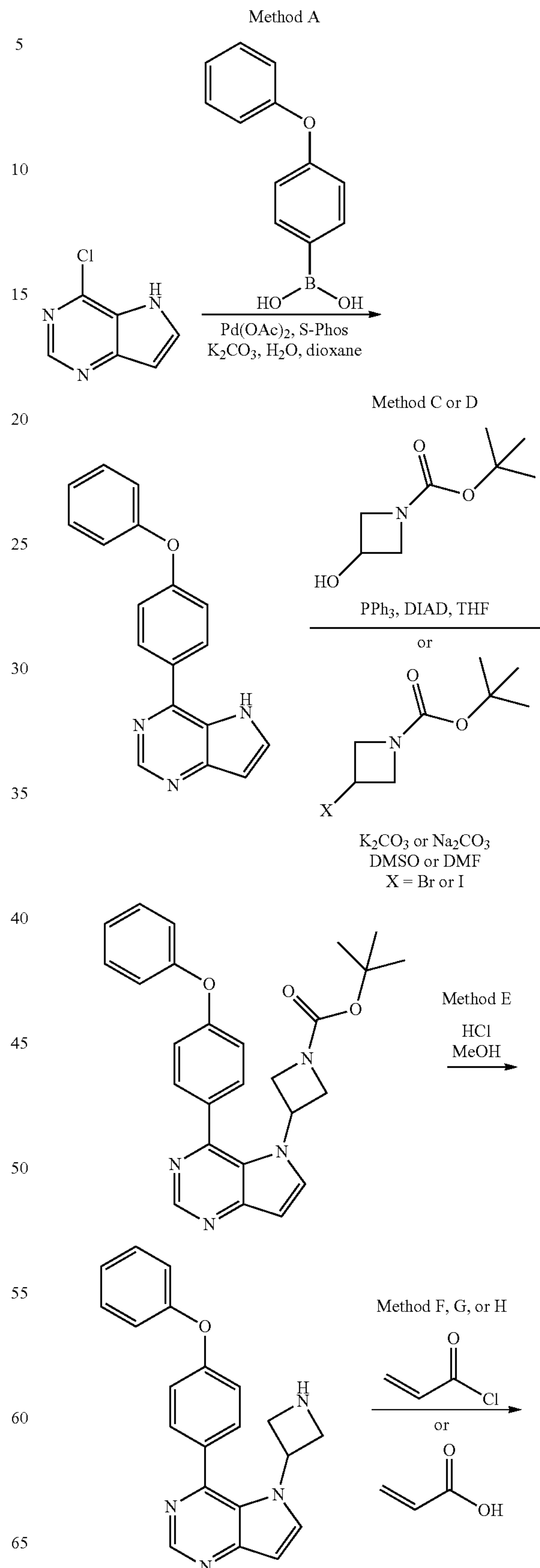
Scheme 1
