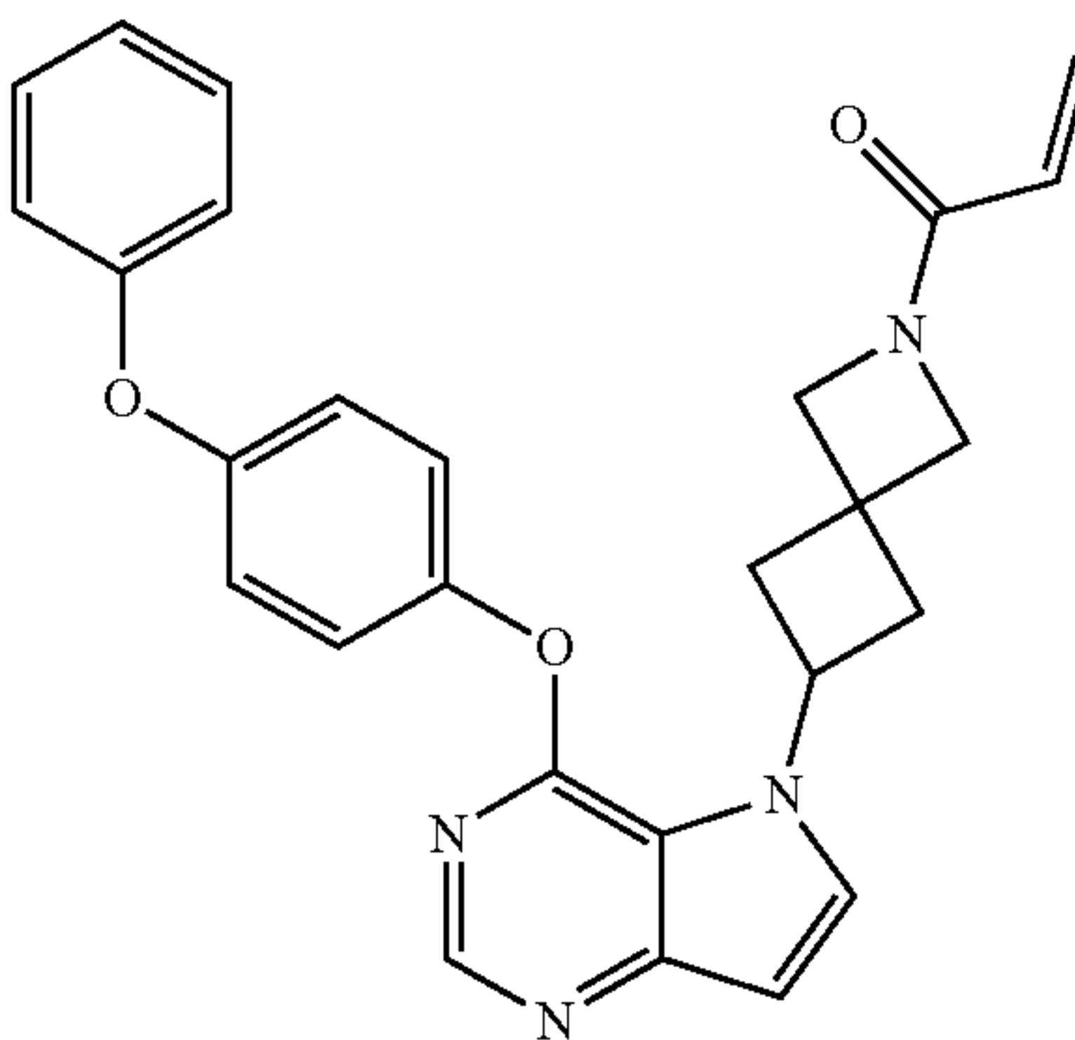
1-(6-(4-(4-phenoxyphenoxy)-5H-pyrrolo[3,2-d]pyrimidin-5-yl)-2-azaspiro[3.3]heptan-2-yl)prop-2-en-1-one (28)
