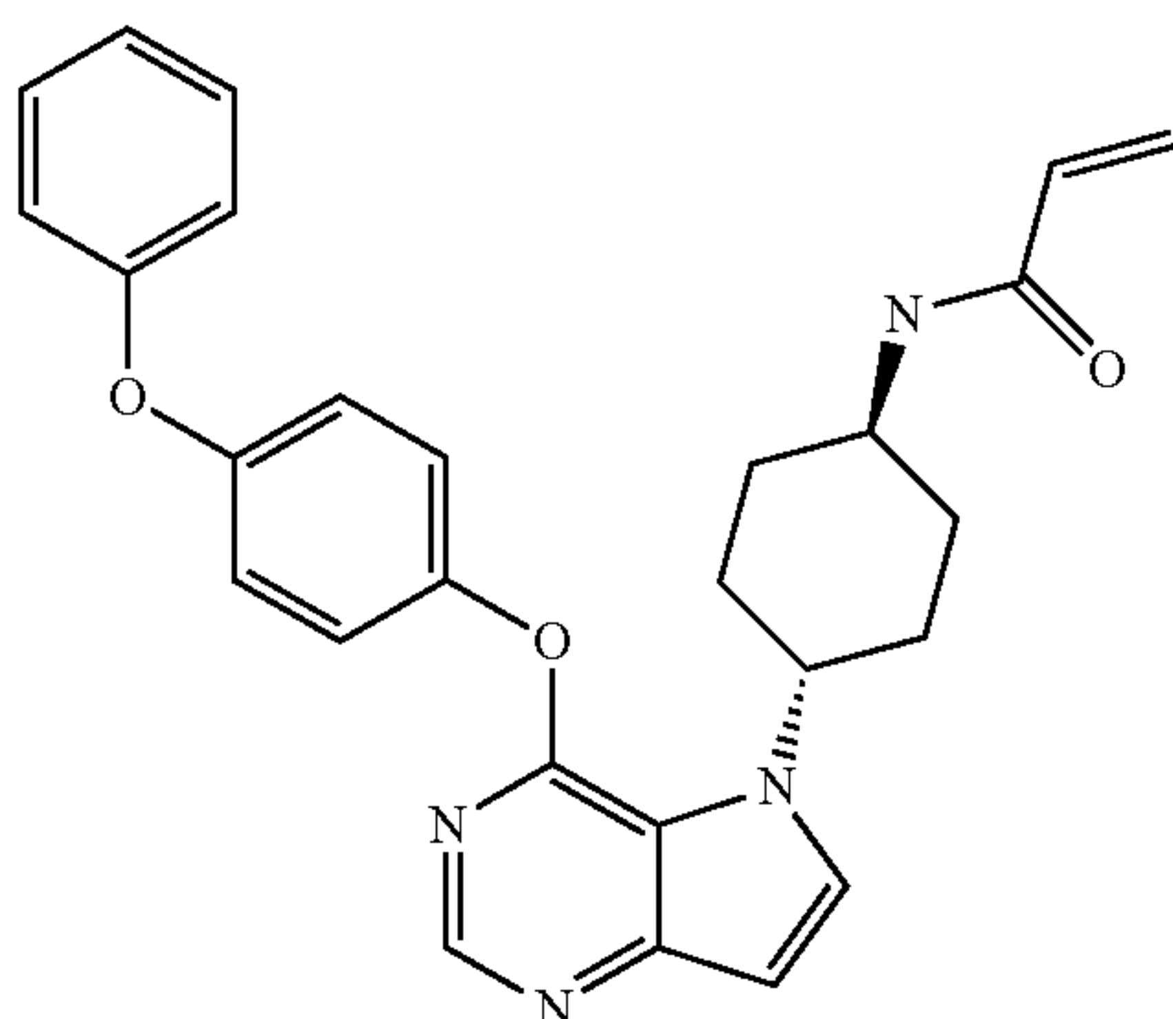
N-(trans-4-(4-(4-phenoxyphenoxy)-5H-pyrrolo[3,2-d]pyrimidin-5-yl)cyclohexyl)acrylamide (39)
