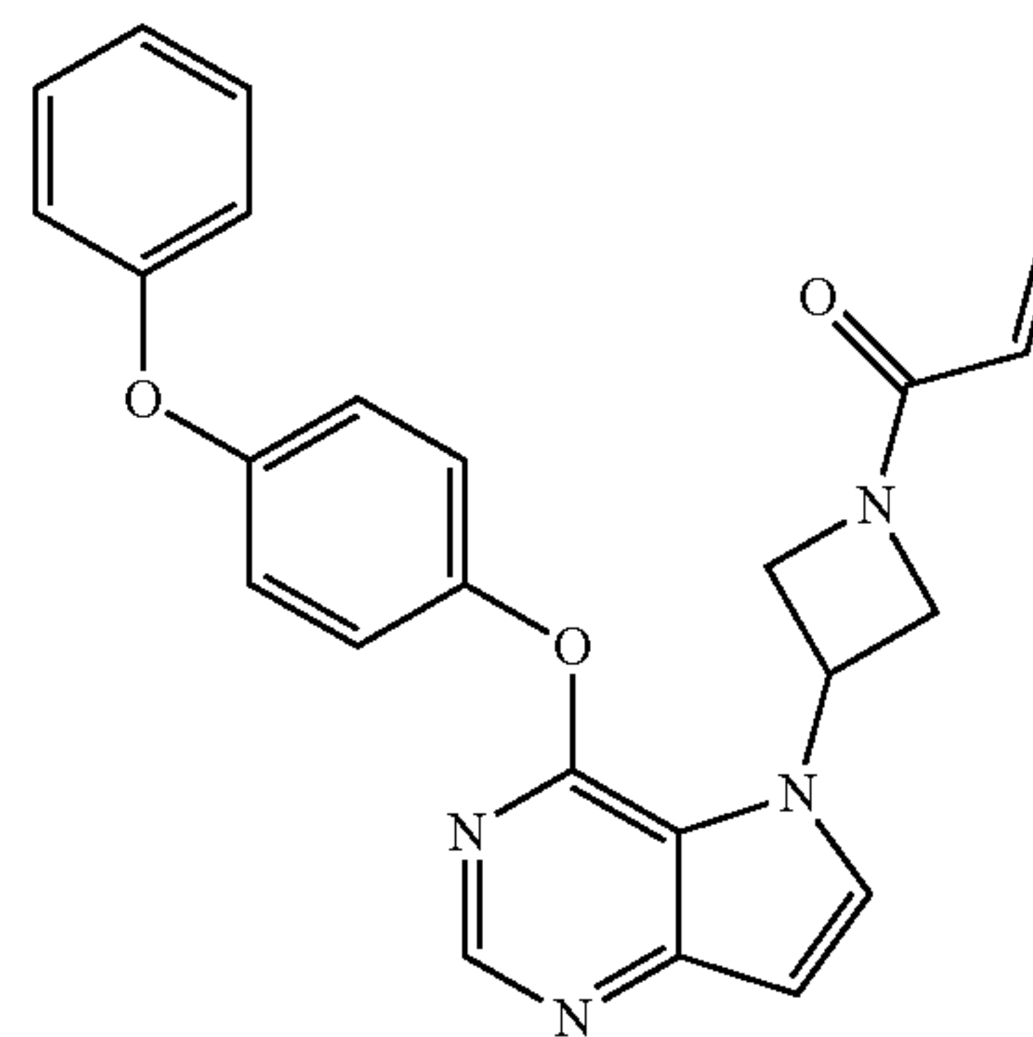
1-(3-(4-((4-phenoxyphenyl)amino)-5H-pyrrolo[3,2-d]pyrimidin-5-yl)azetidin-1-yl)prop-2-en-1-one (6)
