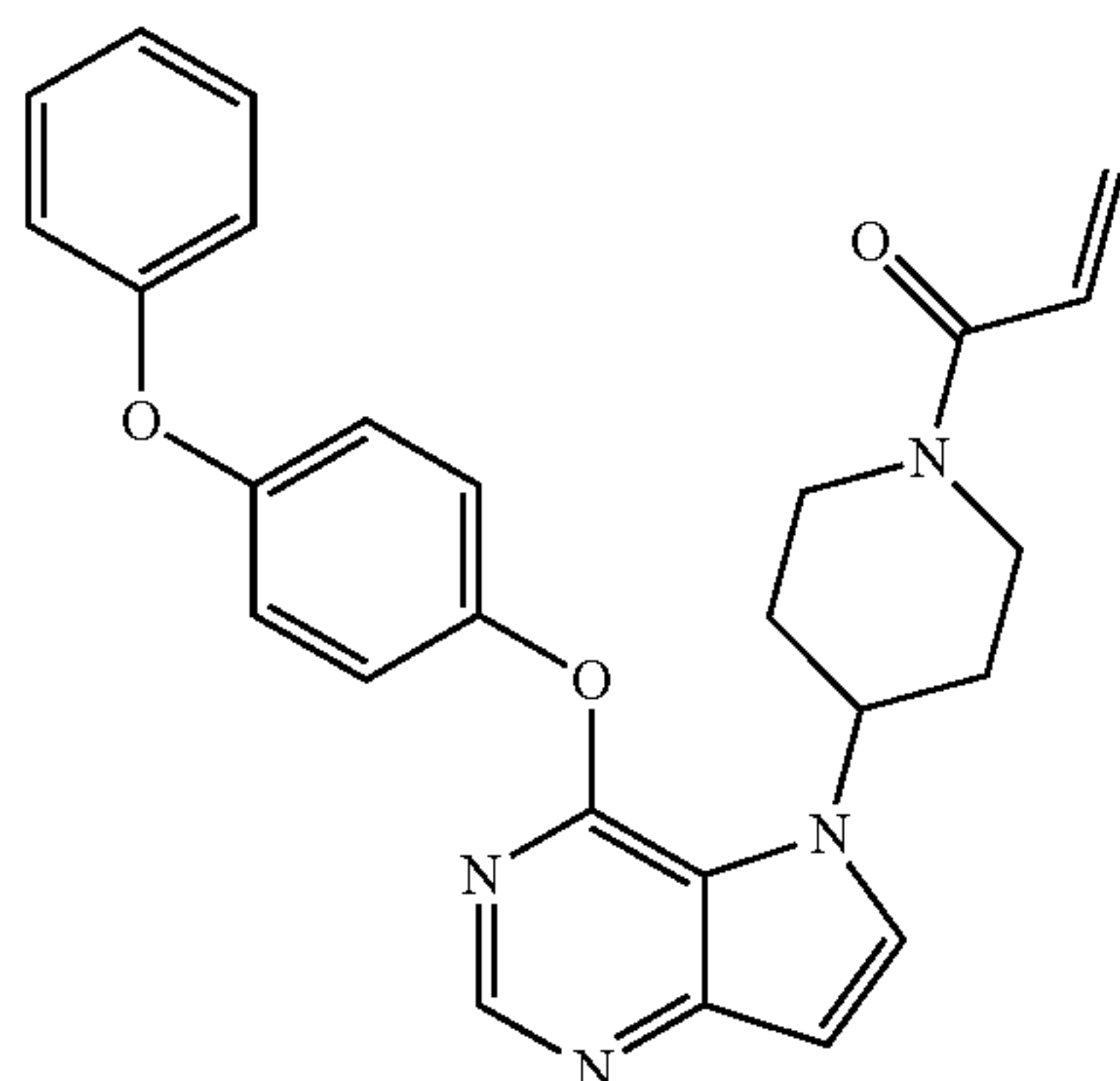
1-(4-(4-(4-phenoxyphenyl)-5H-pyrrolo[3,2-d]pyrimidin-5-yl)piperidin-1-yl)prop-2-en-1-one (2)
