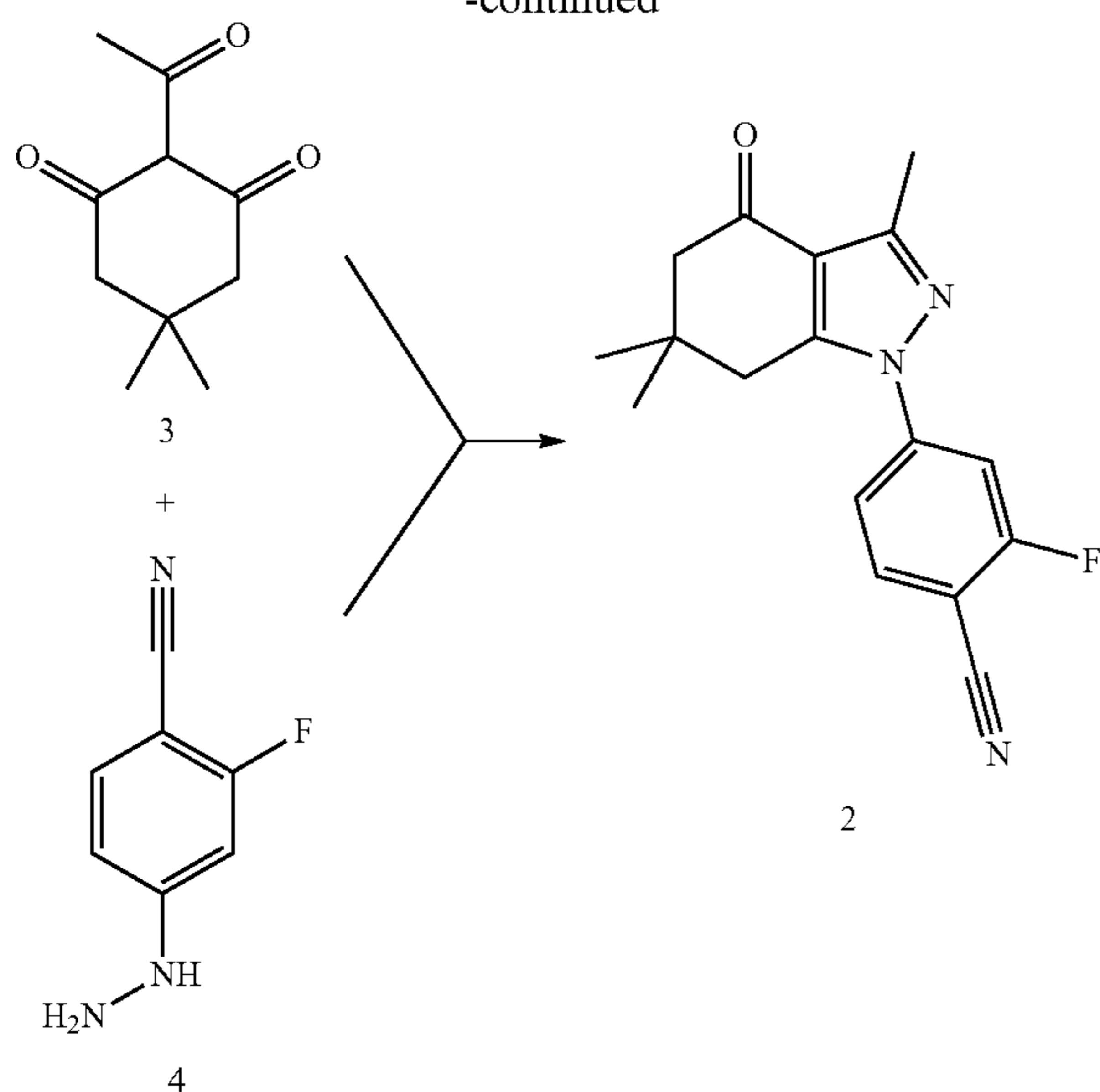
2-Acetyl-5,5-dimethylcyclohexane-1,3-dione (3)
