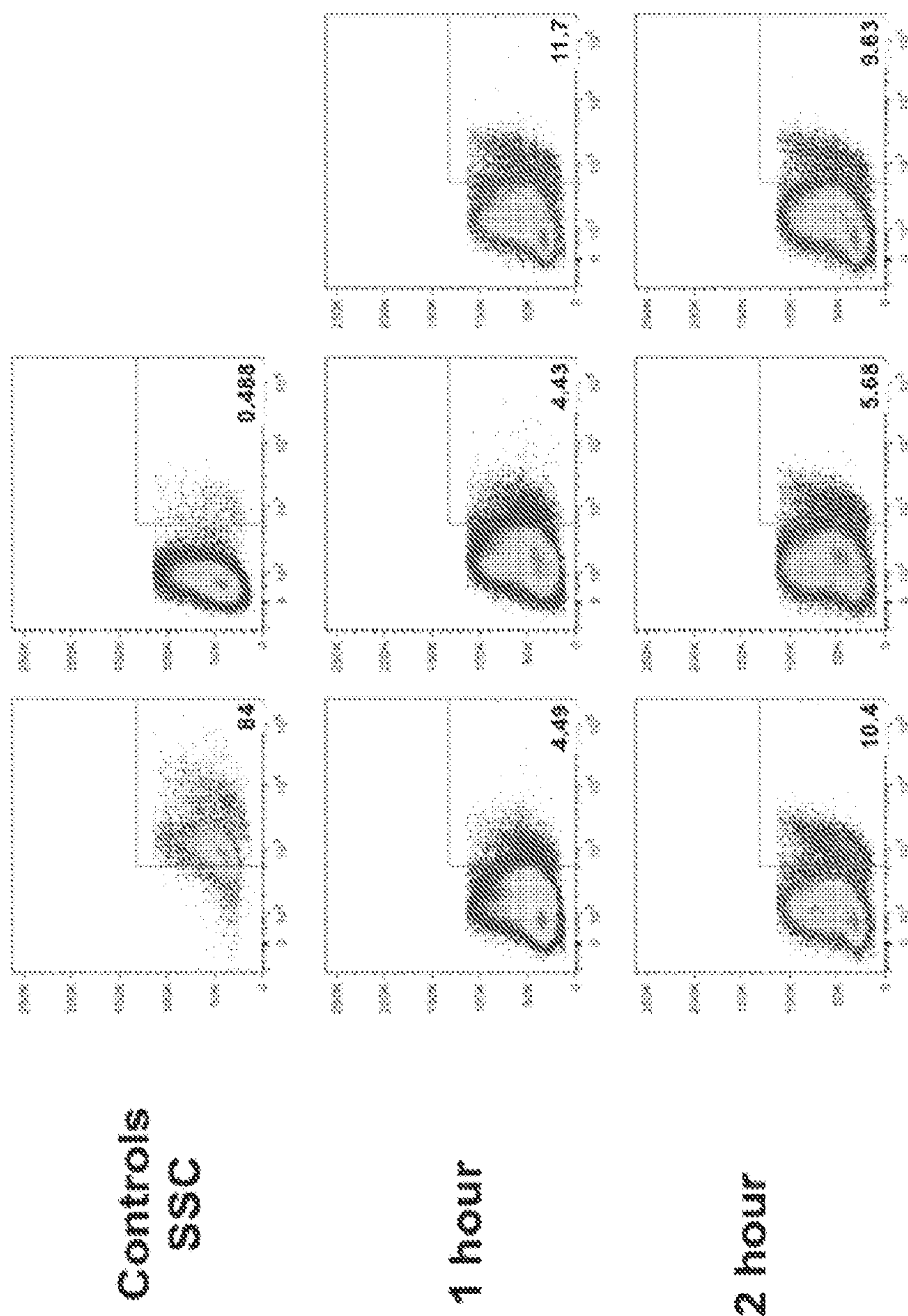
Compound 10
