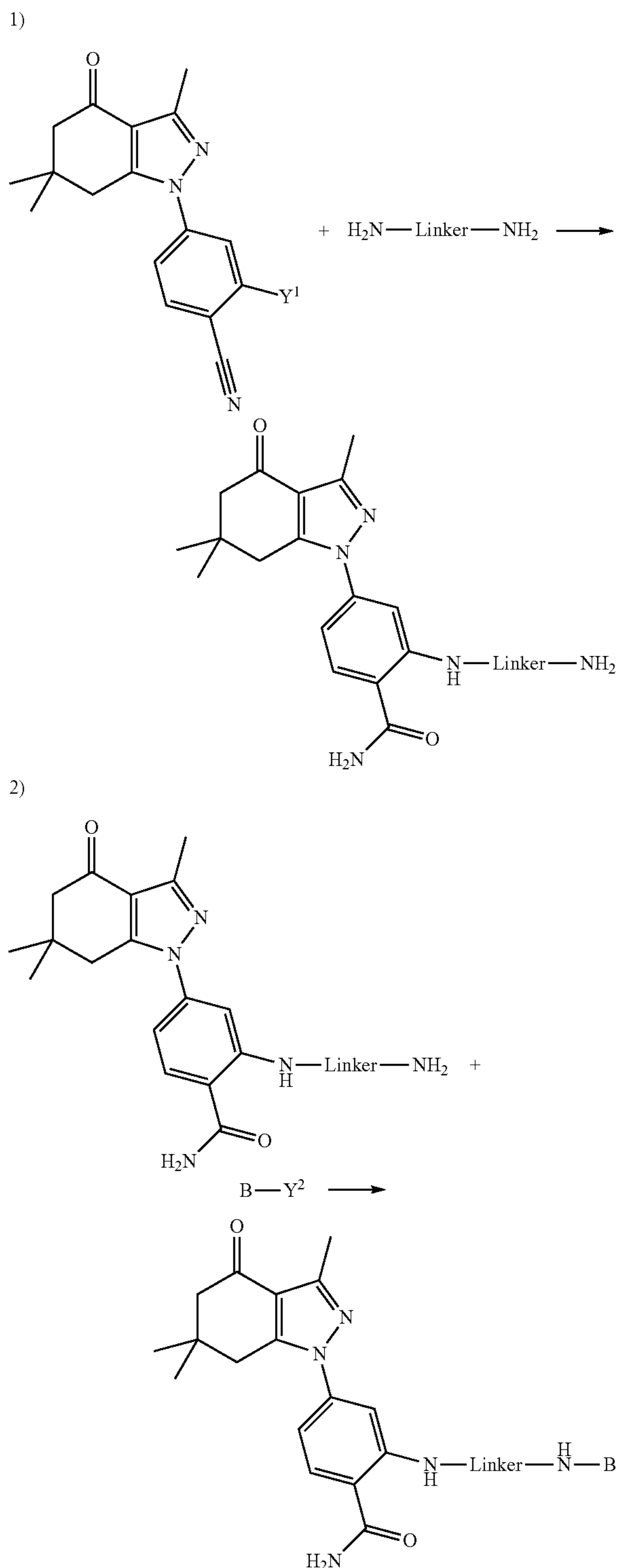
Scheme 1. Exemplary Synthesis
