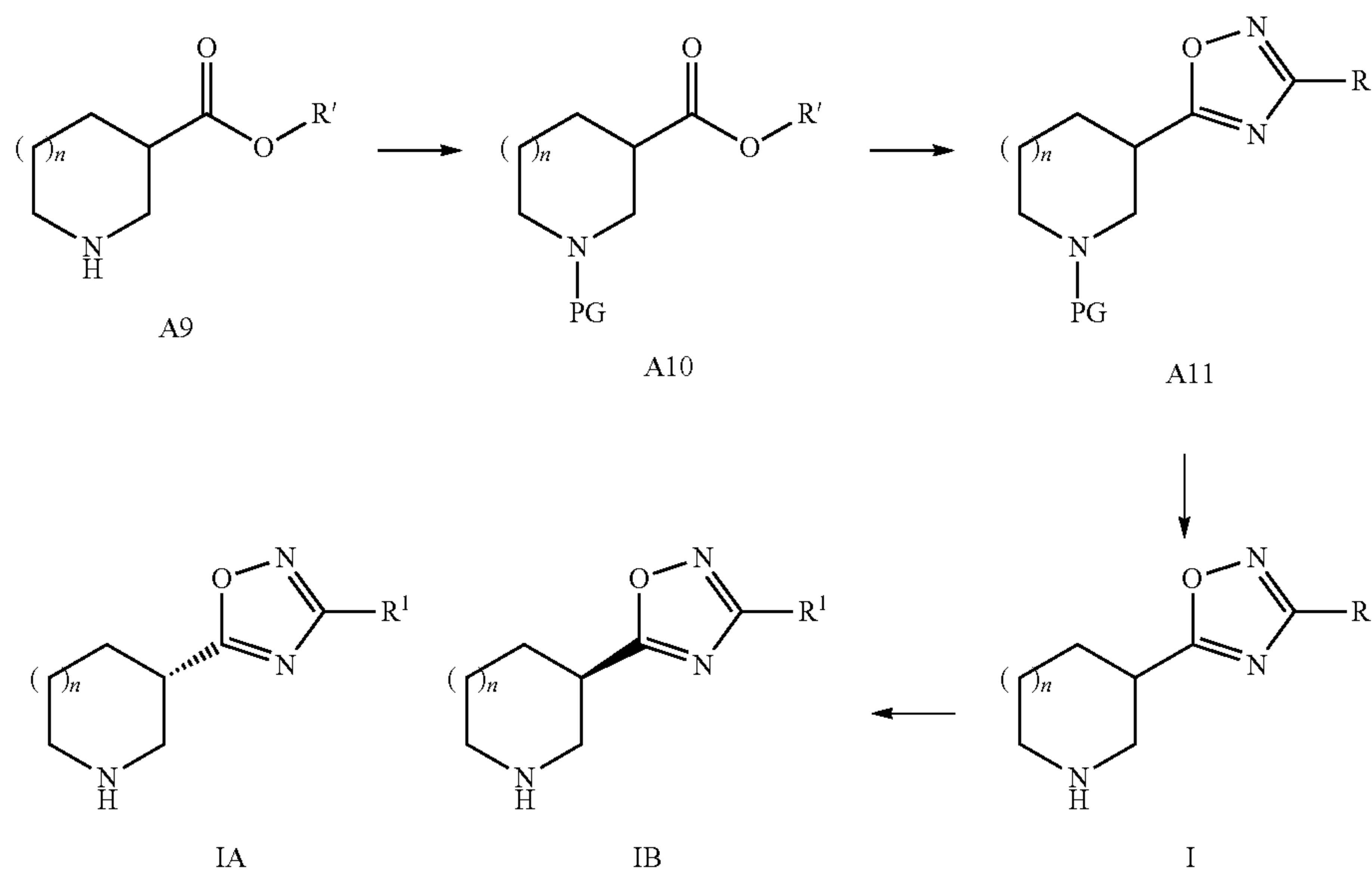
Scheme 4
