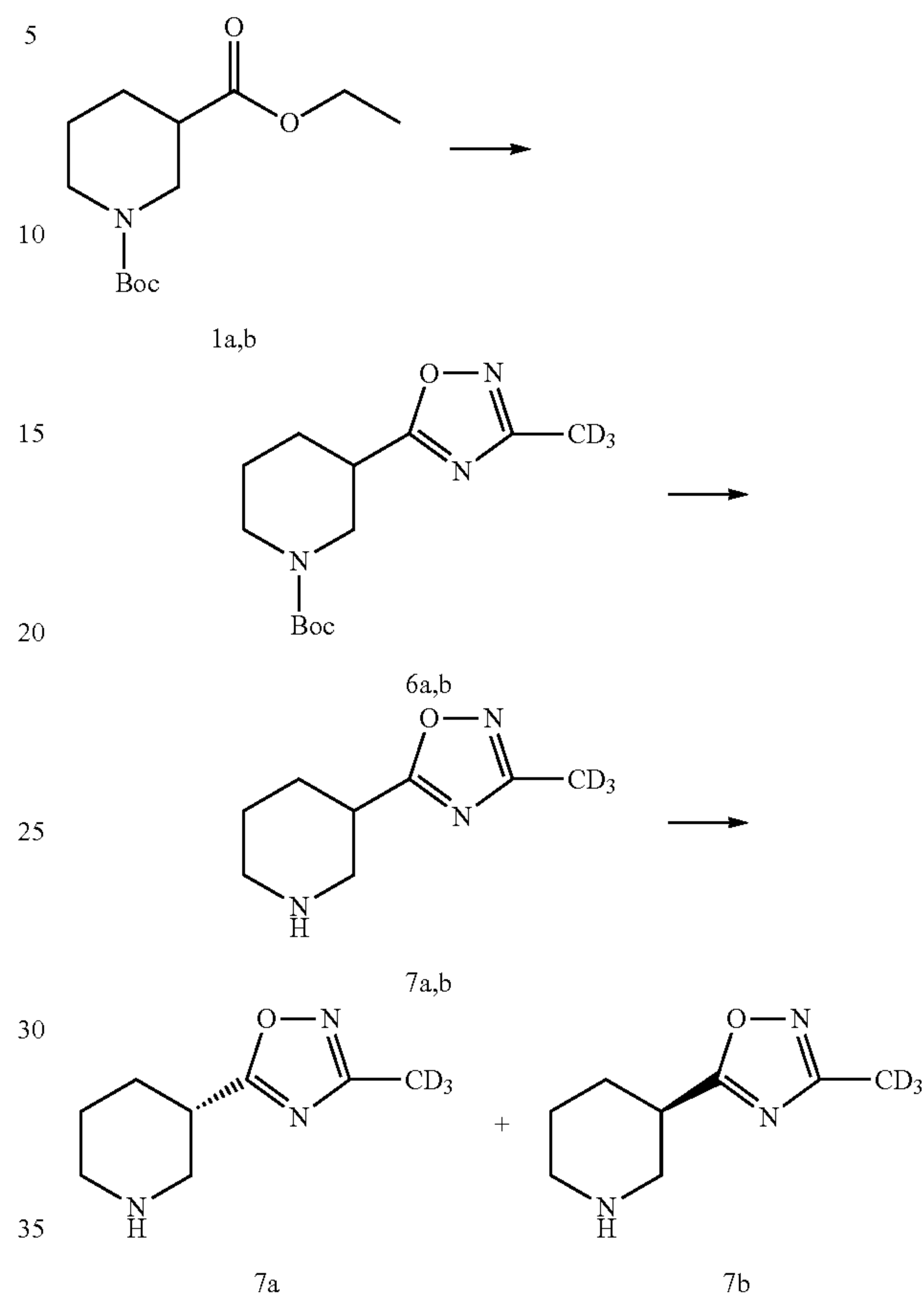
tert-Butyl 3-(3-D3-methyl-1,2,4-oxadiazol-5-yl) piperidine-1-carboxylate (6a,b)
