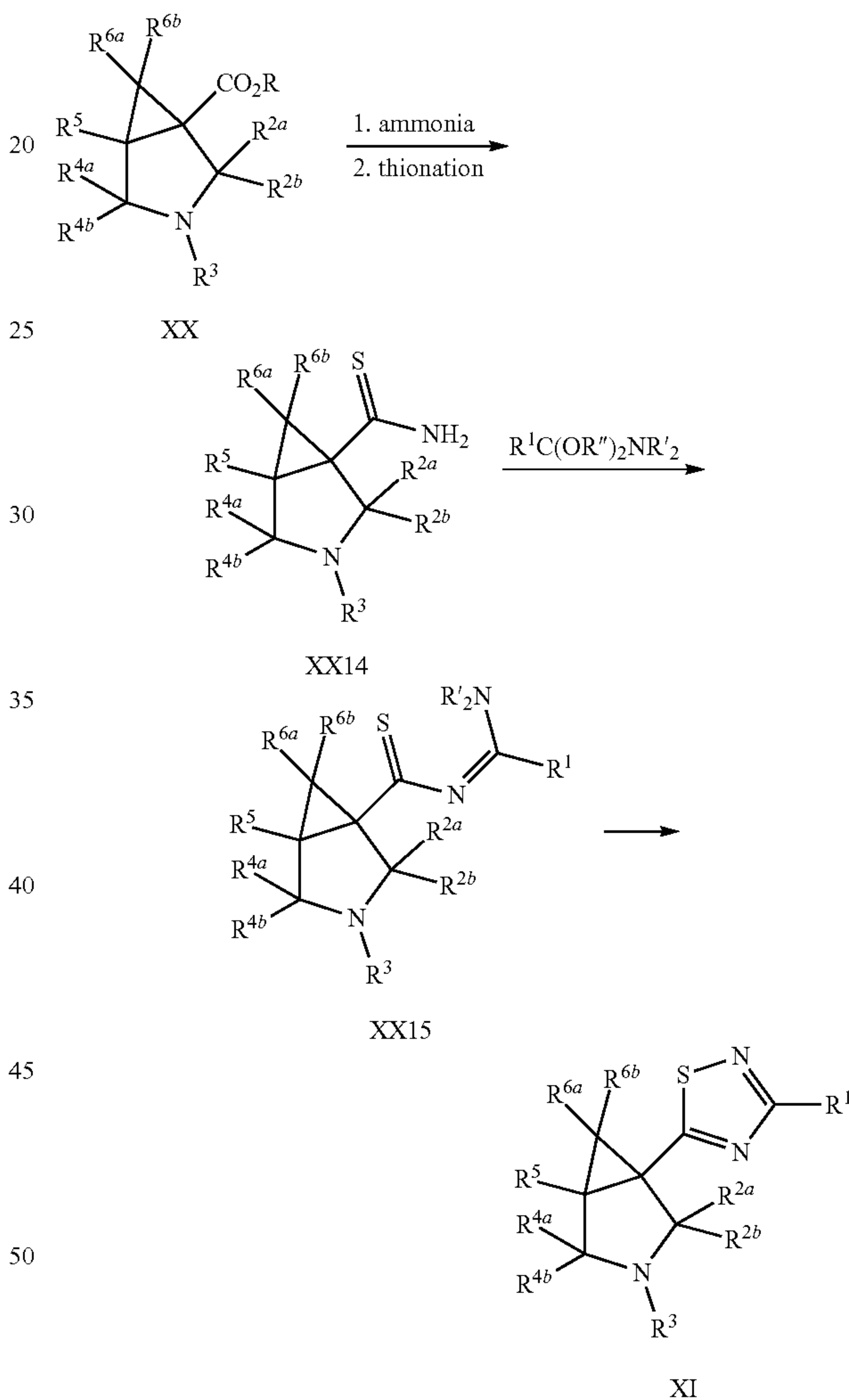
Scheme 8
