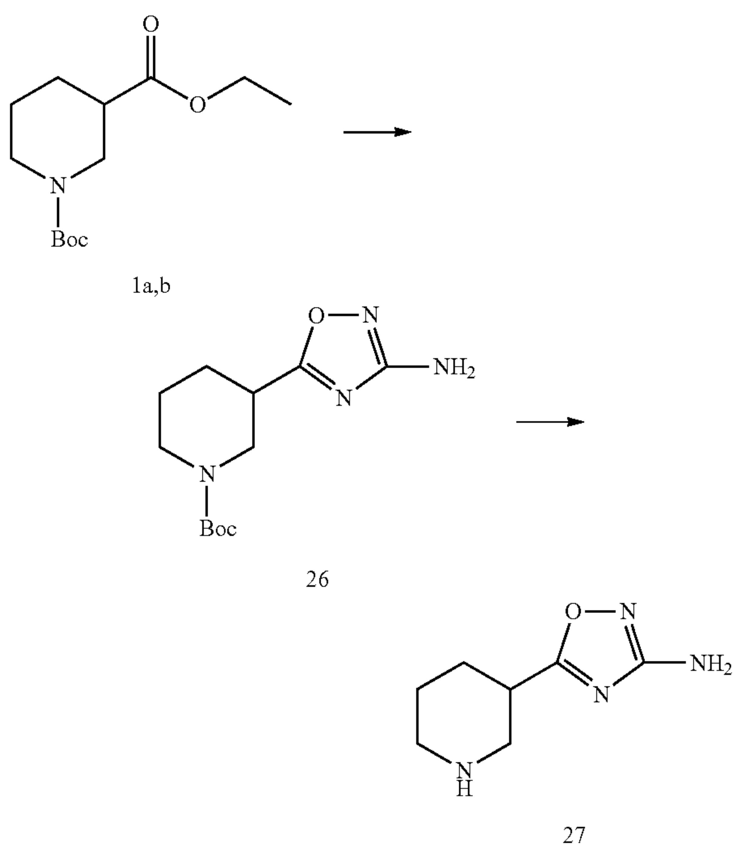
tert-Butyl 3-(3-(3-amino-1,2,4-oxadiazol-5-yl)piperidine-1-carboxylate (26)
