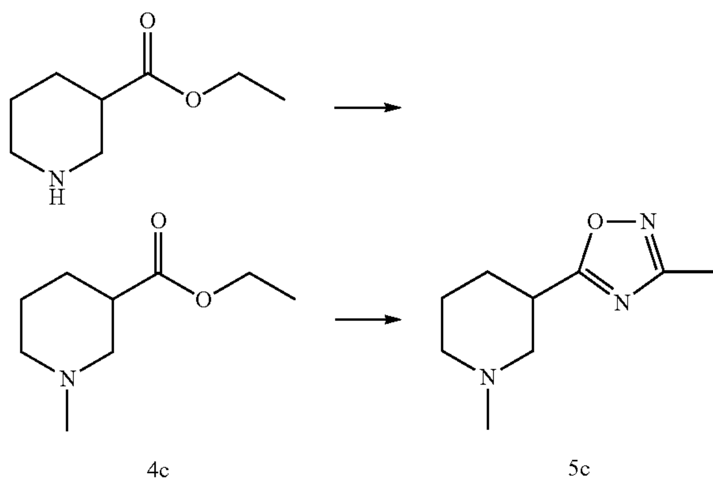
N-Methyl-ethyl nipecotate (4c)
