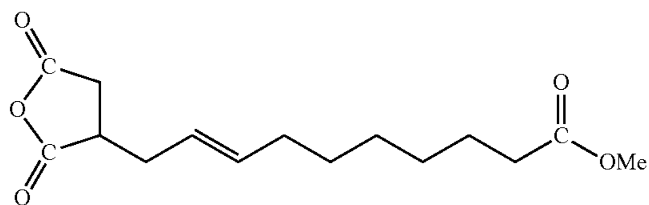
Maleinated 9-DAMe
