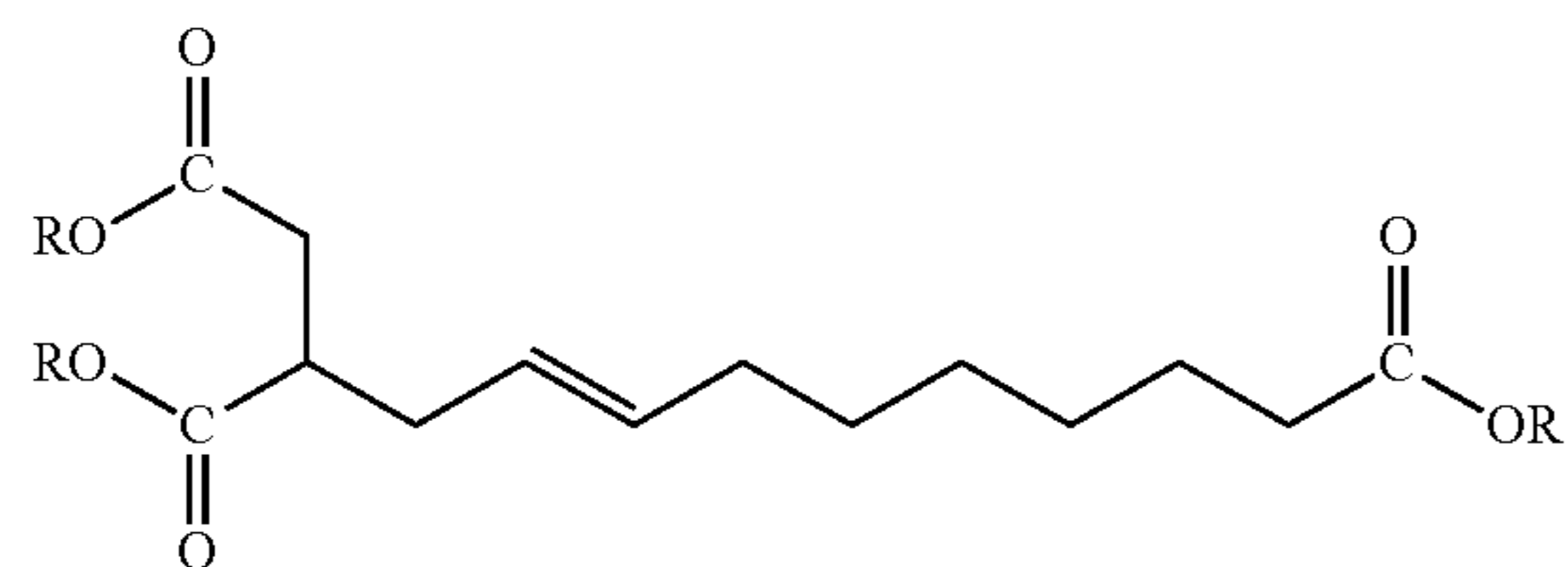
Triester
