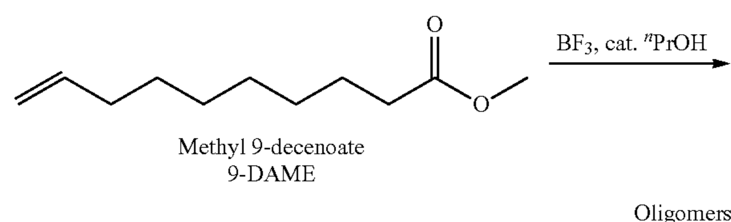
Scheme 1. \text{BF}_3 -mediated homo-oligomerization of methyl 9-decenoate.
