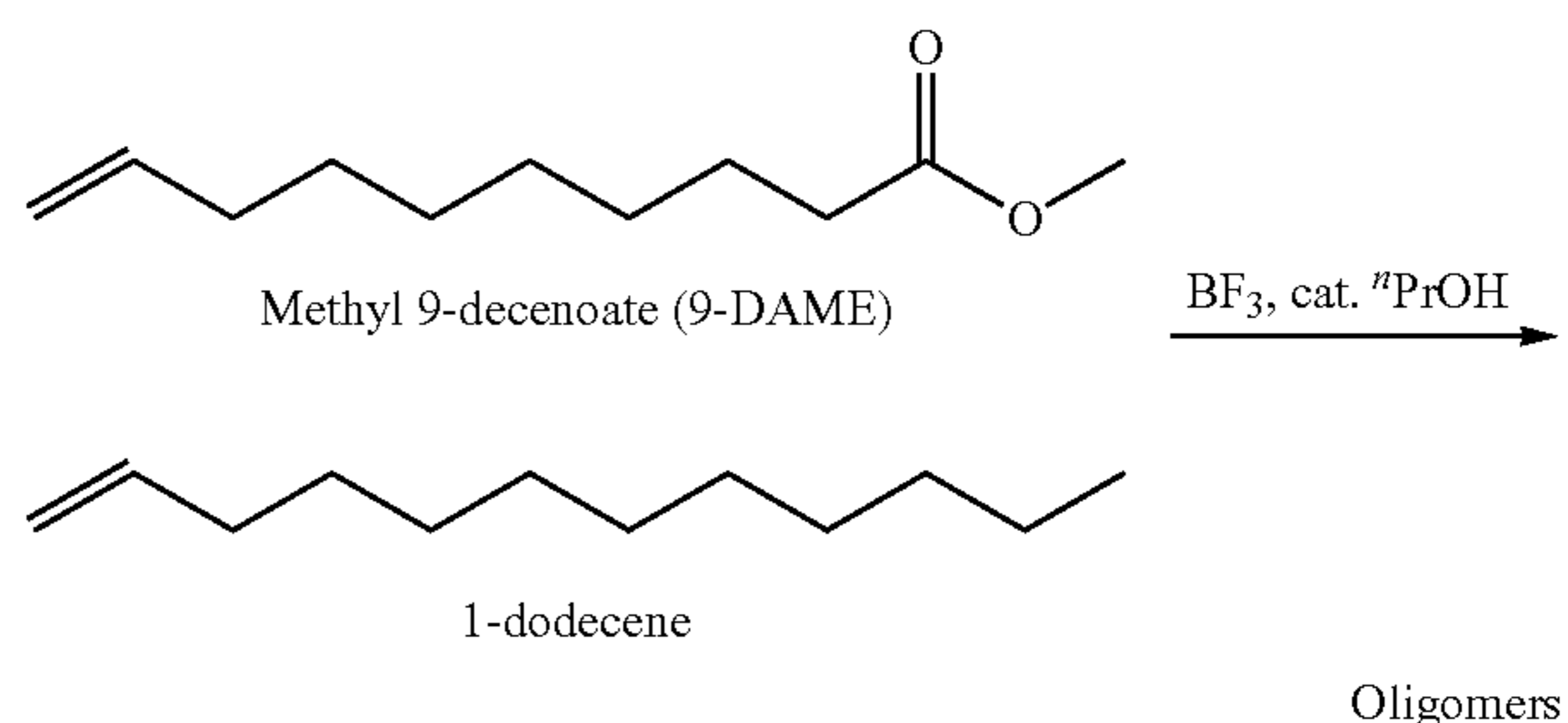
Scheme 1. BF 3 -mediated co-oligomerization of methyl 9-decenoate and 1-dodecene.
