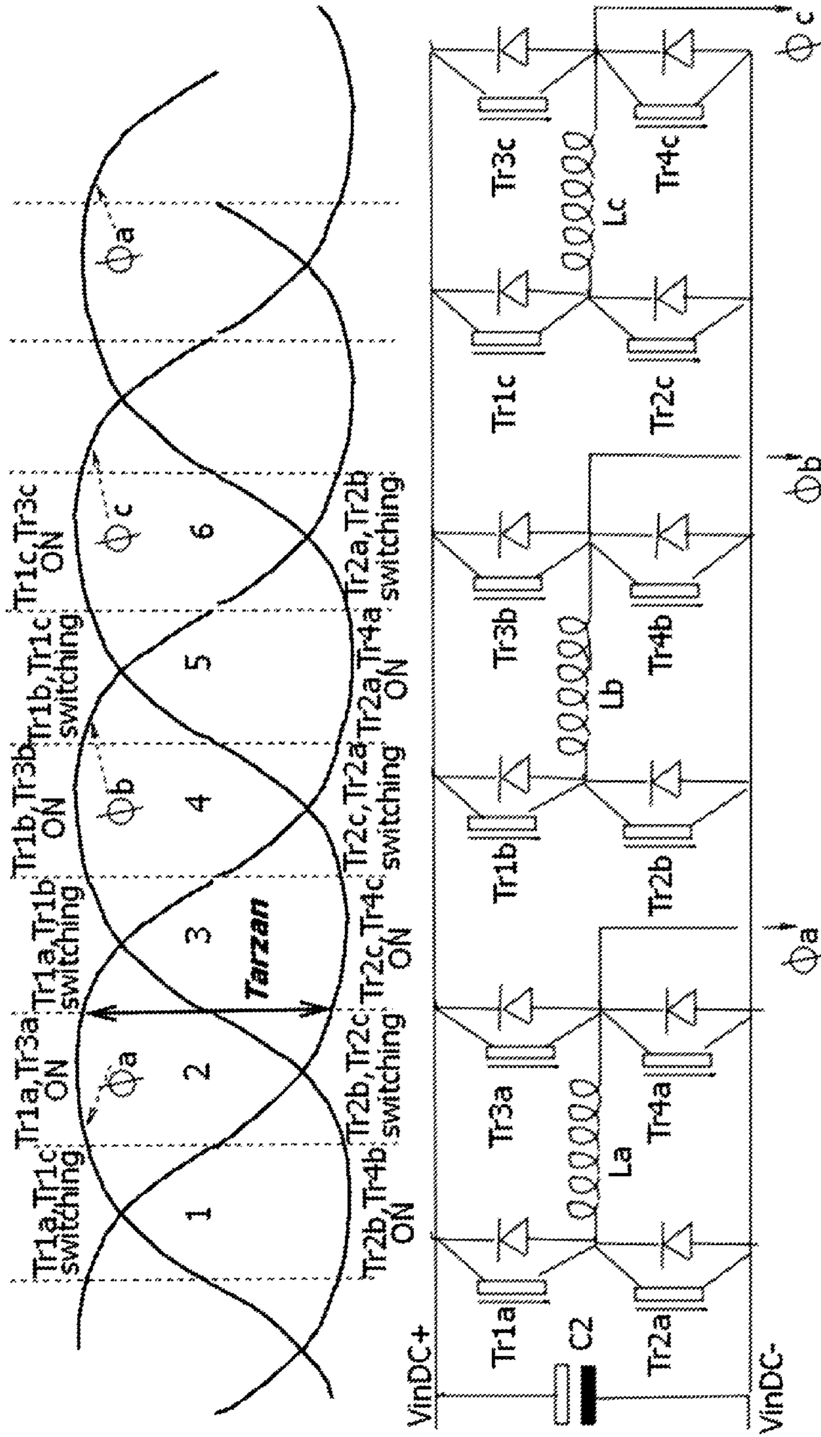
FIGURE 24: ANOTHER ARRANGEMENT OF A 3-PHASE GRID-INTERTIE INVERTER
