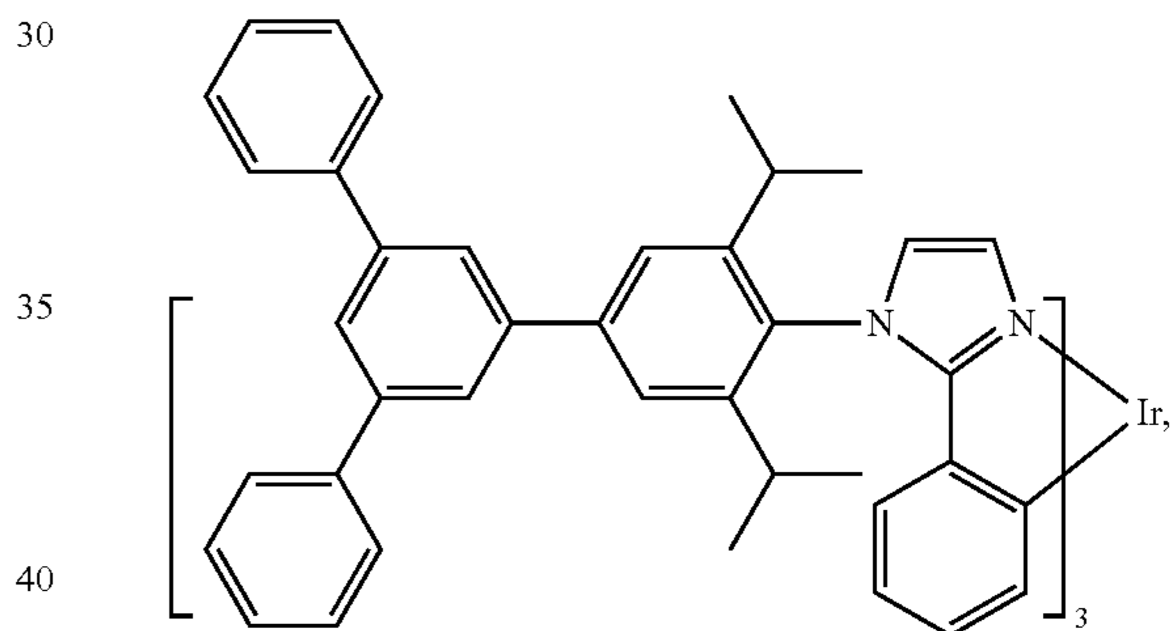
Compound 30
