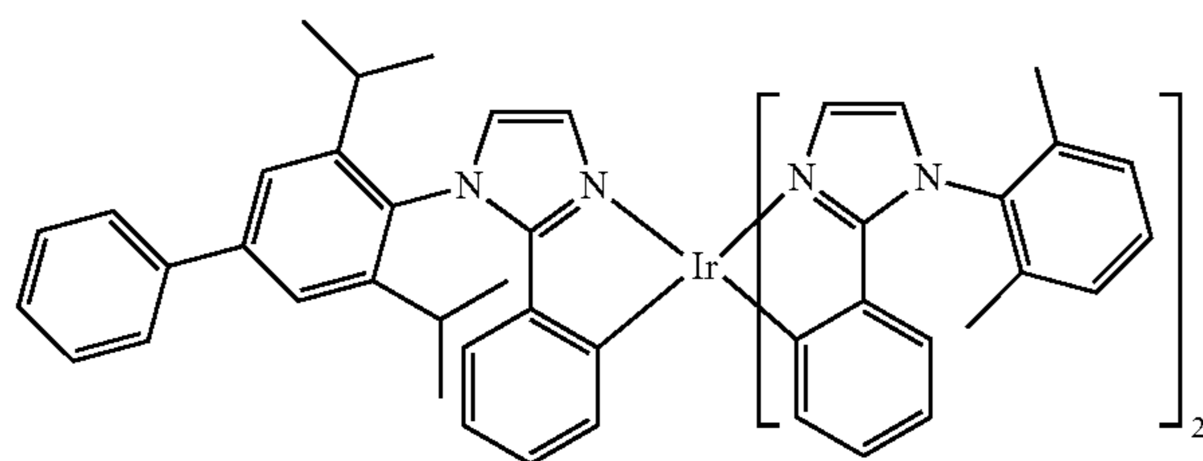
Compound 61
