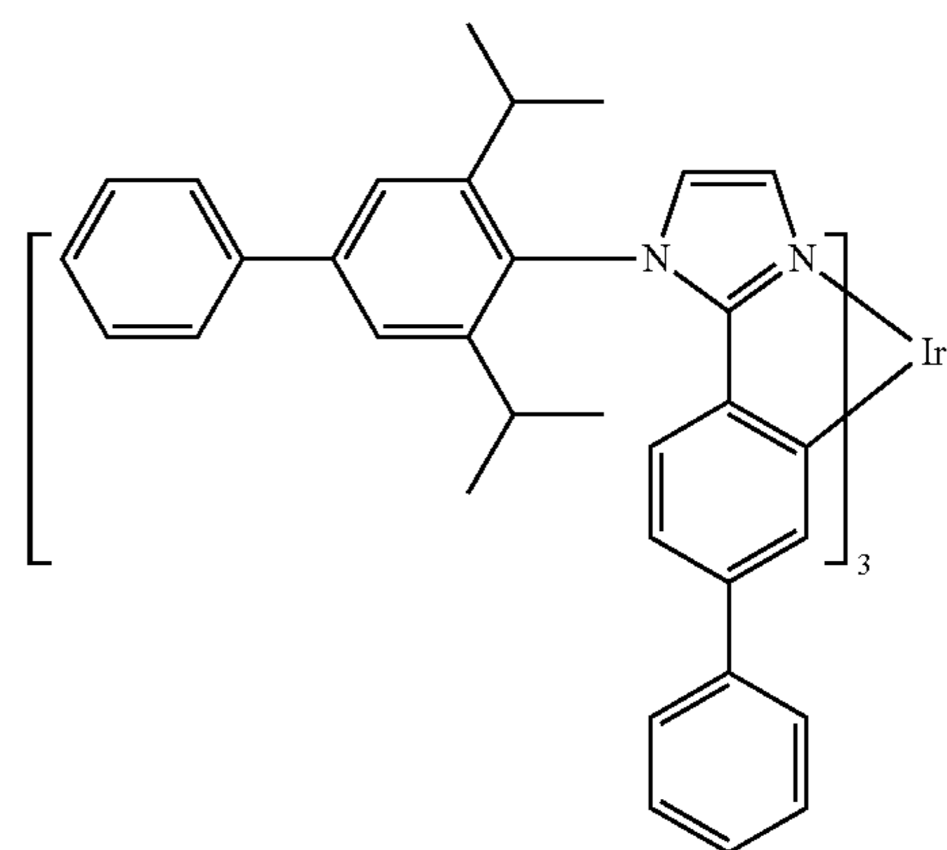
Compound 24
