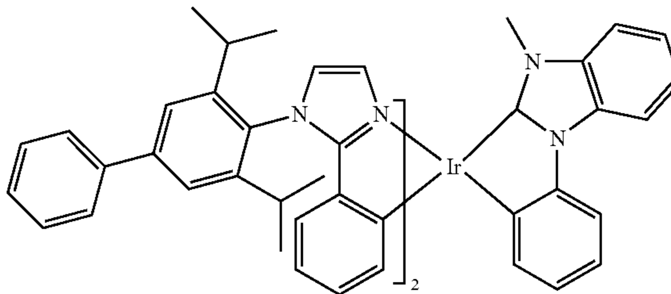
Compound 55
