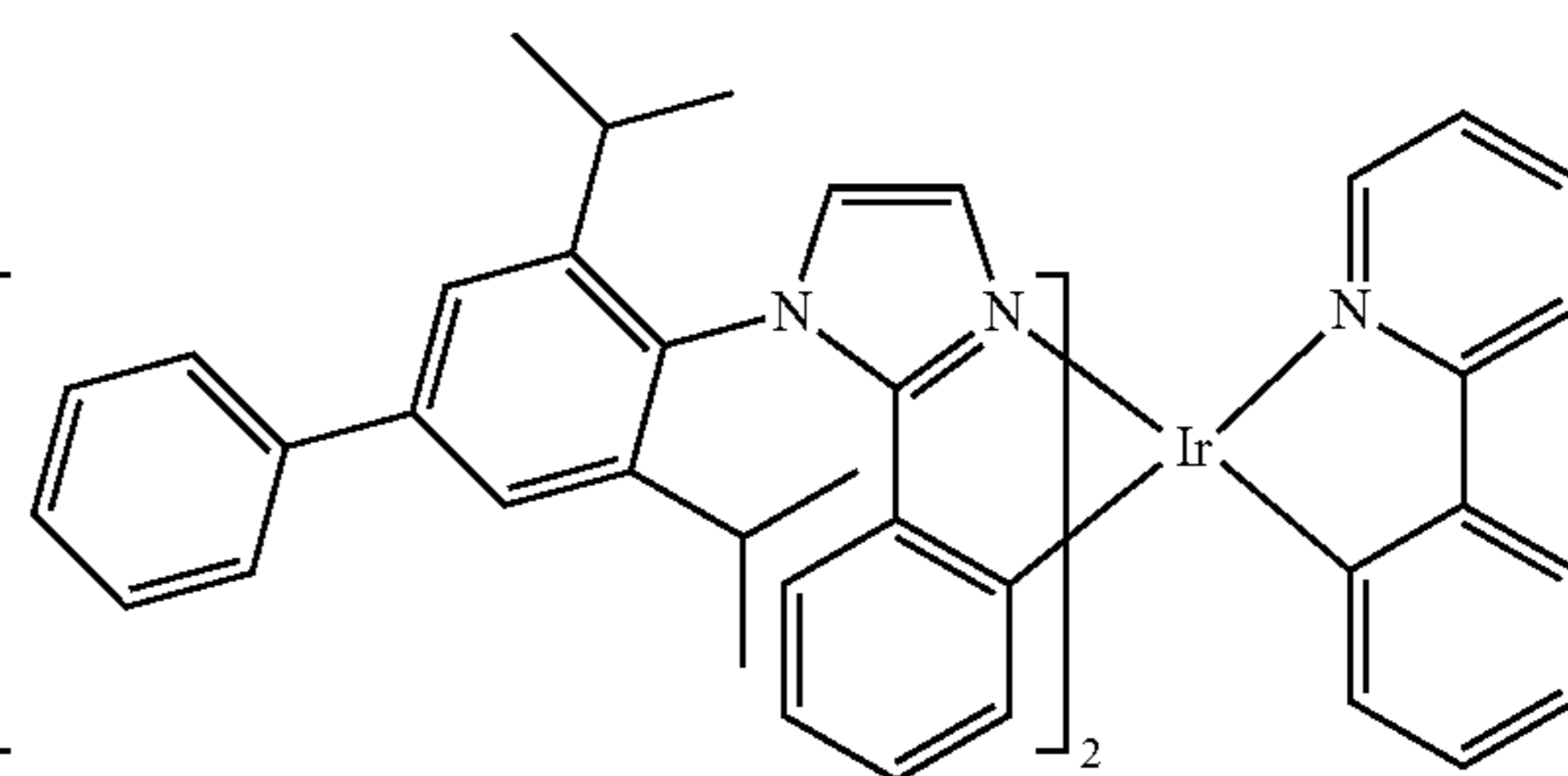
Compound 48
