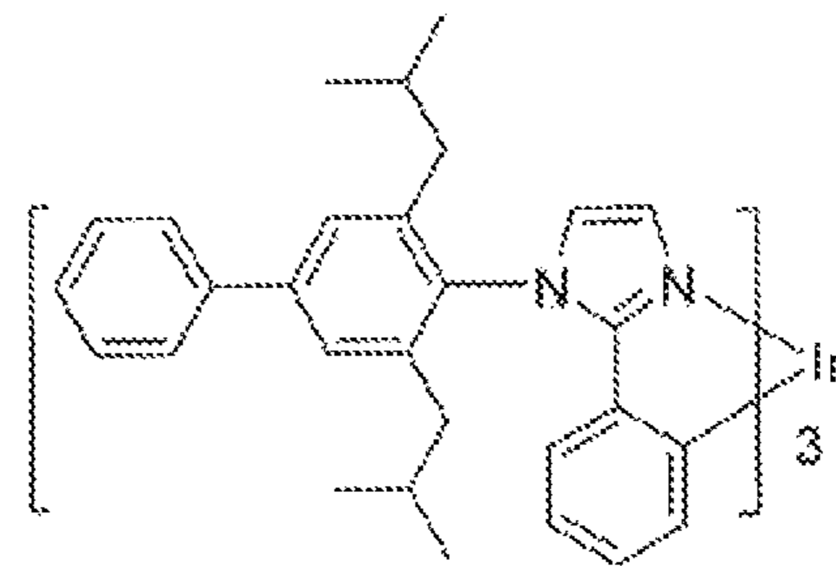
Compound 5
