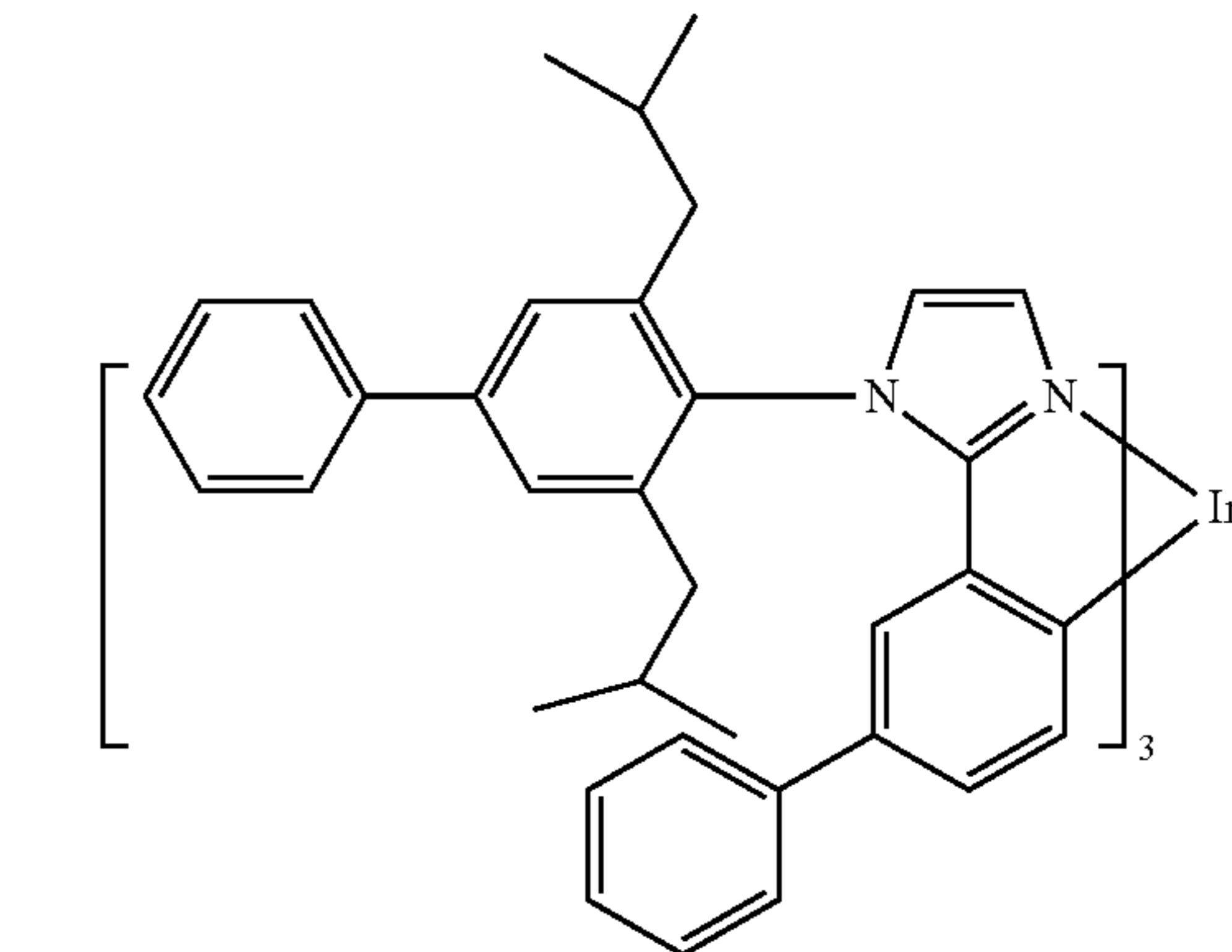
Compound 17
