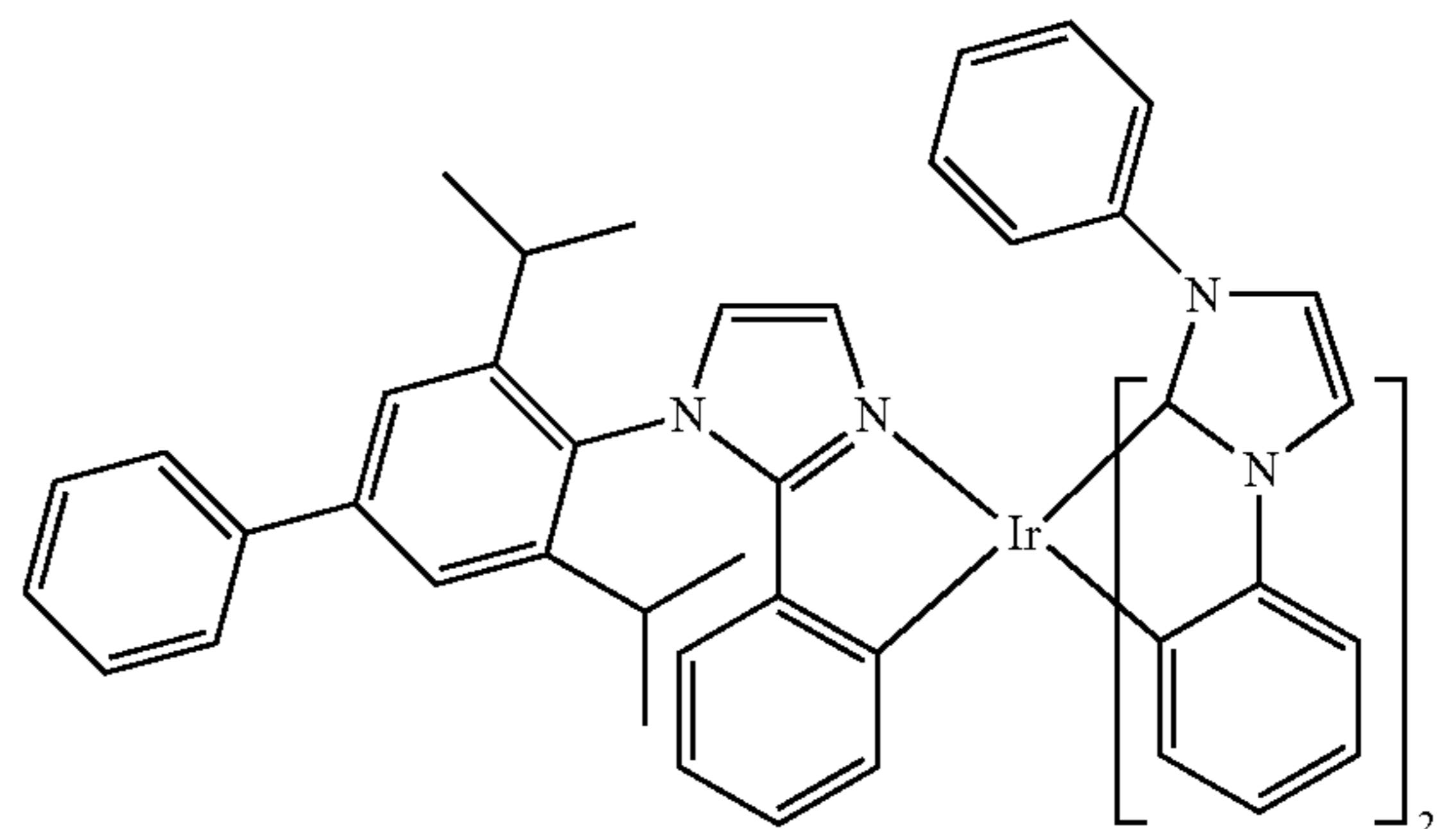
Compound 66
