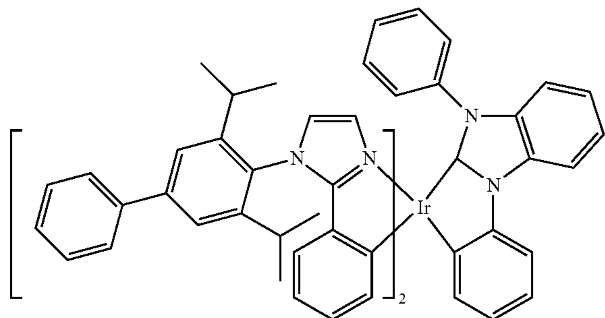
Compound 56
