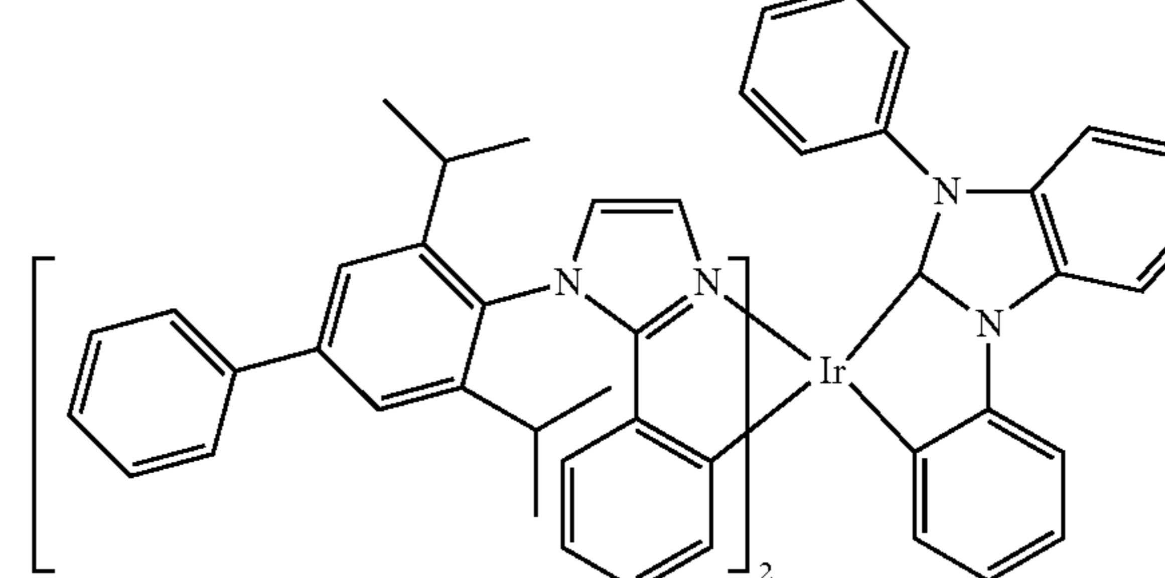
Compound 56
