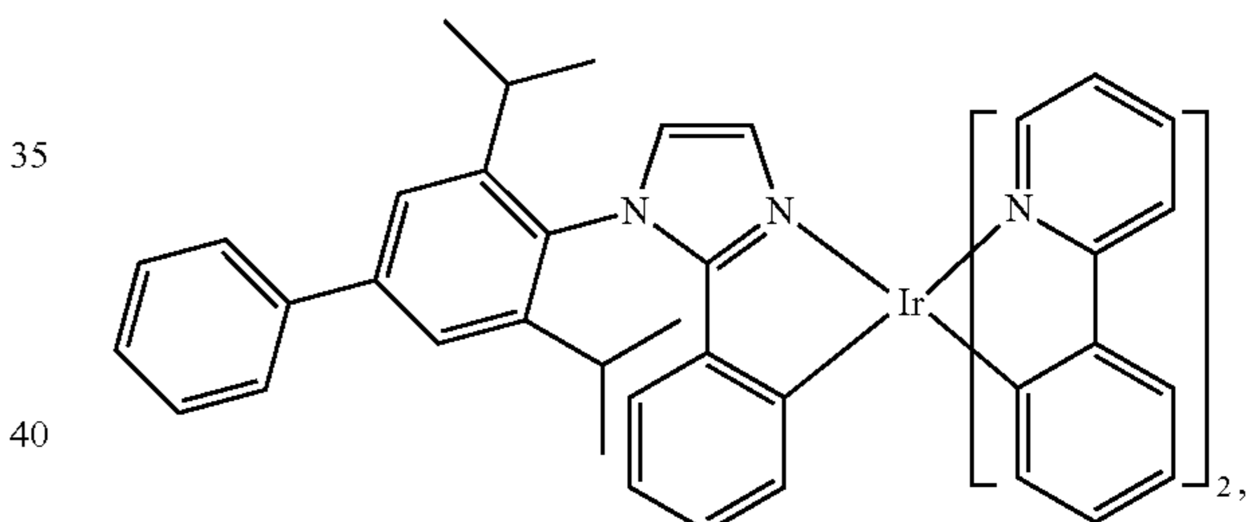
Compound 59
