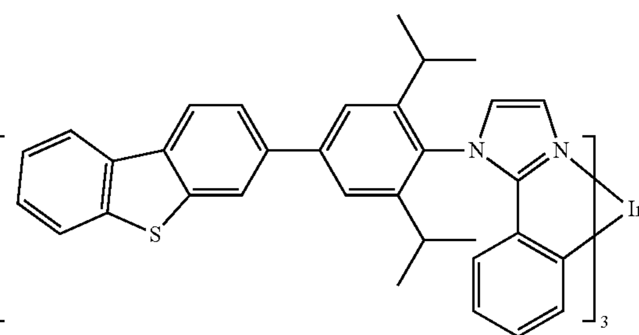
Compound 32
