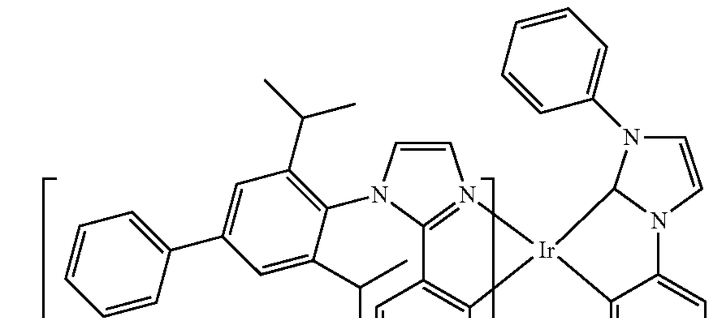
Compound 54
