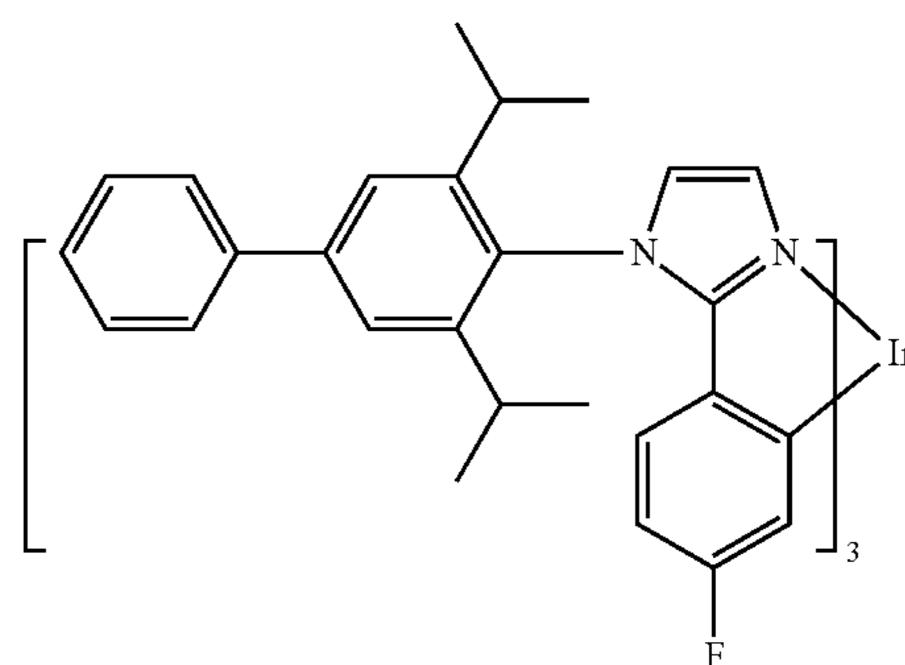
Compound 28
