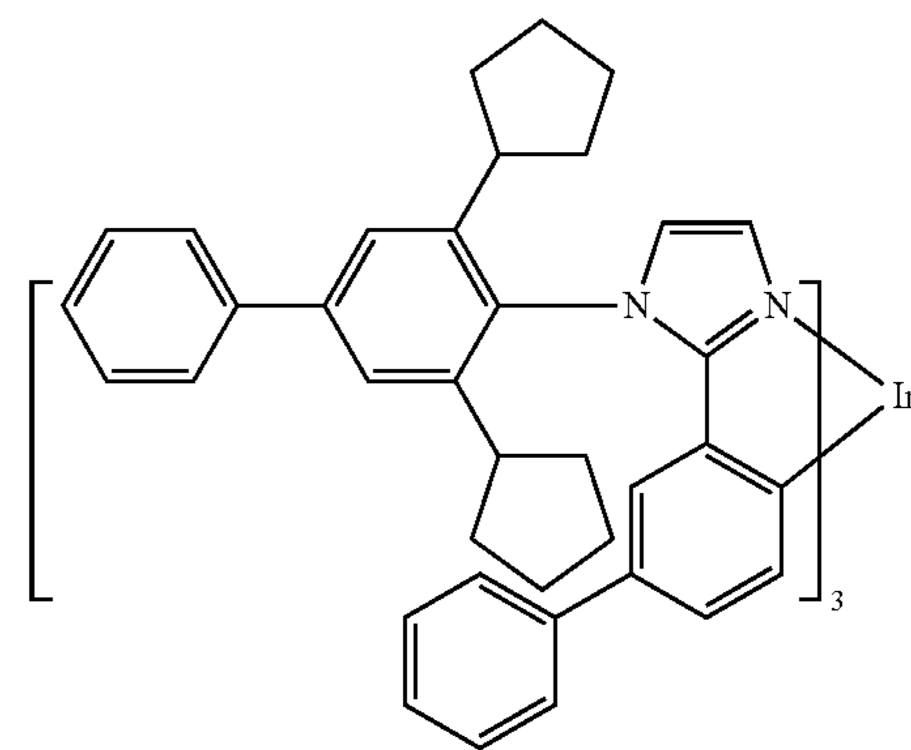
Compound 16
