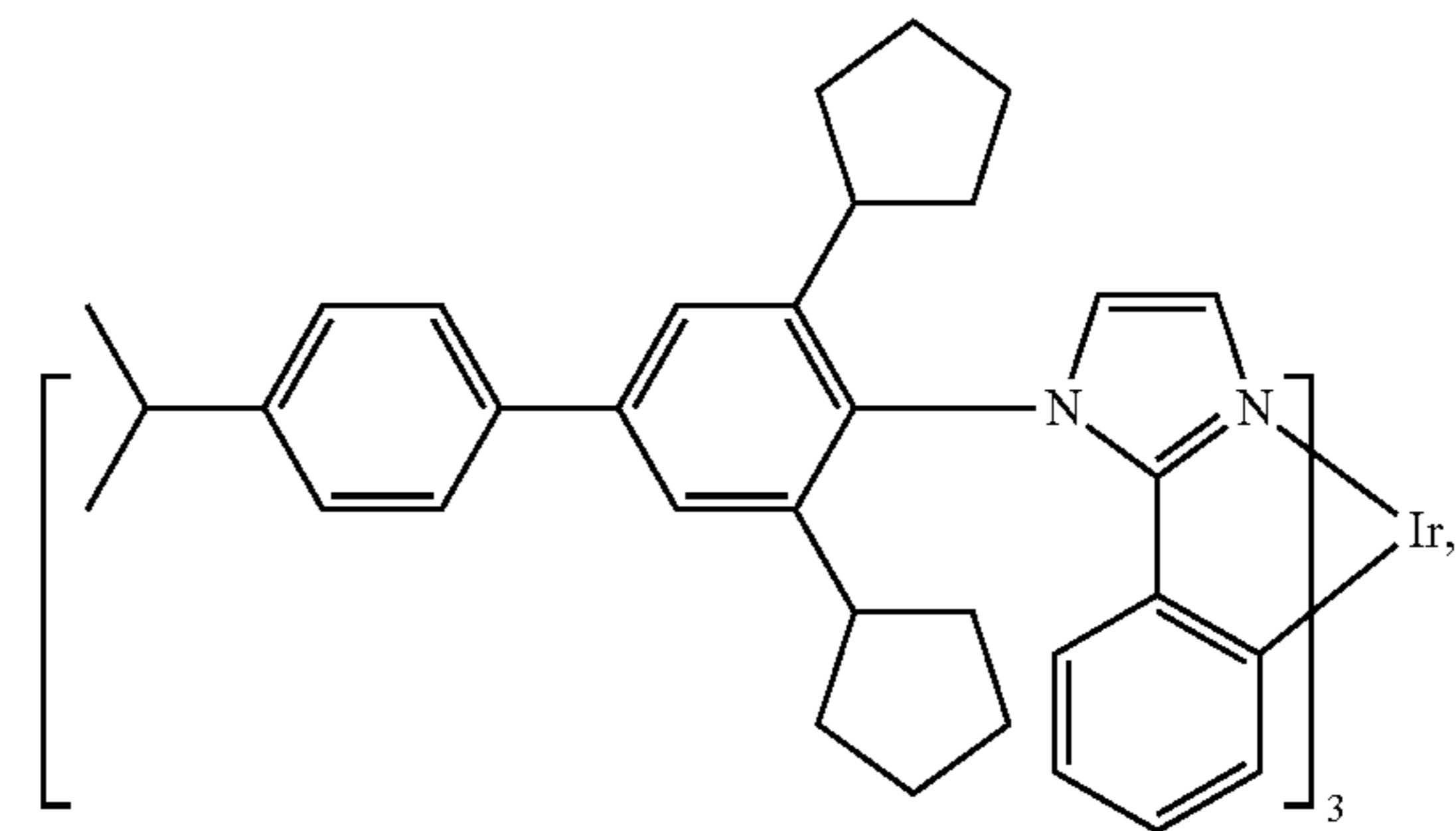
Compound 11
