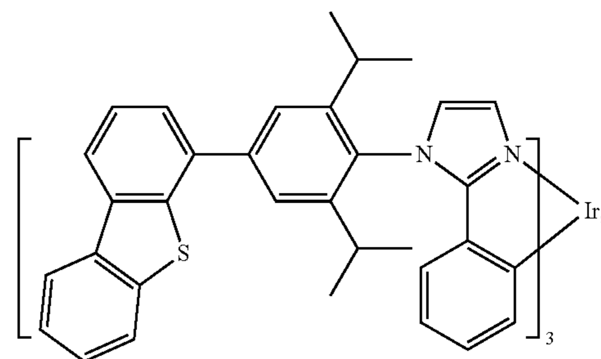
Compound 33
