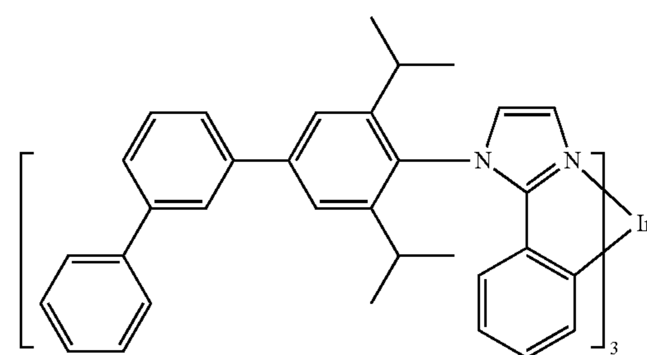
Compound 30
