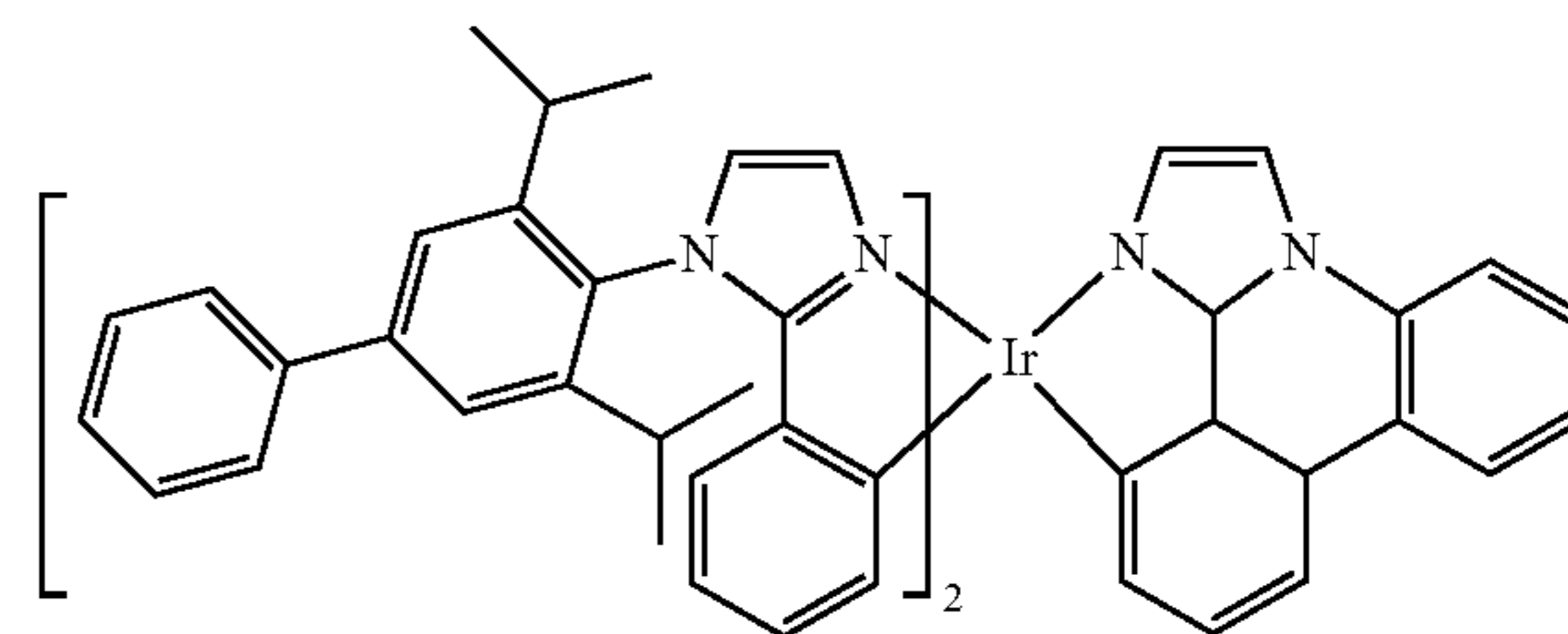
Compound 57
