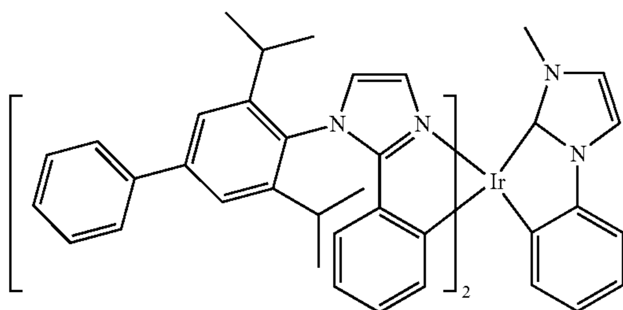
Compound 53
