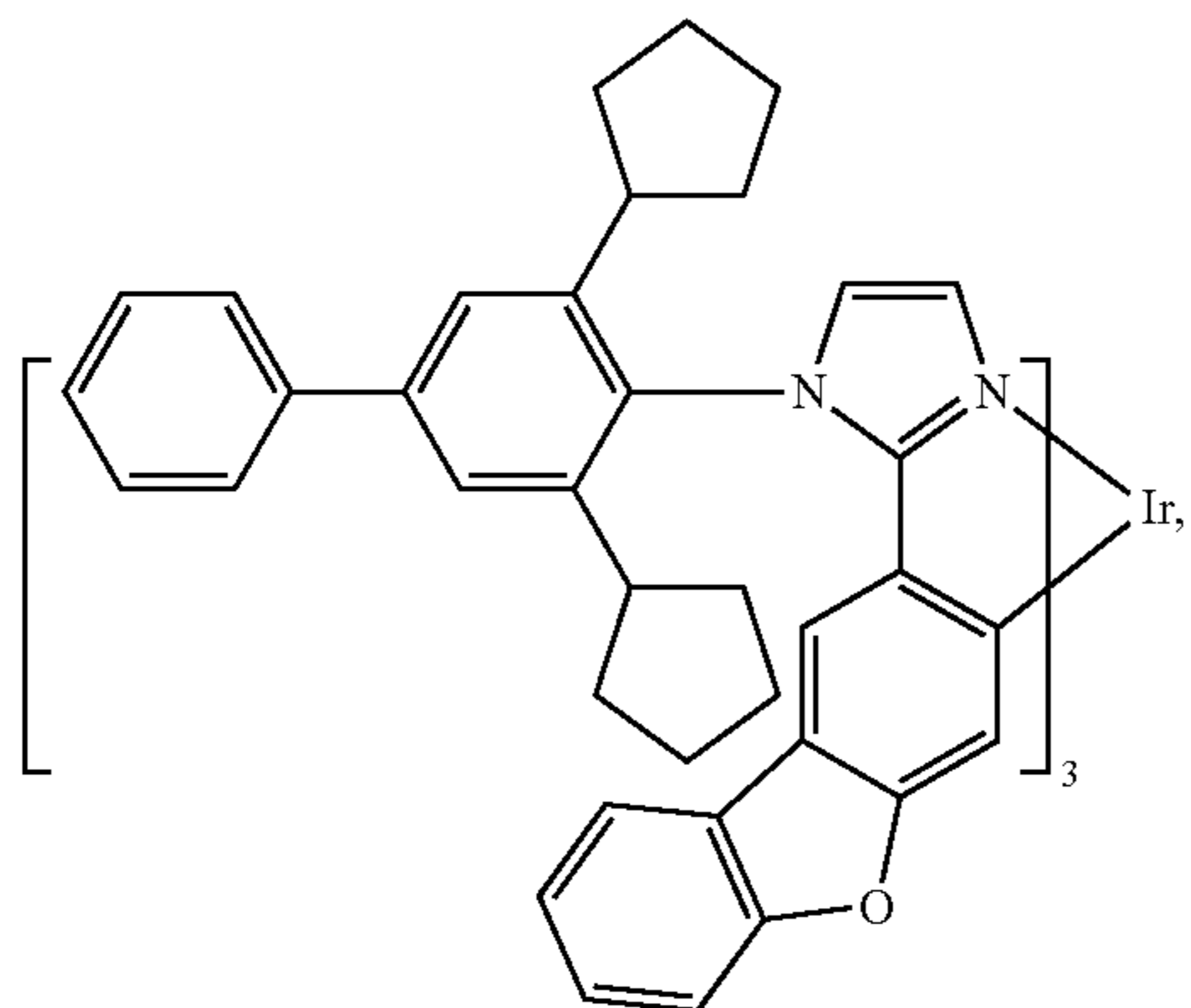
Compound 19
