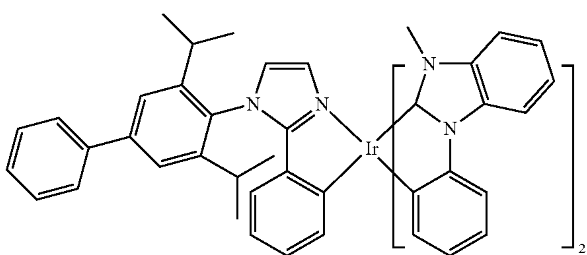
Compound 66
