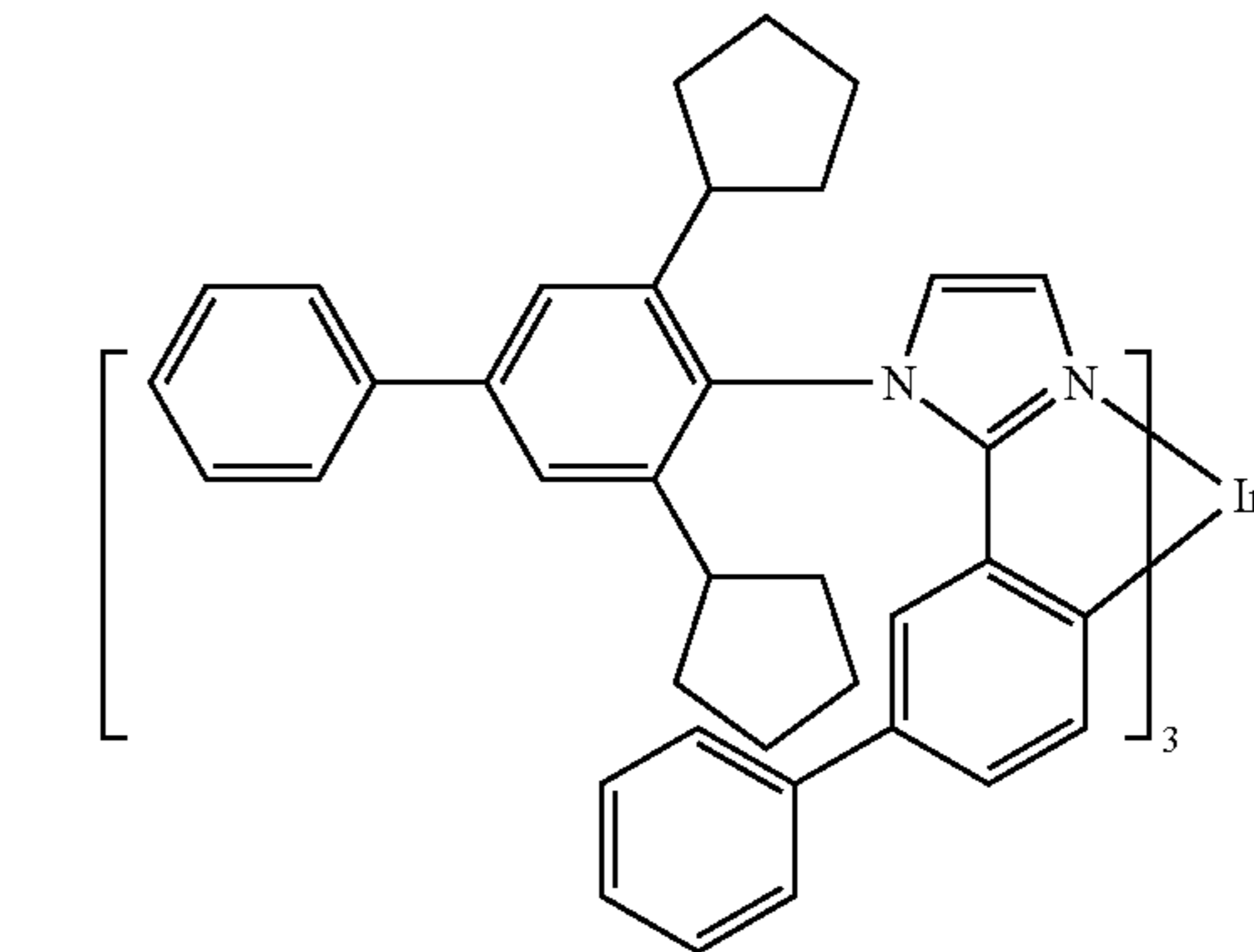
Compound 16
