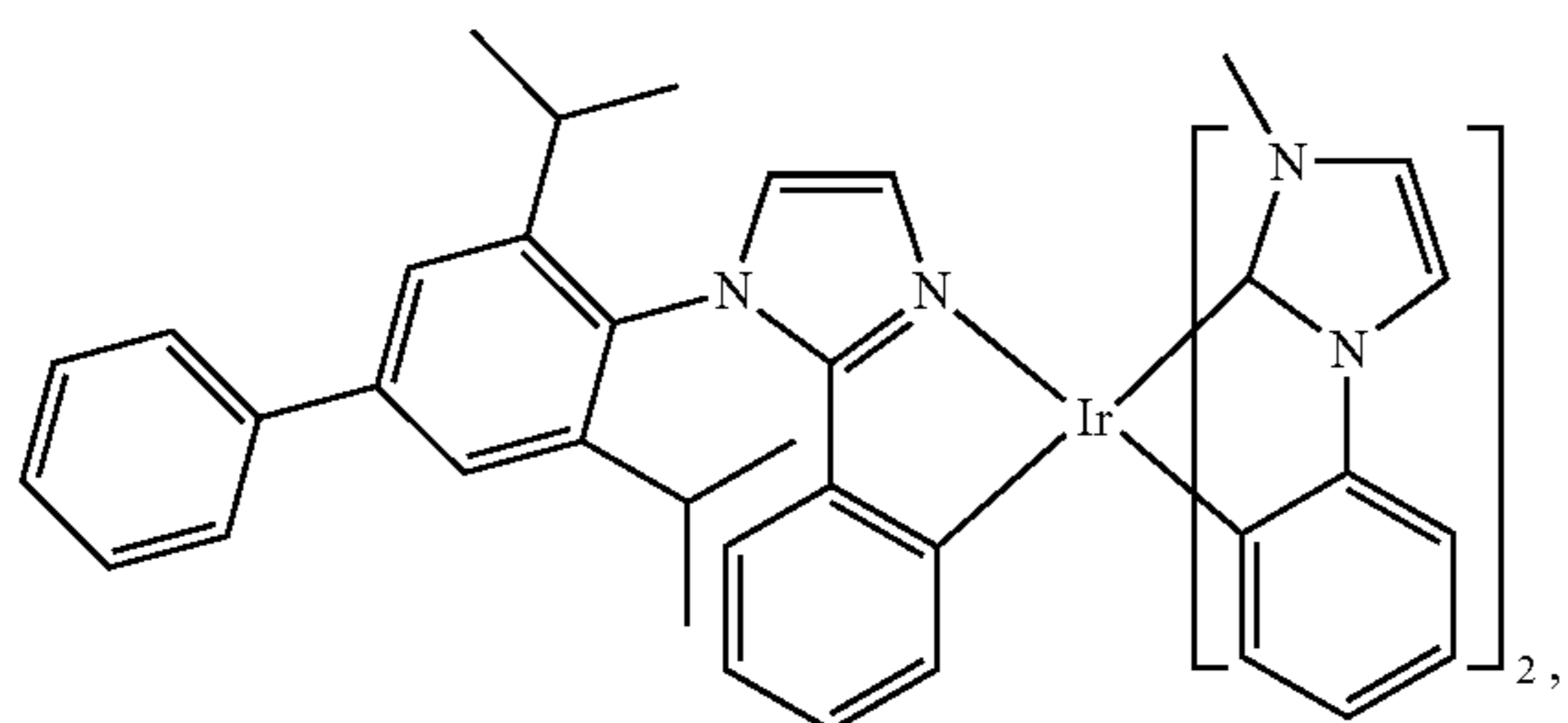
Compound 64
