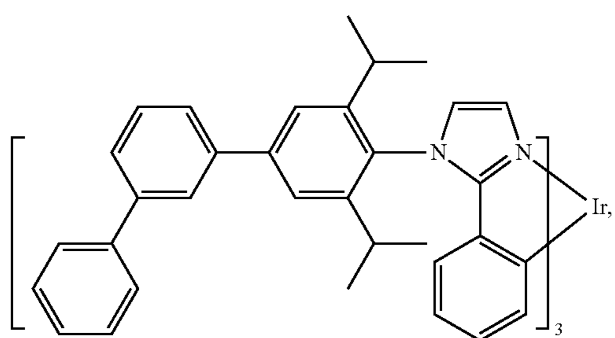
Compound 29
