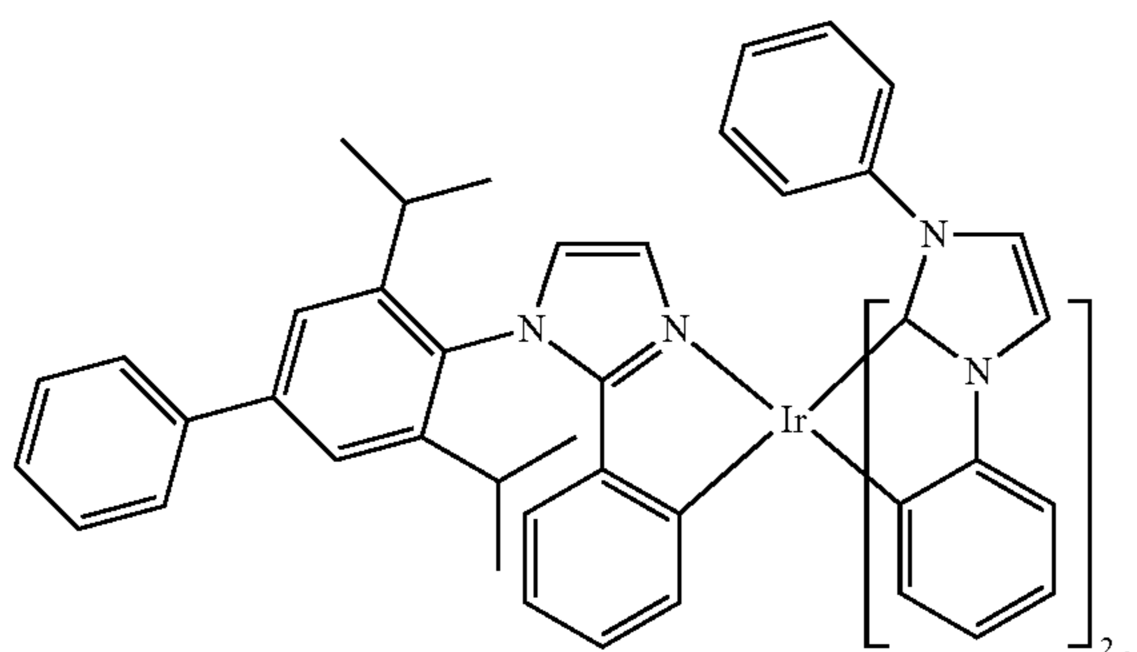
Compound 66
