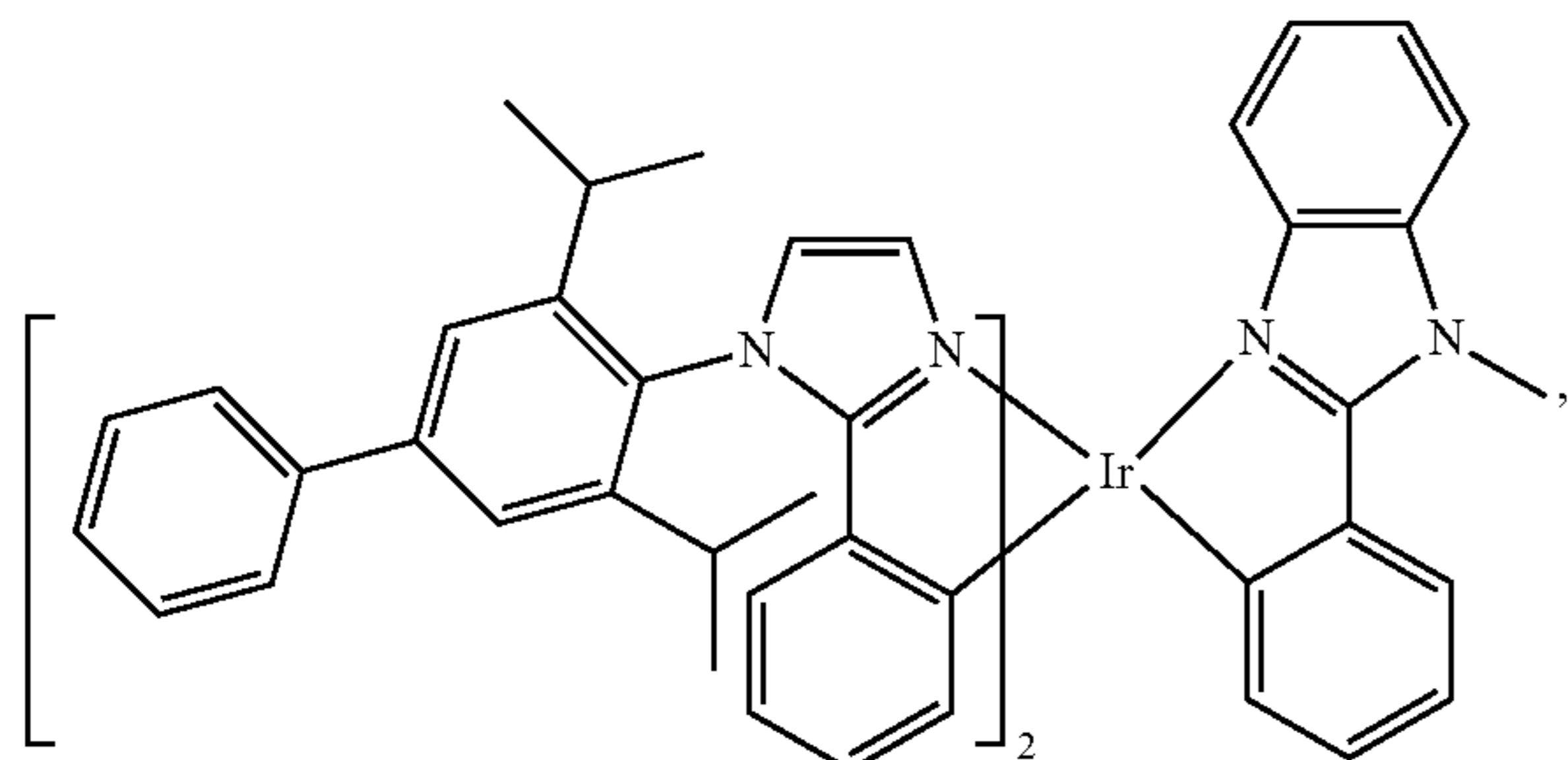
Compound 51
