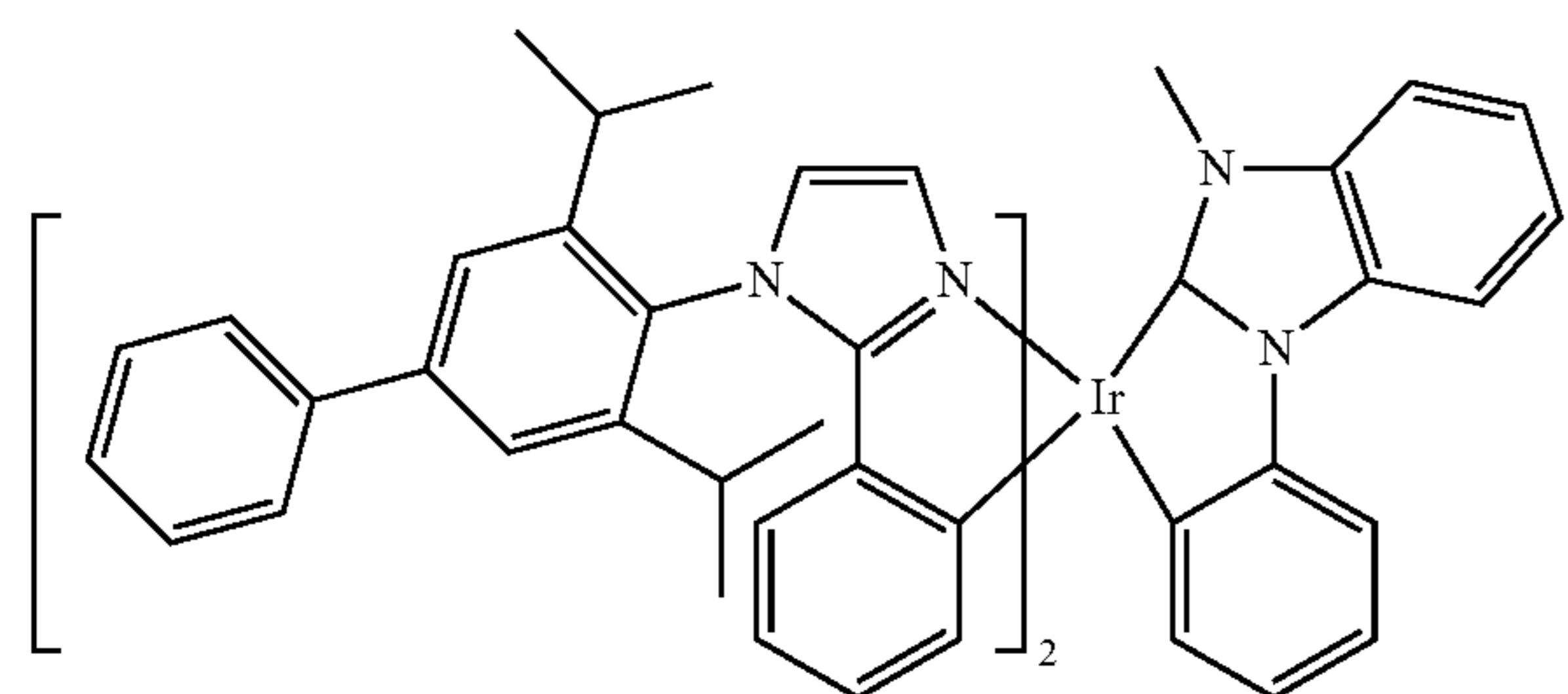
Compound 56
