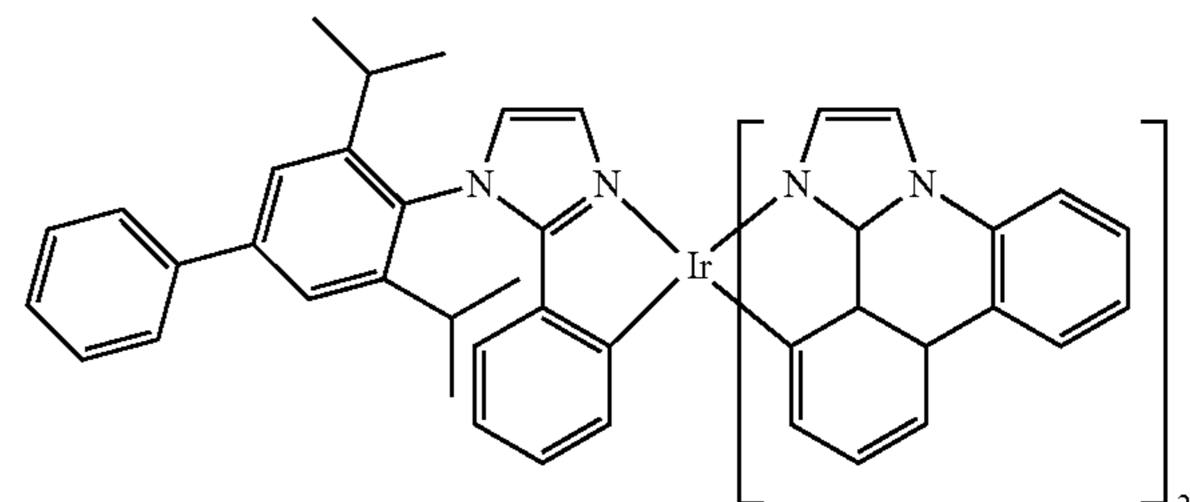
Compound 69
