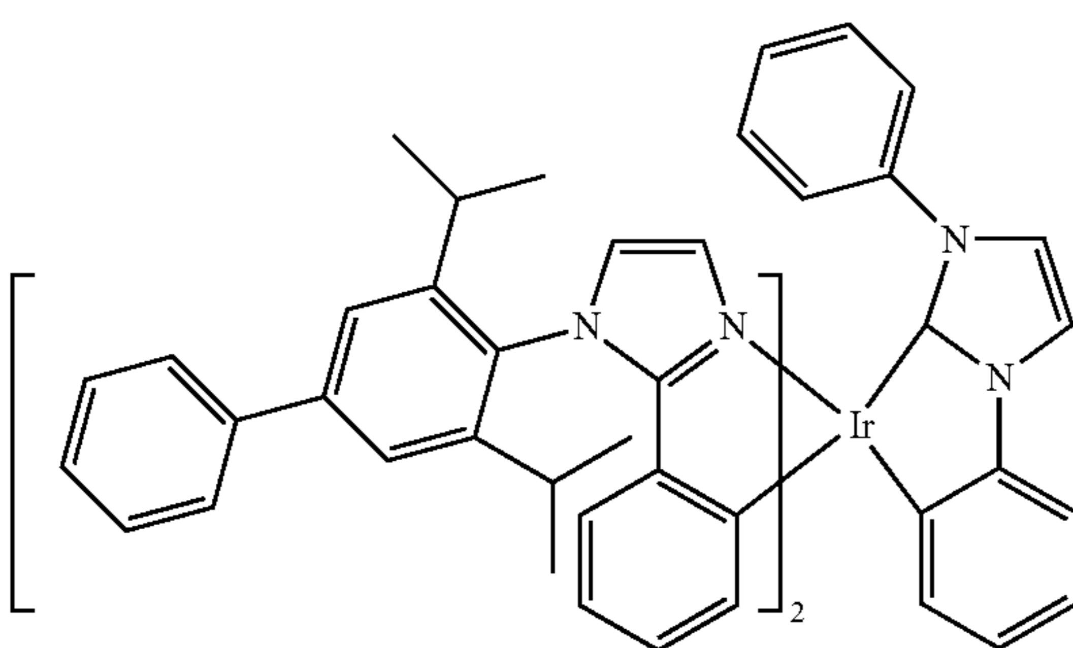
Compound 55
