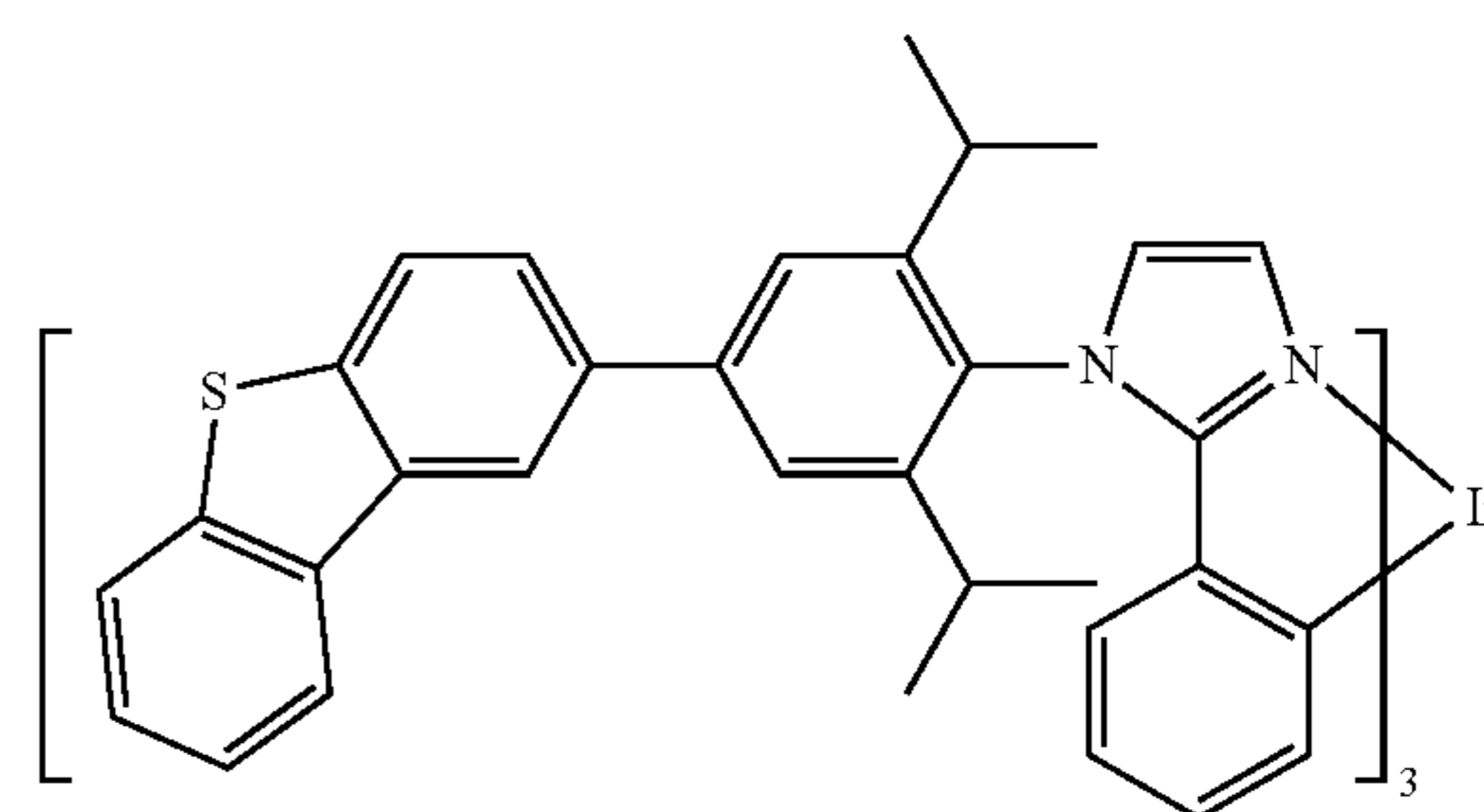
Compound 32
