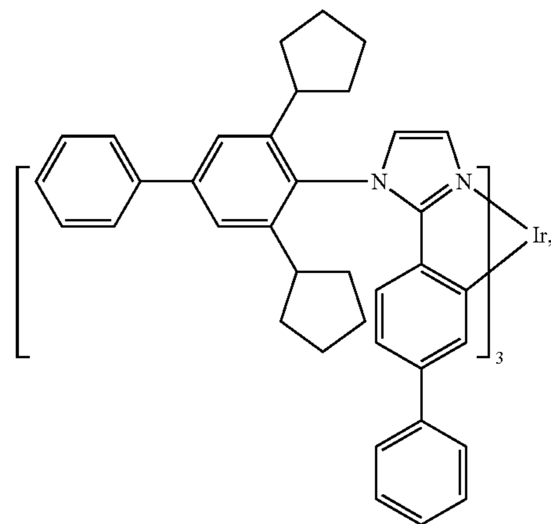
Compound 21
