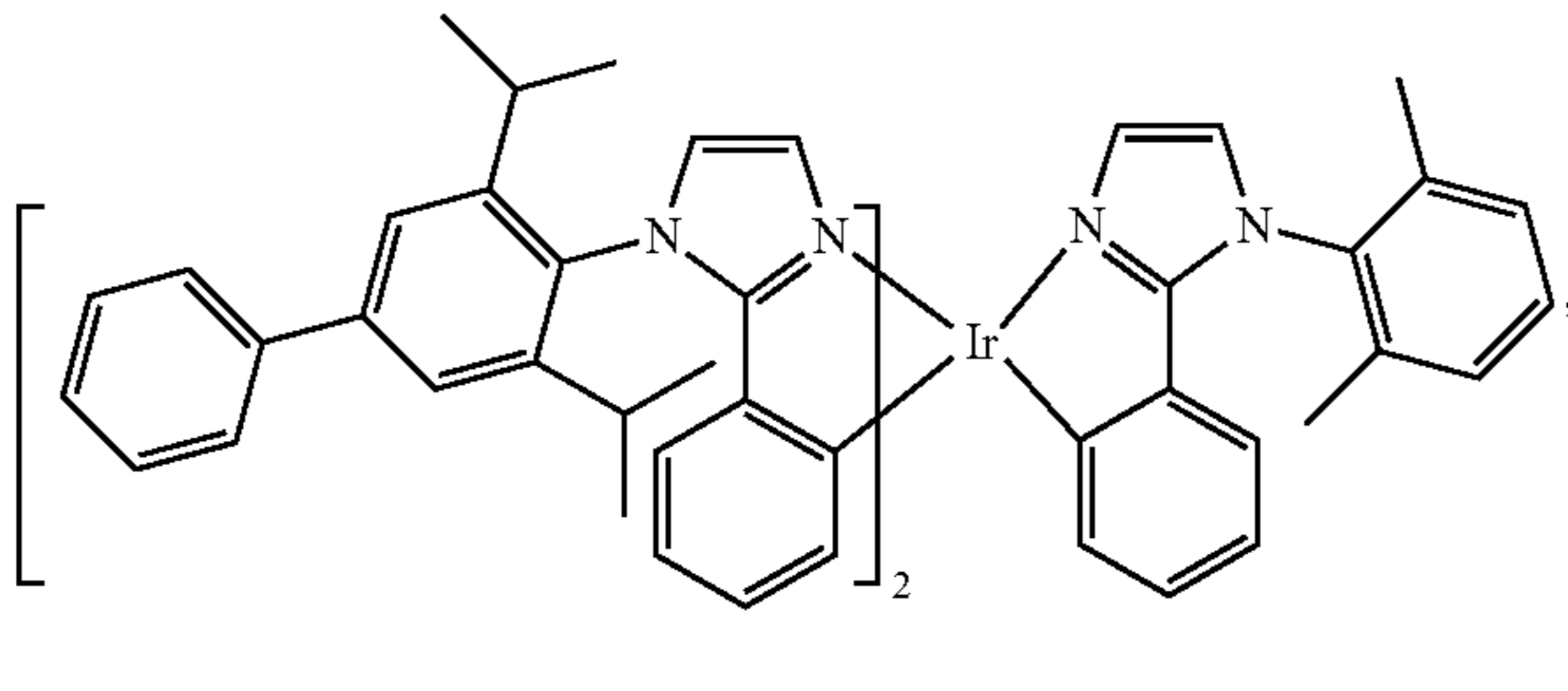
Compound 50
