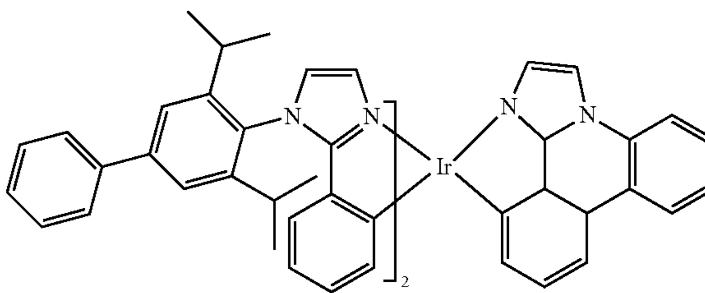
Compound 58
