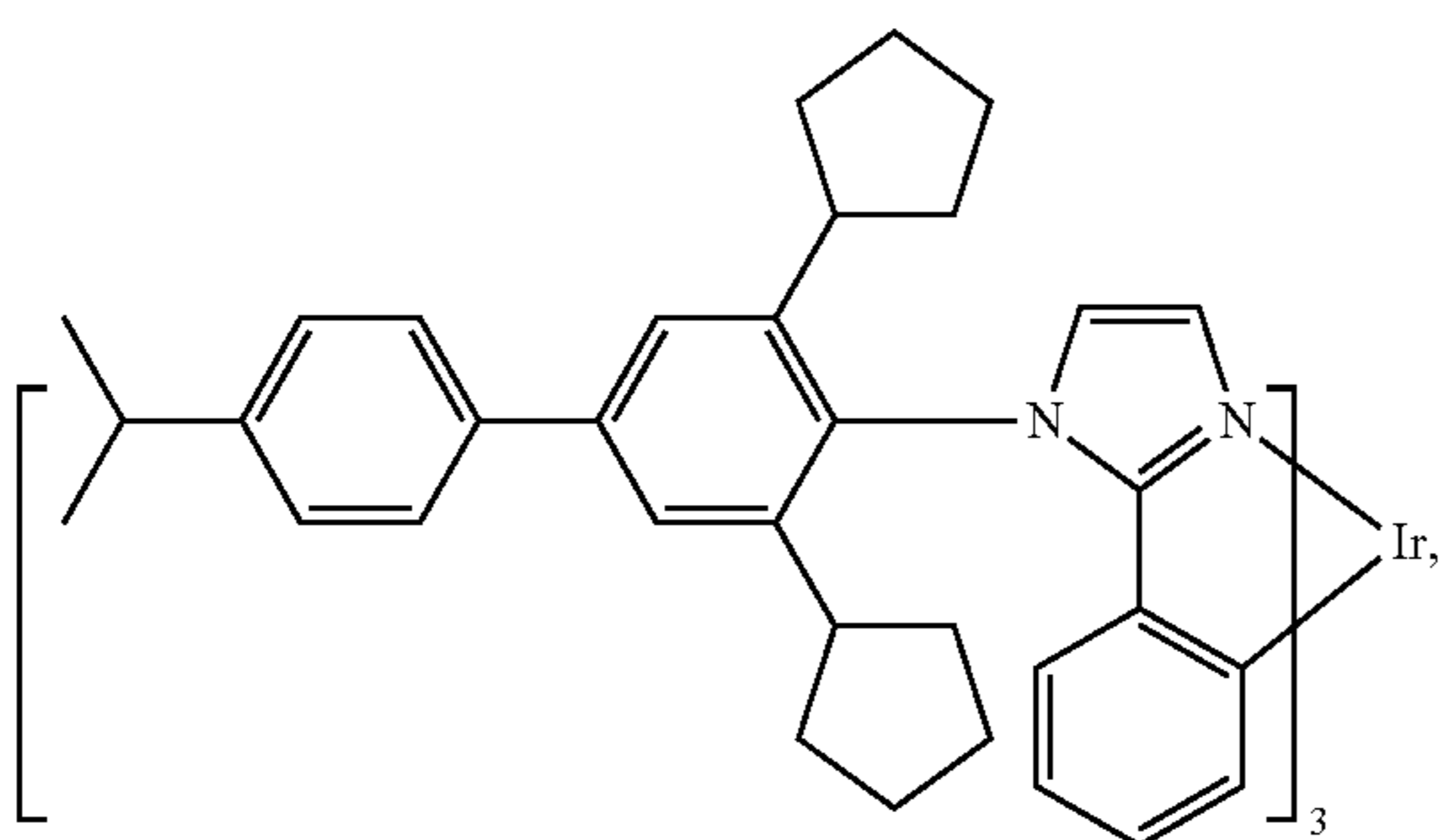
Compound 10
