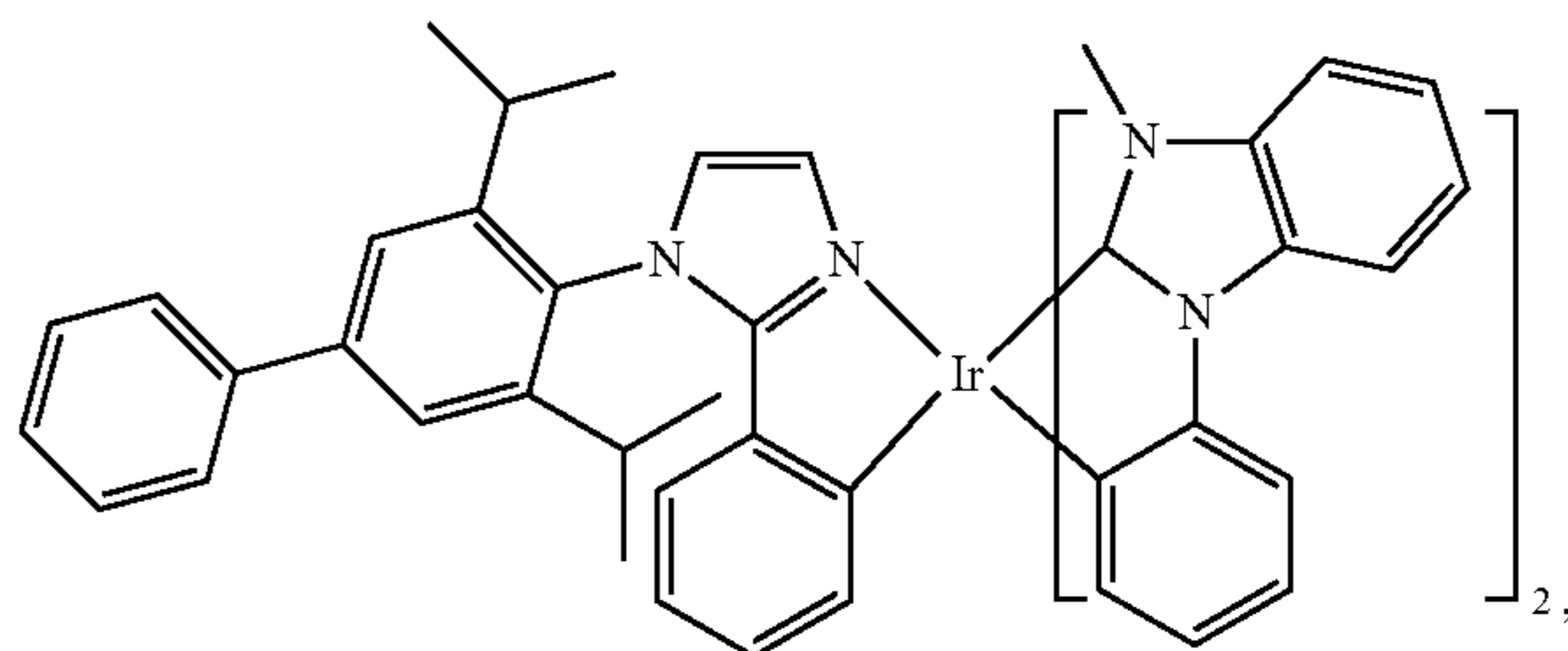
Compound 66
