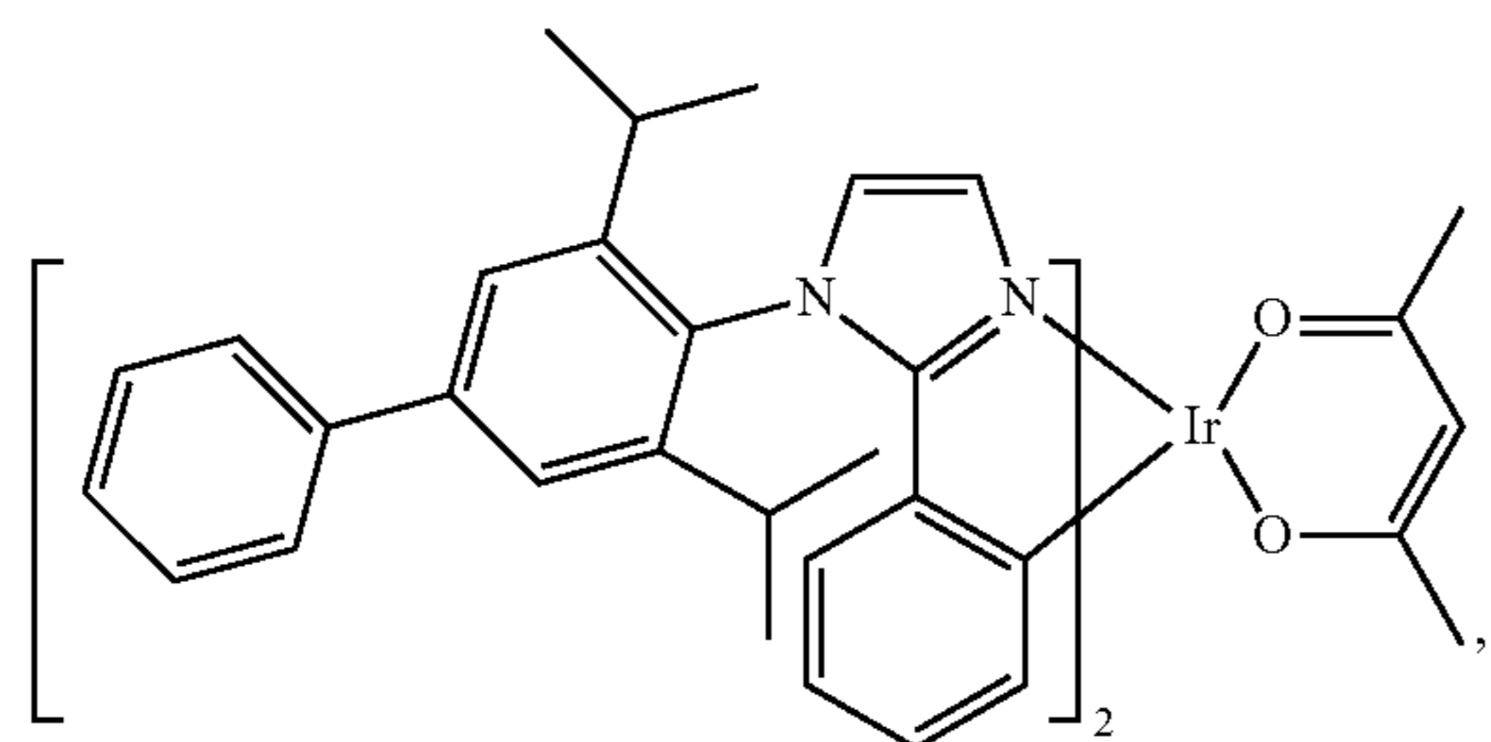
Compound 48
