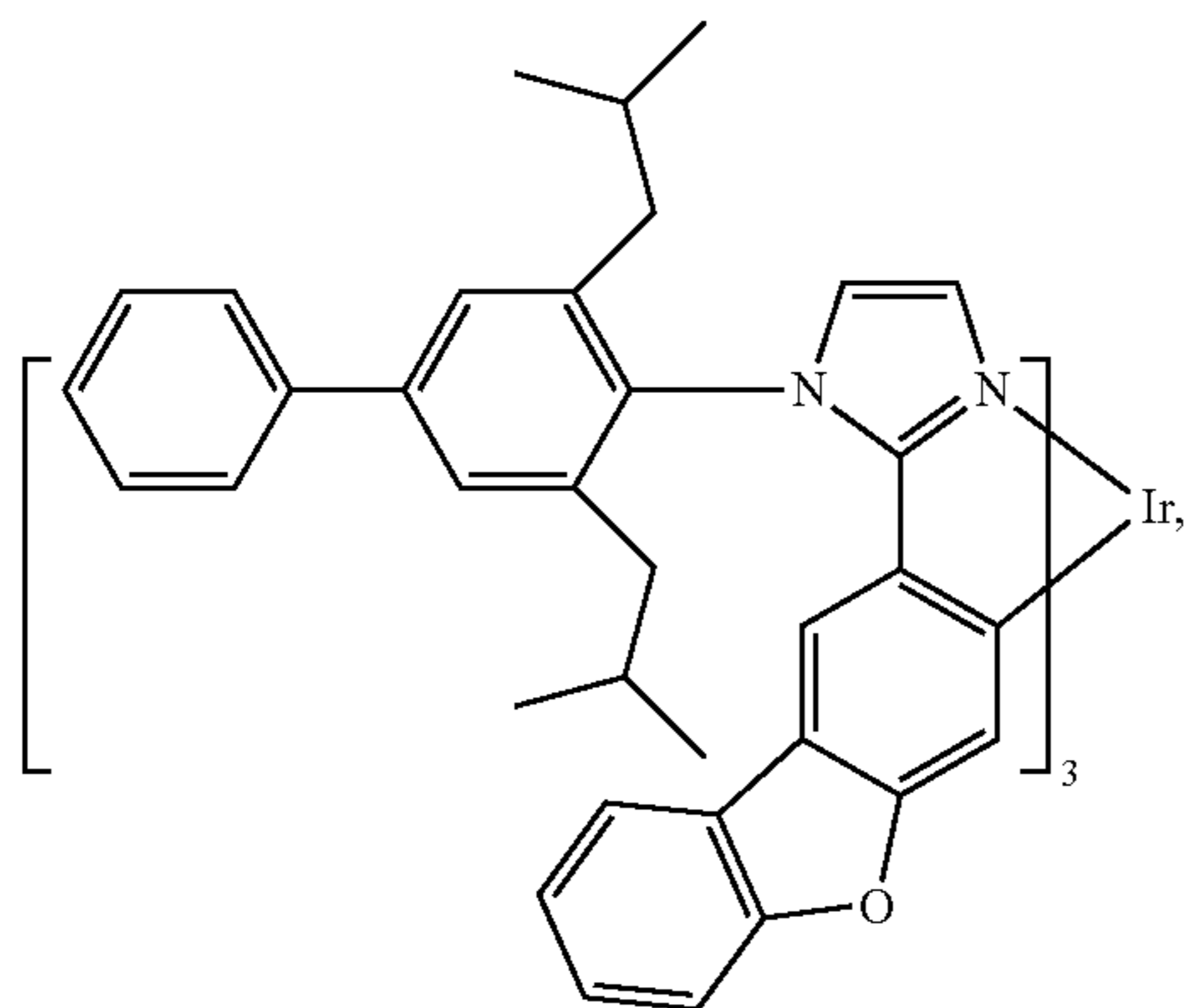
Compound 20
