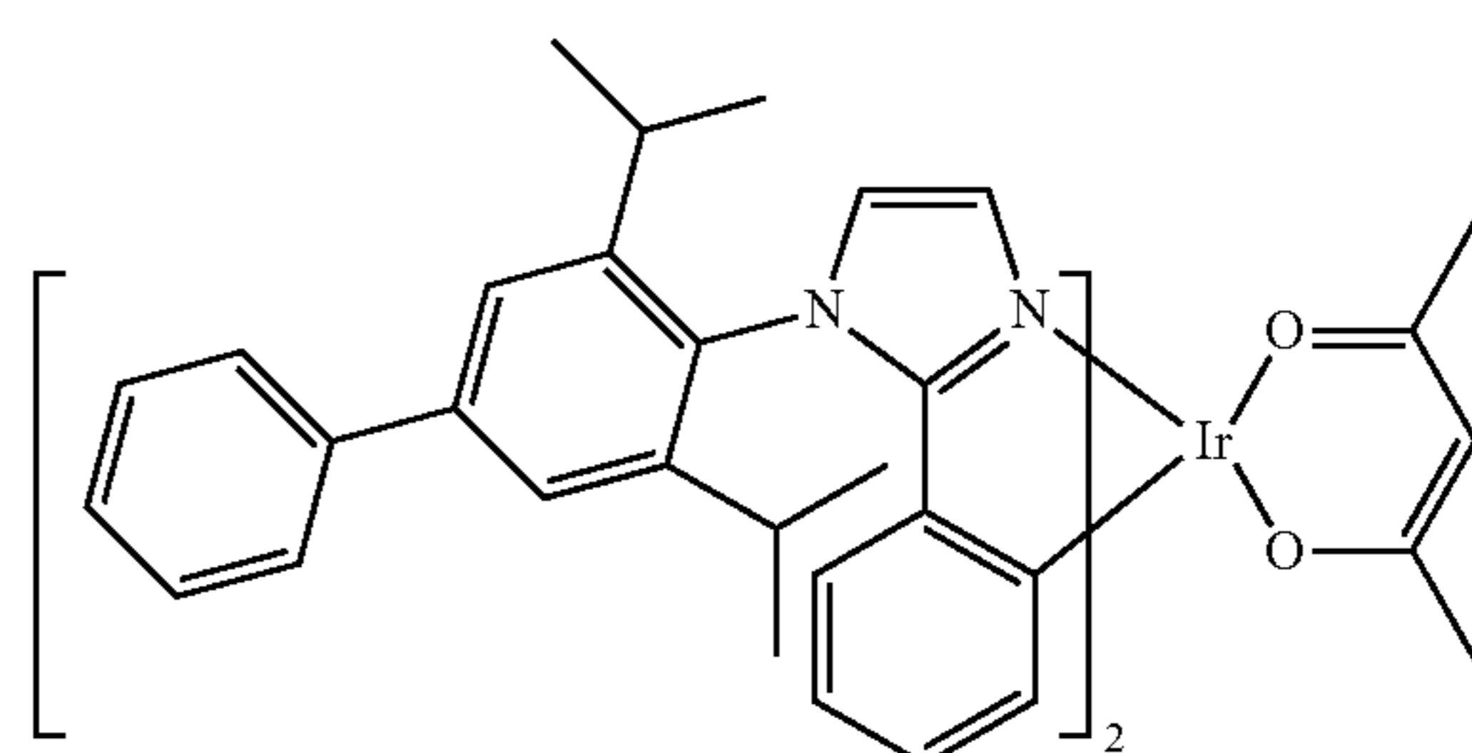
Compound 48
