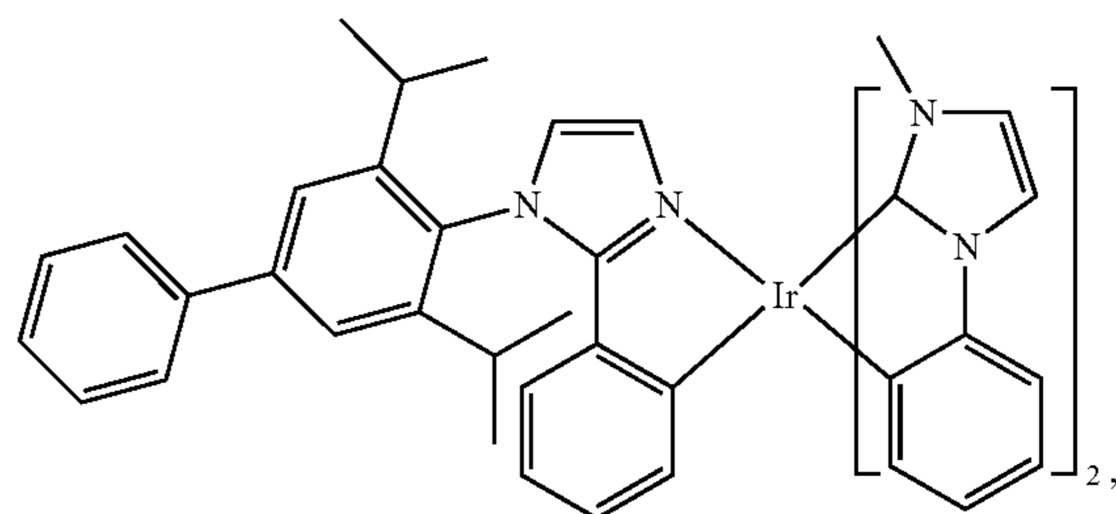
Compound 65
