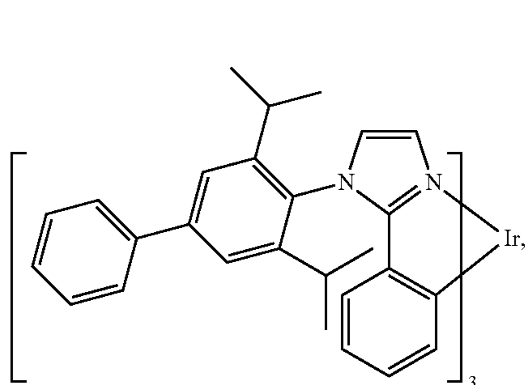
Compound 1
