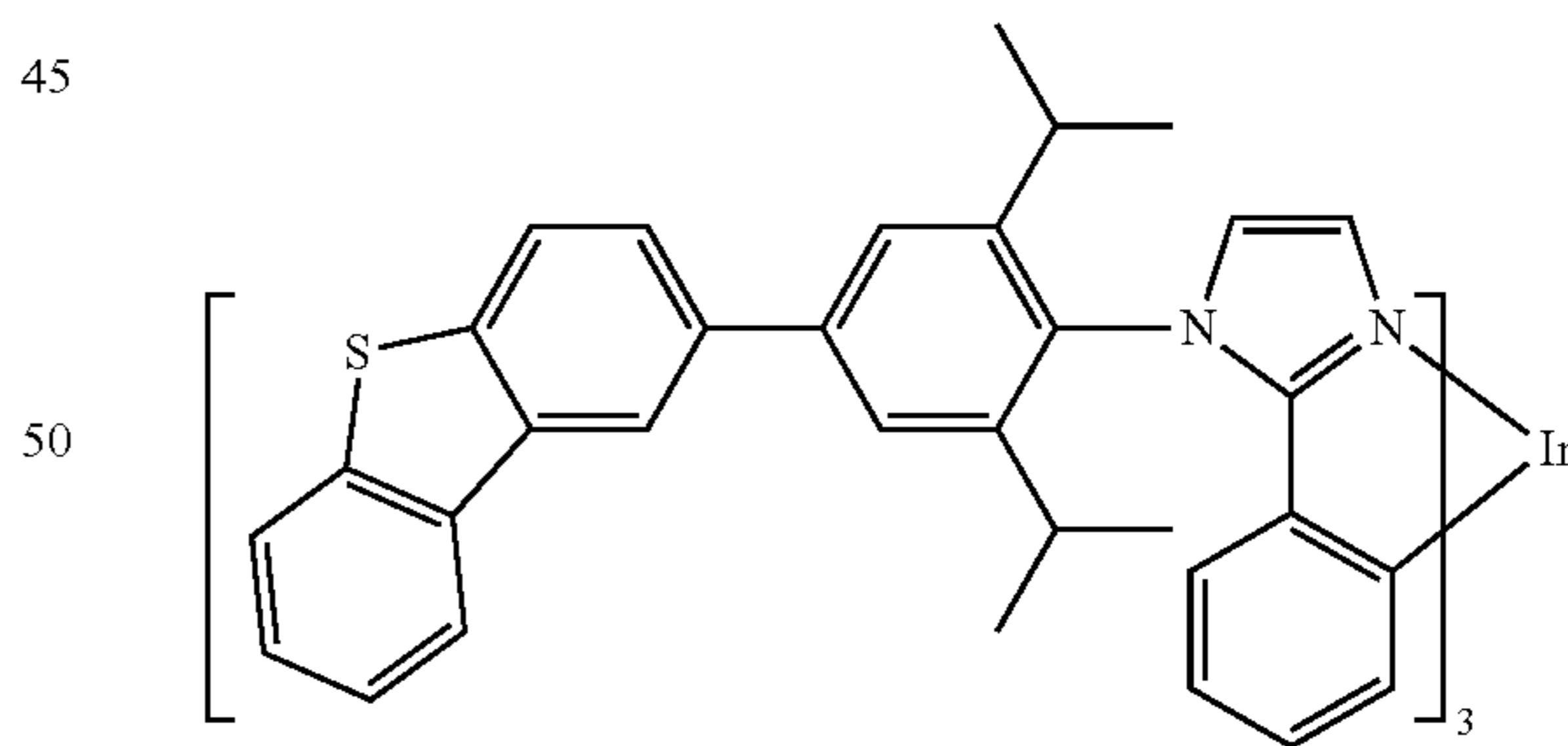
Compound 32
