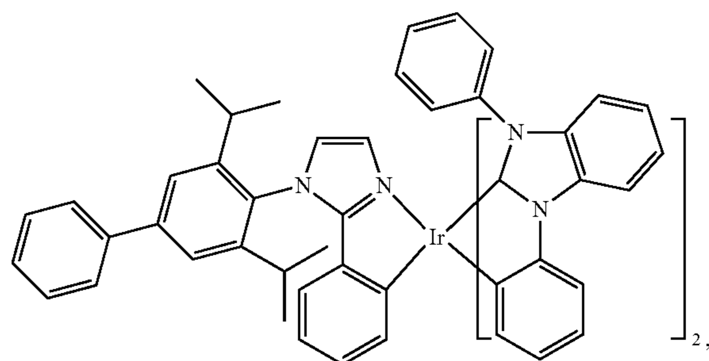
Compound 67
