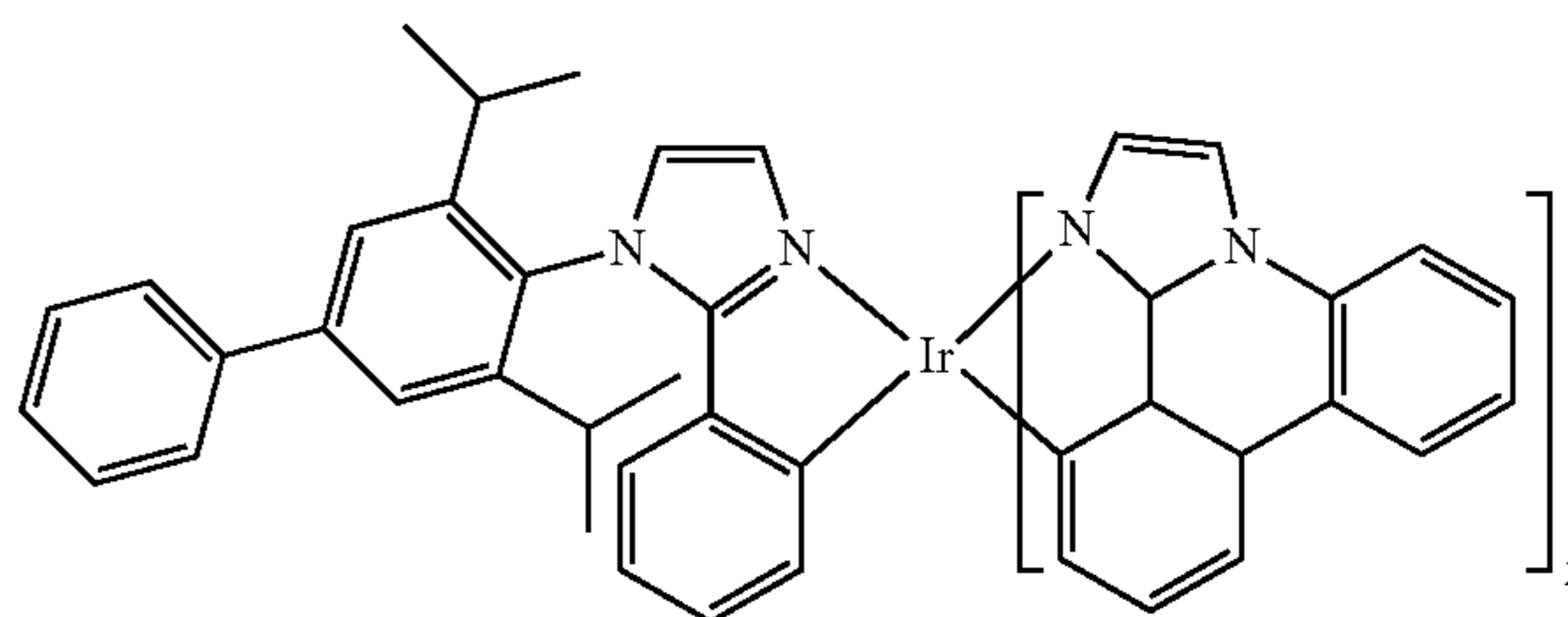
Compound 68
