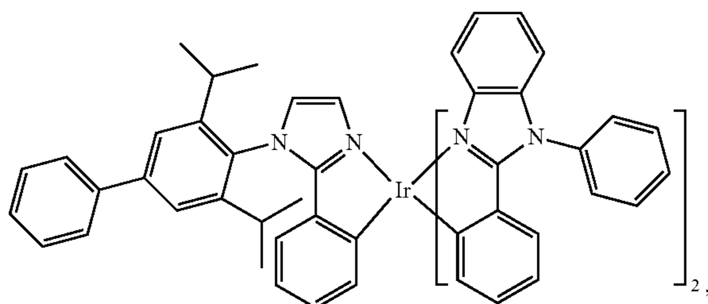
Compound 63
