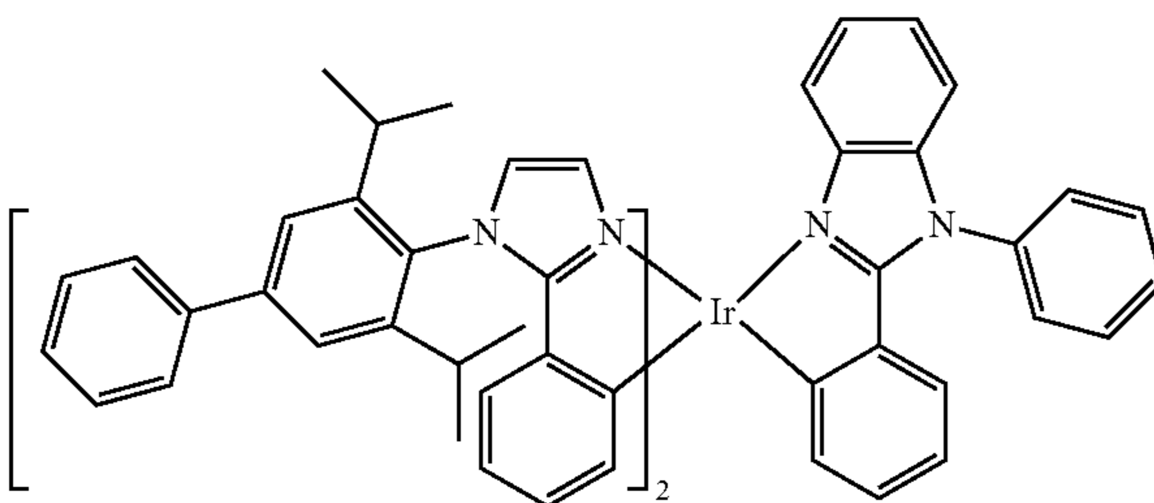
Compound 52
