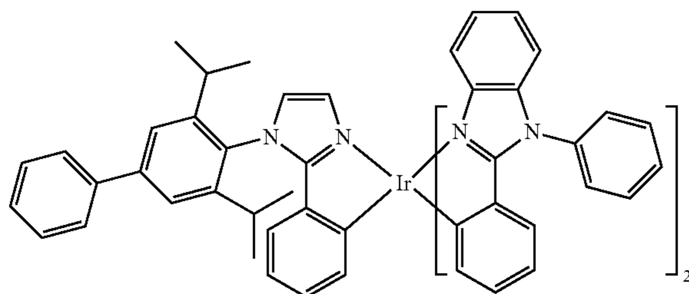
Compound 63
