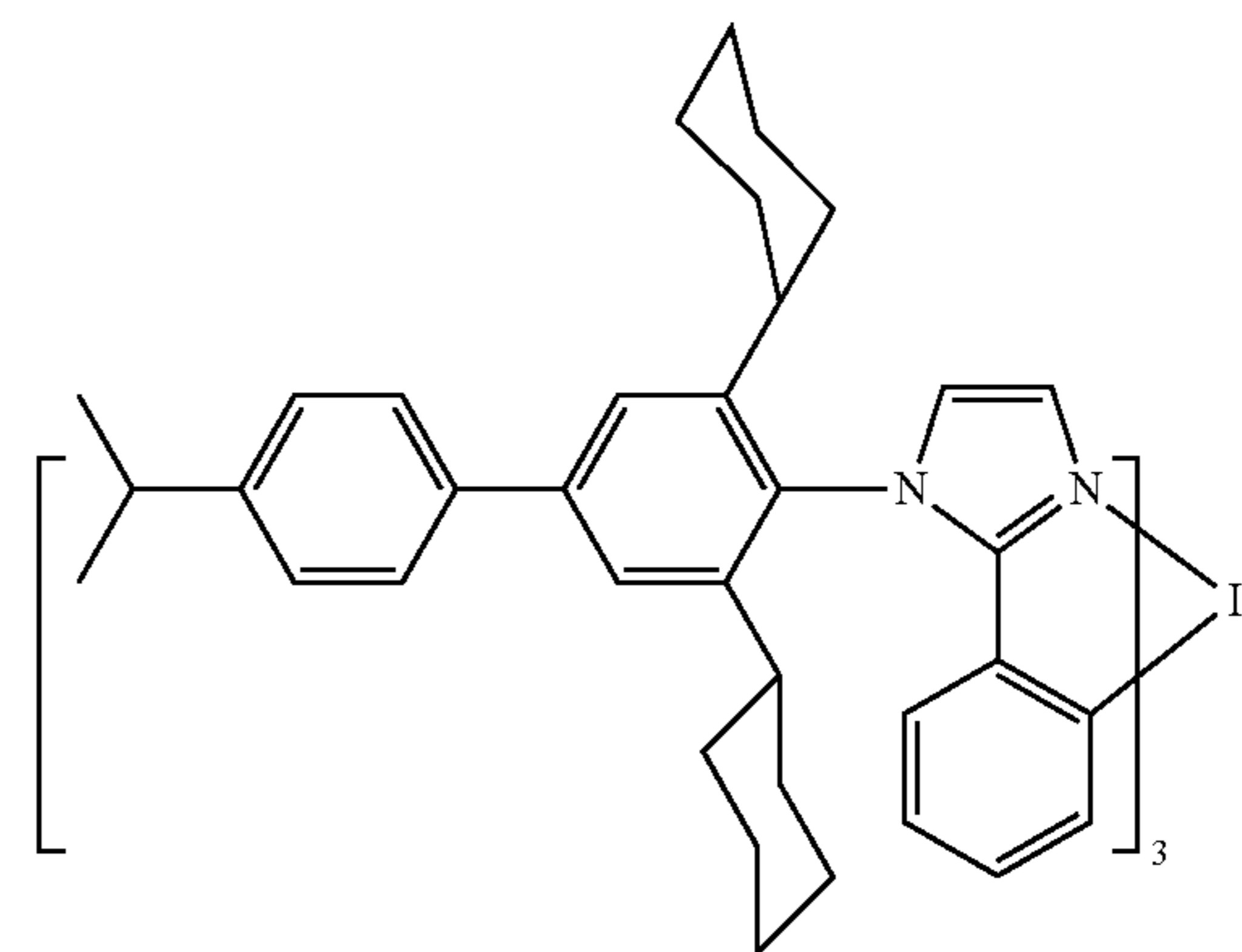
Compound 14
