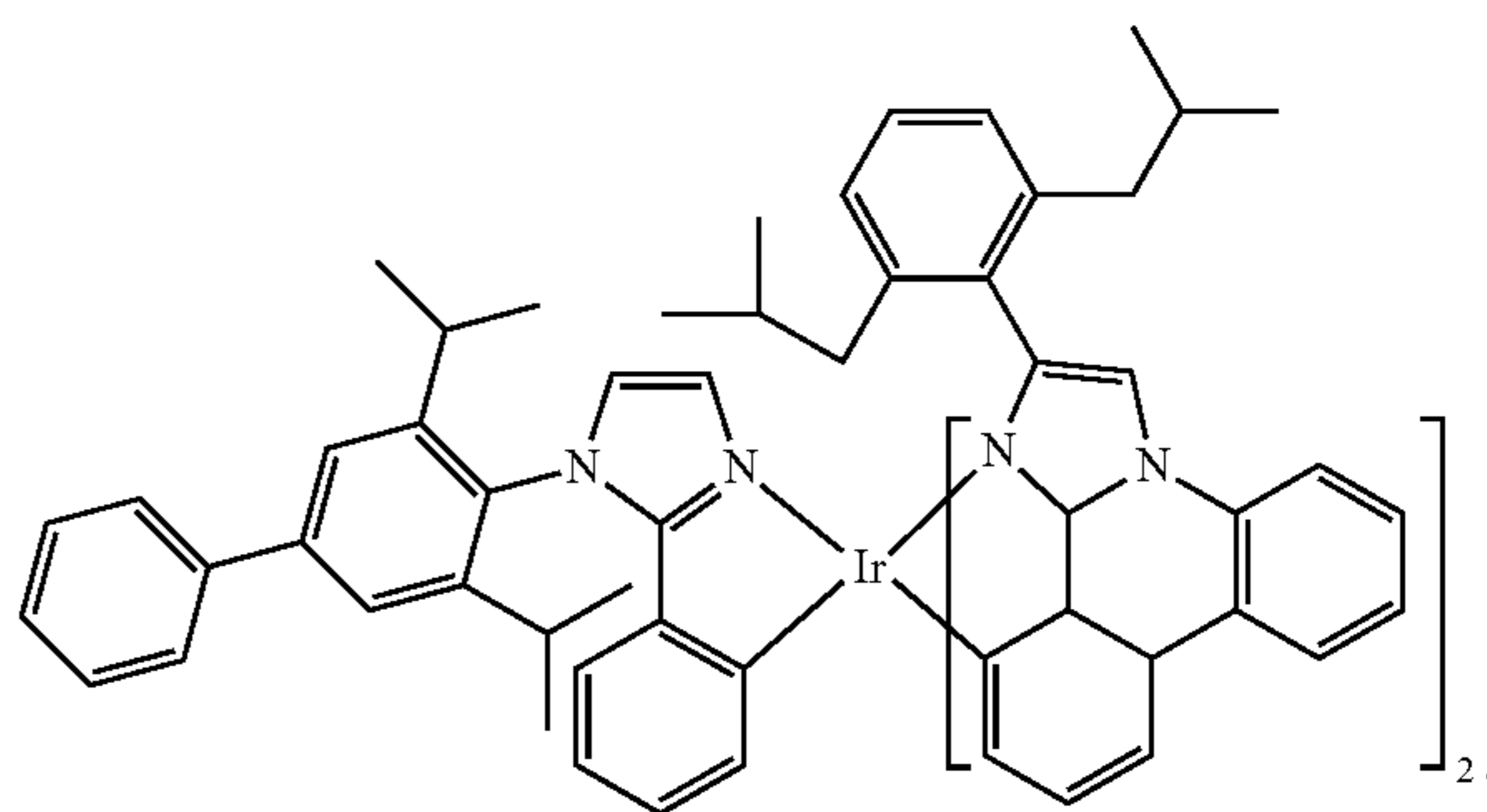
Compound 69
