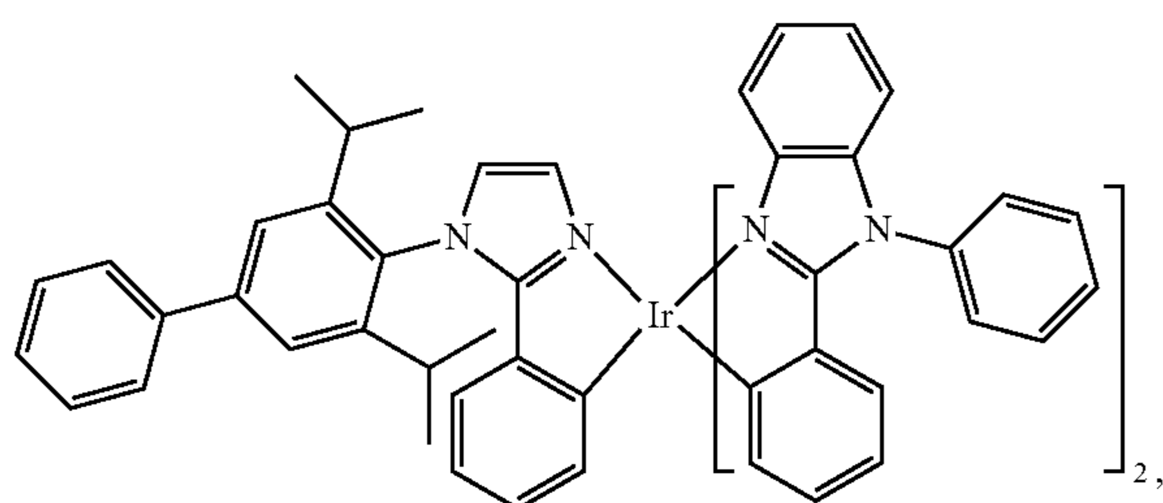
Compound 63
