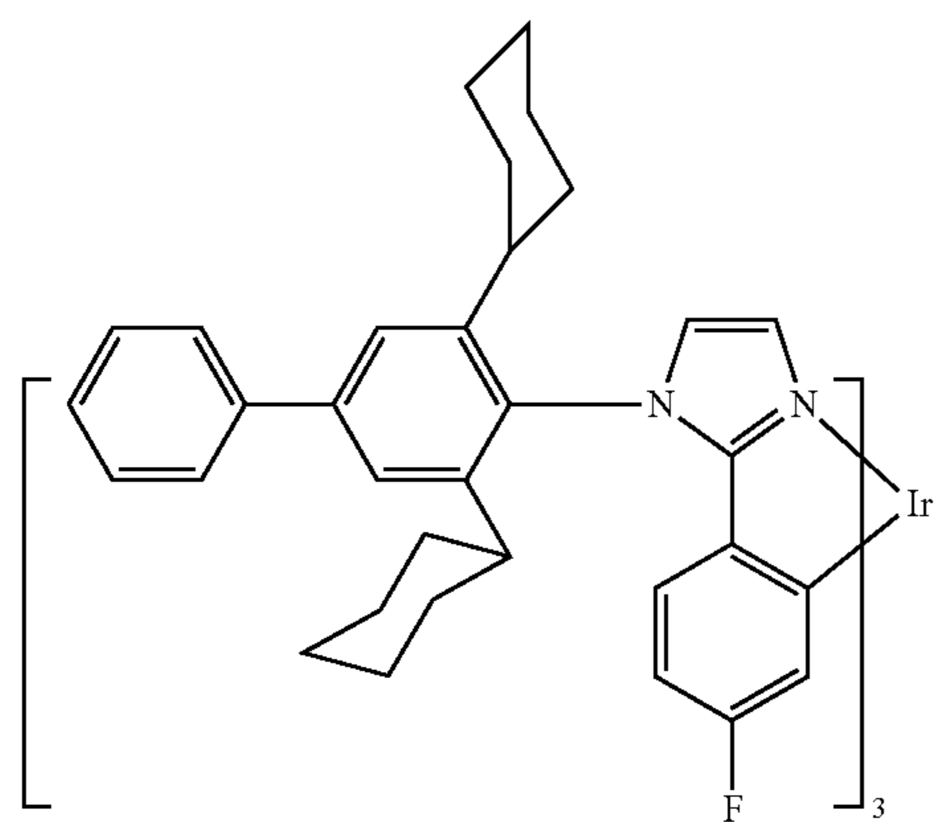
Compound 27
