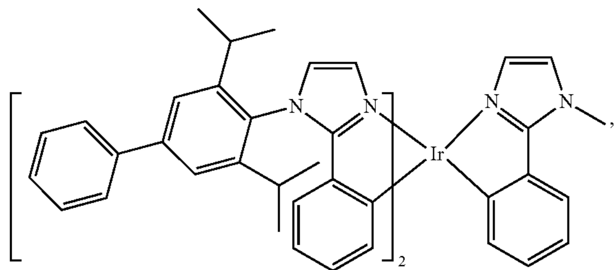
Compound 49
