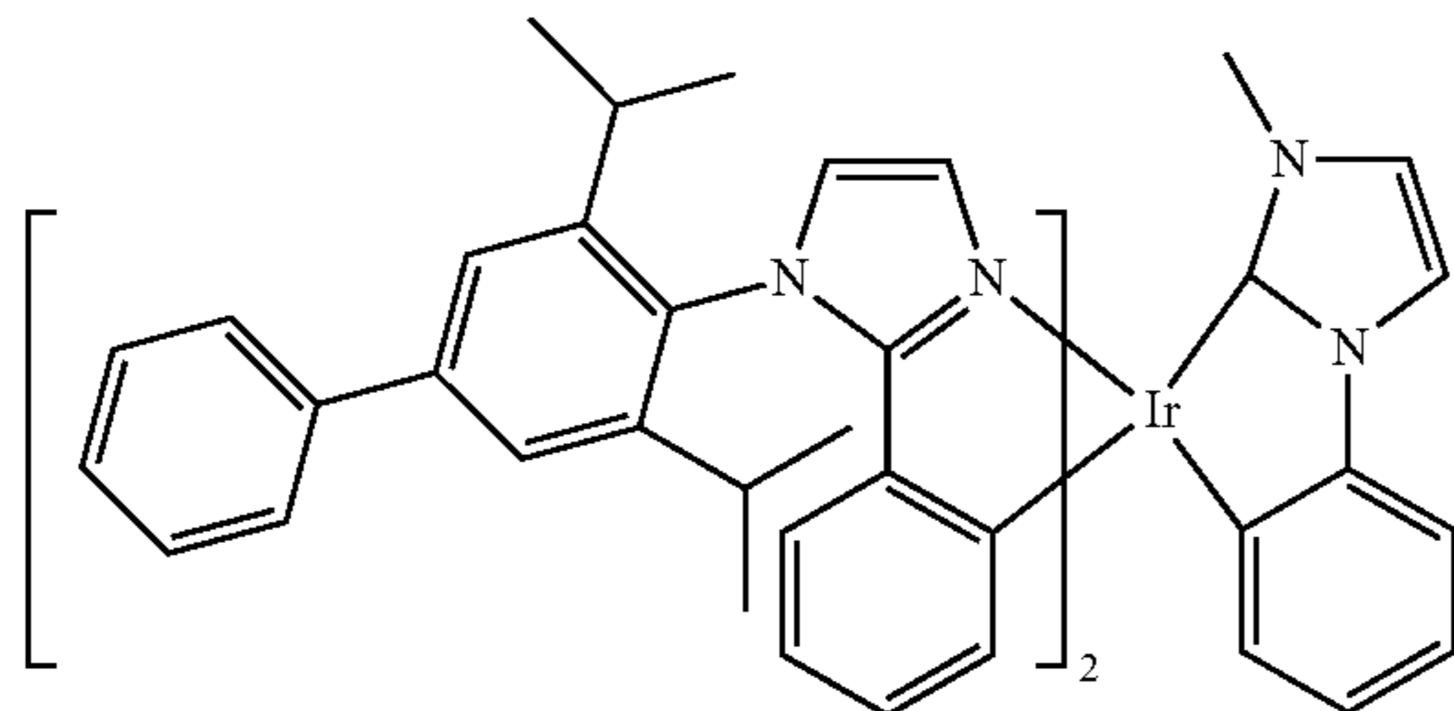
Compound 53
