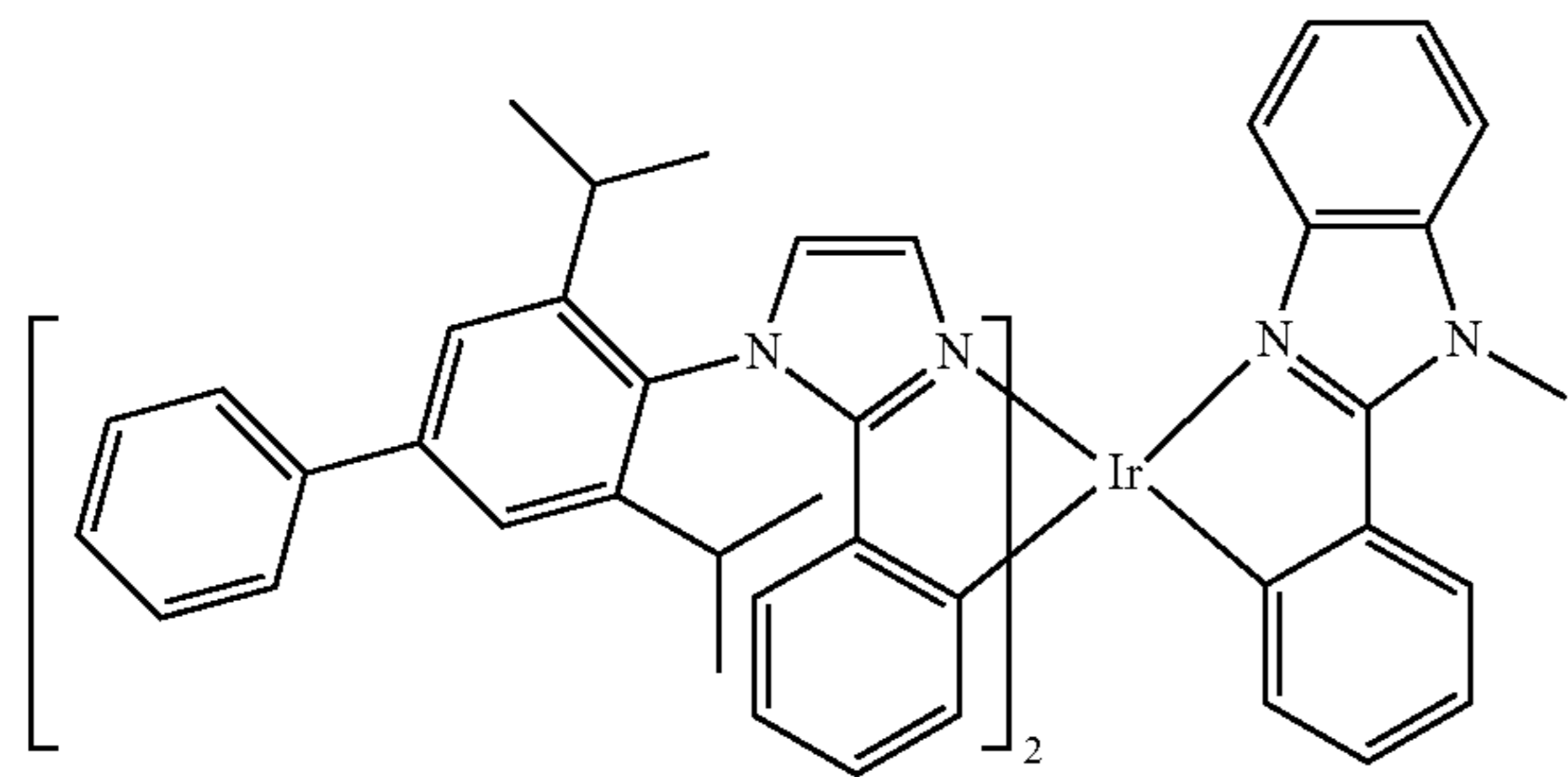
Compound 51
