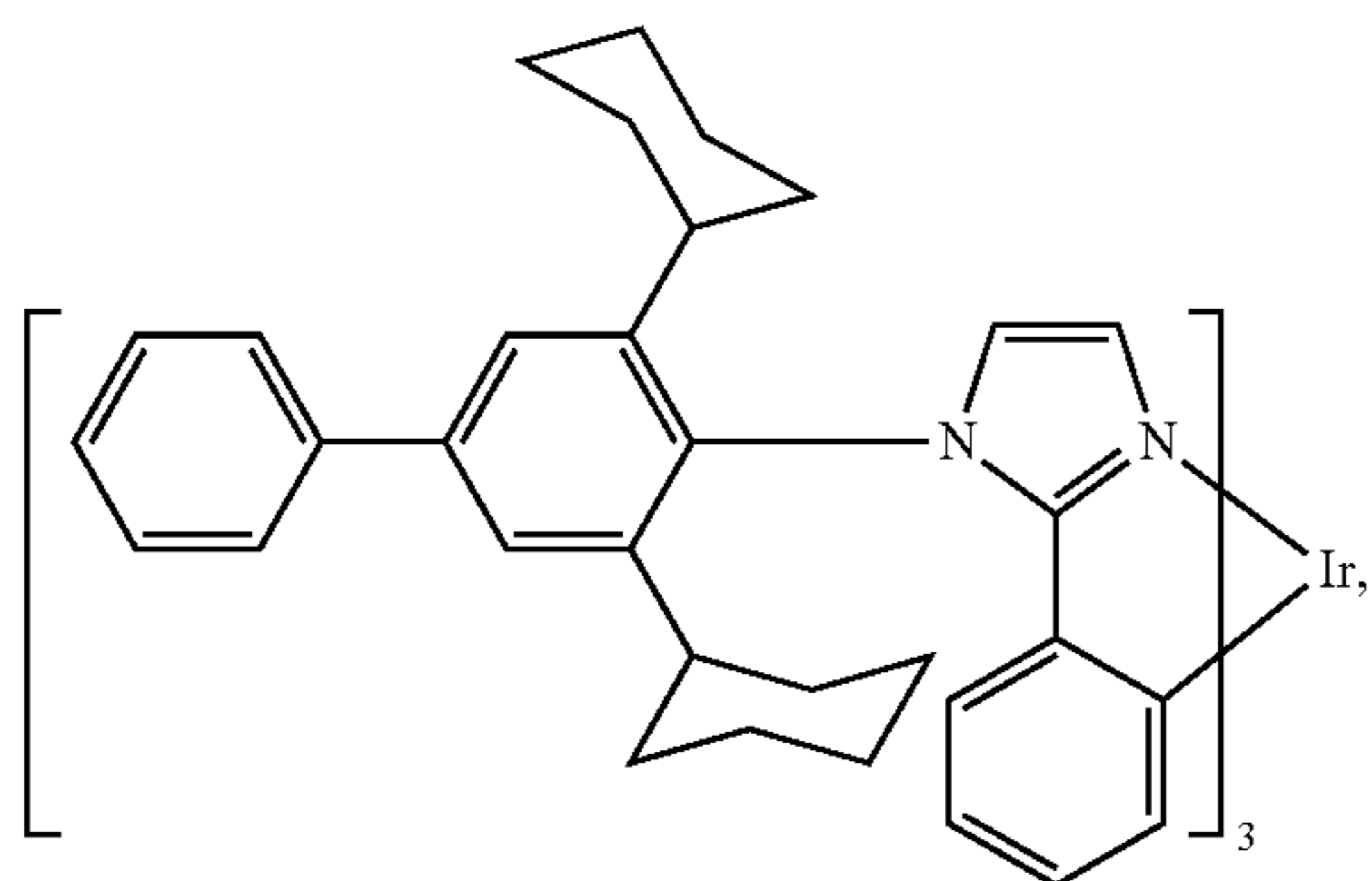
Compound 4
