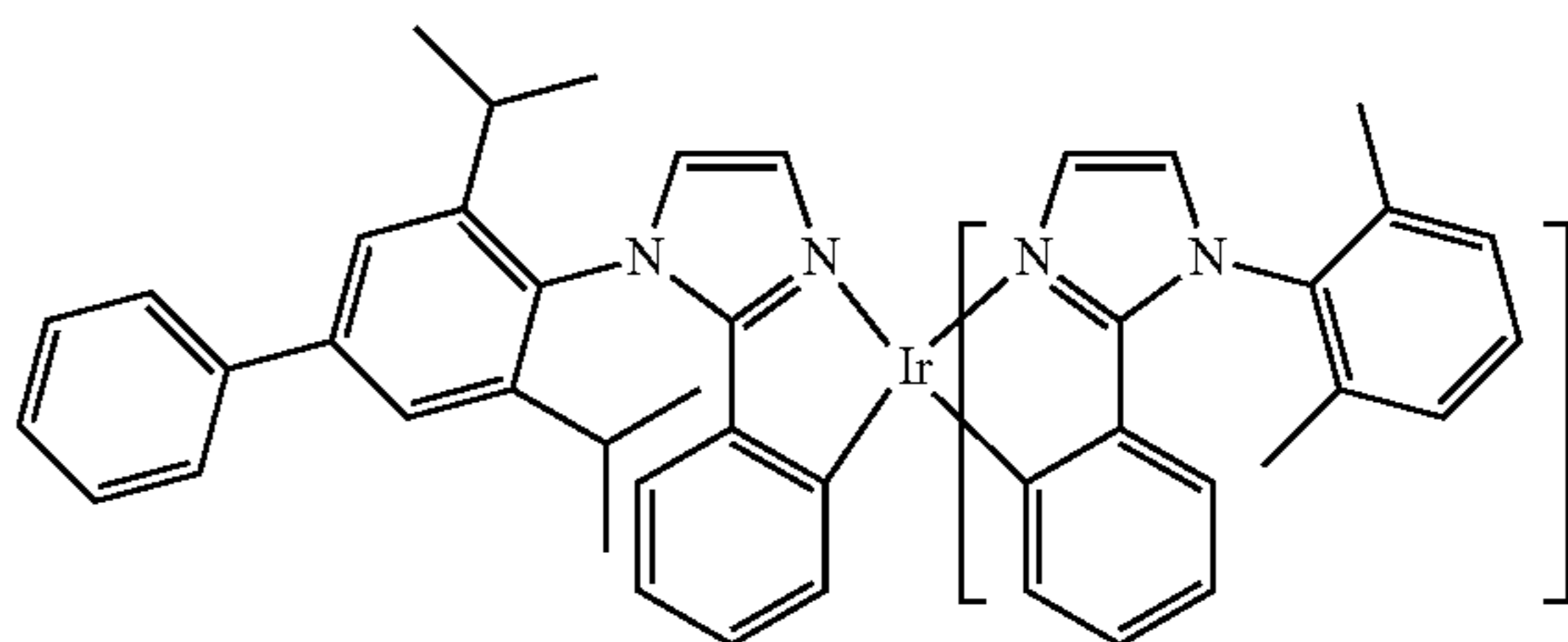
Compound 61
