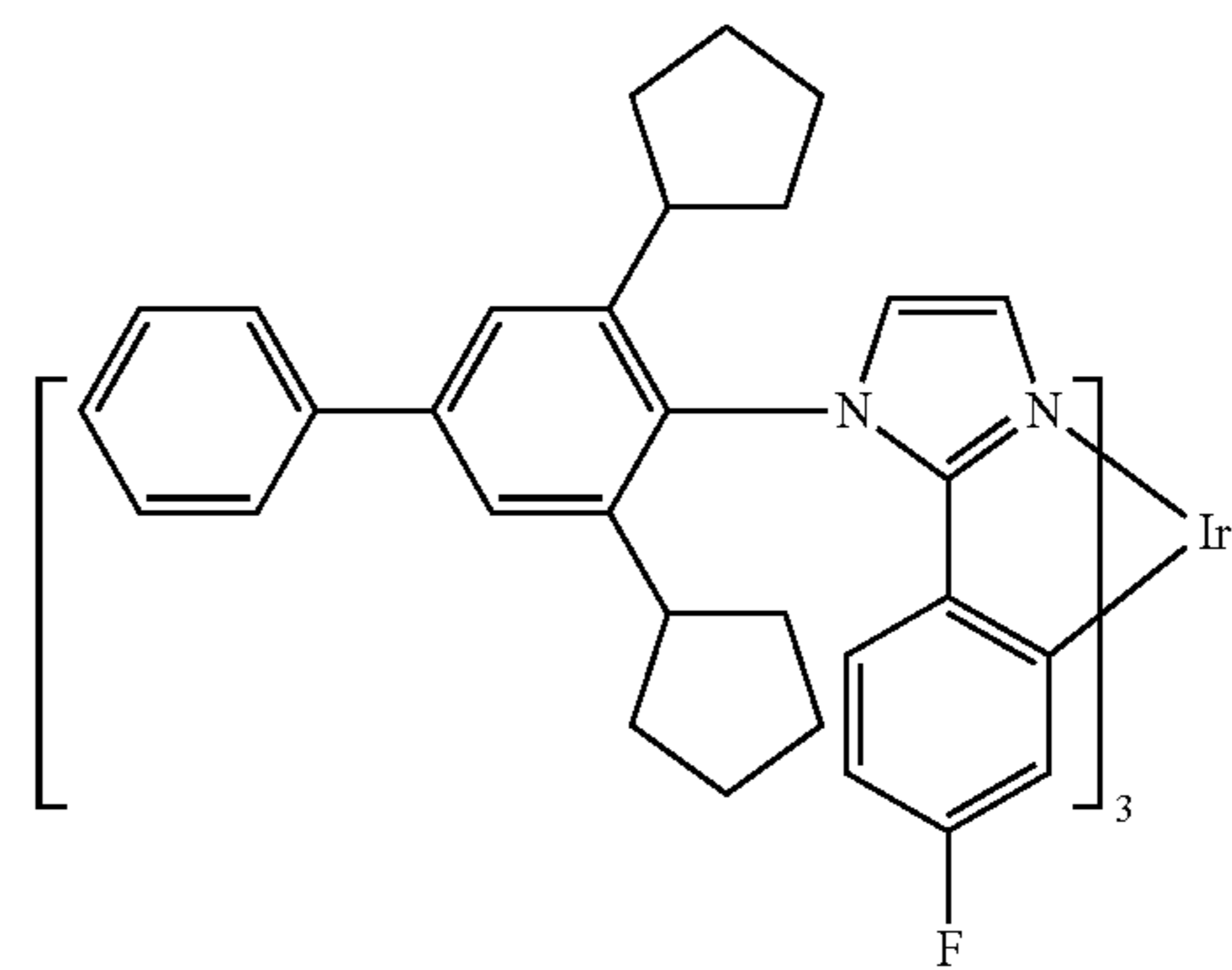
Compound 25
