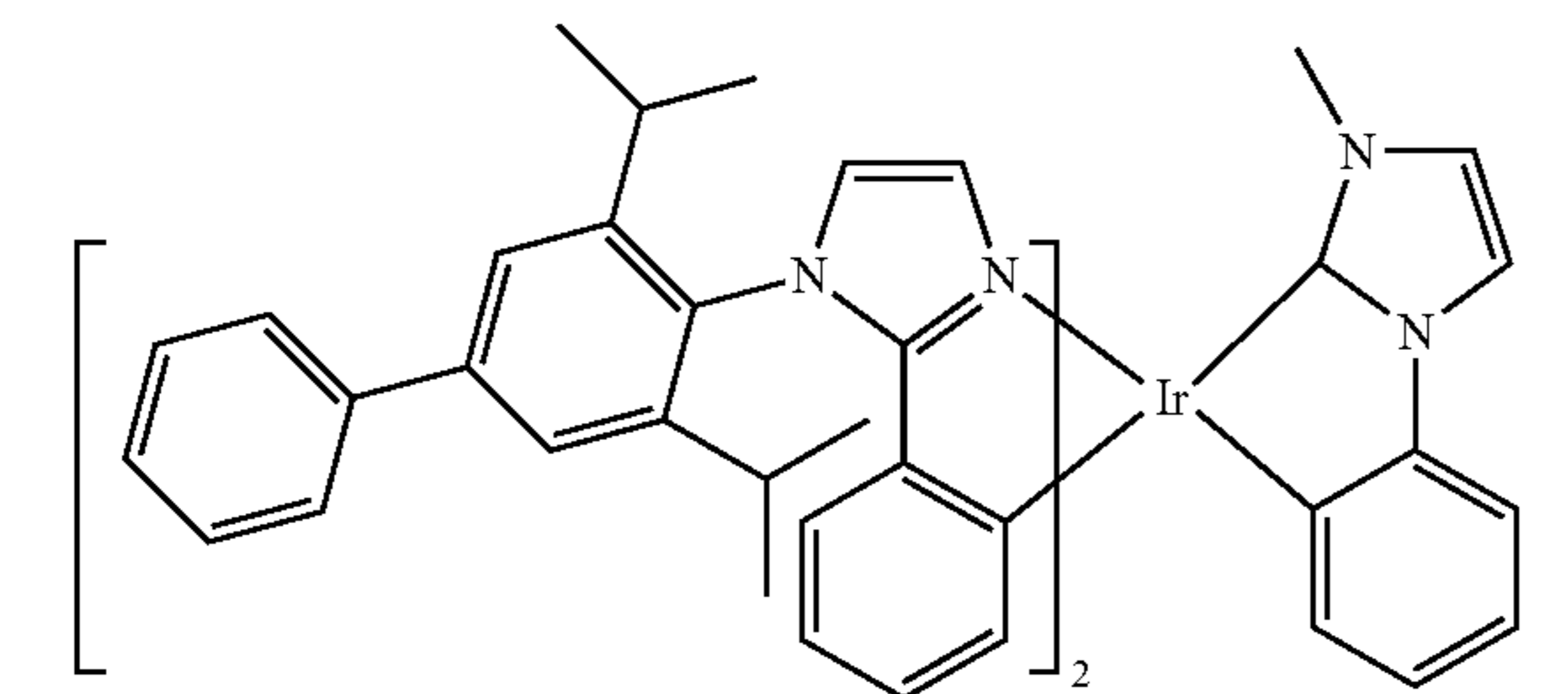
Compound 53
