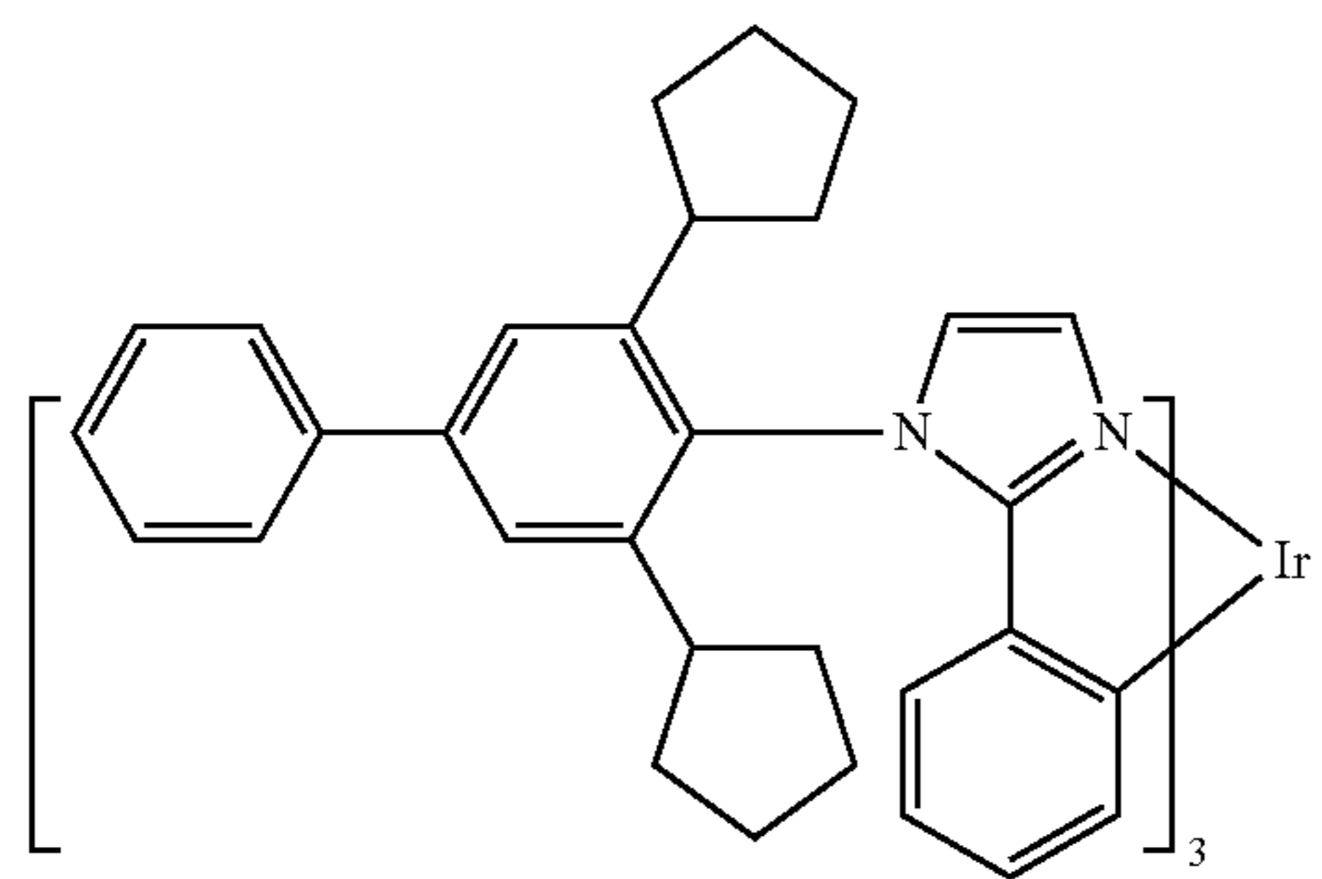
Compound 8
