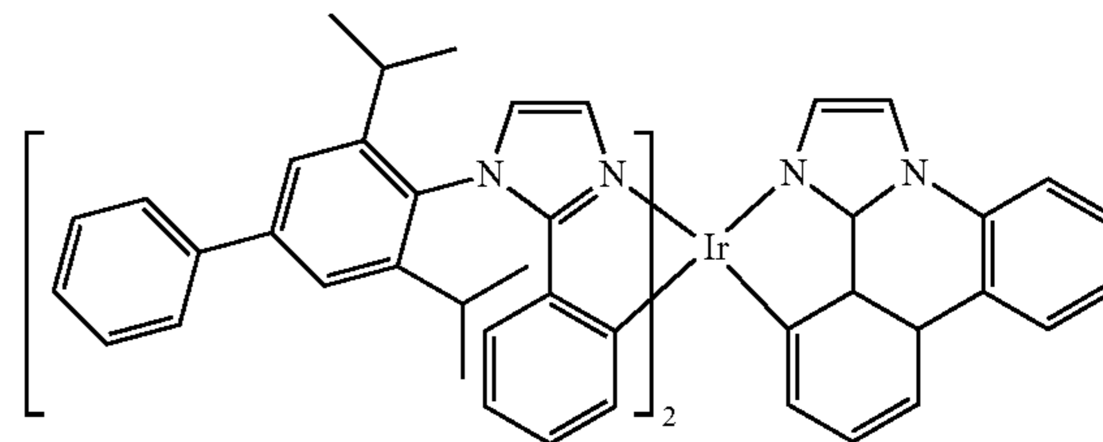
Compound 57
