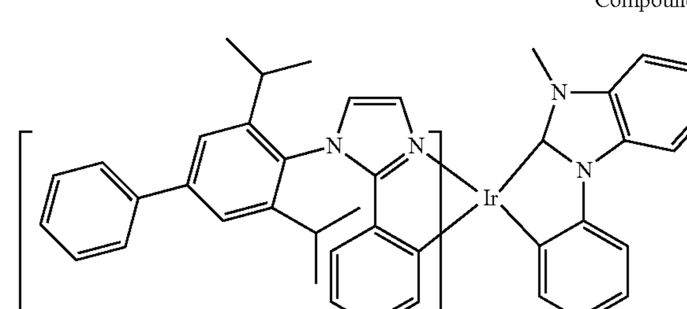
Compound 56
