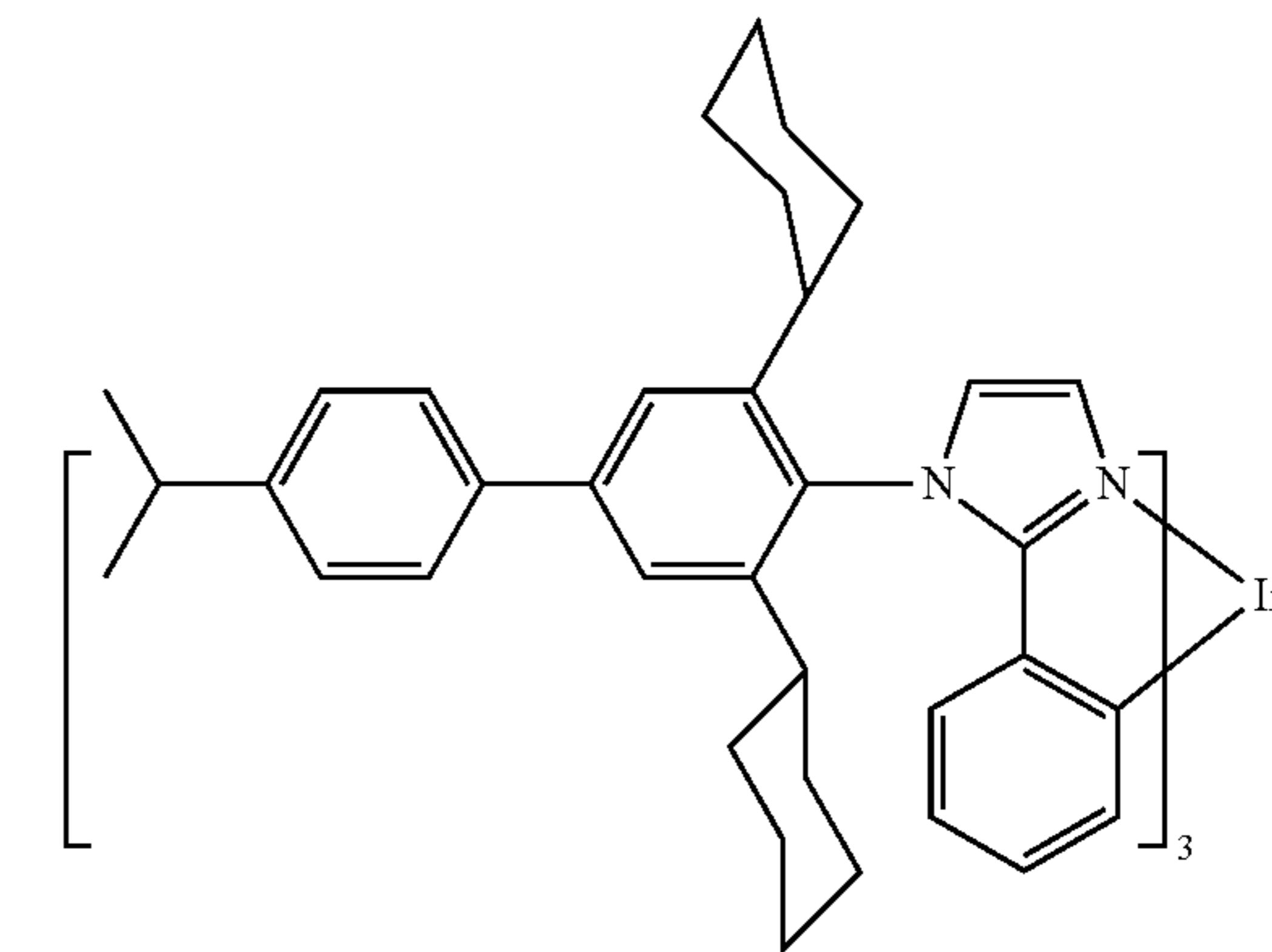
Compound 14
