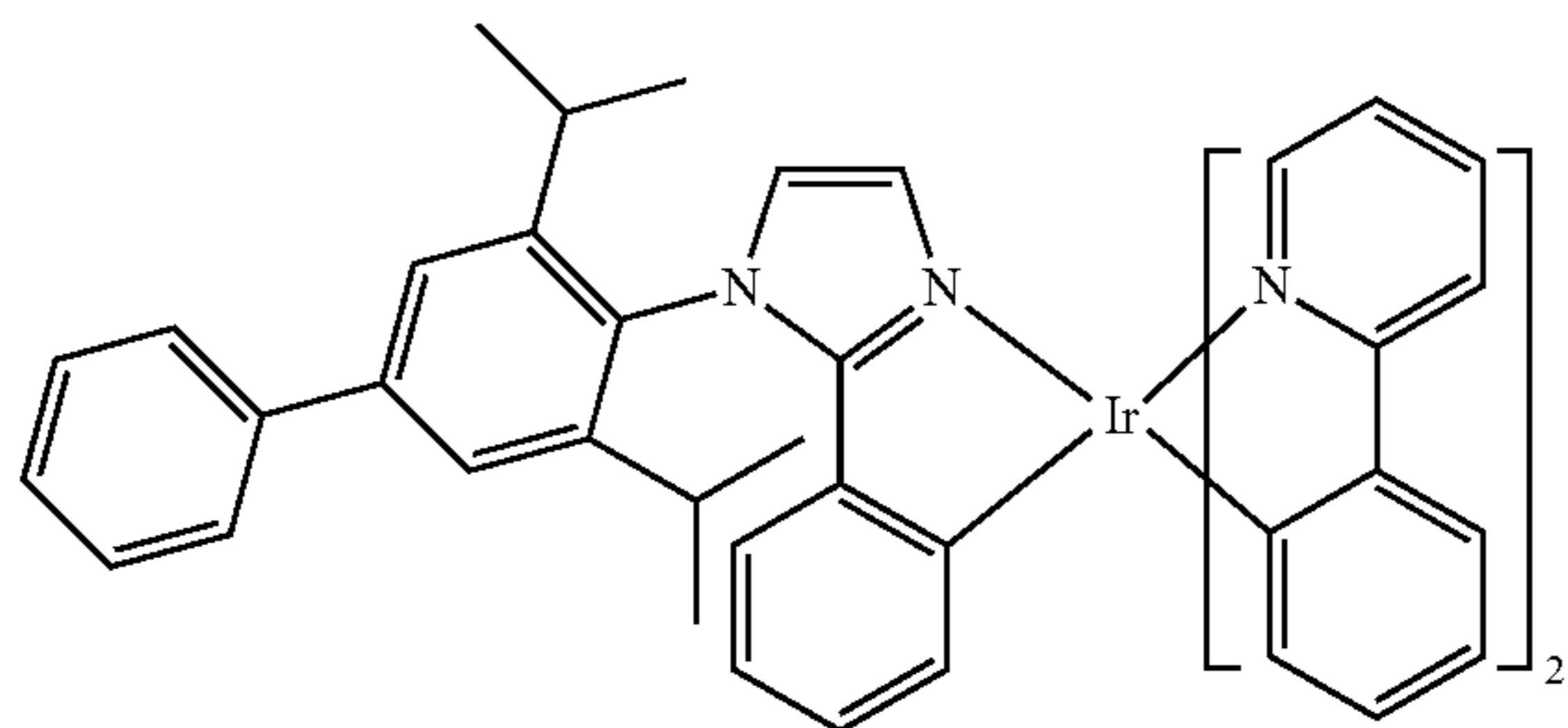
Compound 59
