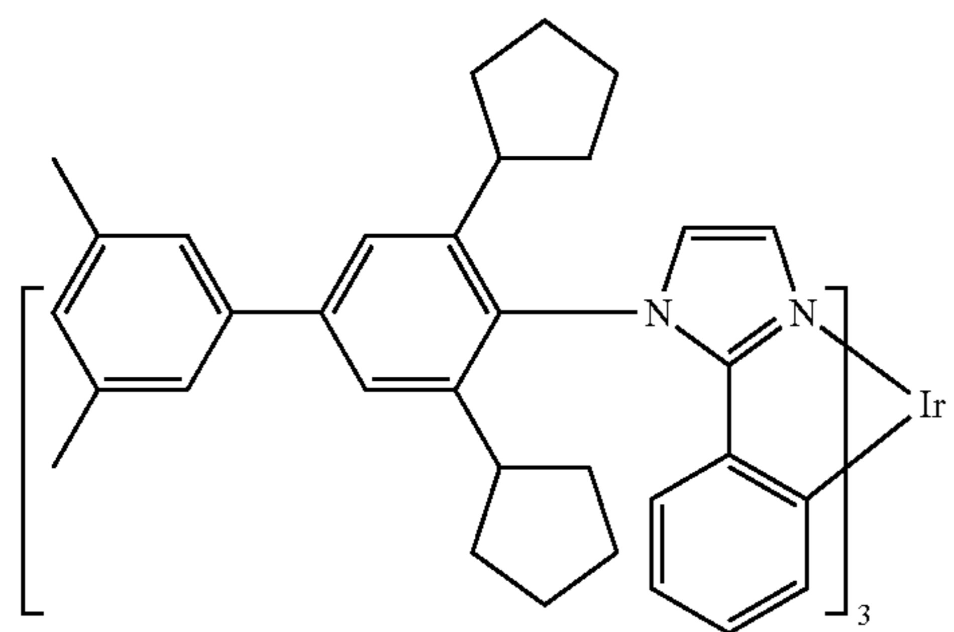
Compound 9
