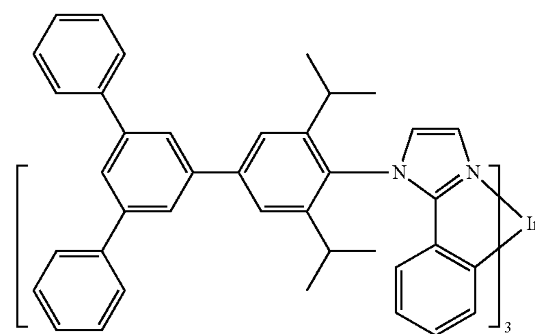
Compound 31
