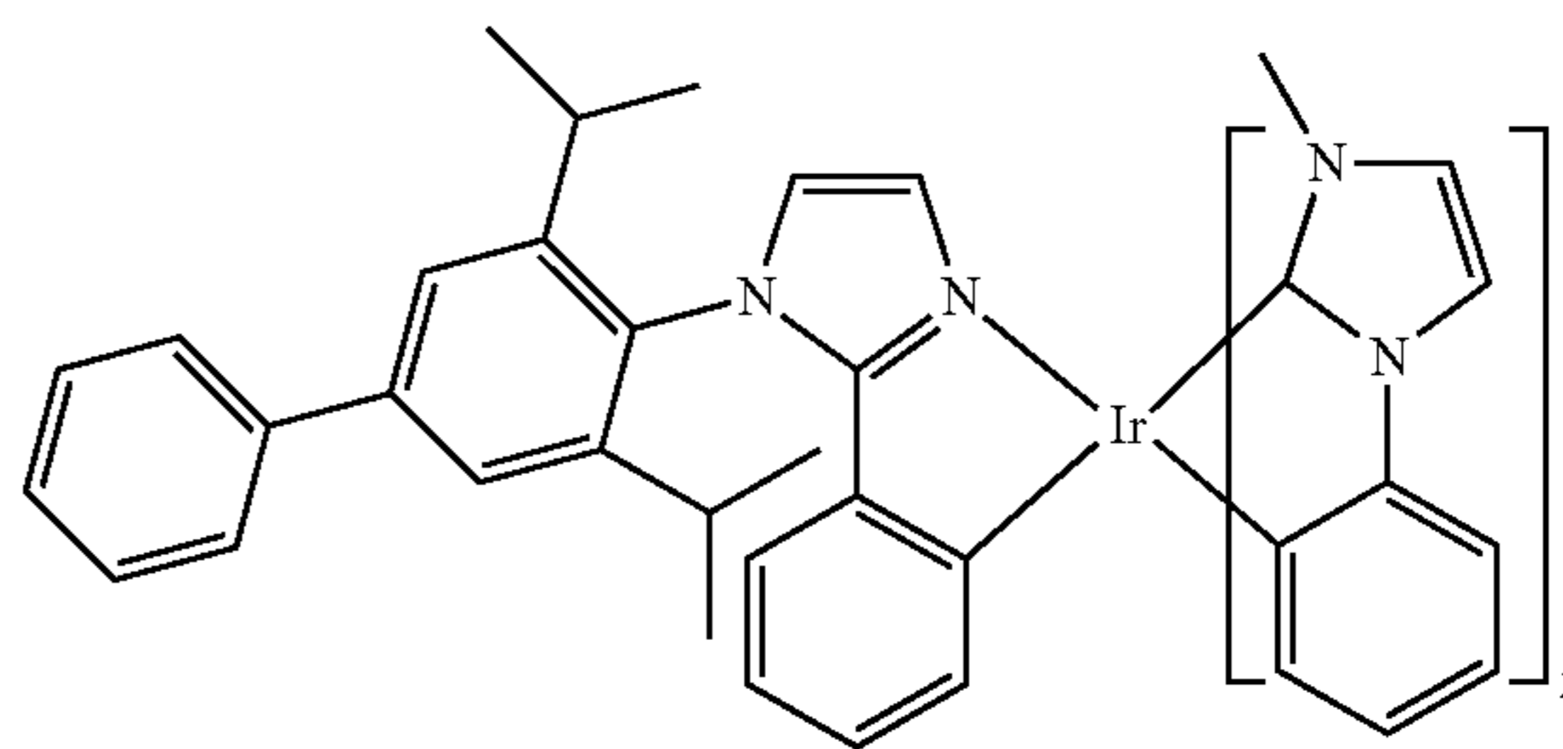
Compound 64
