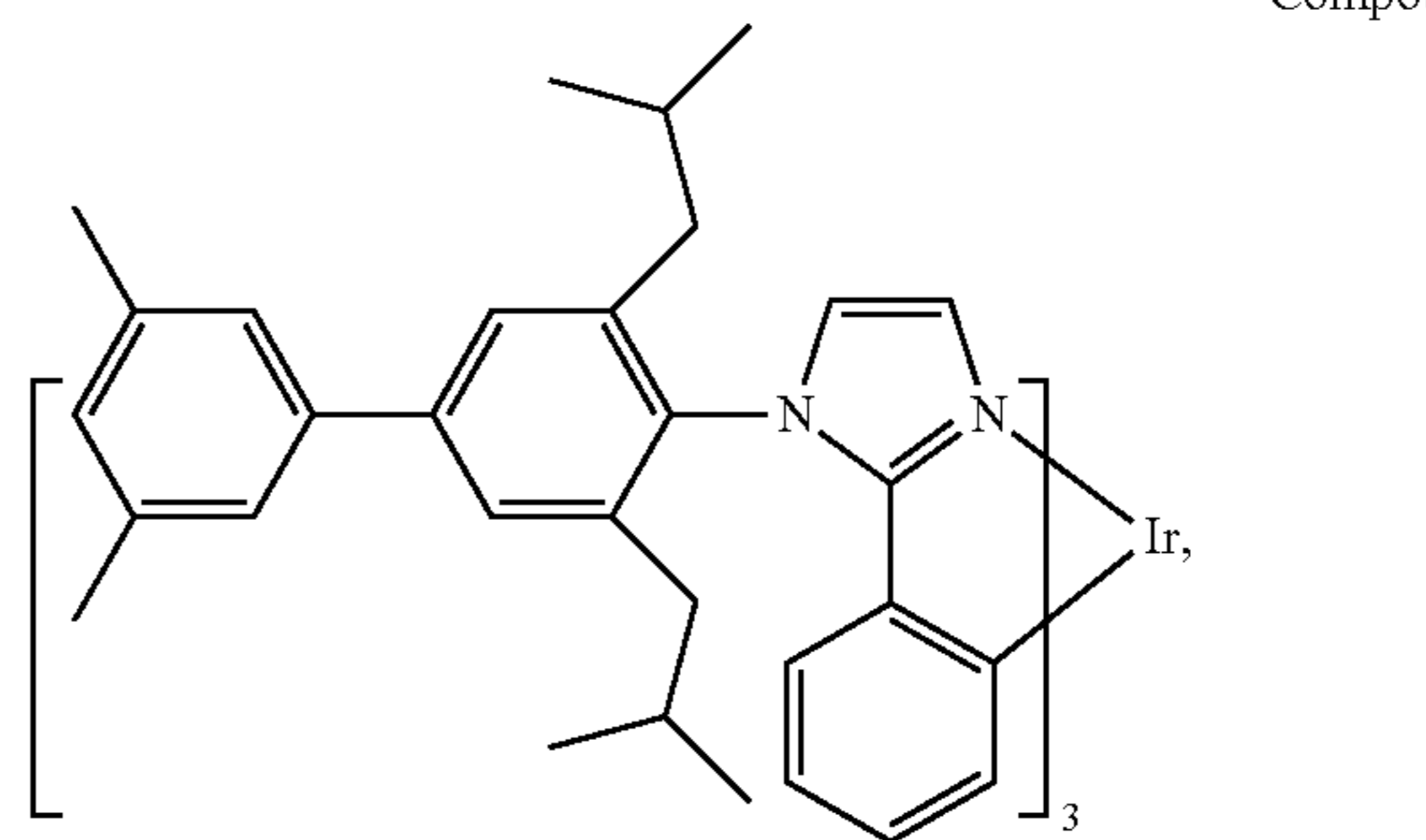
Compound 12
