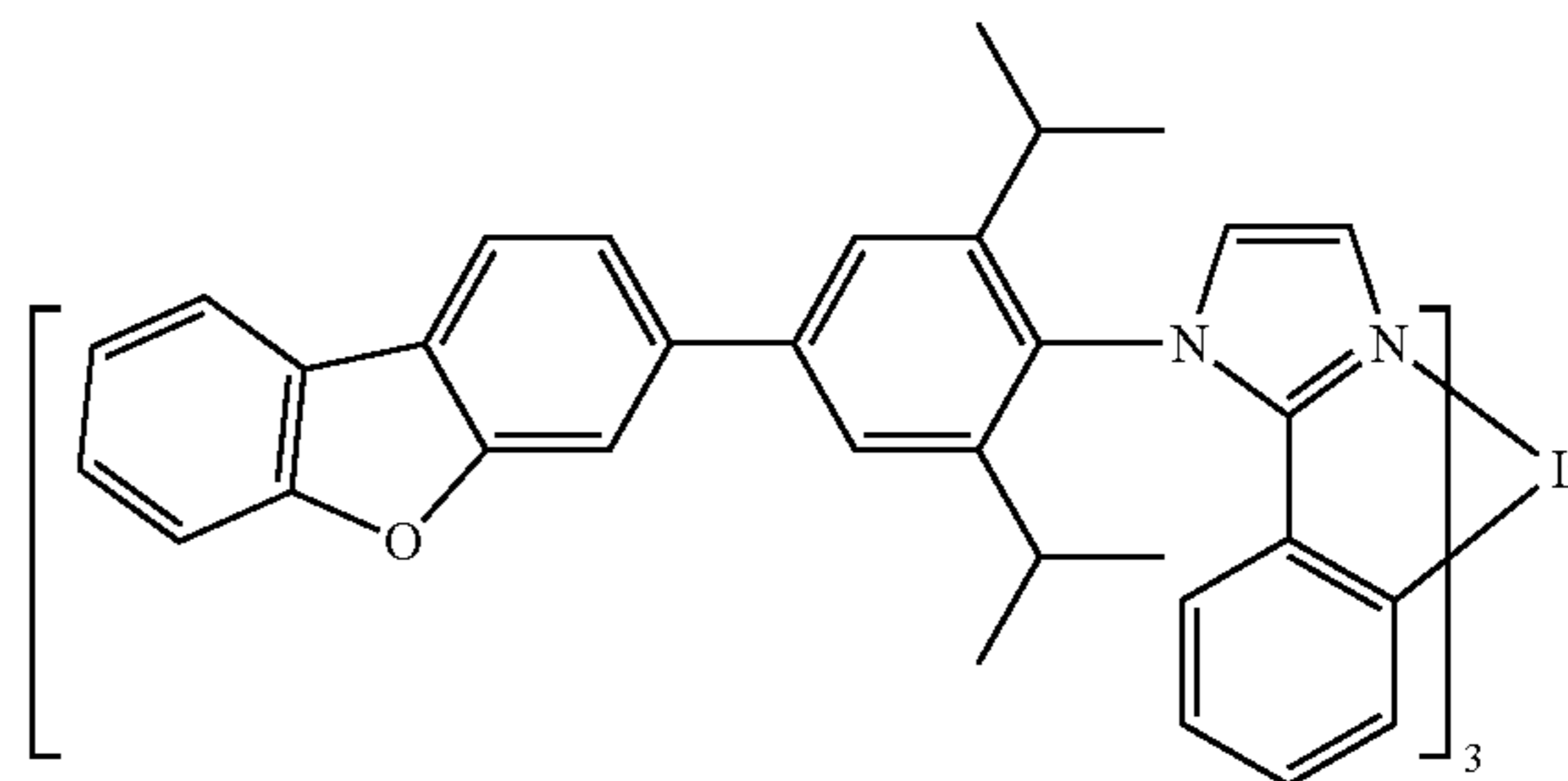
Compound 35
