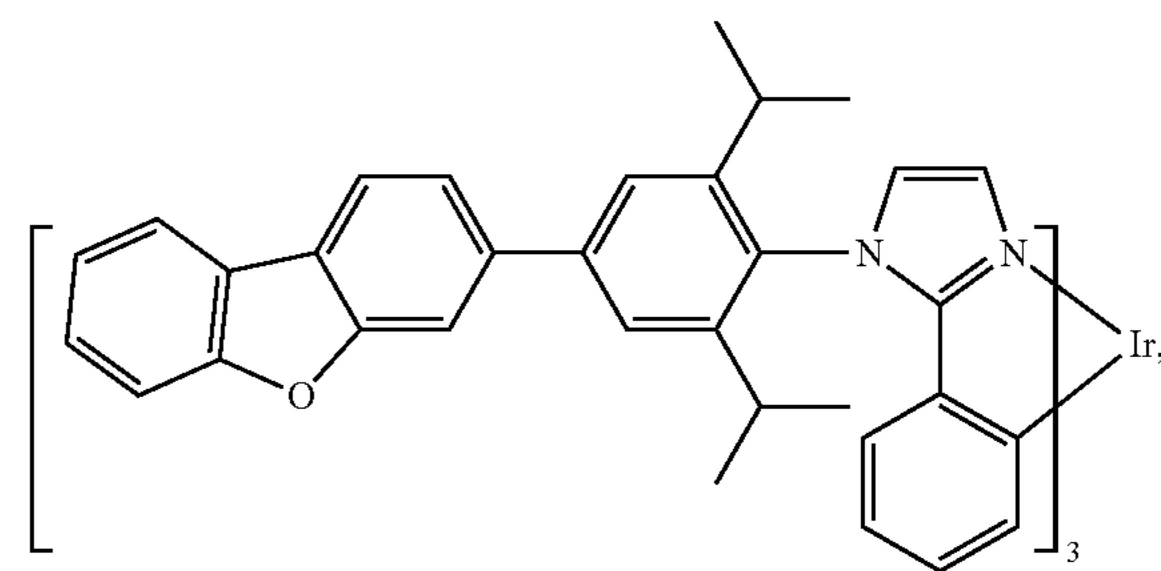
Compound 35
