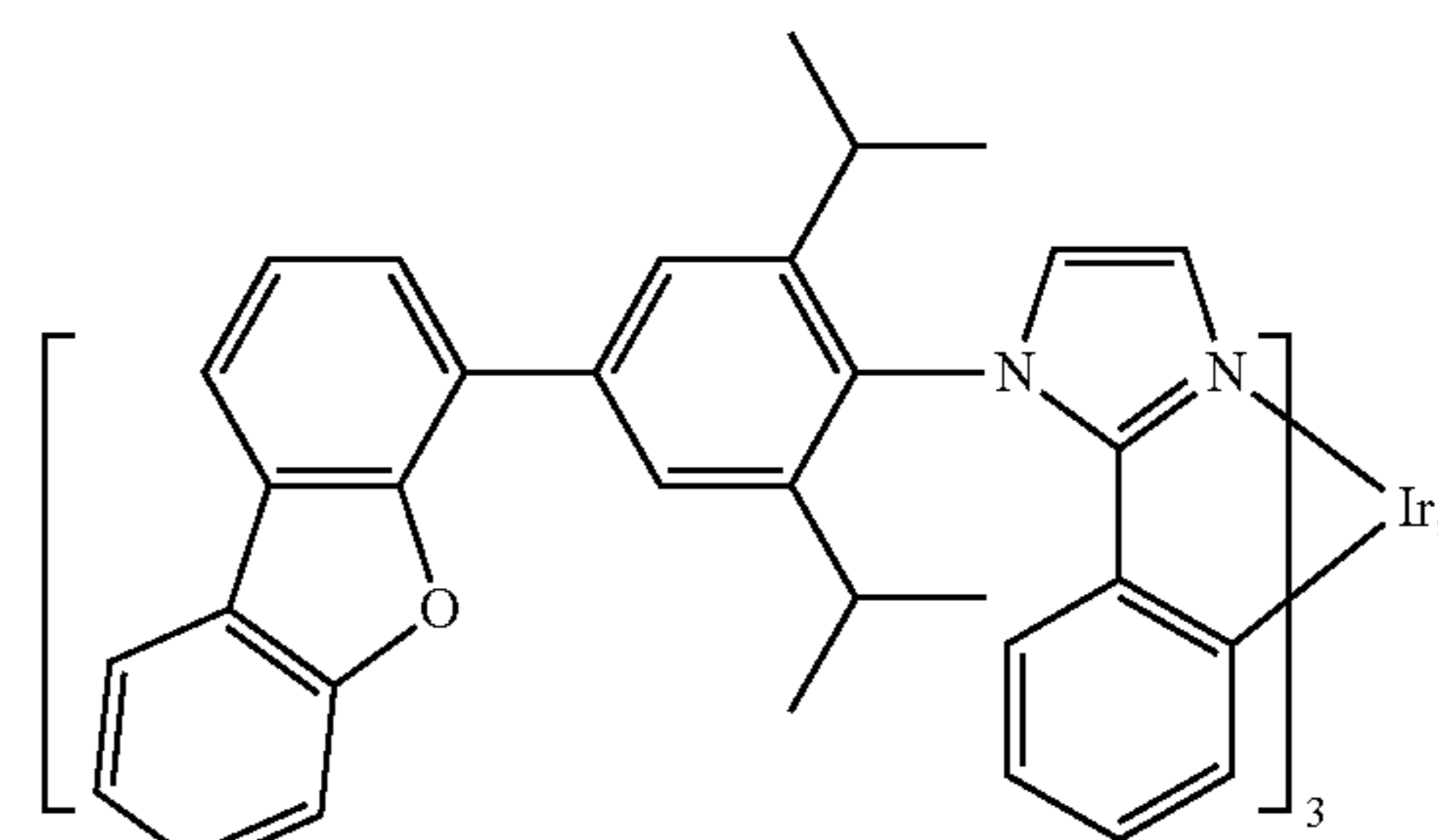
Compound 37
