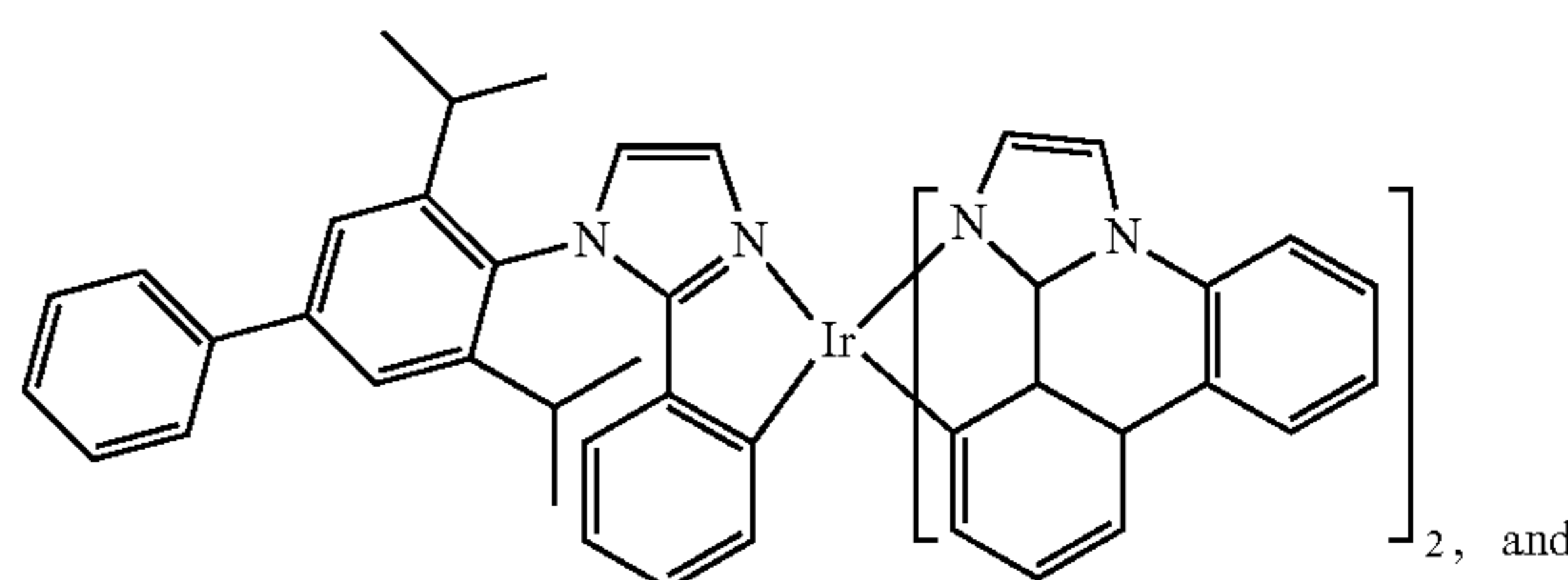
Compound 69
