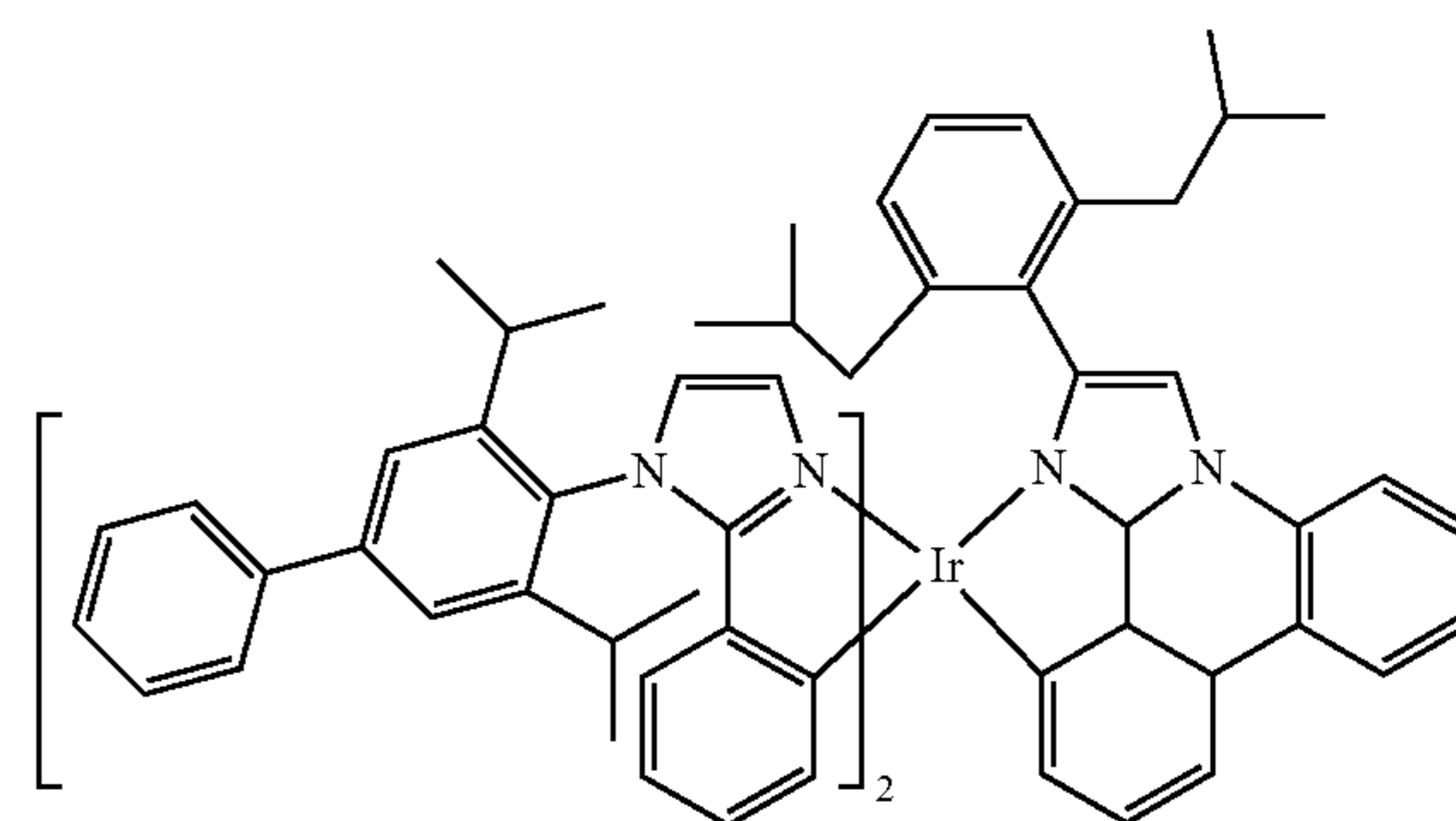
Compound 58
