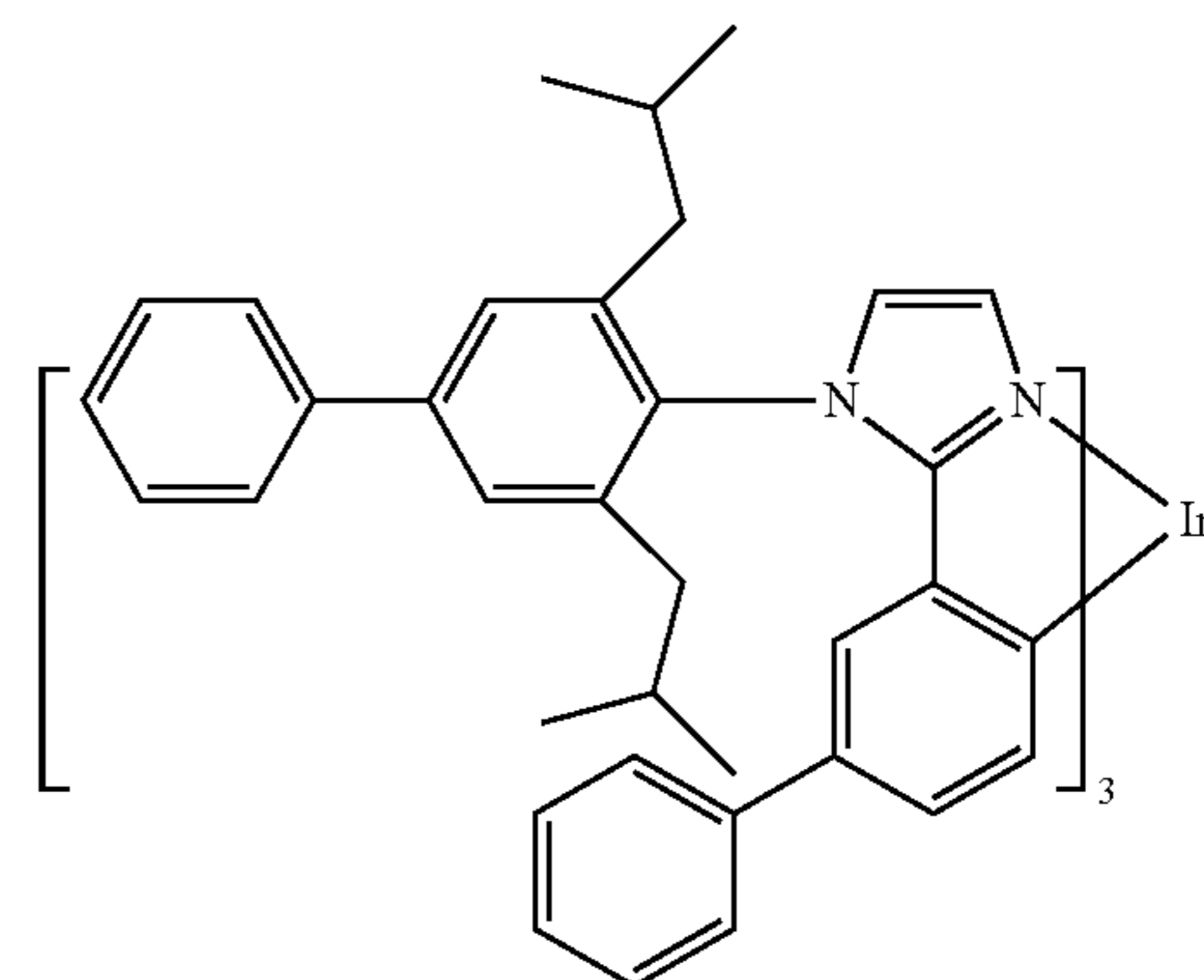
Compound 16
