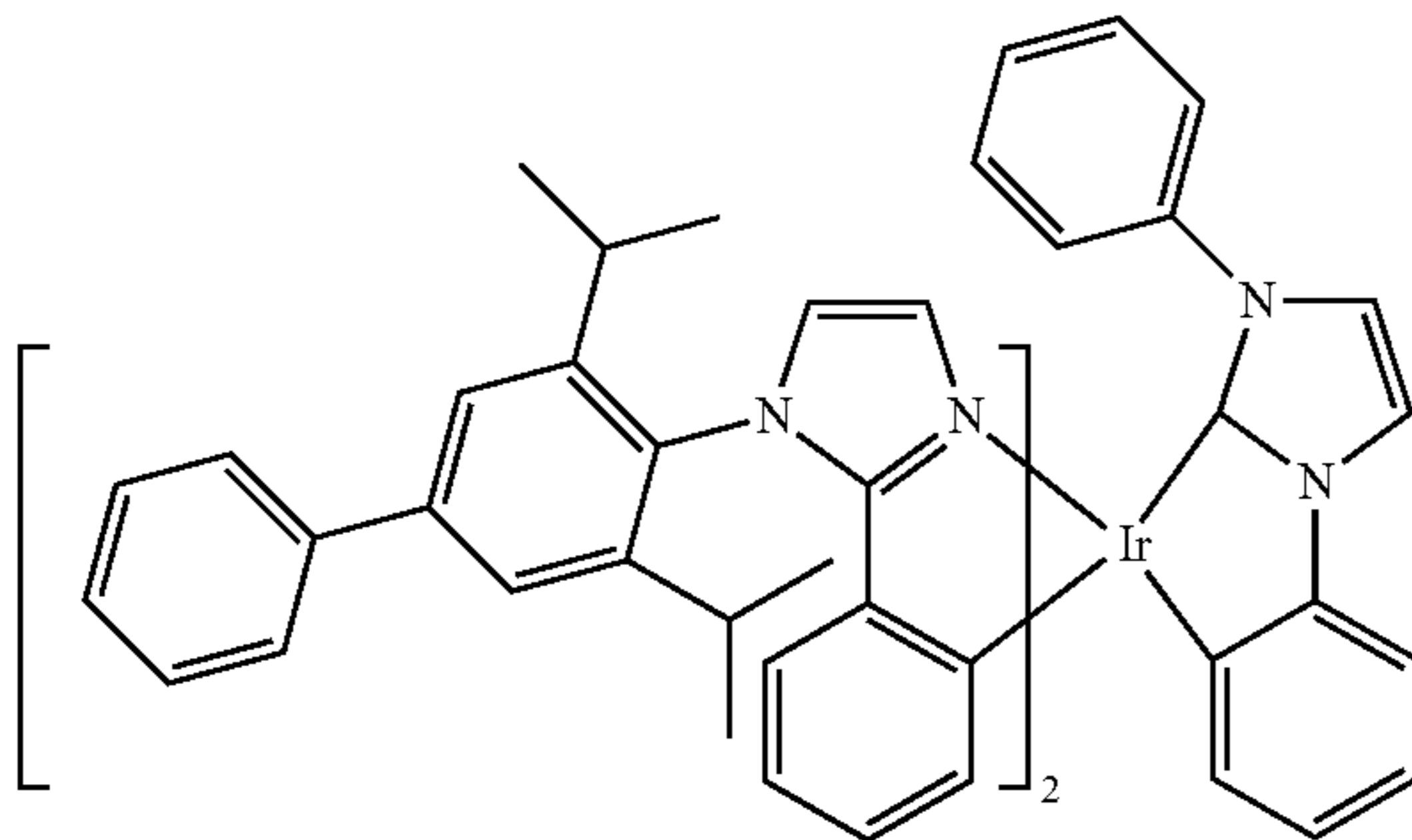
Compound 54
