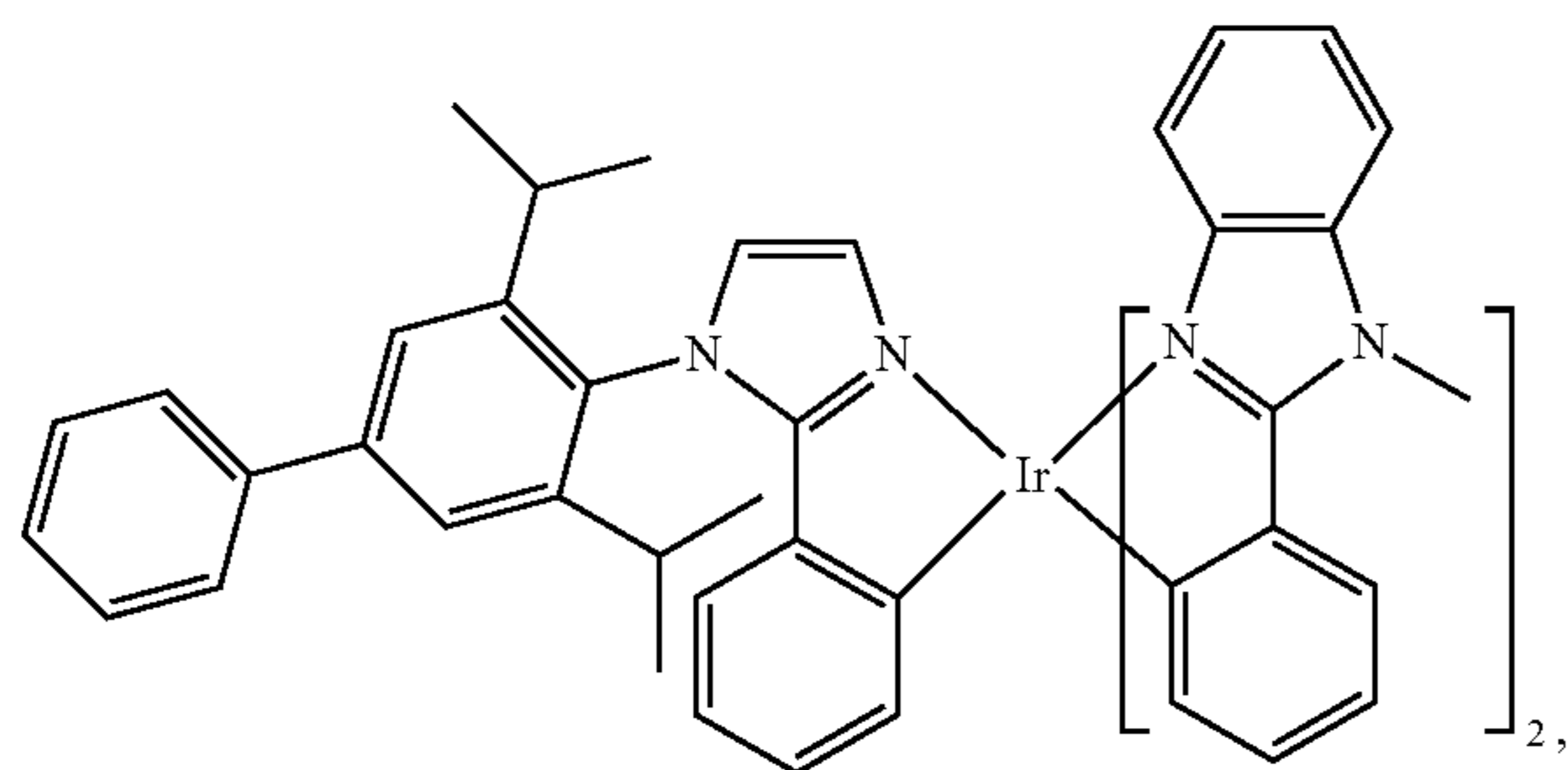
Compound 62
