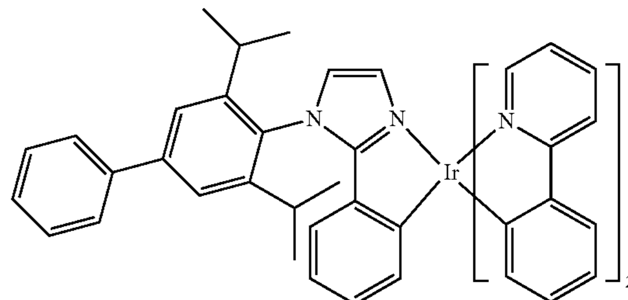
Compound 59
