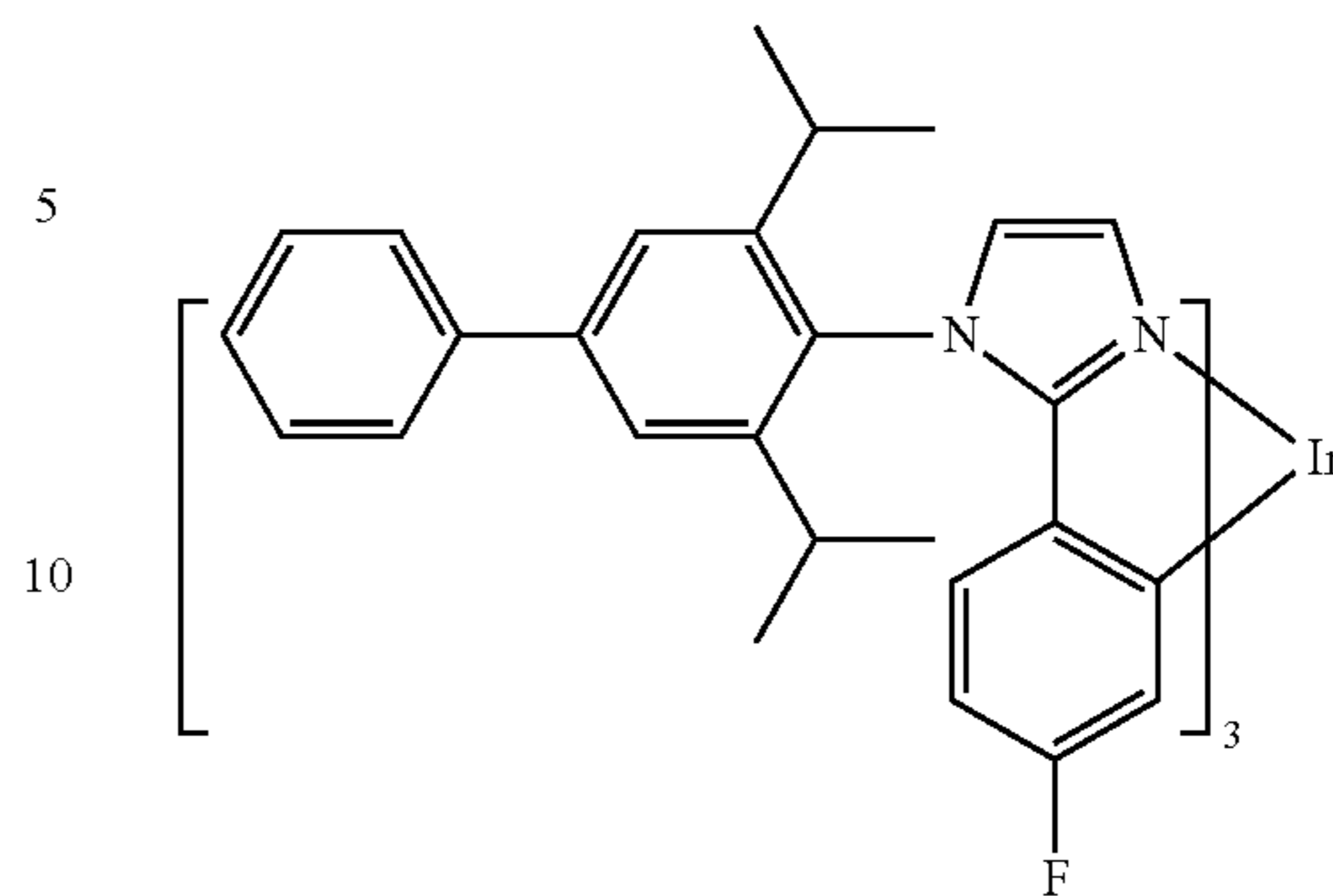
Compound 29
