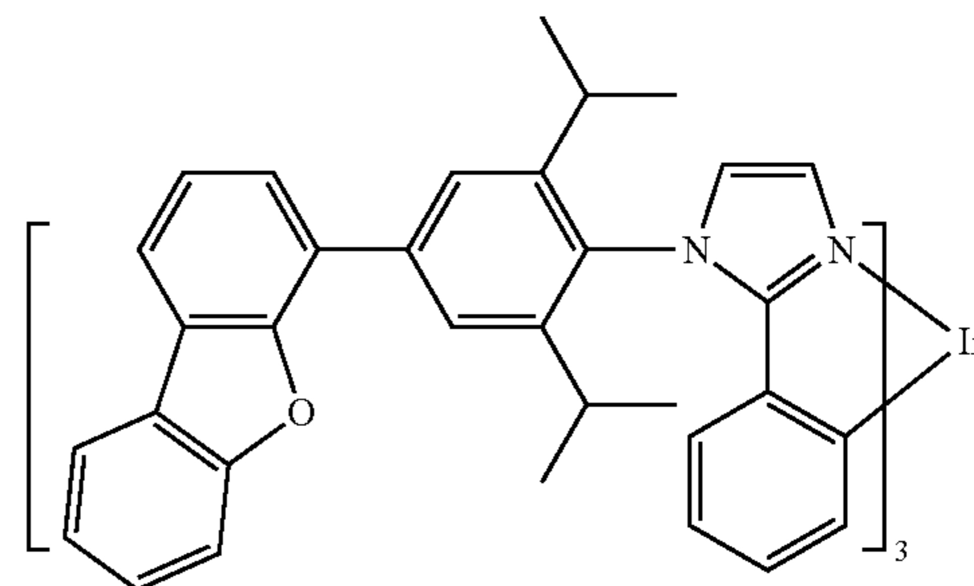
Compound 37
