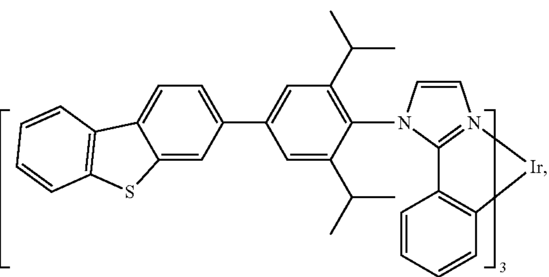
Compound 32
