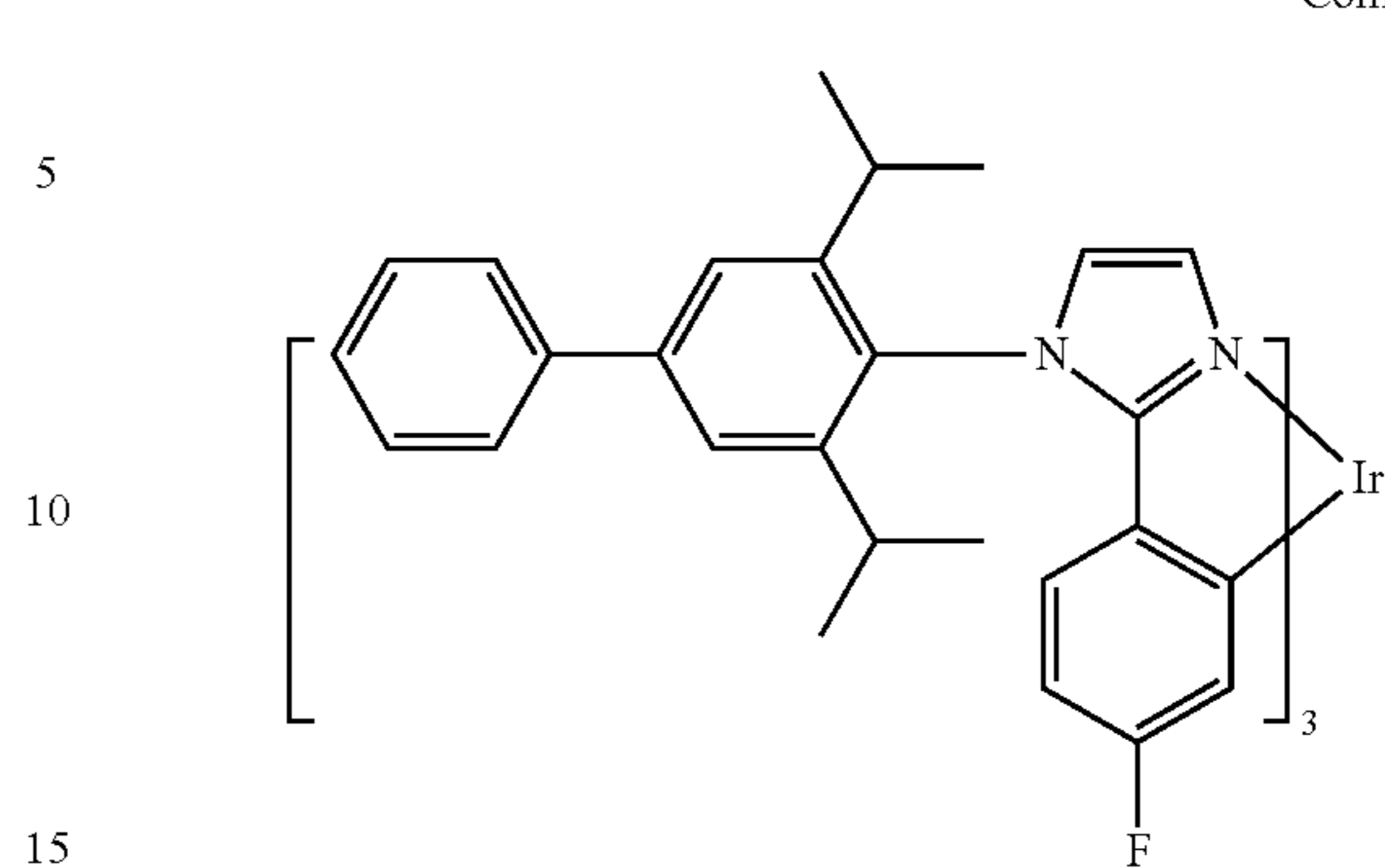
Compound 28
