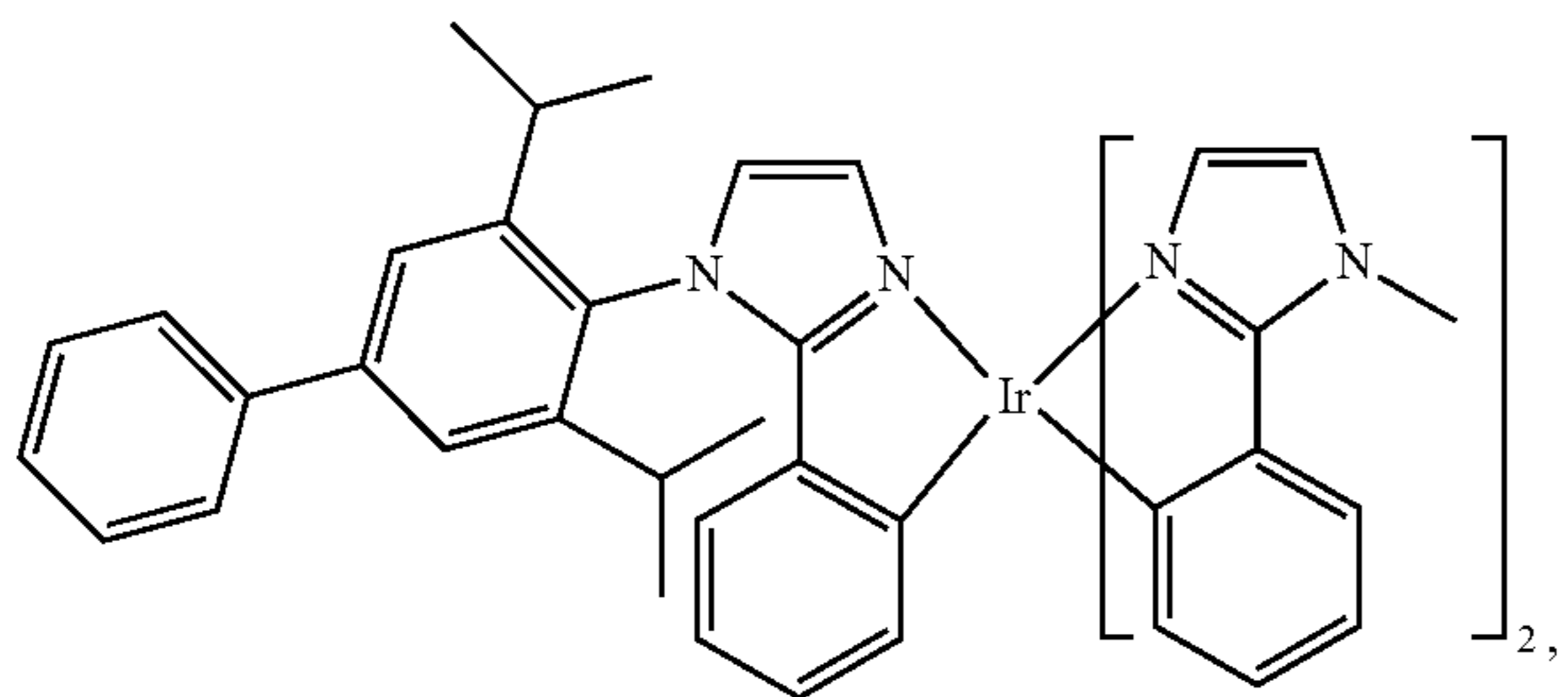
Compound 61
