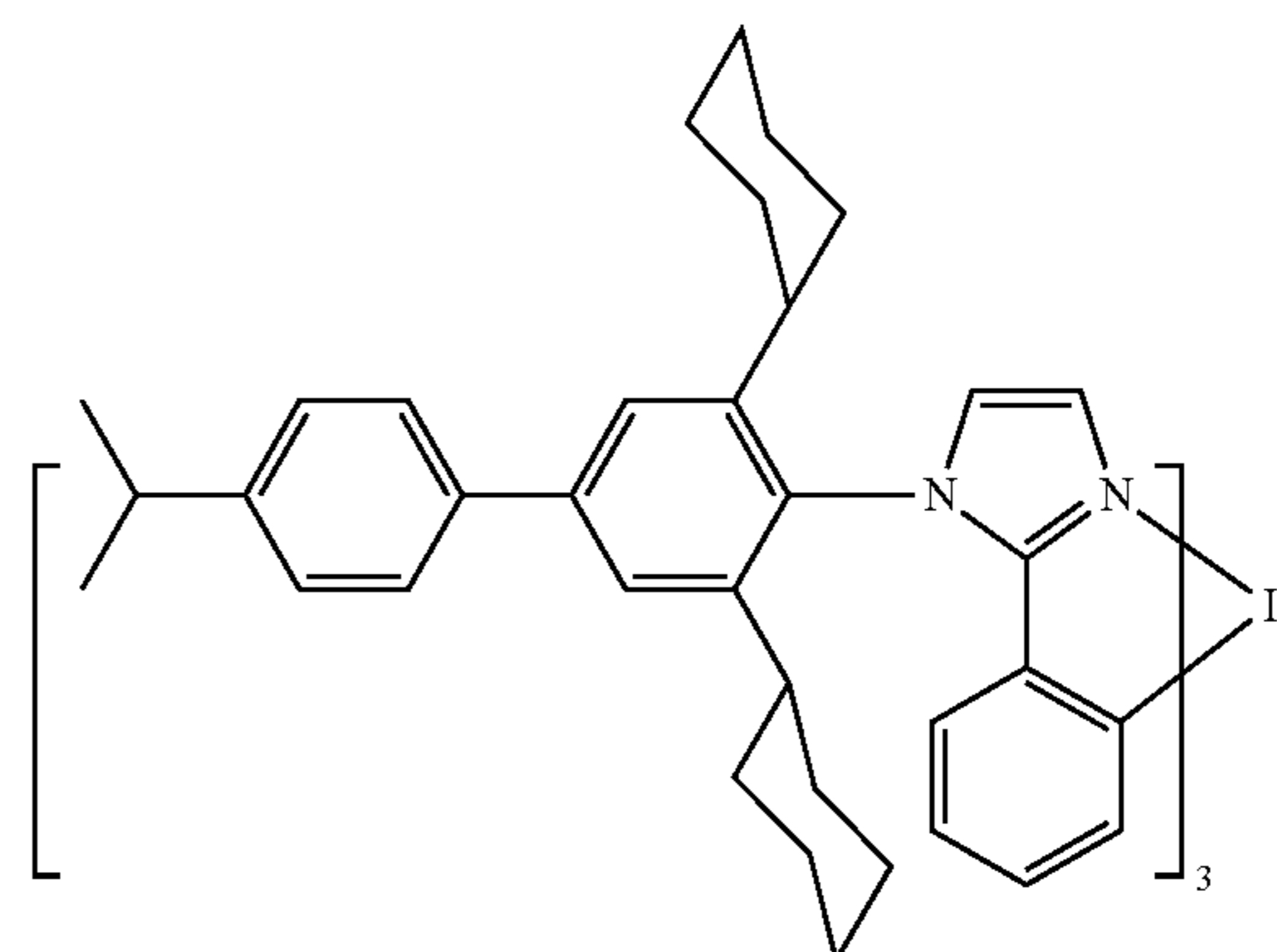
Compound 15
