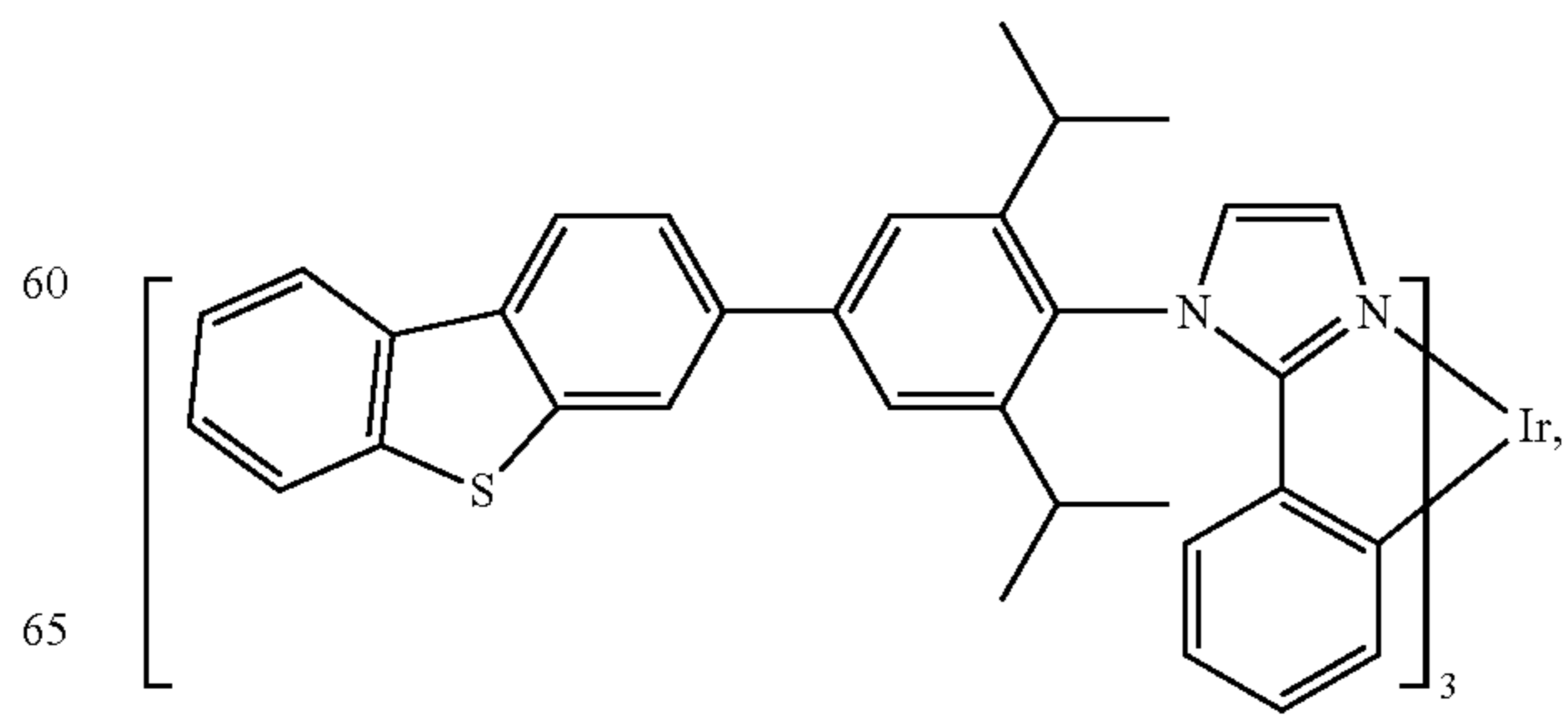
Compound 32
