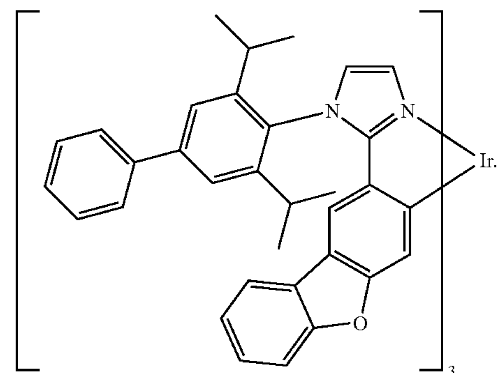
Compound 7
