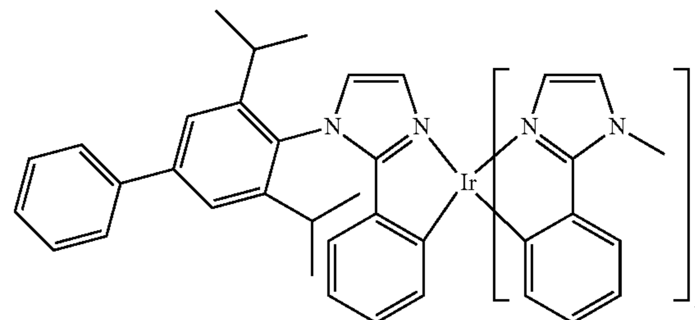
Compound 60
