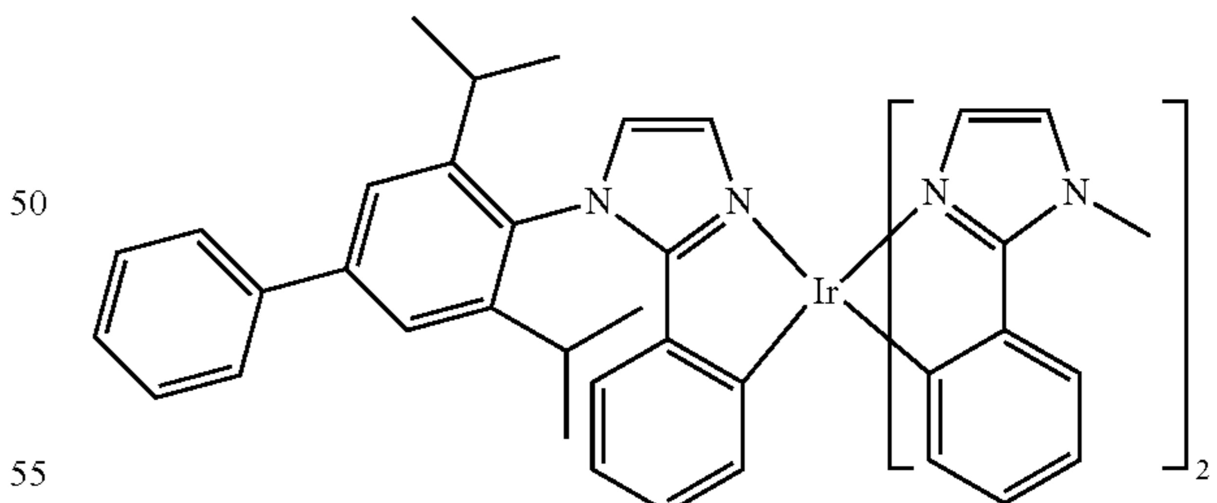
Compound 61
