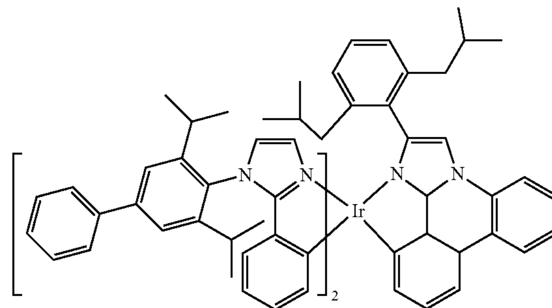
Compound 58
