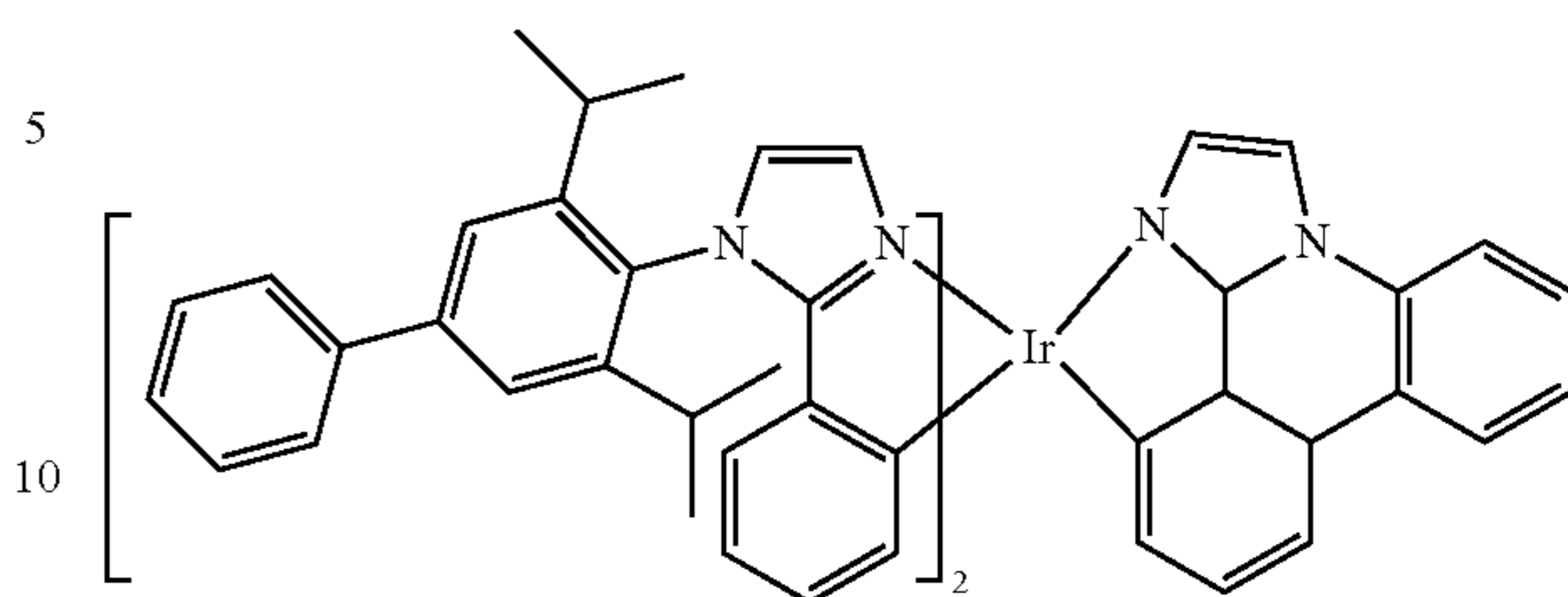
Compound 57
