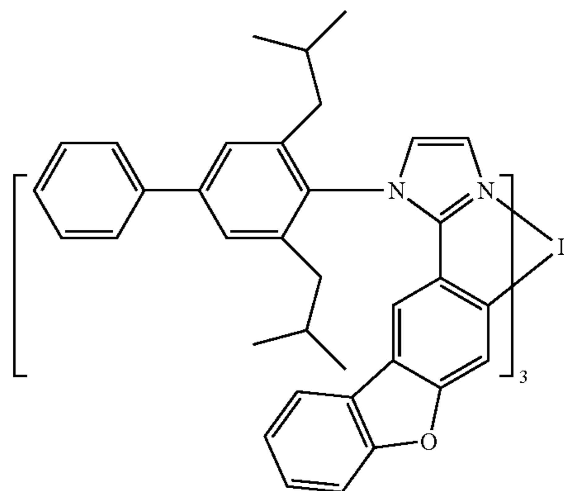
Compound 19
