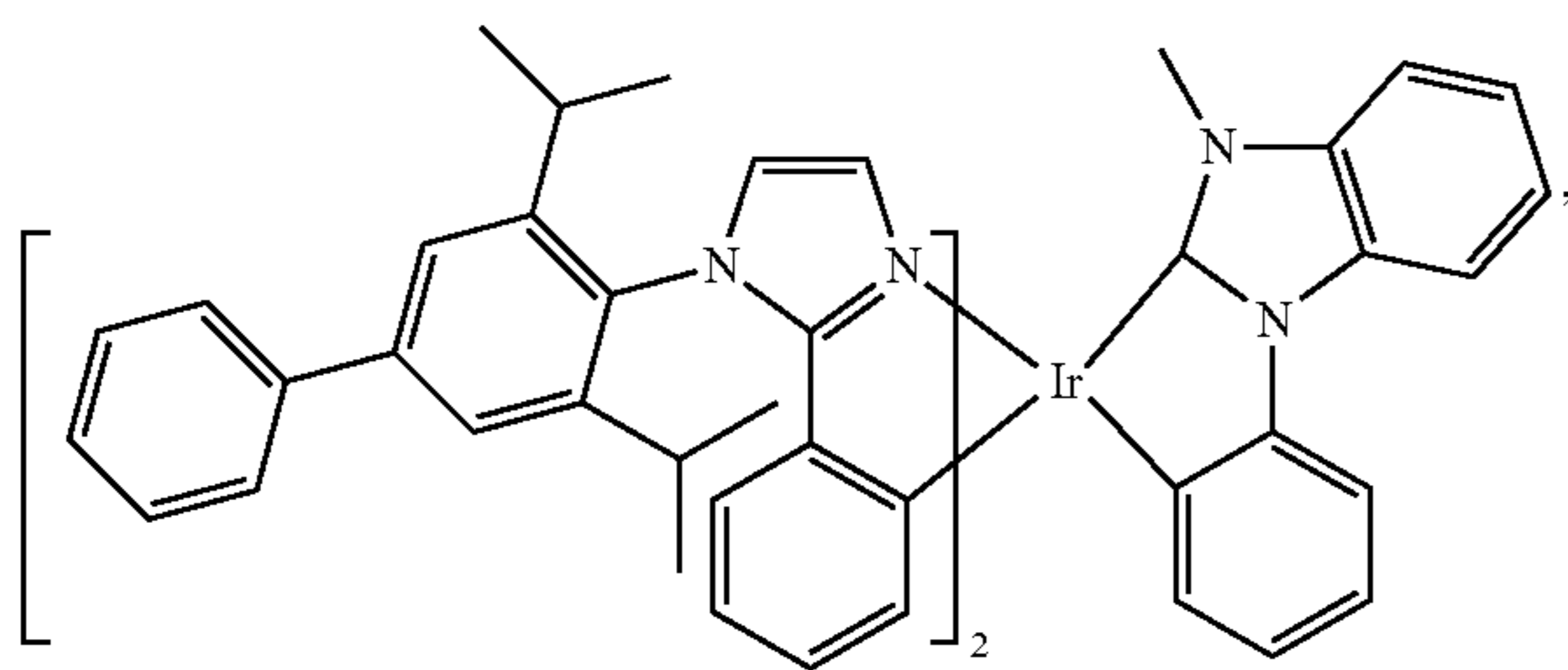
Compound 55
