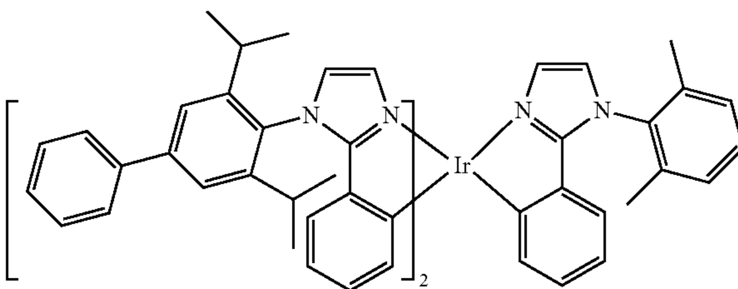
Compound 50
