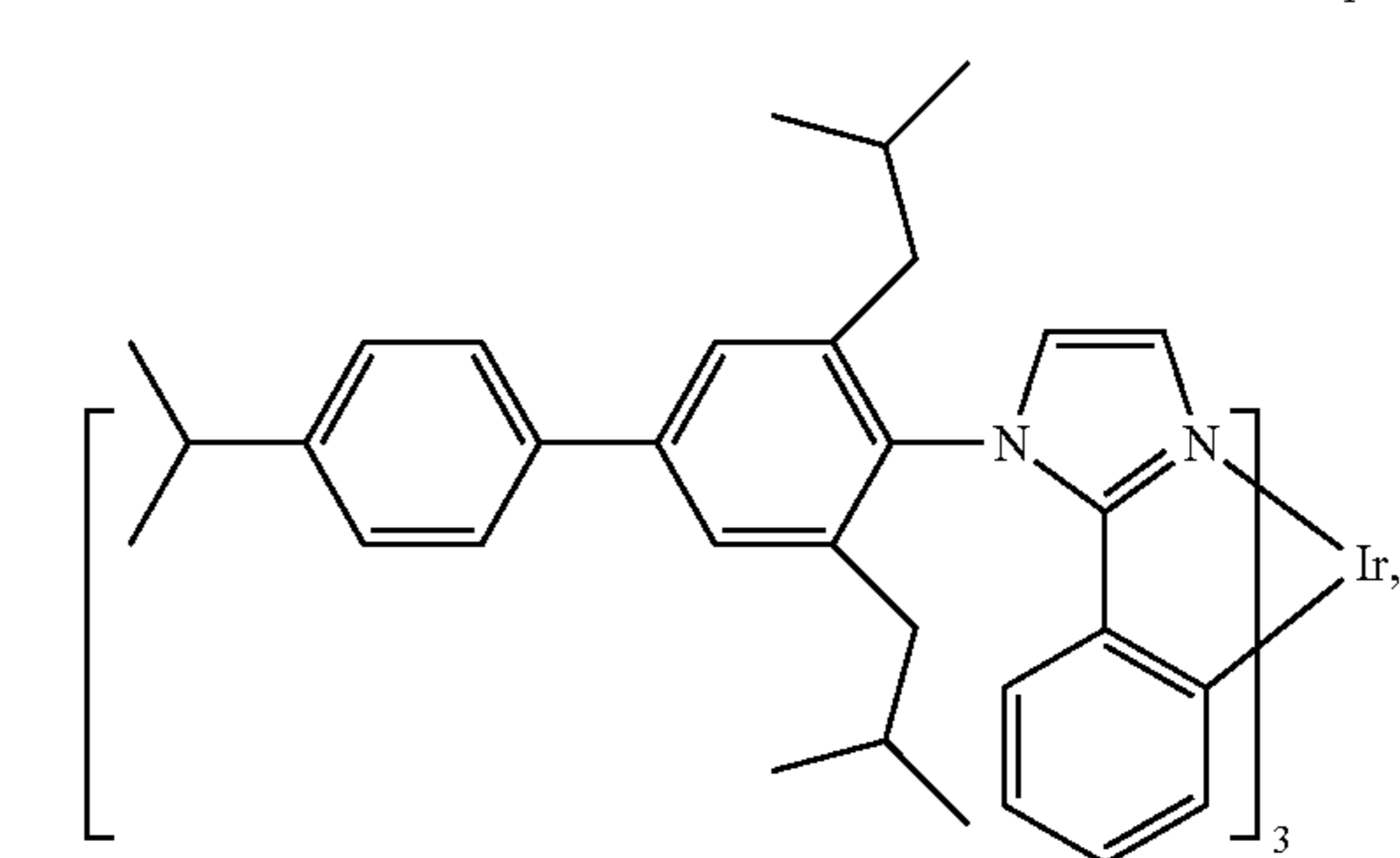
Compound 12
