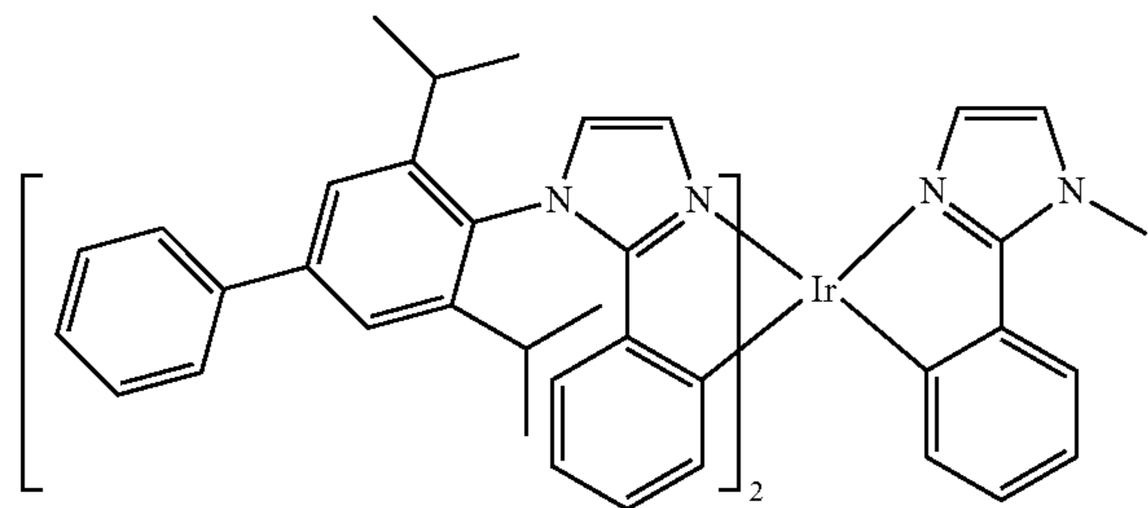
Compound 49
