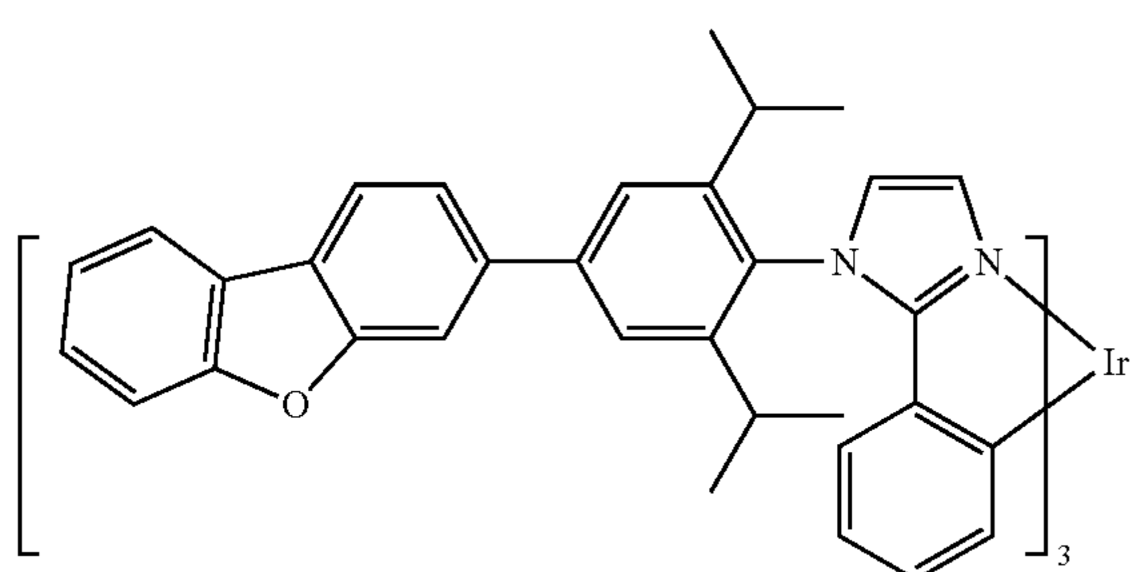
Compound 36
