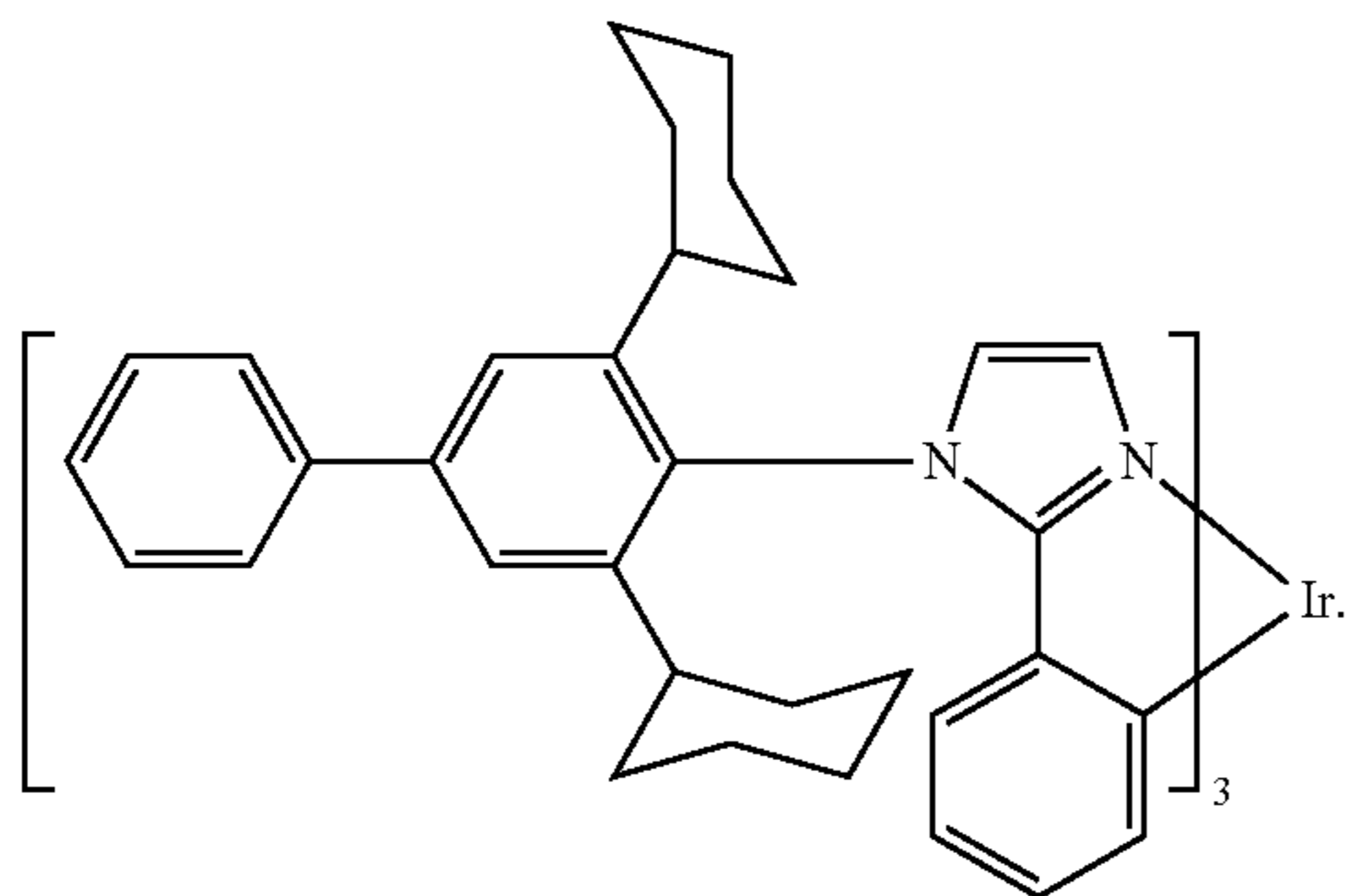
Compound 3
