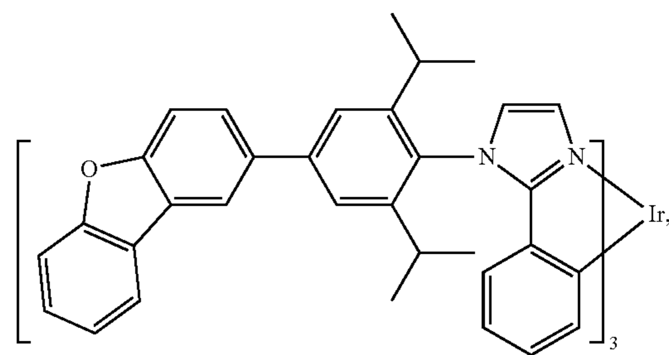
Compound 34
