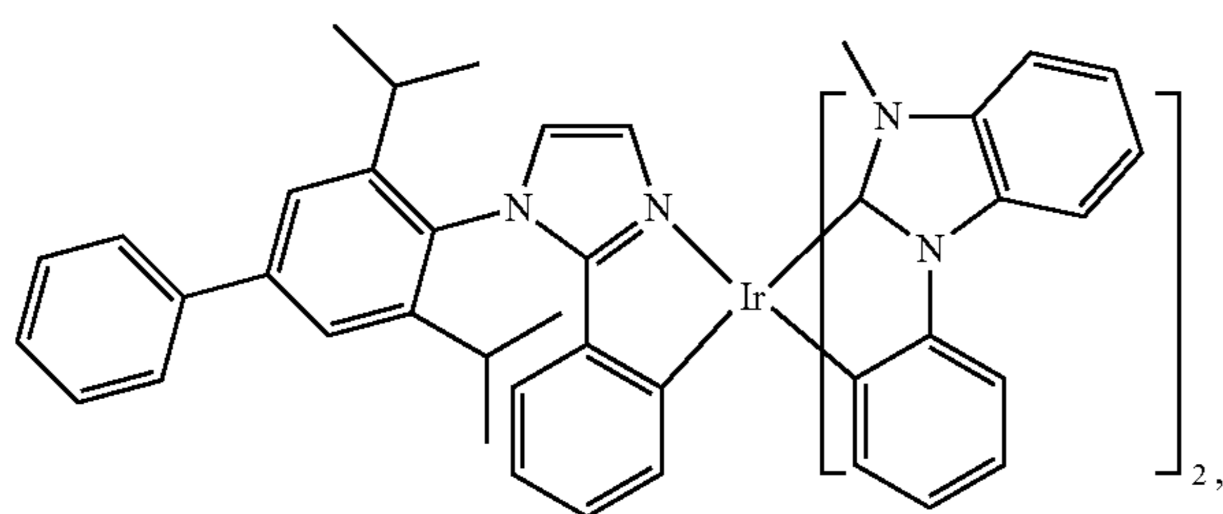
Compound 66
