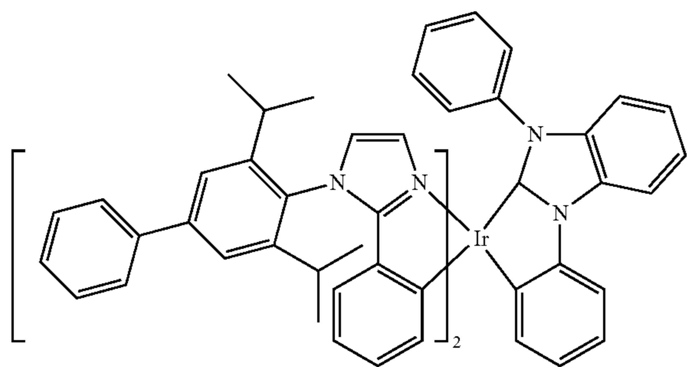
Compound 56
