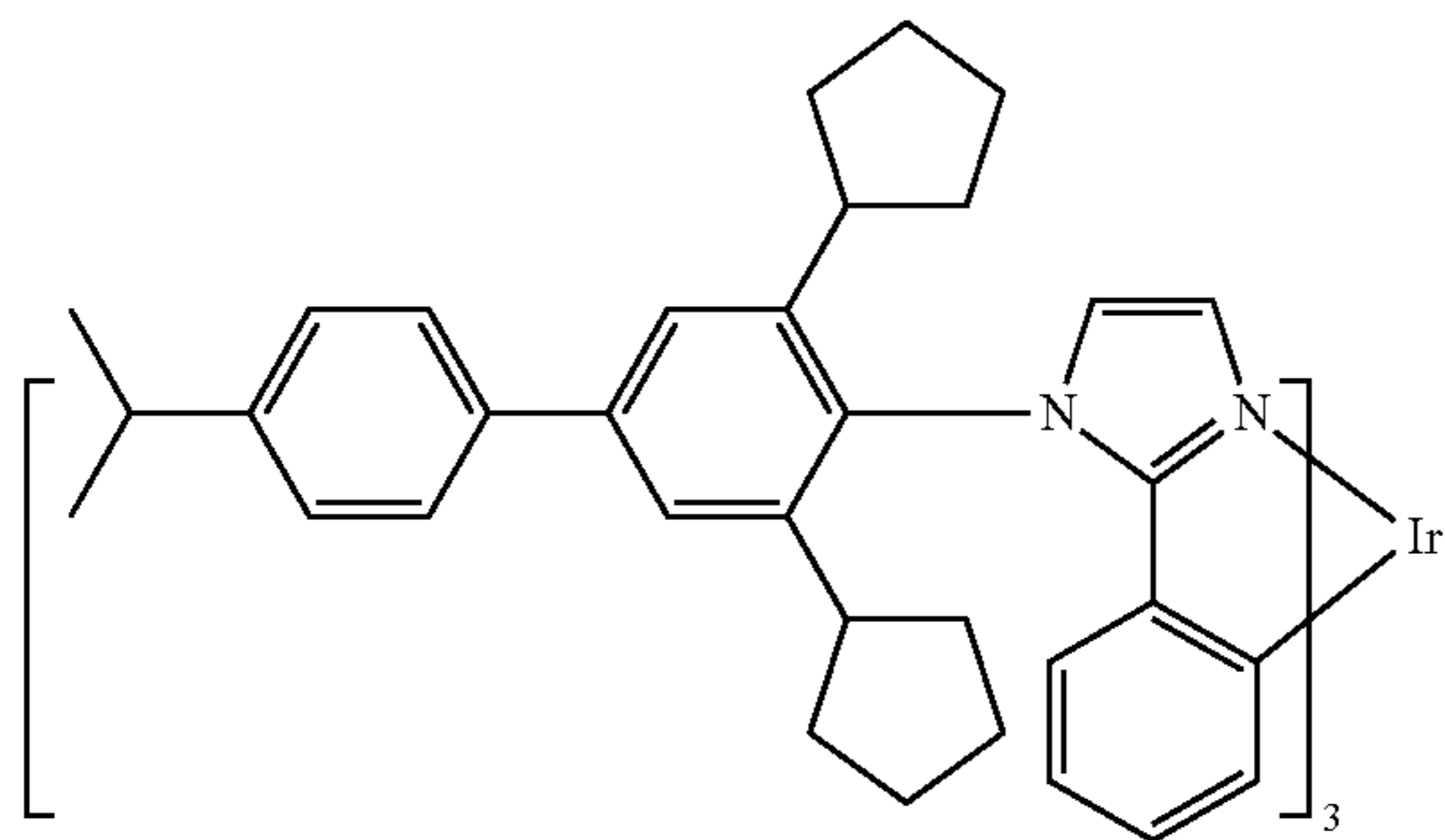
Compound 10
