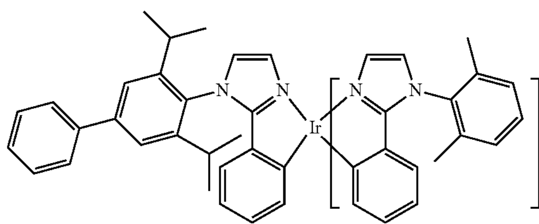
Compound 61
