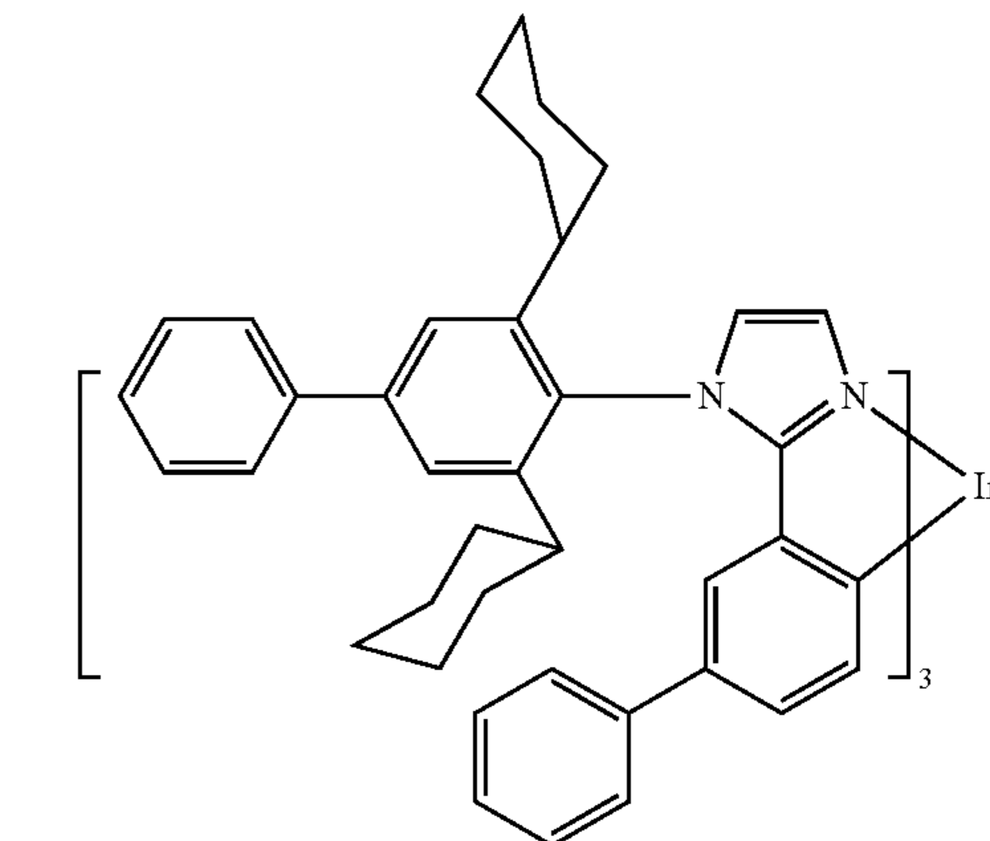
Compound 17
