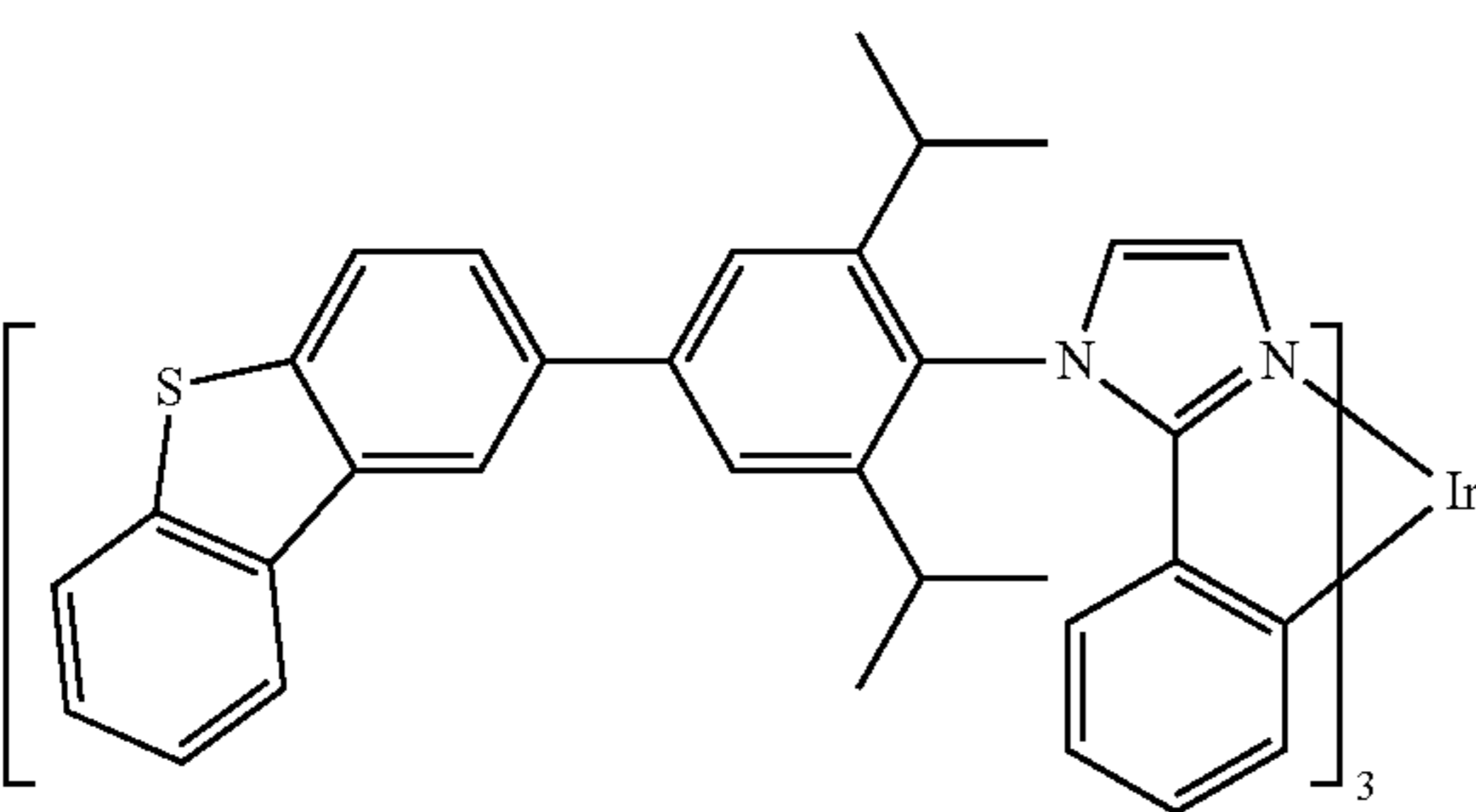
Compound 32
