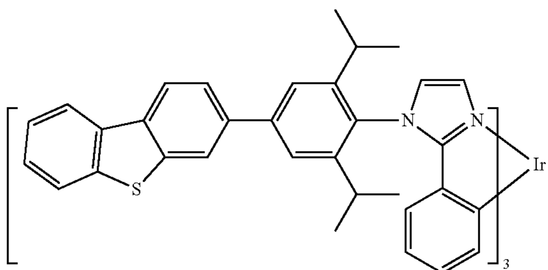
Compound 33
