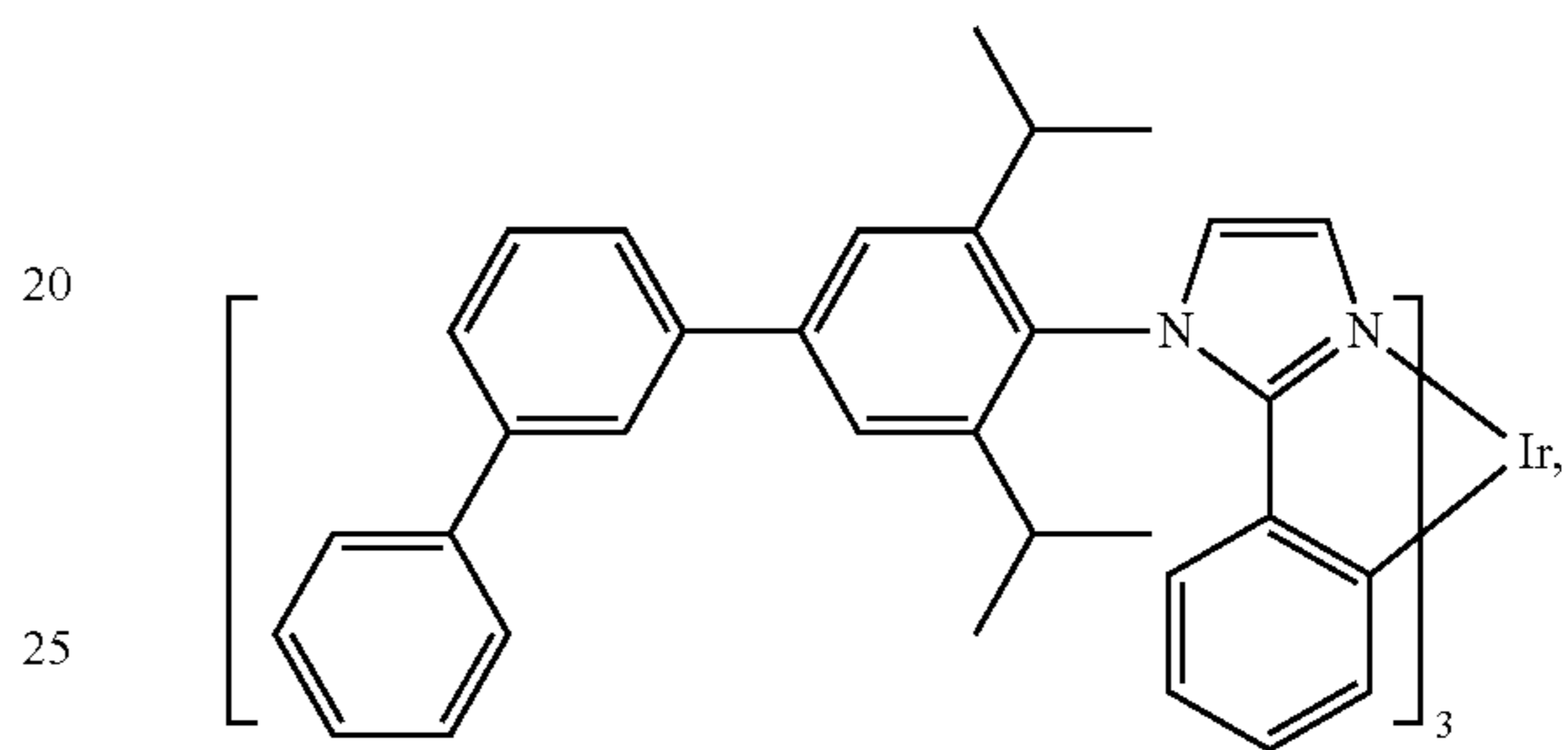
Compound 29
