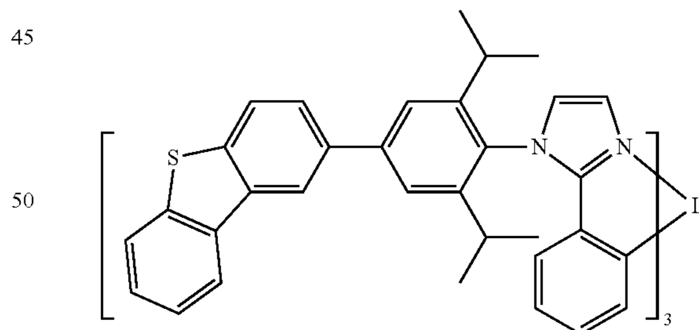
Compound 32
