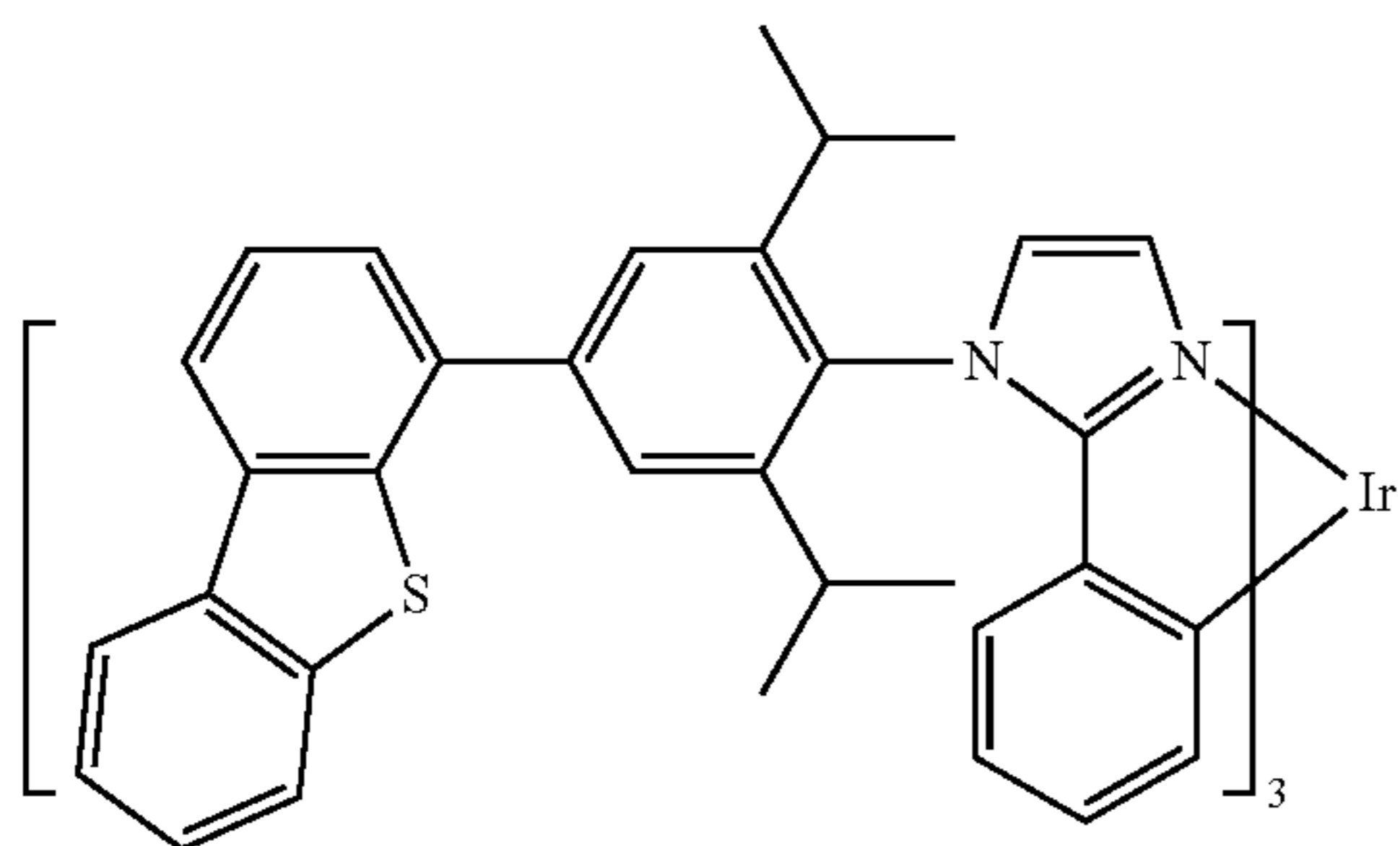
Compound 33
