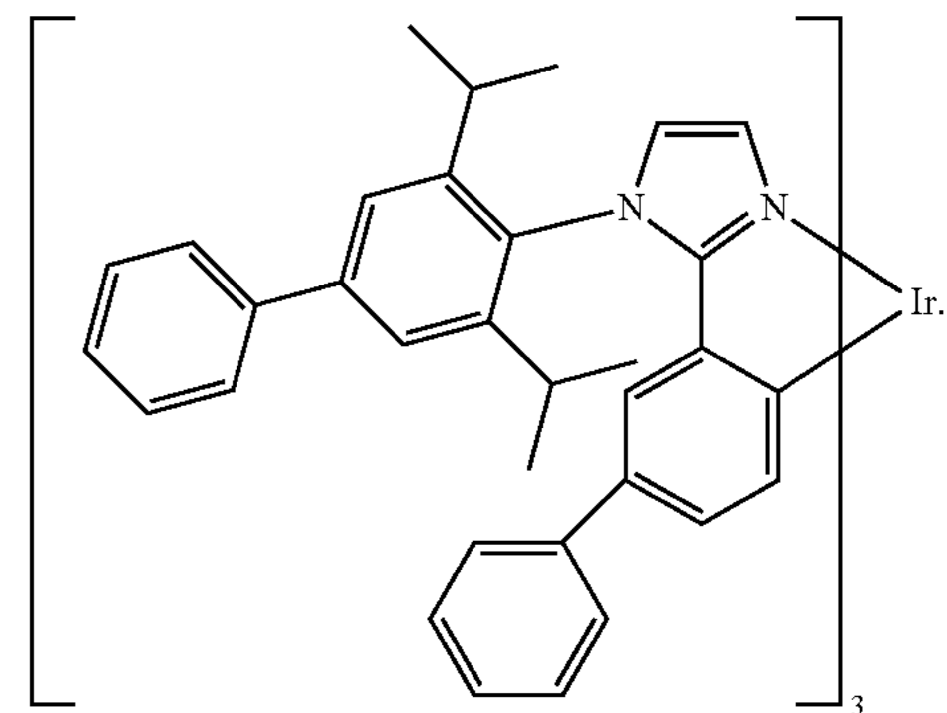
Compound 6
