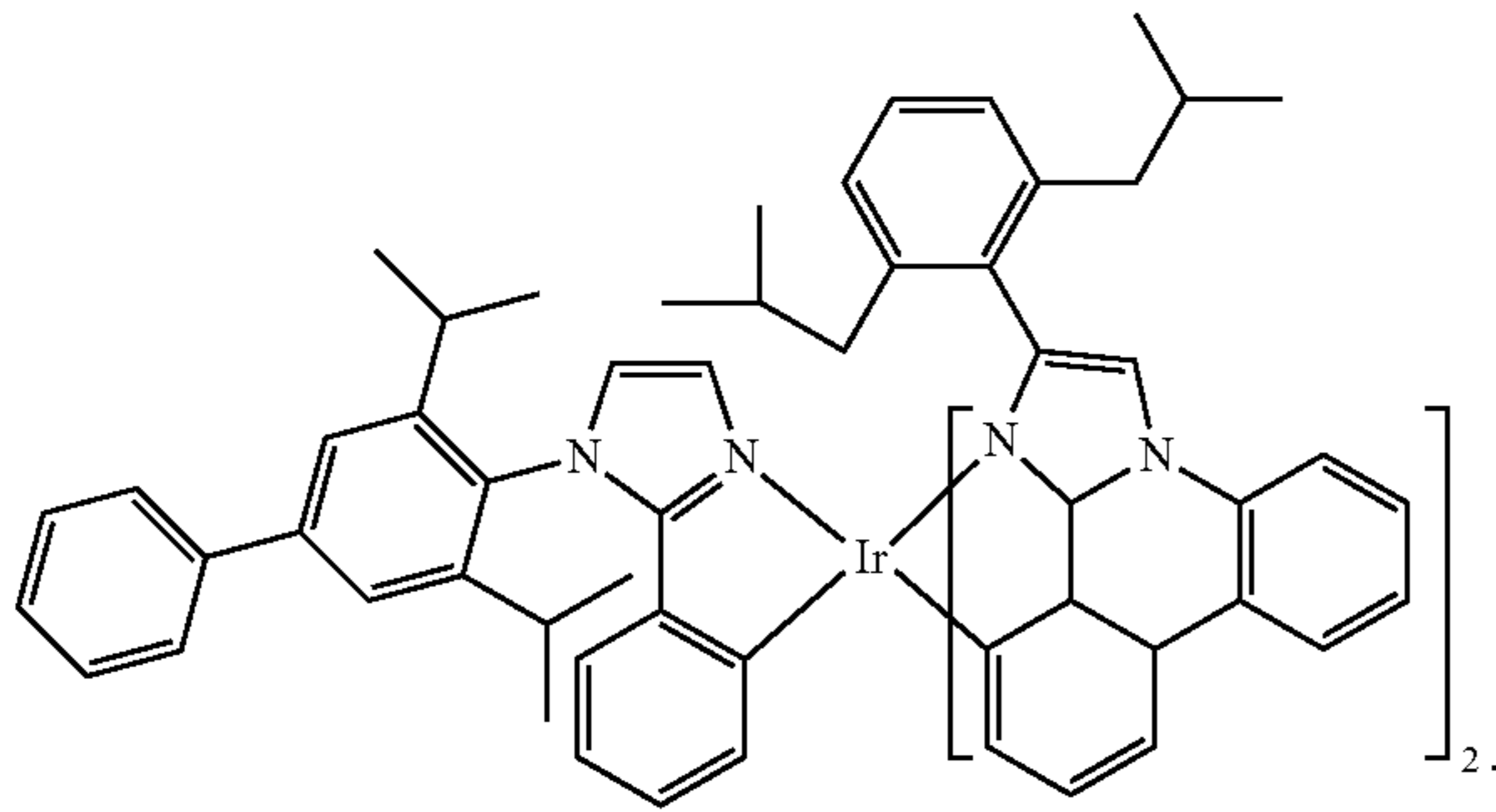
Compound 69
