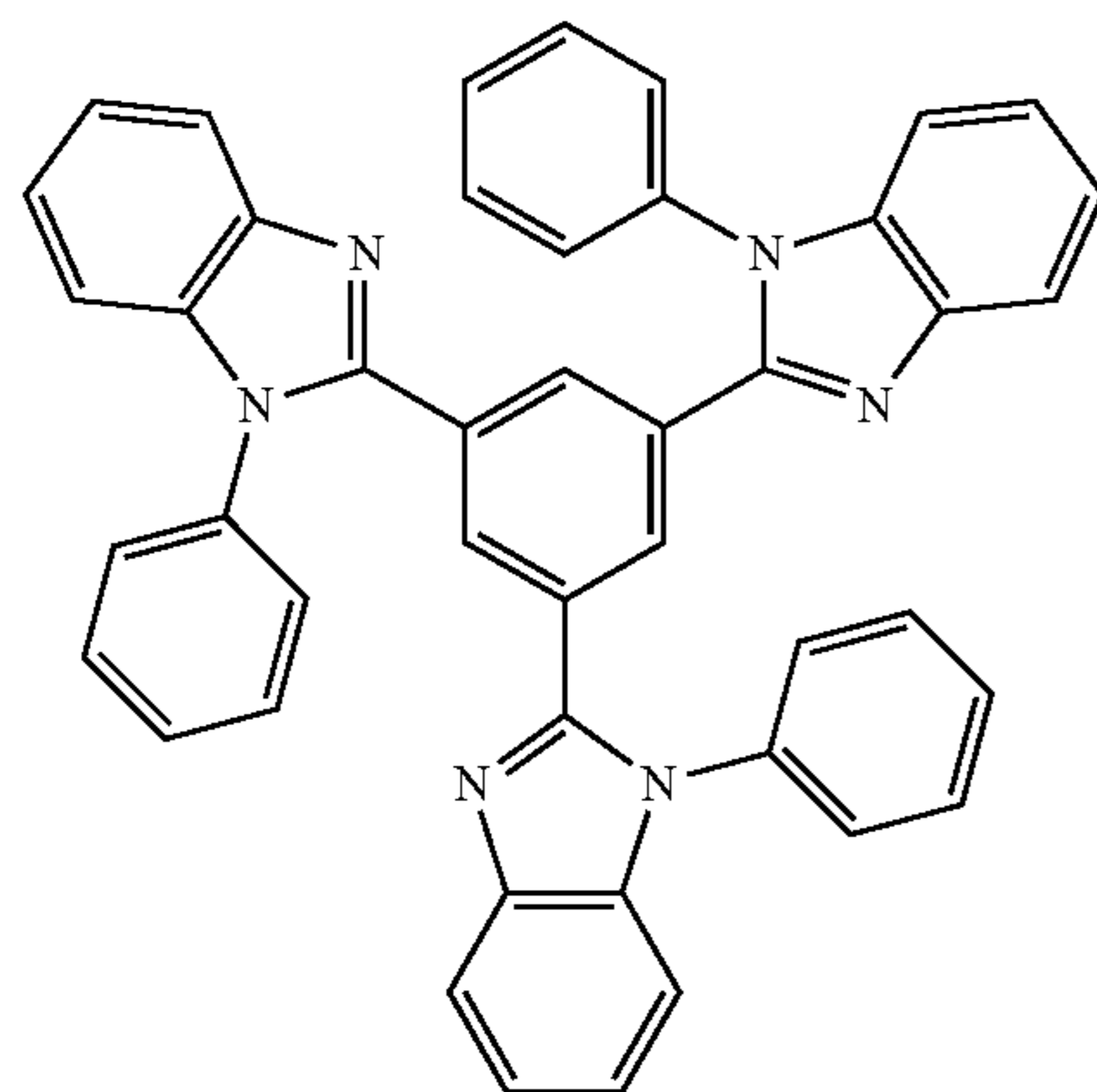
TPBi
