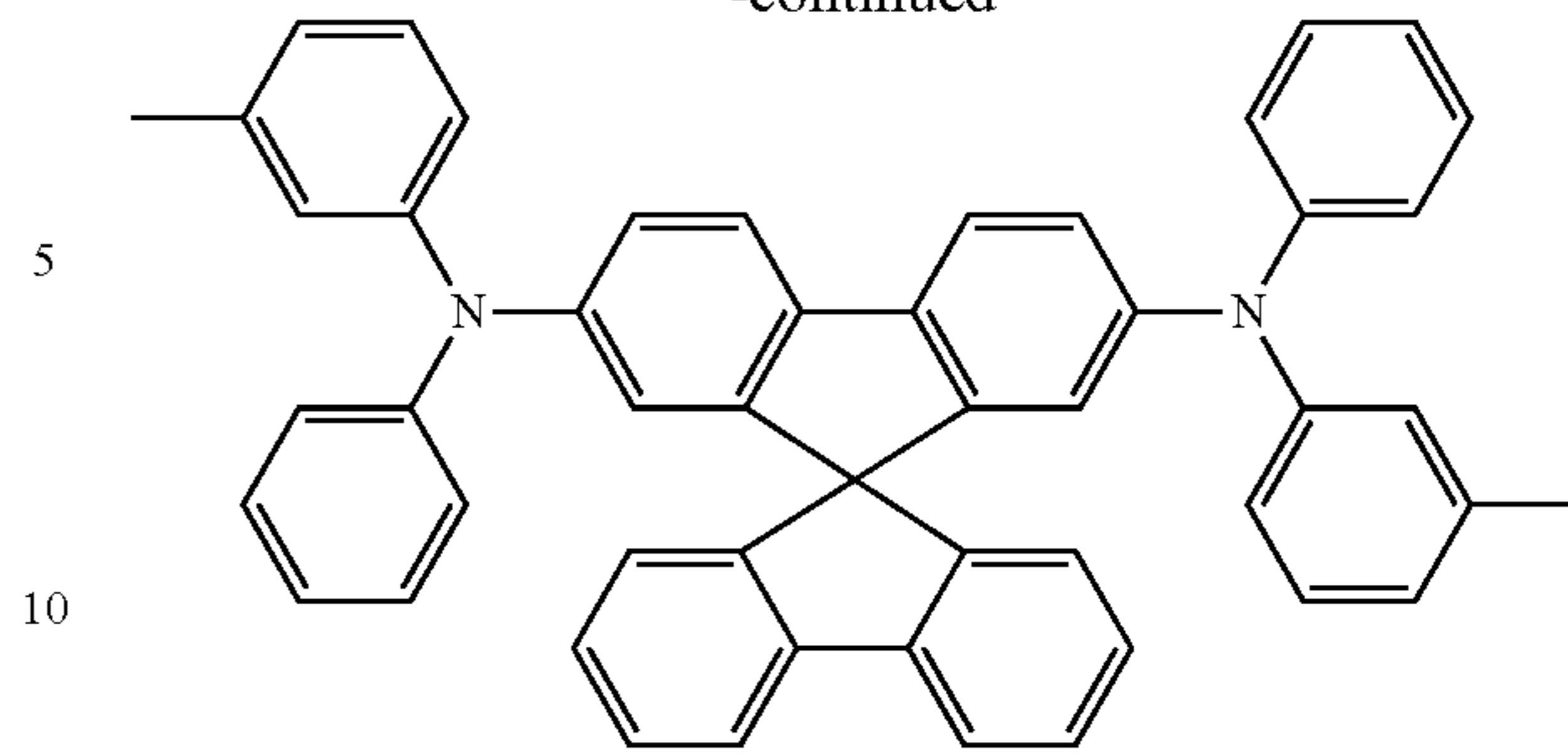
Spiro-TPD
