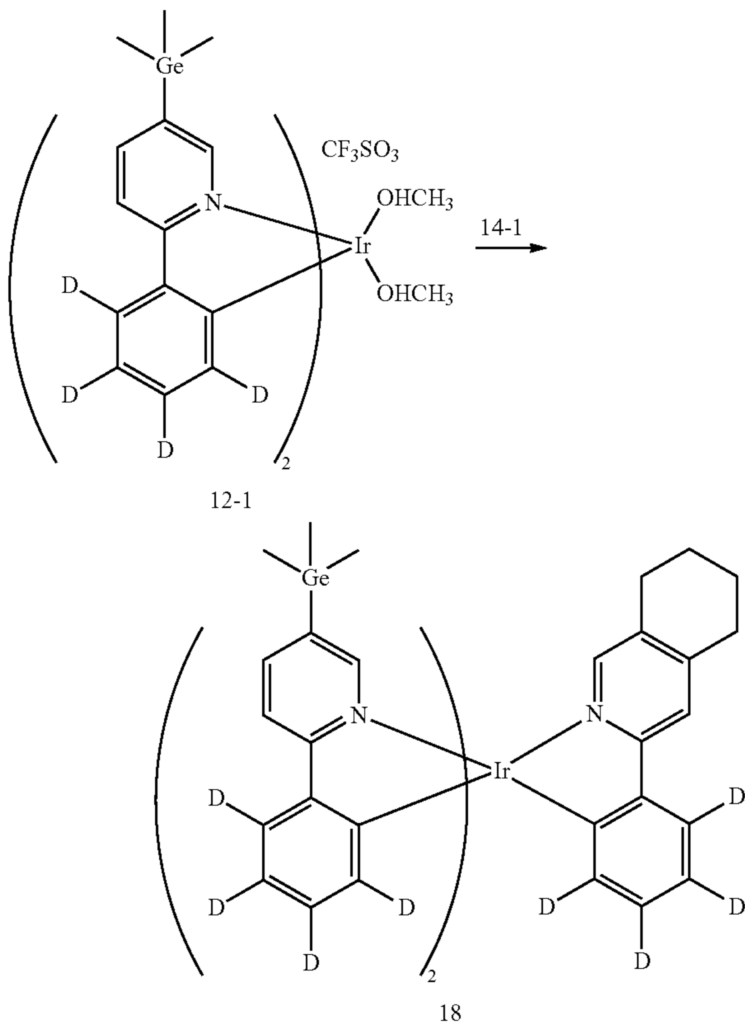
Reaction Scheme 18
