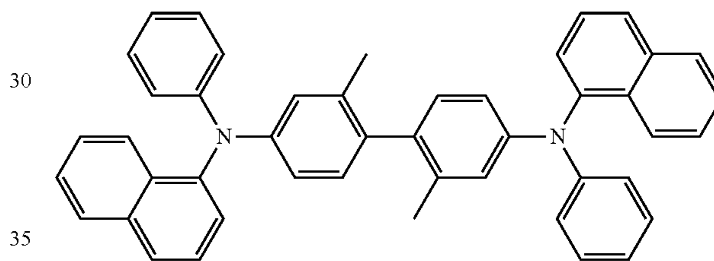
\alpha -NPB
