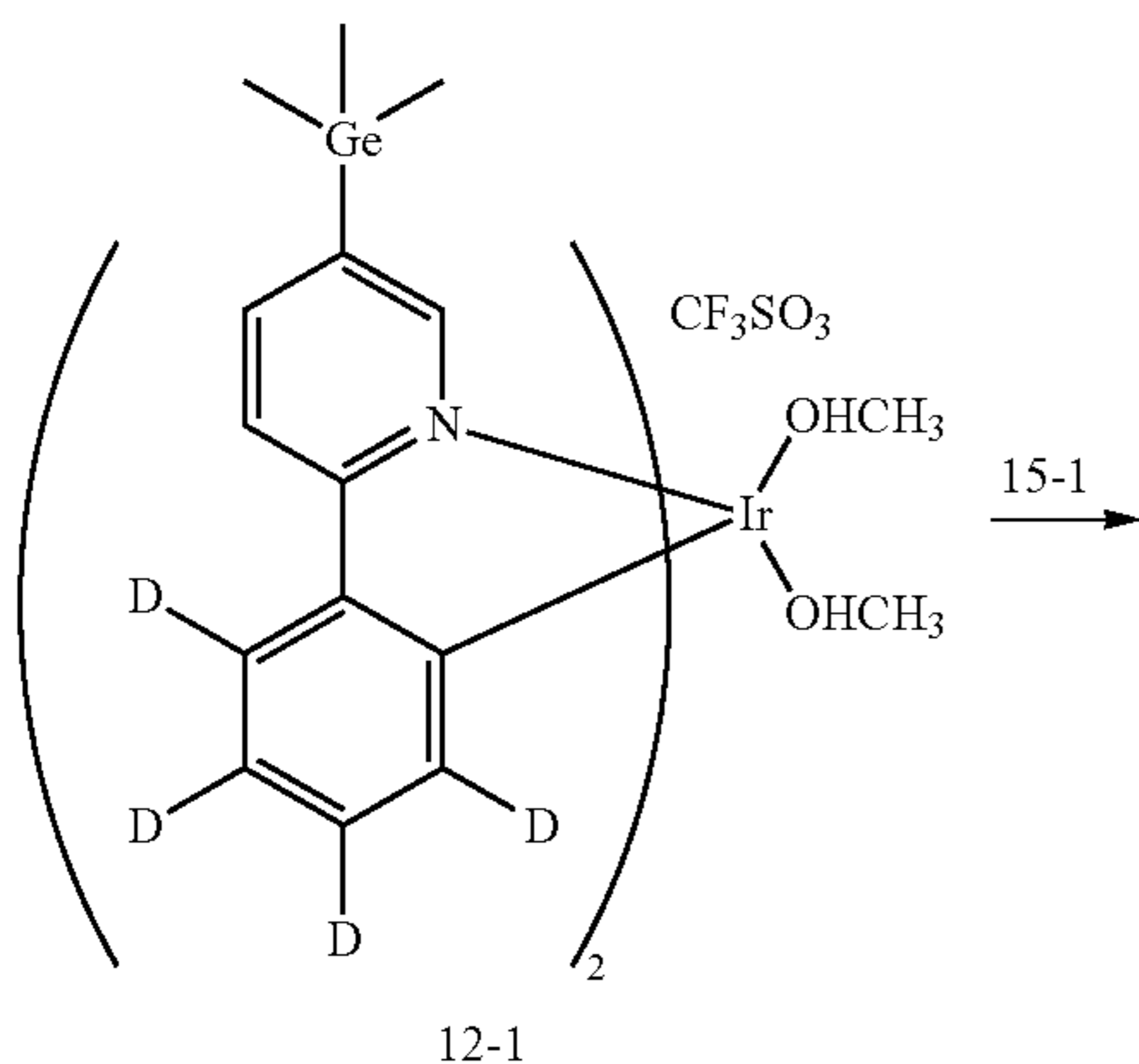
Reaction Scheme 19
