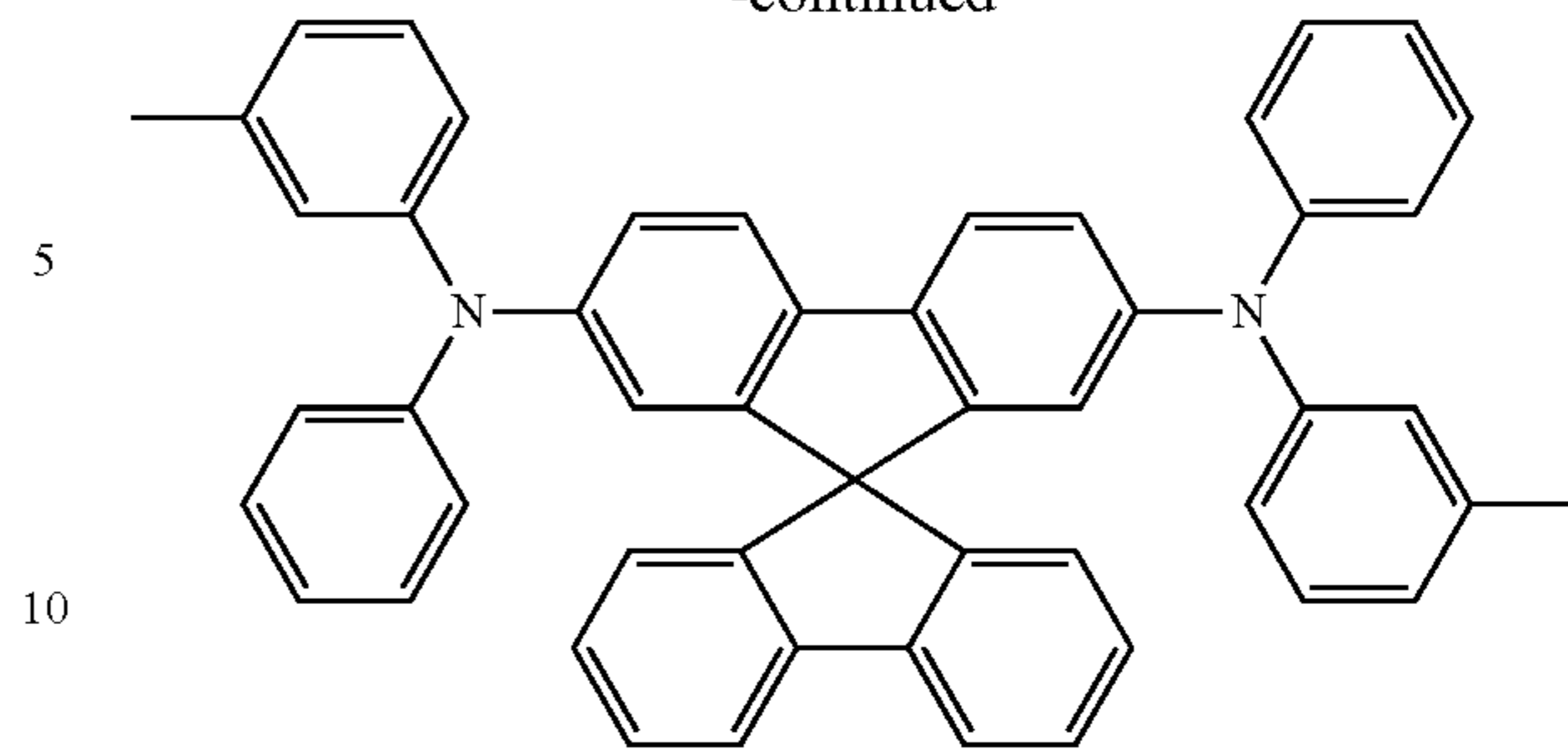
Spiro-TPD
