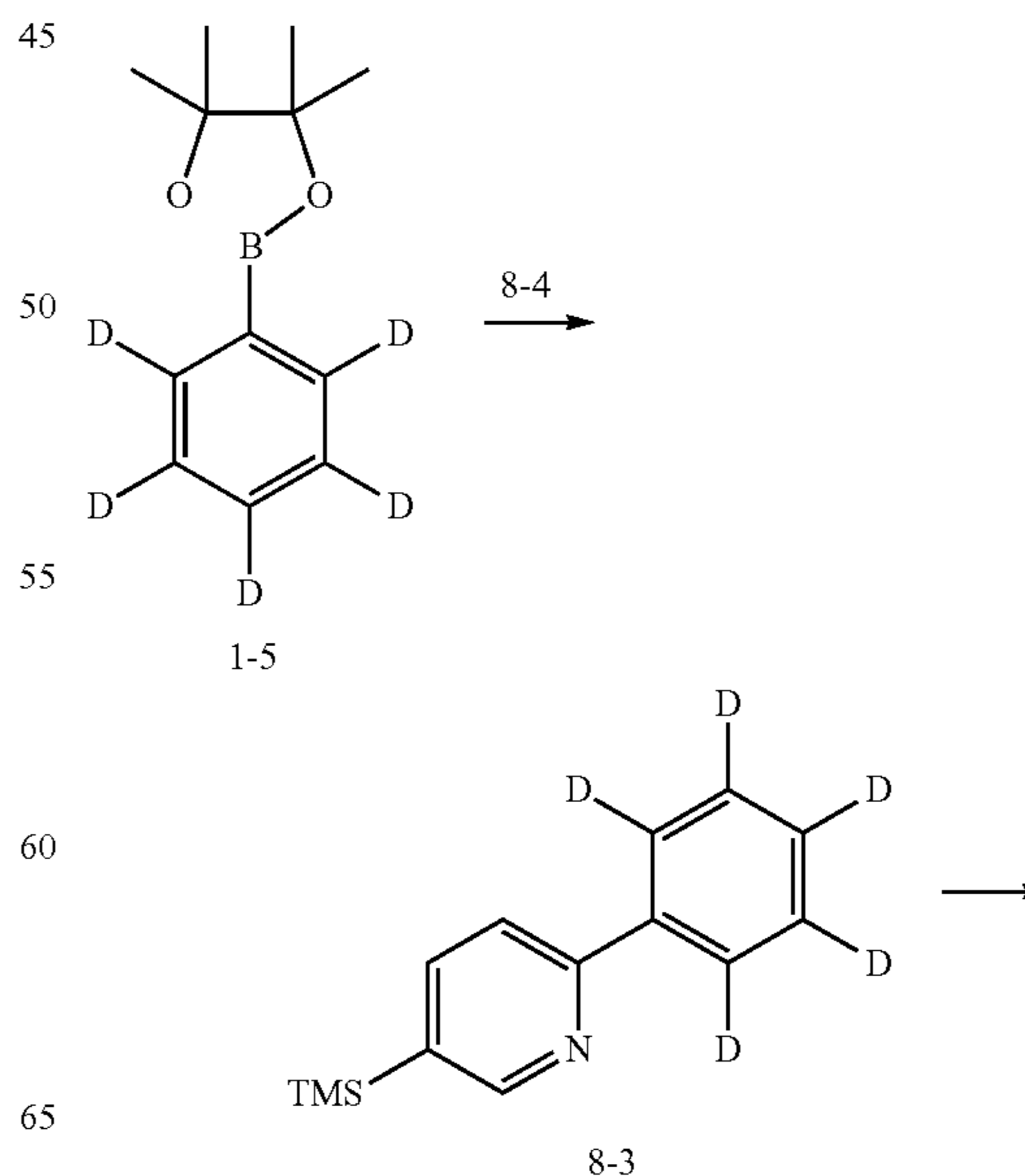
Reaction Scheme 8
