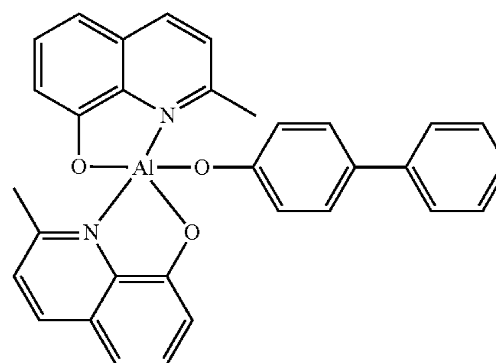
BAIq
