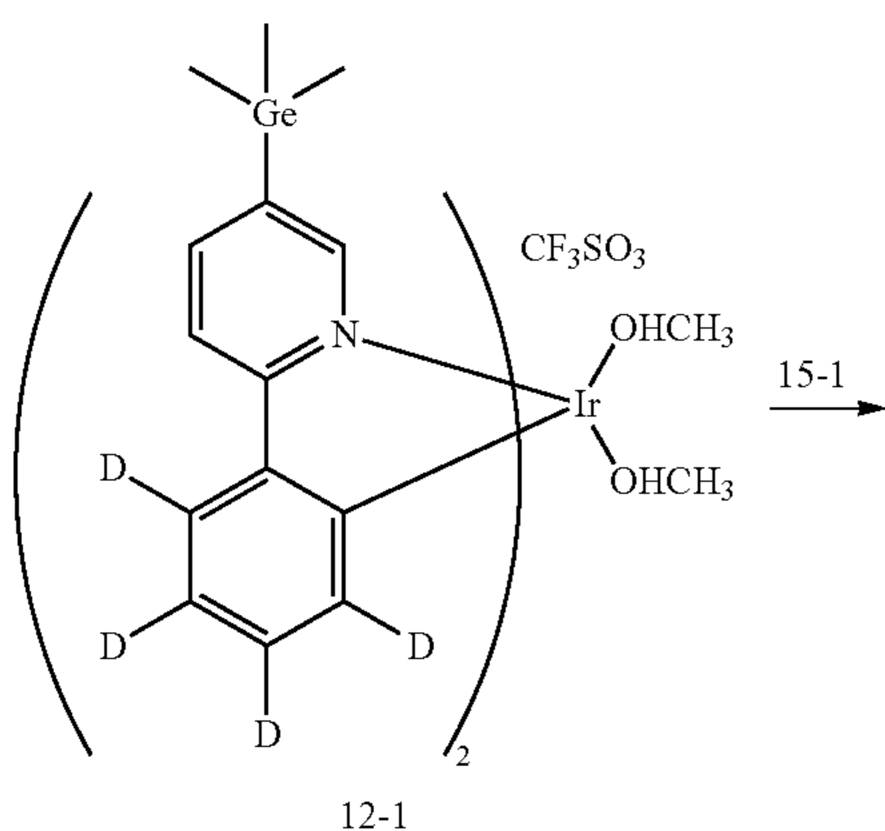
Reaction Scheme 19
