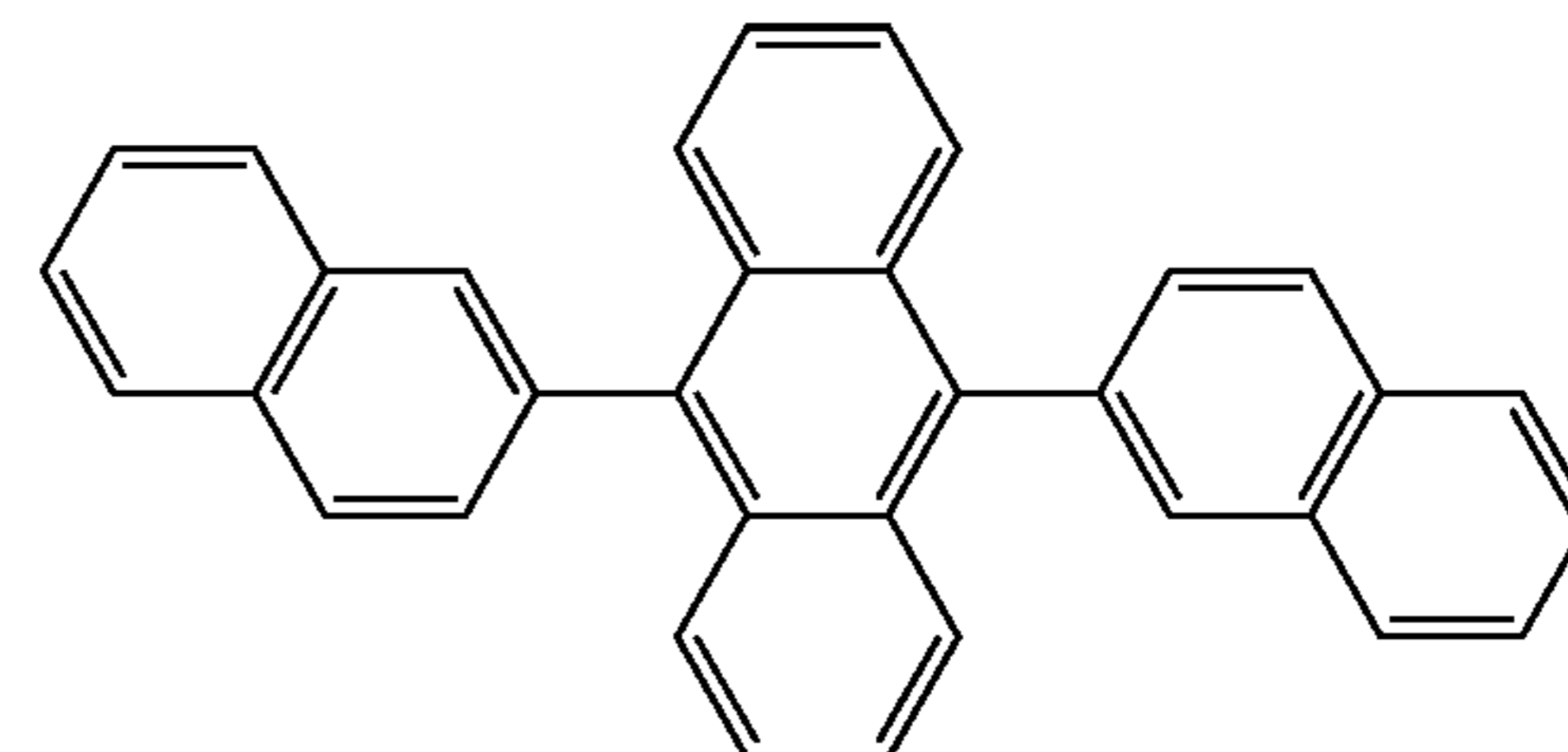
ADN
