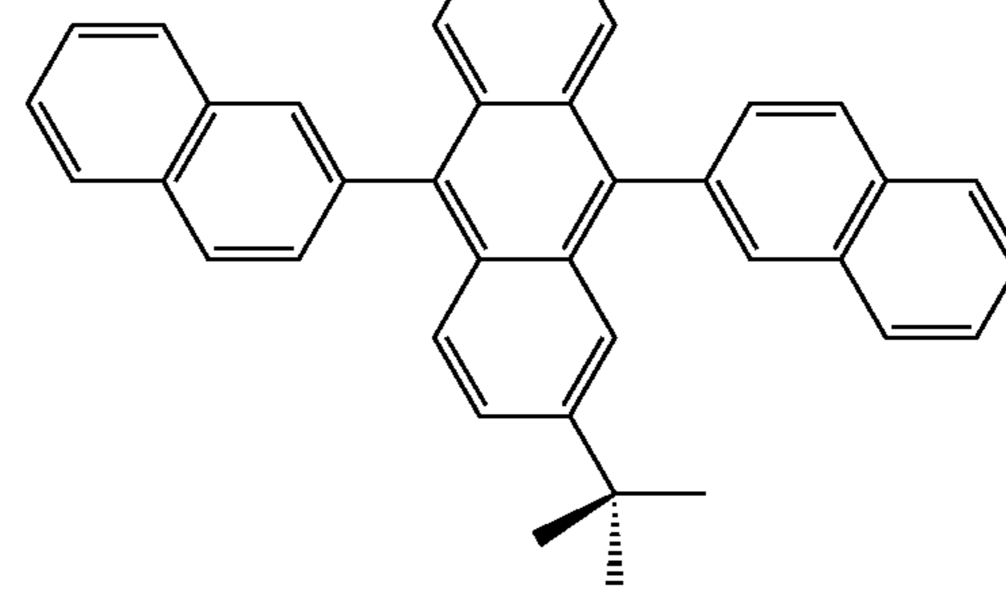
TBADN
