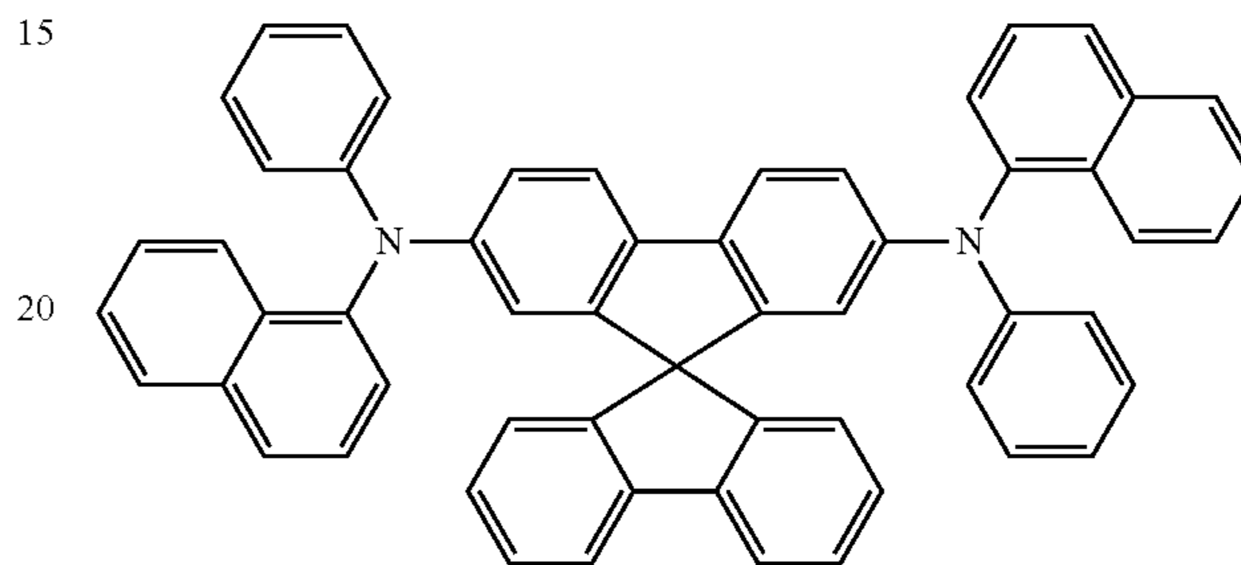
Spiro-NPB
