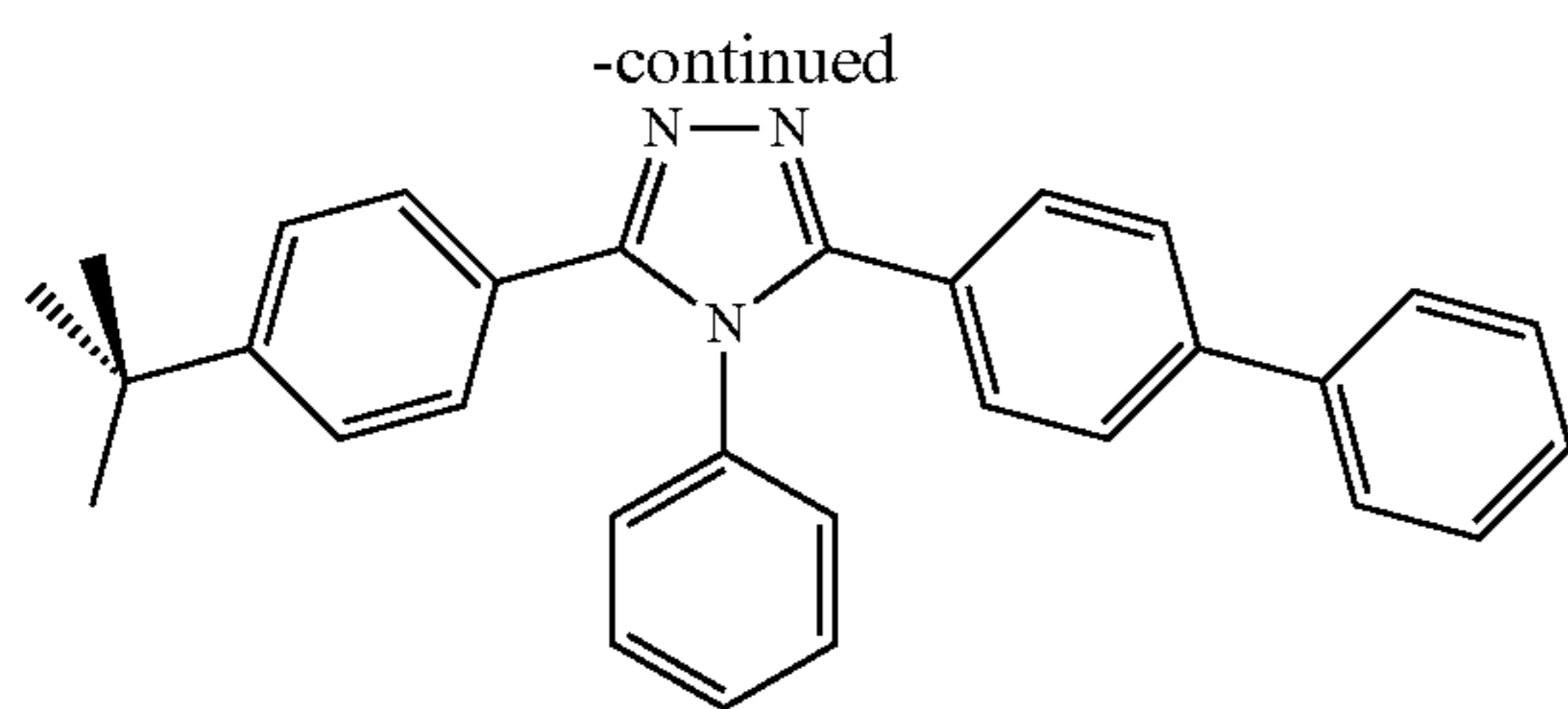
TAZ
