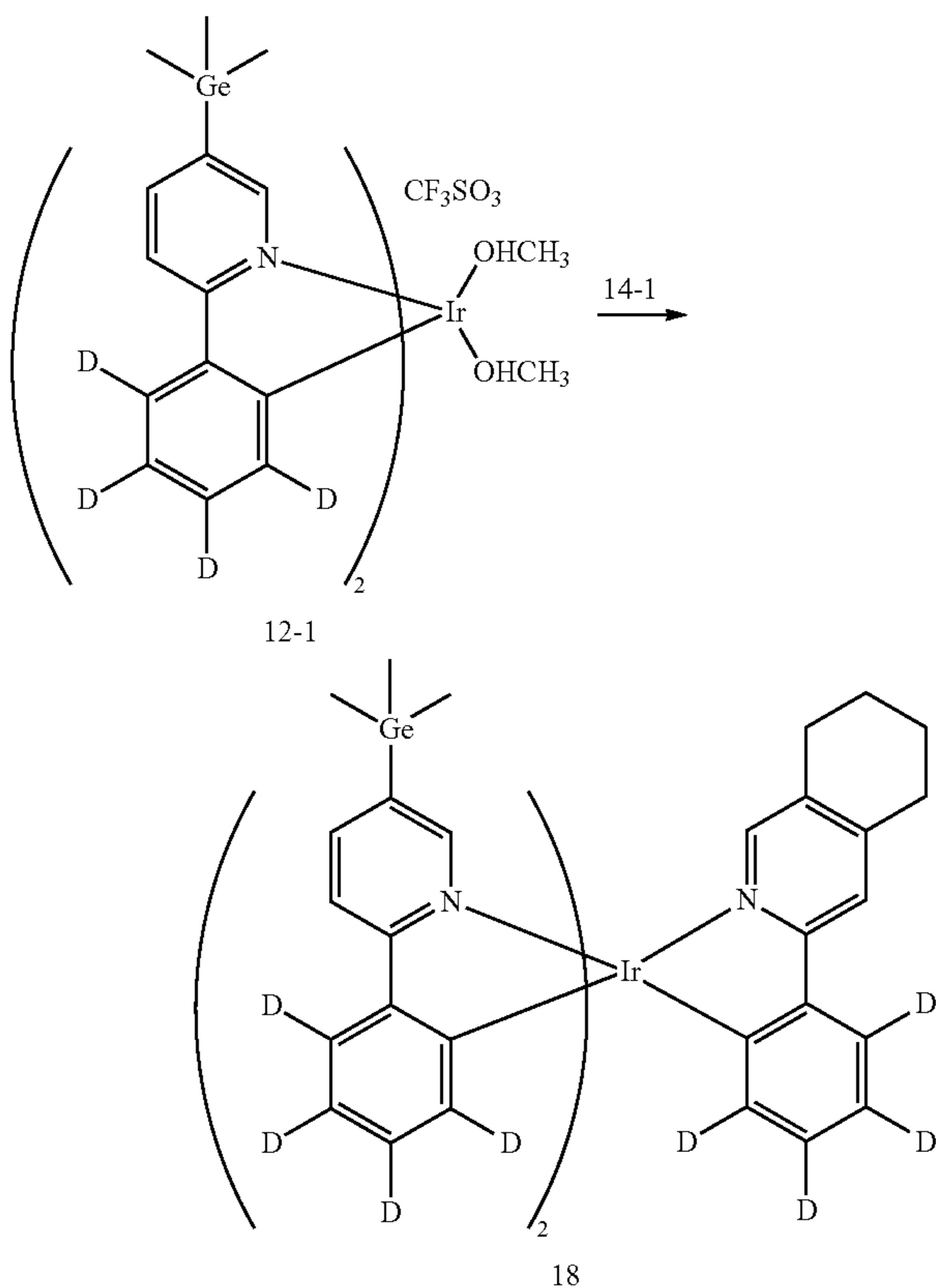
Reaction Scheme 18
