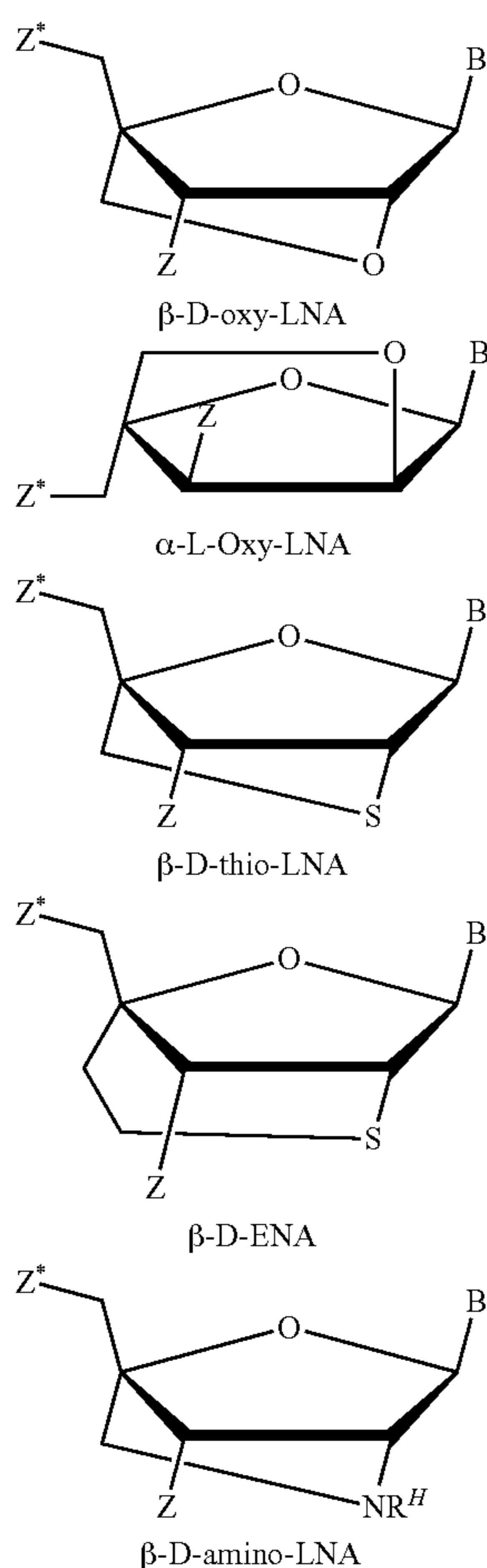
Scheme 2
