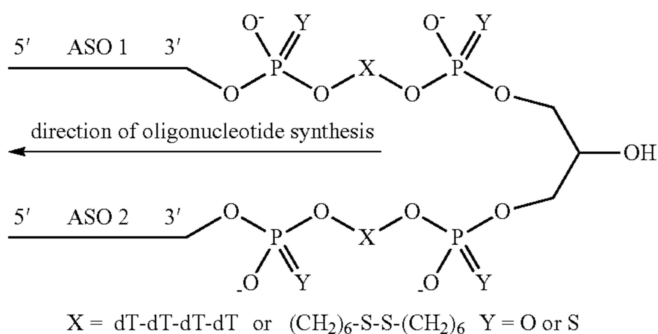
Formula VIII
