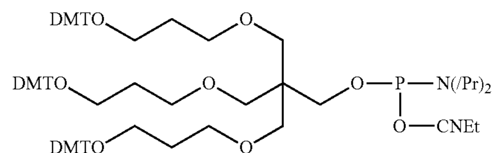
Formula X
