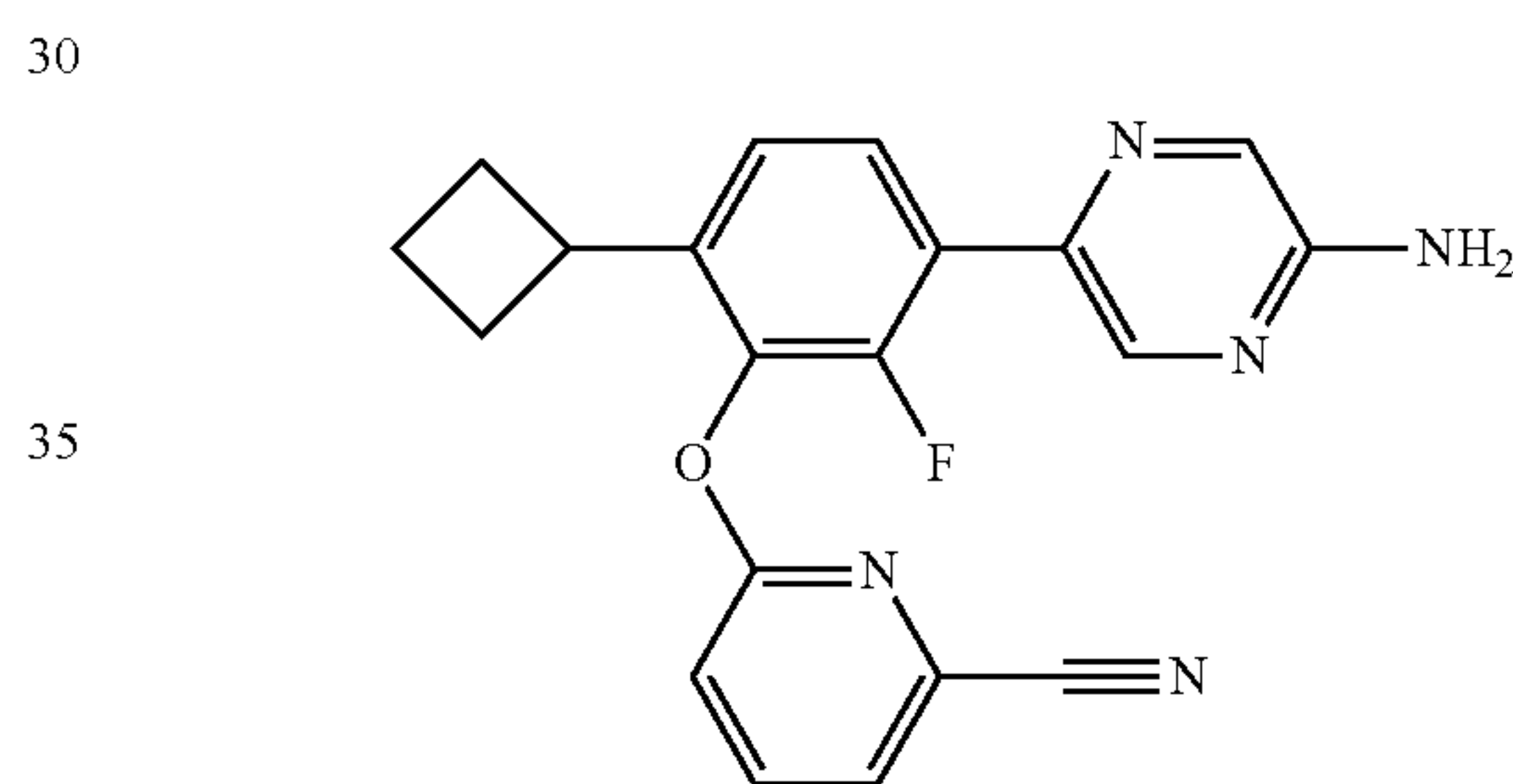
6-[3-(5-Aminopyrazin-2-yl)-6-cyclobutyl-2-fluorophenoxy]pyridine-2-carbonitrile
