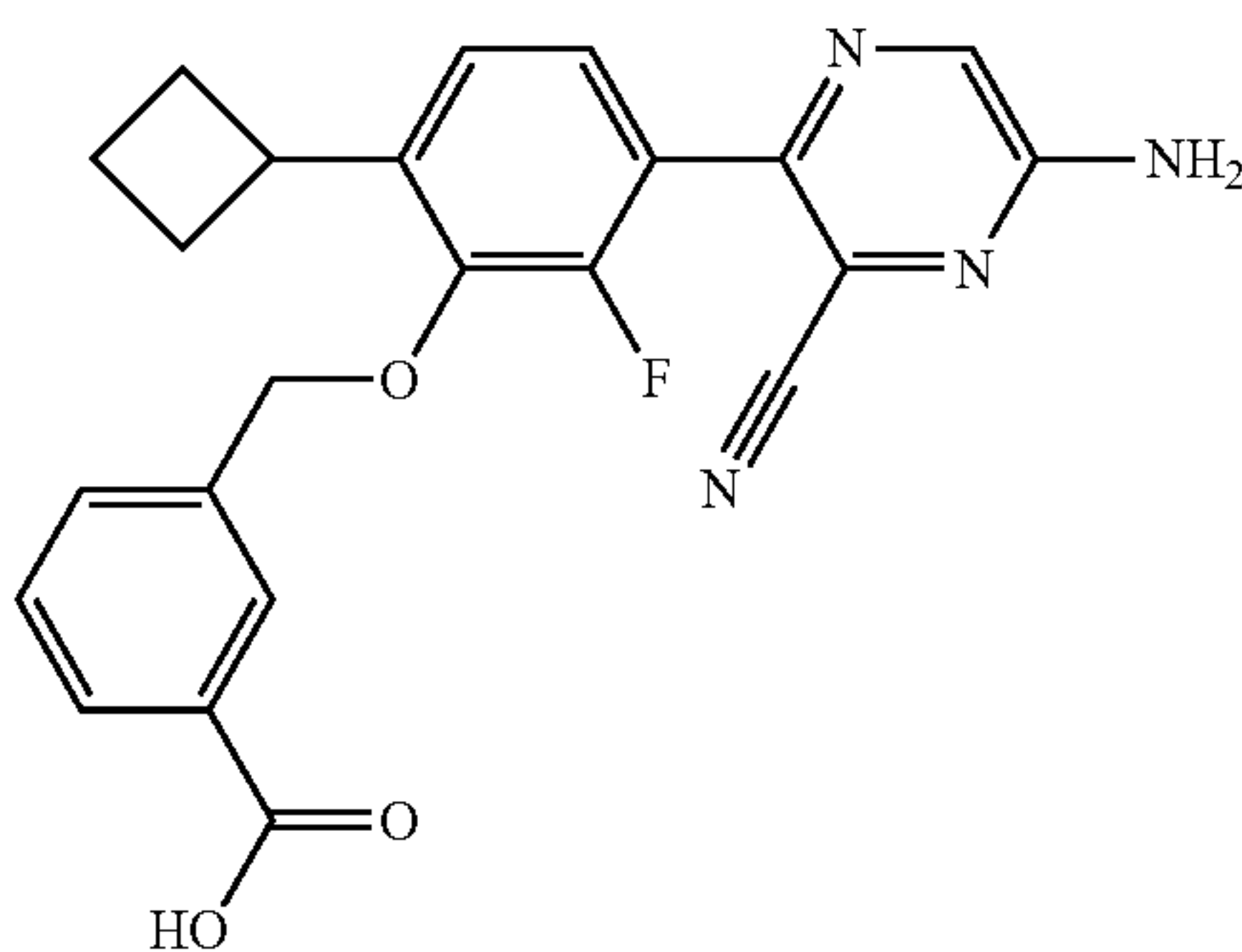
3-{[3-(5-Amino-3-cyanopyrazin-2-yl)-6-cyclobutyl- 2-fluorophenoxy]methyl}benzoic acid
