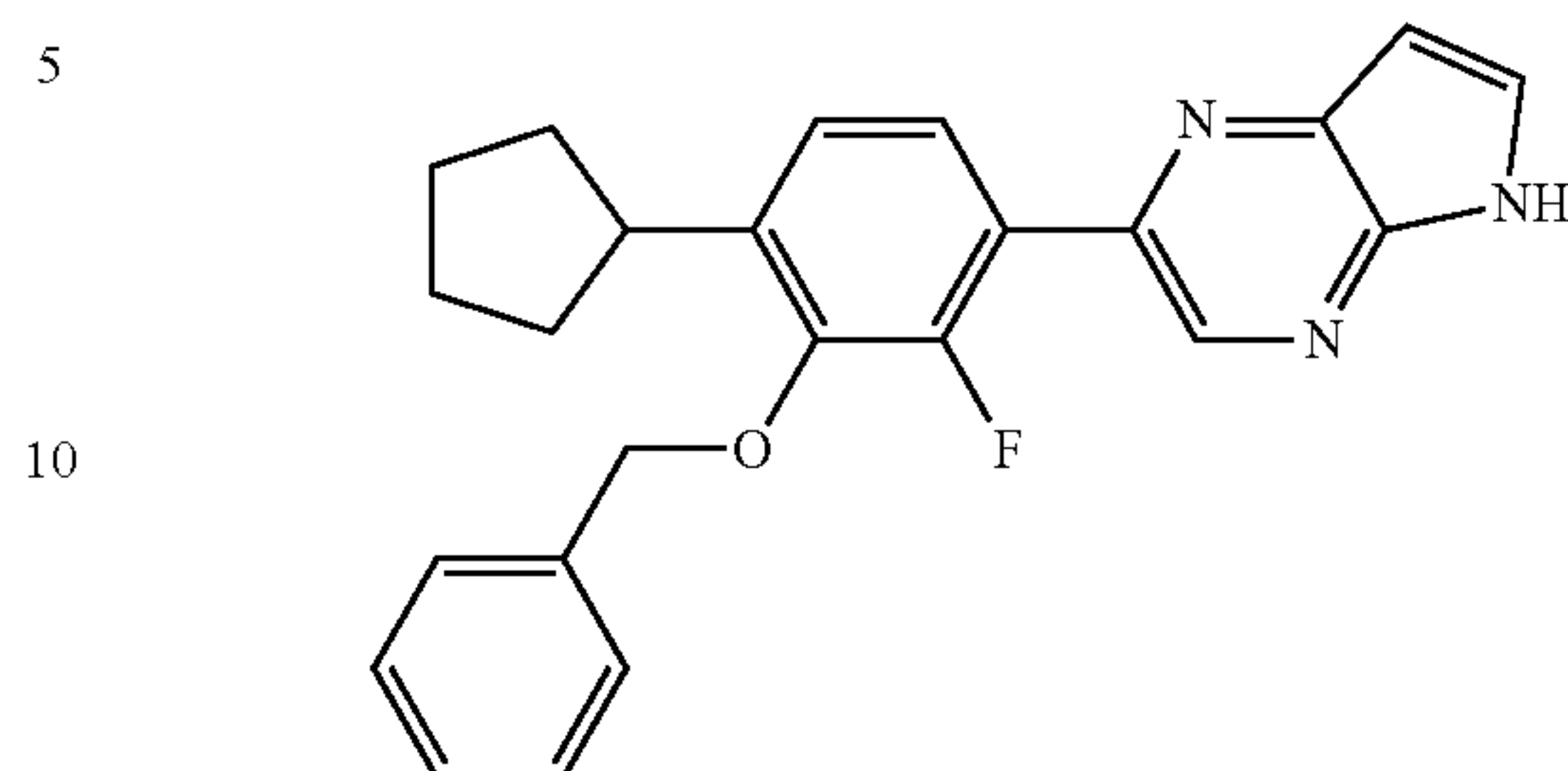
2-[3-(Benzyloxy)-4-cyclopentyl-2-fluorophenyl]- 5H-pyrrolo[2,3-b]pyrazine
