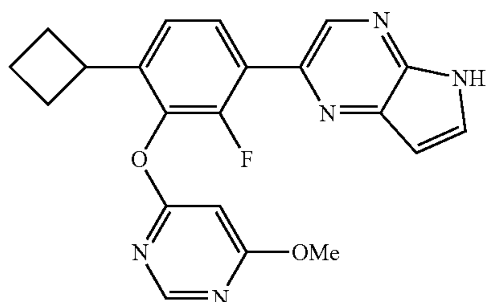
2-(4-Cyclobutyl-2-fluoro-3-((6-methoxypyrimidin-4-yl)oxy)phenyl)-5H-pyrrolo[2,3-b]pyrazine
