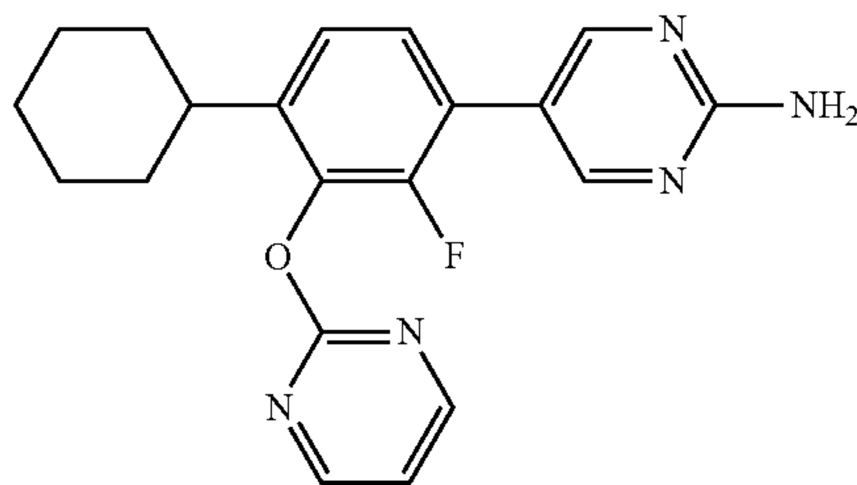
5-[4-Cyclohexyl-2-fluoro-3-(pyrimidin-2-yloxy)phenyl]pyrimidin-2-amine
