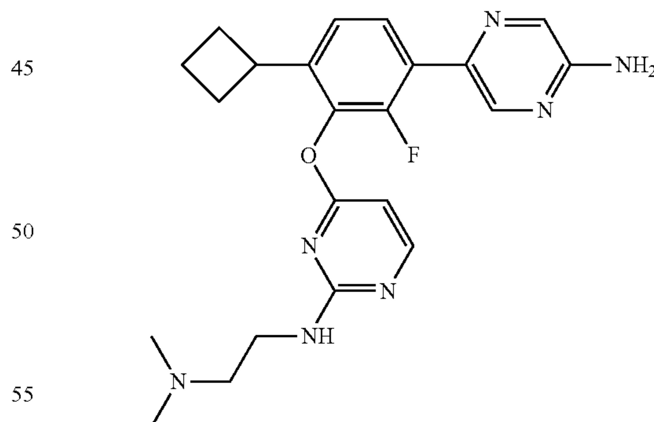
N'-{4-[3-(5-Aminopyrazin-2-yl)-6-cyclobutyl-2-fluorophenoxy]pyrimidin-2-yl}-N, N-dimethylethane-1,2-diamine hydrochloride
