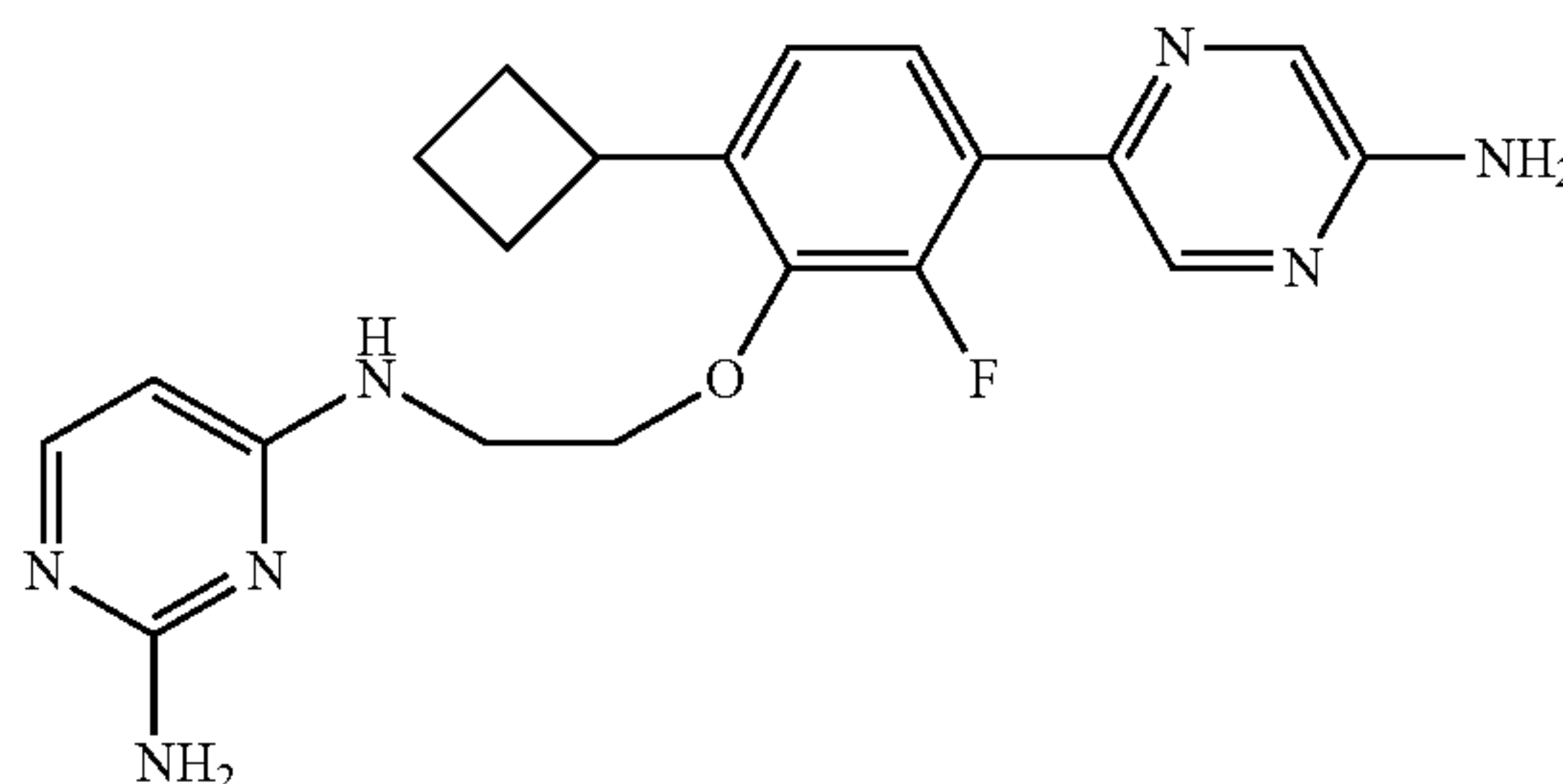
N'-(2-(3-(5-Aminopyrazin-2-yl)-6-cyclobutyl-2-fluorophenoxy)ethyl)pyrimidine-2,4-diamine
