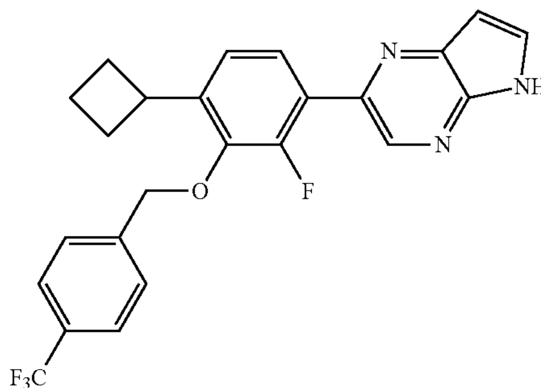
2-(4-Cyclobutyl-2-fluoro-3-{[4-(trifluoromethyl) benzyl]oxy}phenyl)-5H-pyrrolo[2,3-b]pyrazine trif- luoroacetate salt
