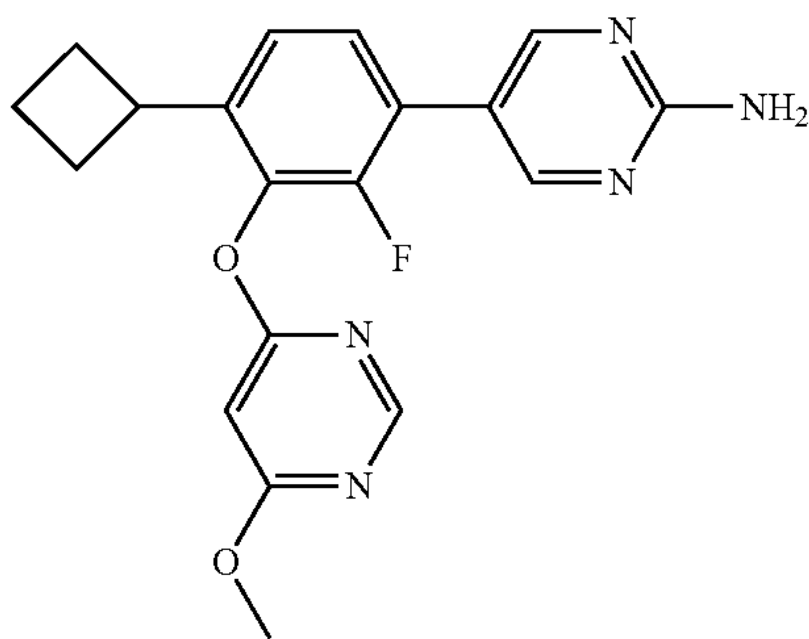
5-(4-cyclobutyl-2-fluoro-3-((6-methoxypyrimidin-4-yl)oxy)phenyl)pyrimidin-2-amine trifluoroacetate salt
