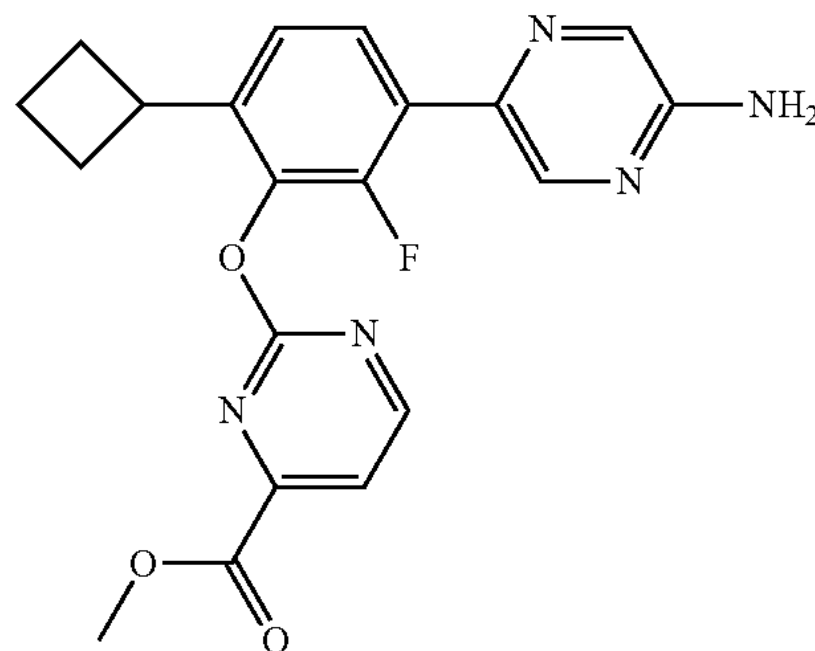
Methyl 2-[3-(5-aminopyrazin-2-yl)-6-cyclobutyl-2-fluorophenoxy]pyrimidine-4-carboxylate trifluoroacetate salt
