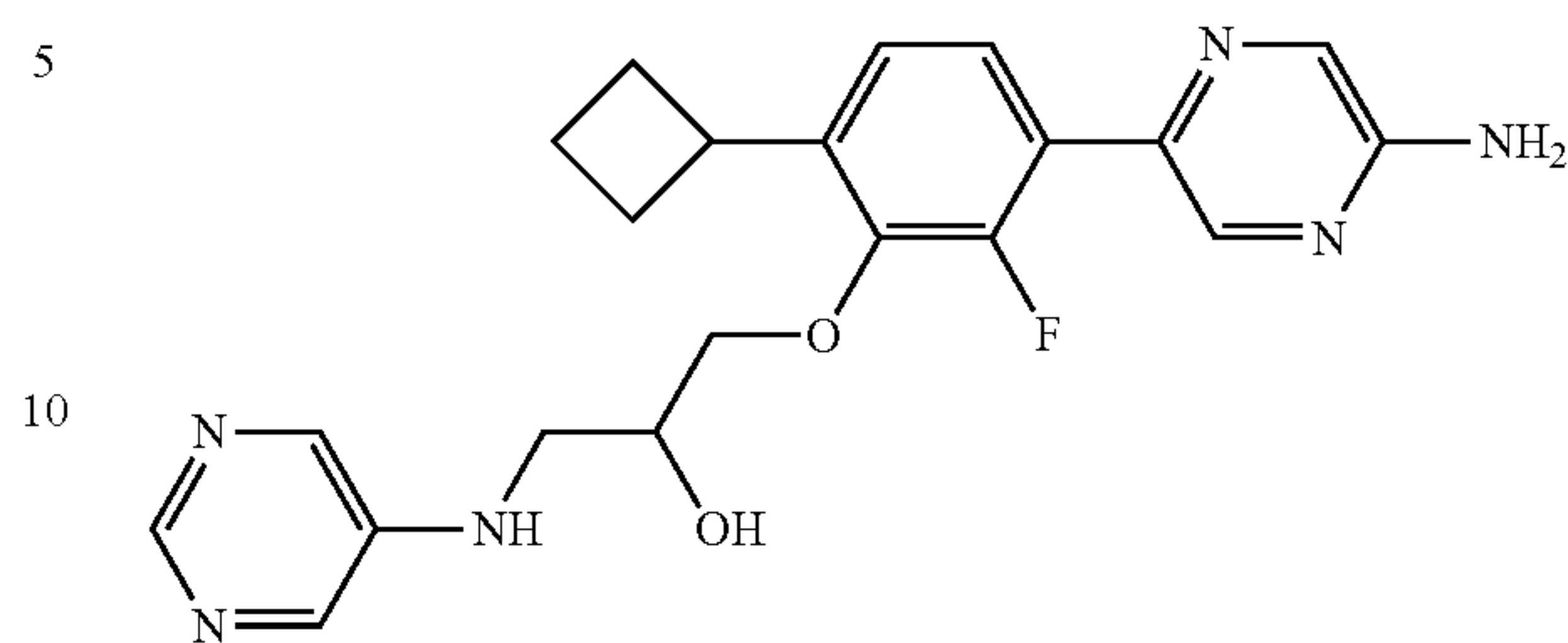
racemic 1-(3-(3-(5-Aminopyrazin-2-yl)-6-cyclobutyl-2-fluorophenoxy)-3-(pyrimidin-5-ylamino)propan-2-ol
