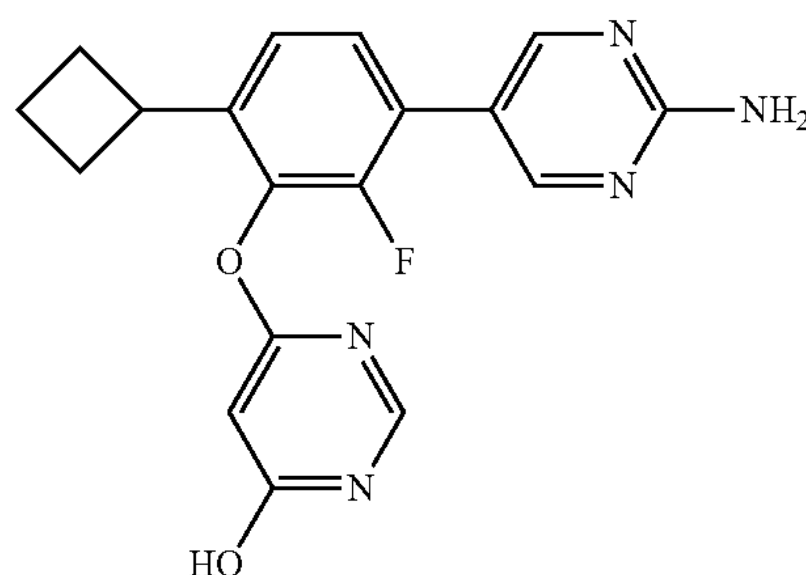
6-[3-(2-Aminopyrimidin-5-yl)-6-cyclobutyl-2-fluorophenoxy]pyrimidin-4-ol trifluoroacetate salt
