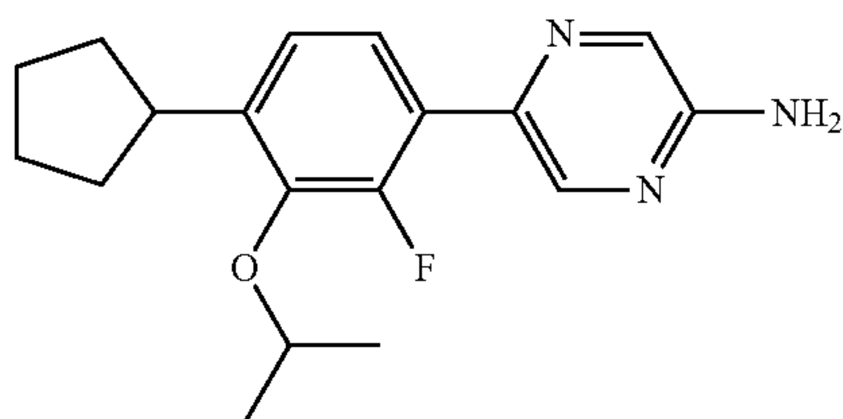
5-[4-Cyclopentyl-2-fluoro-3-(1-methylethoxy)phenyl] pyrazin-2-amine
