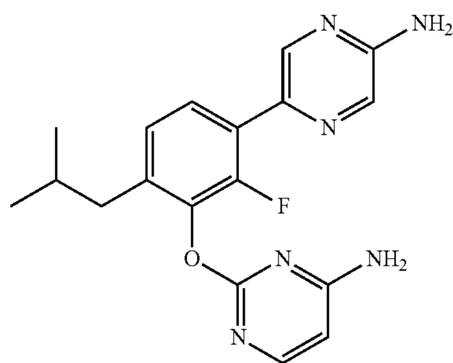
2-(3-(5-Aminopyrazin-2-yl)-2-fluoro-6-isobutylphenoxy)pyrimidin-4-amine
