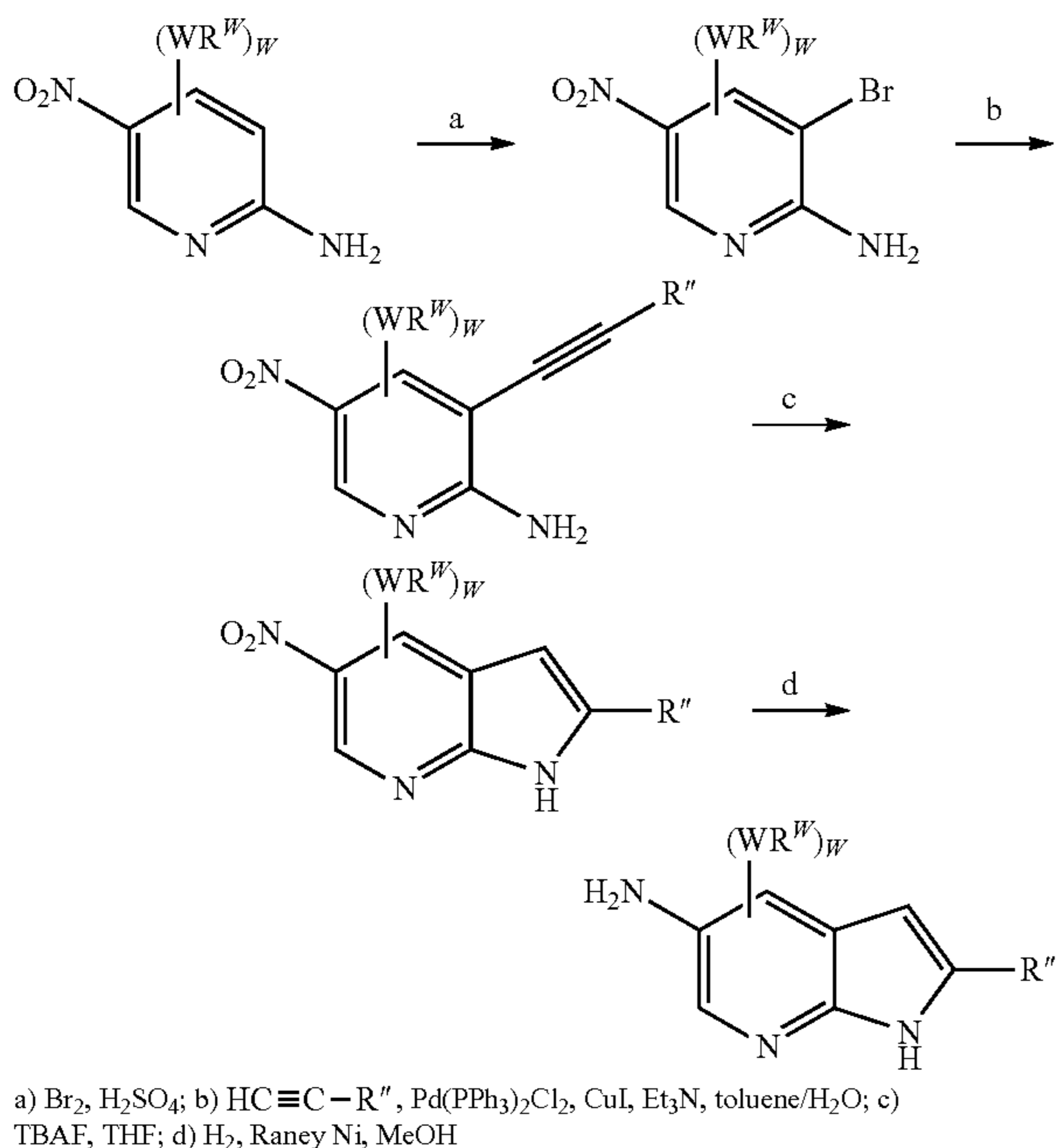
Scheme VIII
