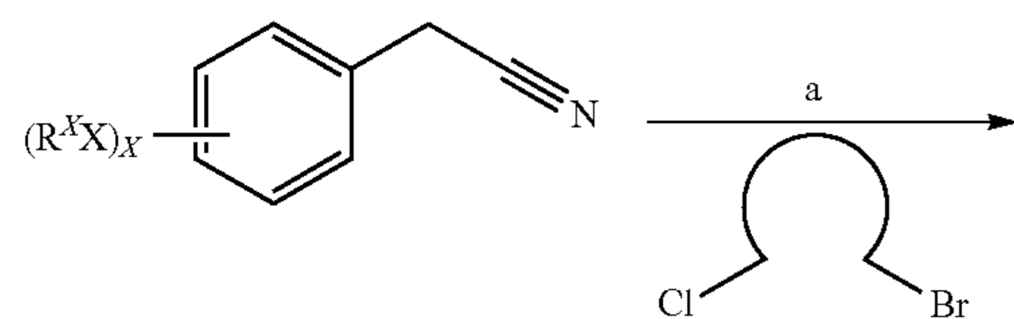
Scheme III
