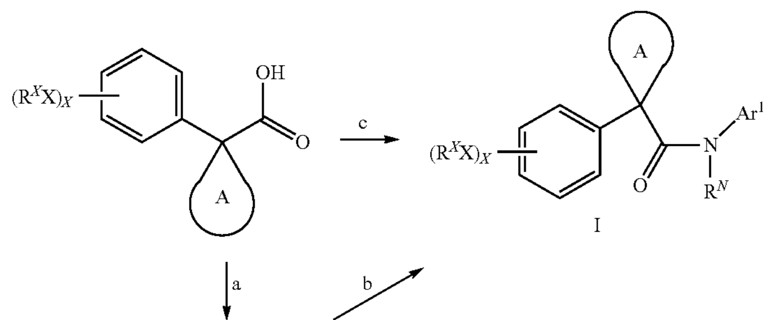
Scheme I
