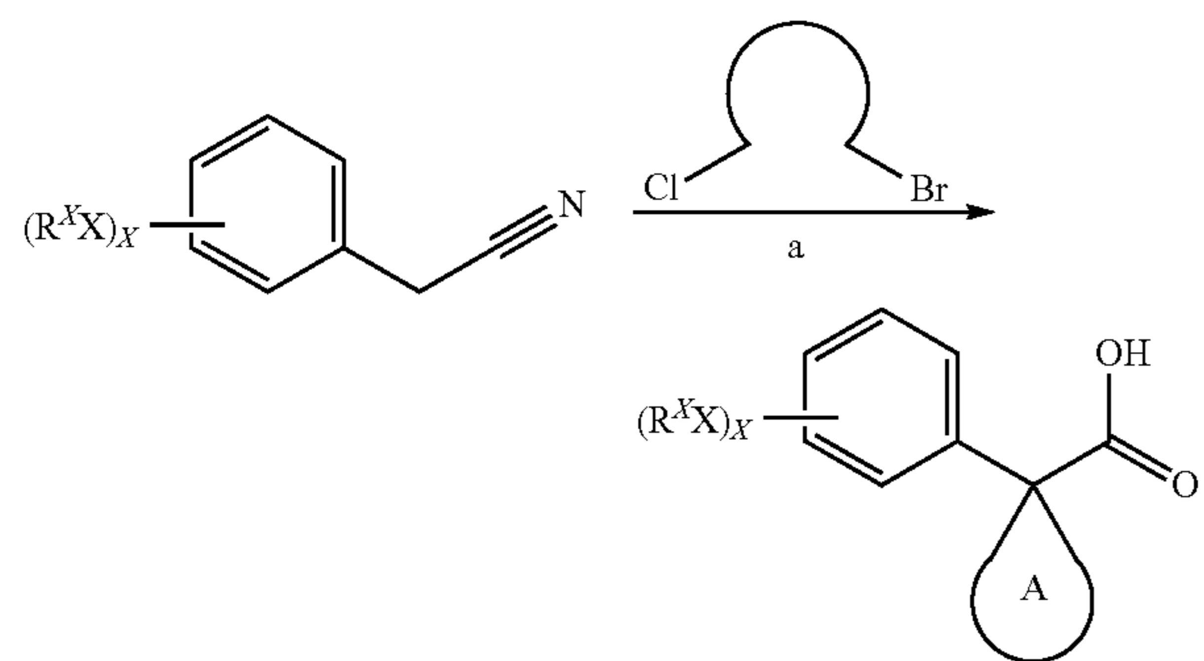
Scheme II
