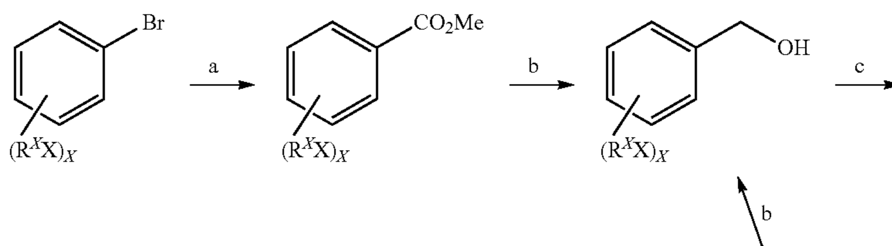
Scheme IV
