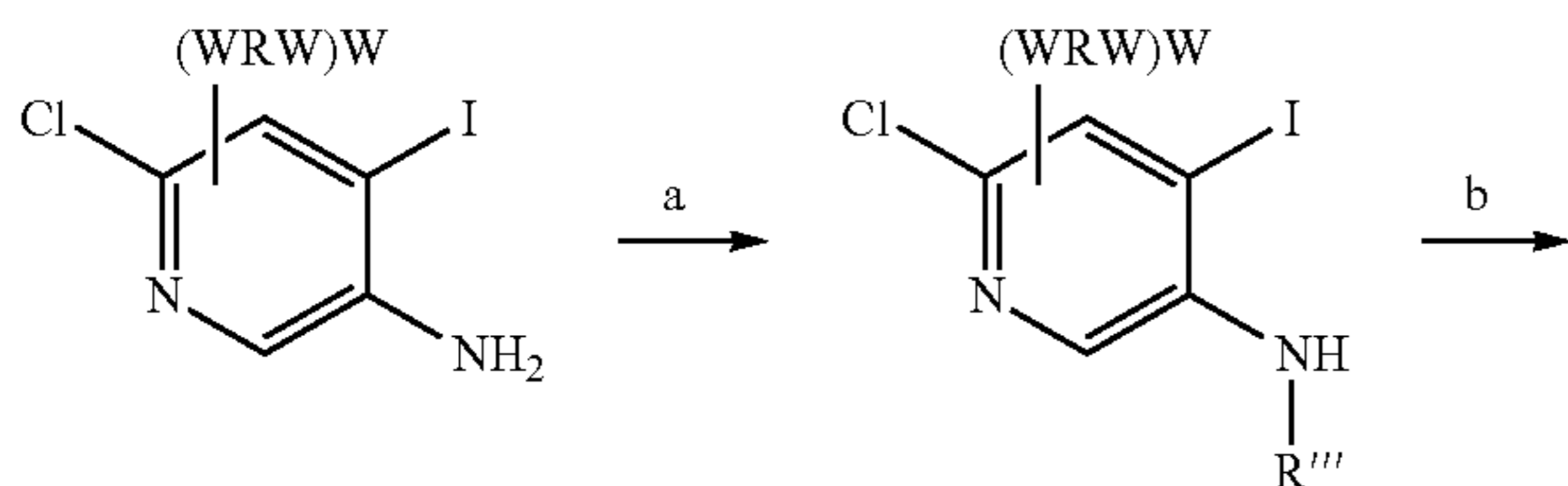
Scheme IX
