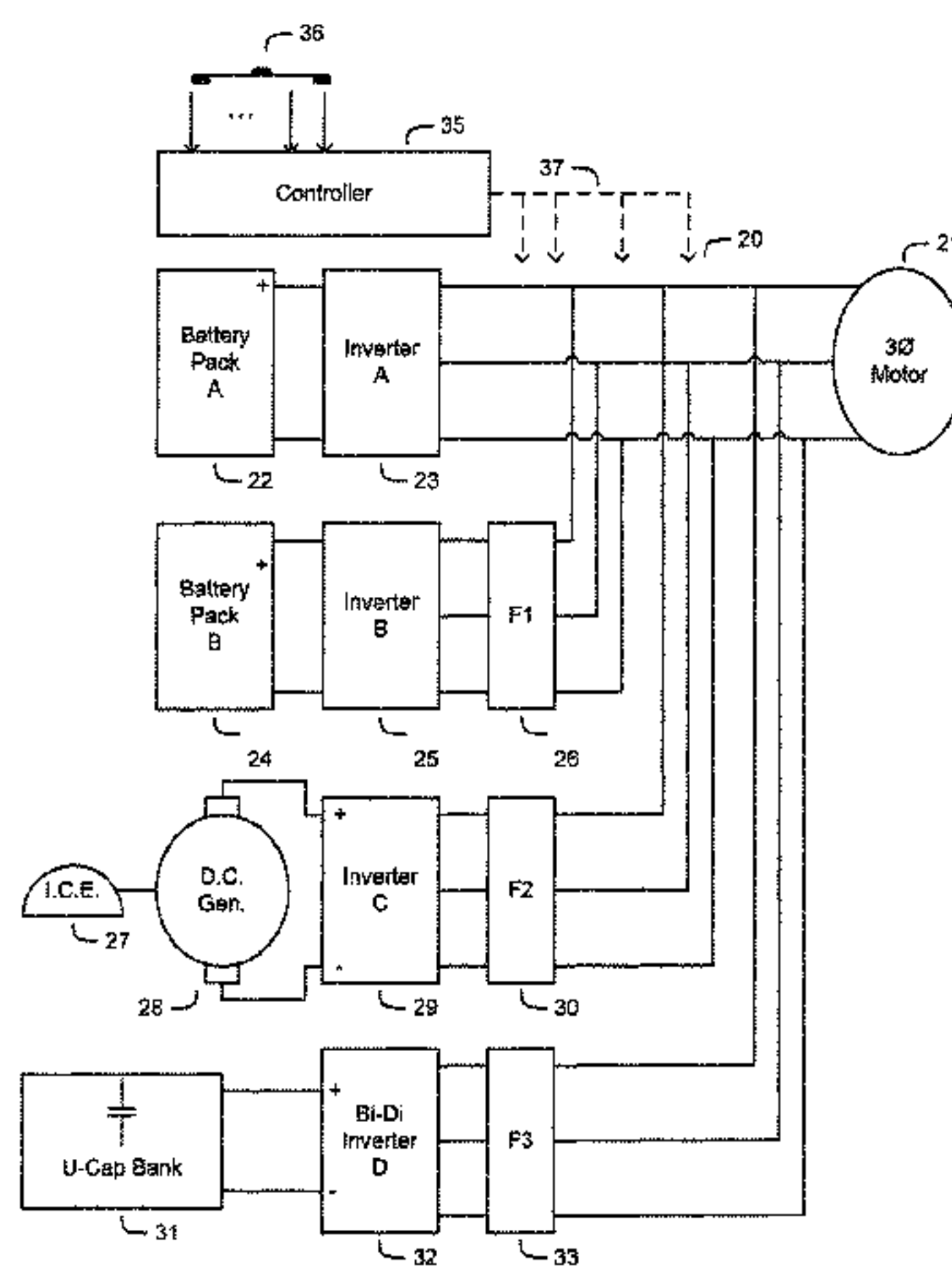
Multiple DC Sources and AC Motor
