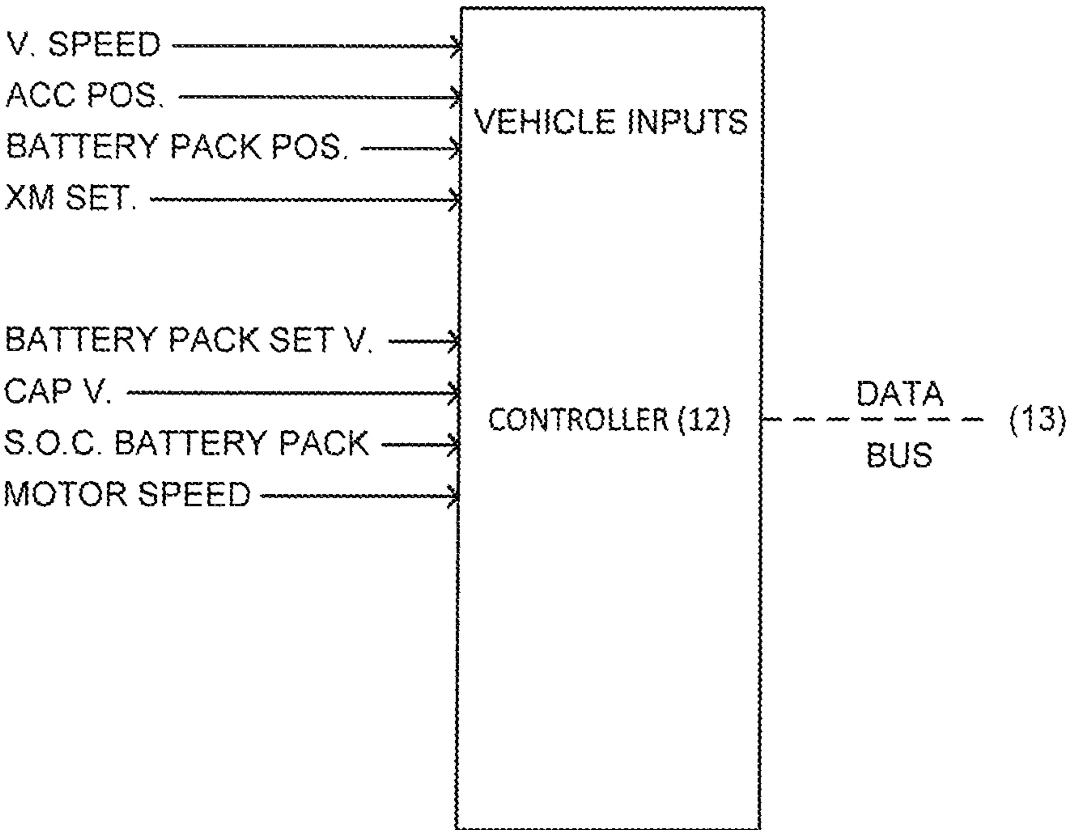
Figure 4: Vehicle Controller
