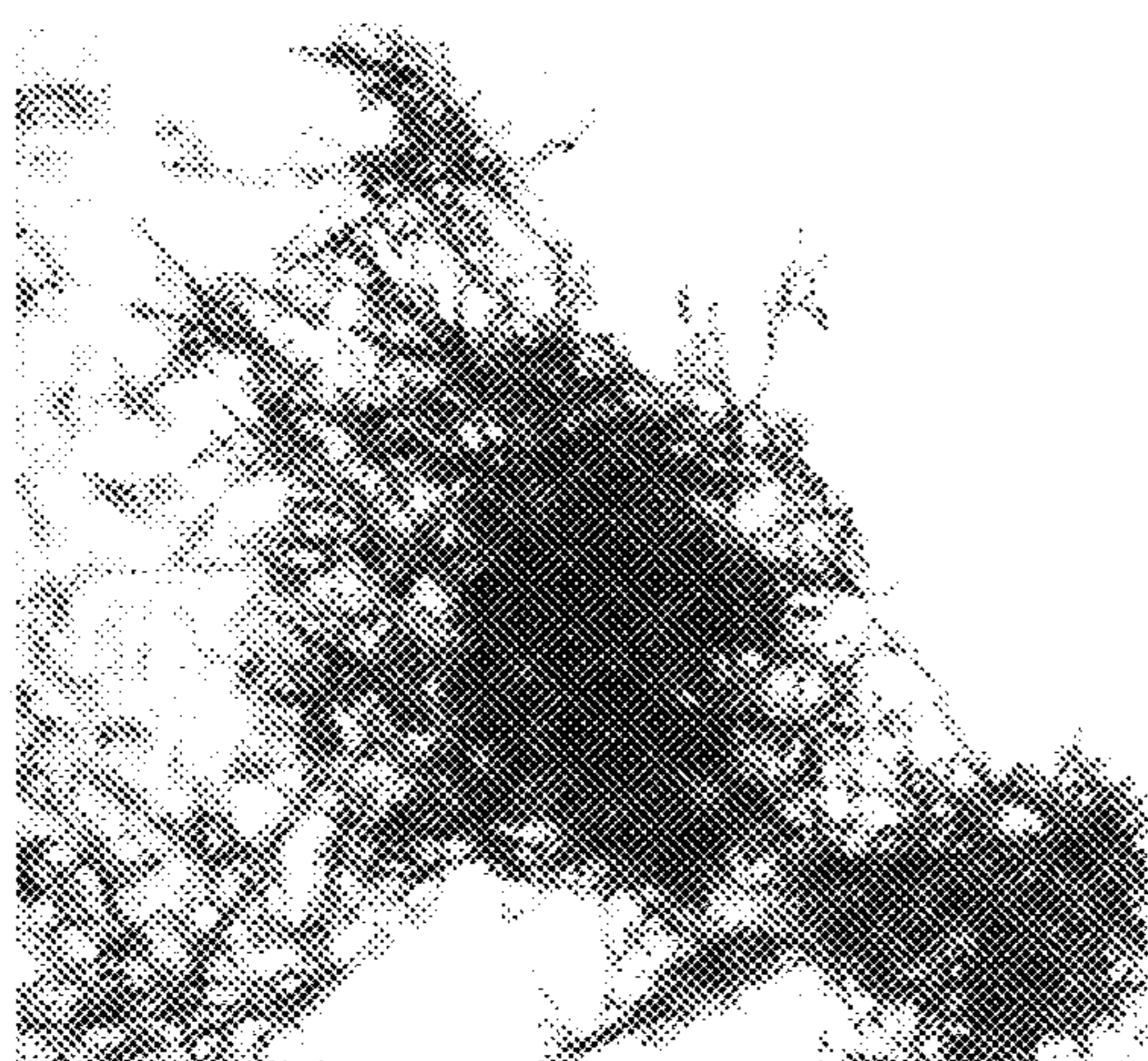
Crystal Form 1
