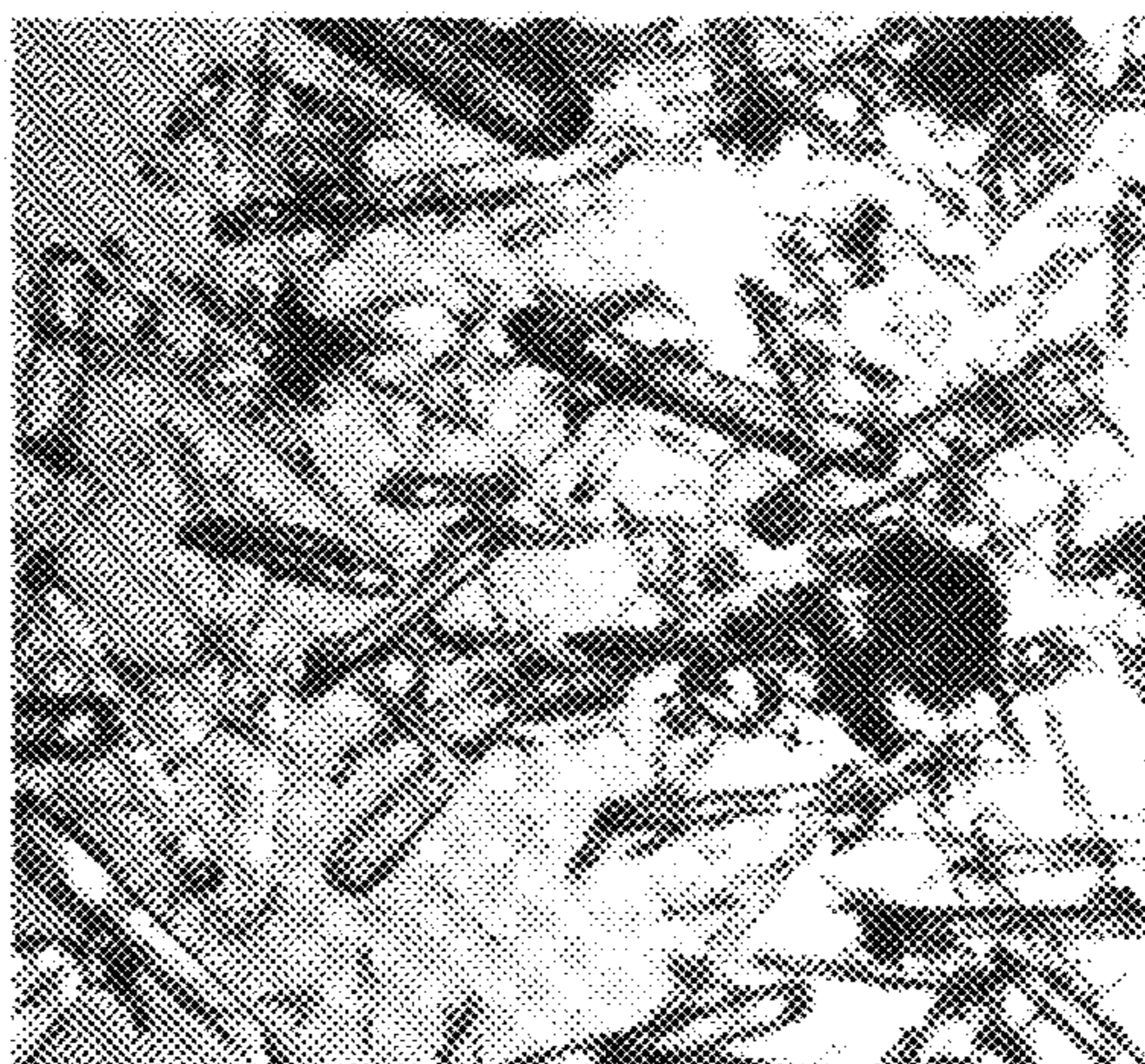
Crystal Form 3
