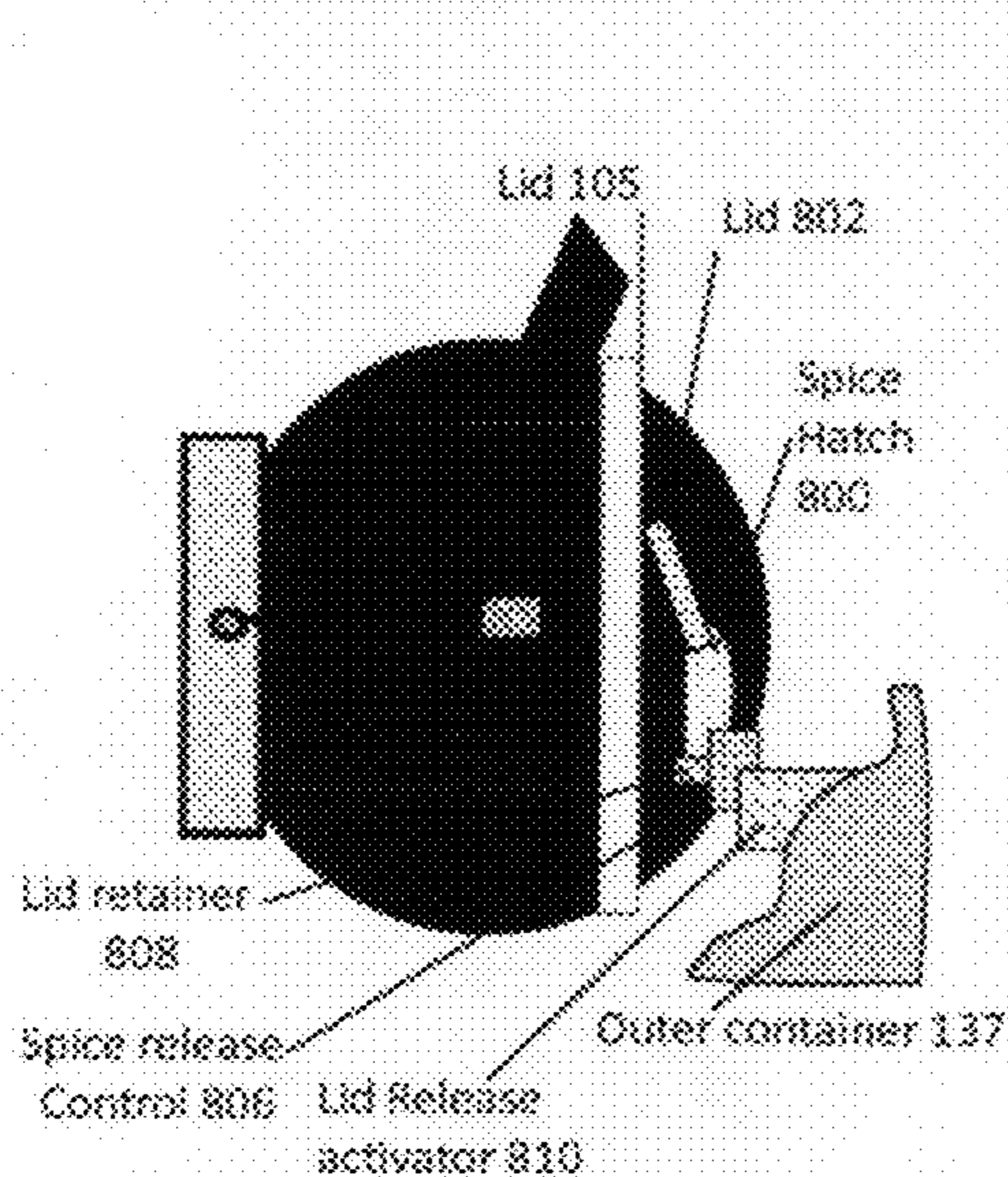
FIG. 8c: SIDE VIEW, Spice hatch release
