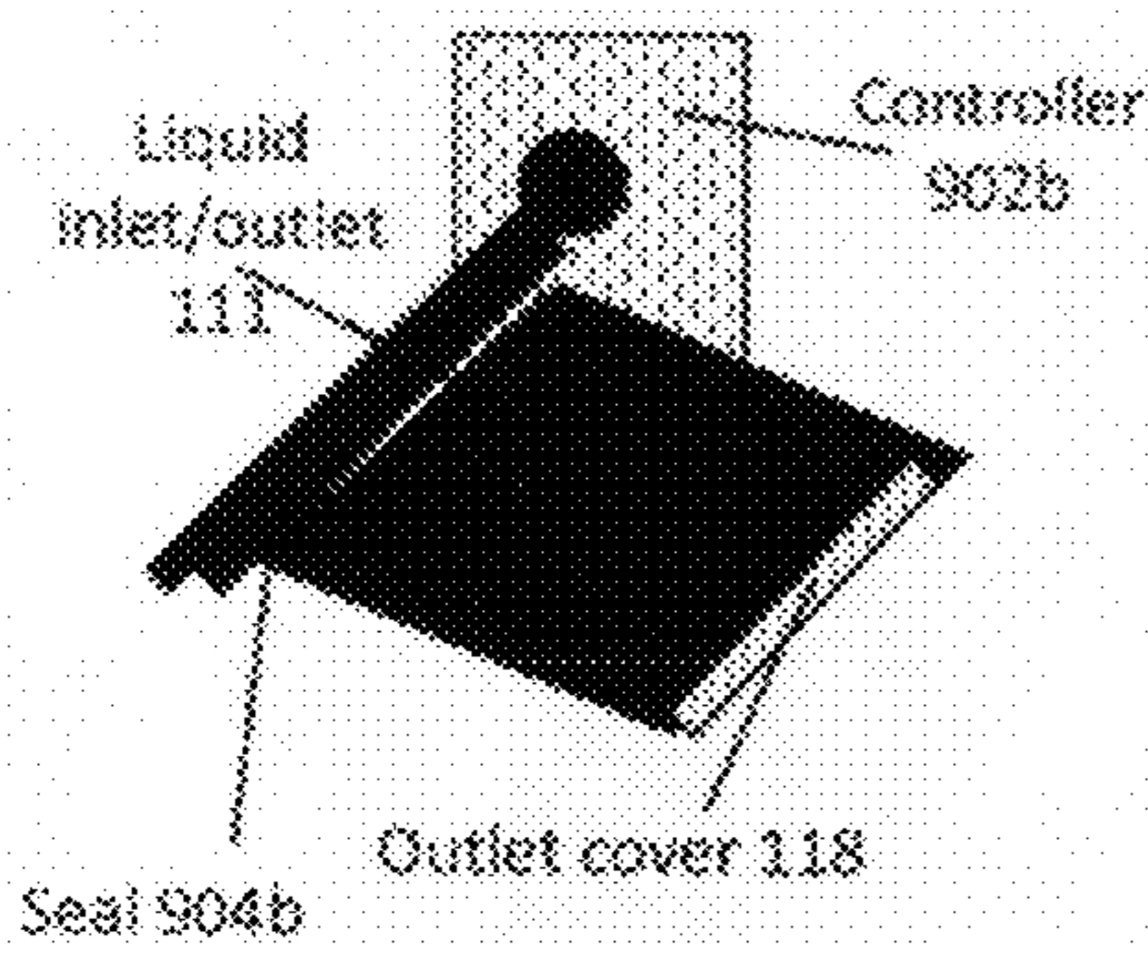
FIG. 9c: Inlet/Outlet valve closed
