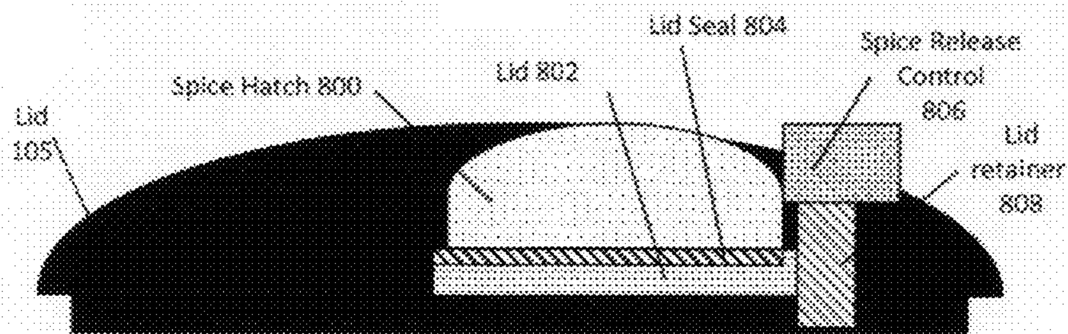
FIG. 8a: SIDE VIEW, Single Spice Hatch
