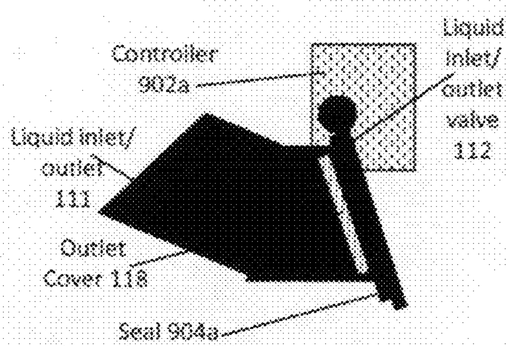
FIG. 9a: Inlet/Outlet valve closed
