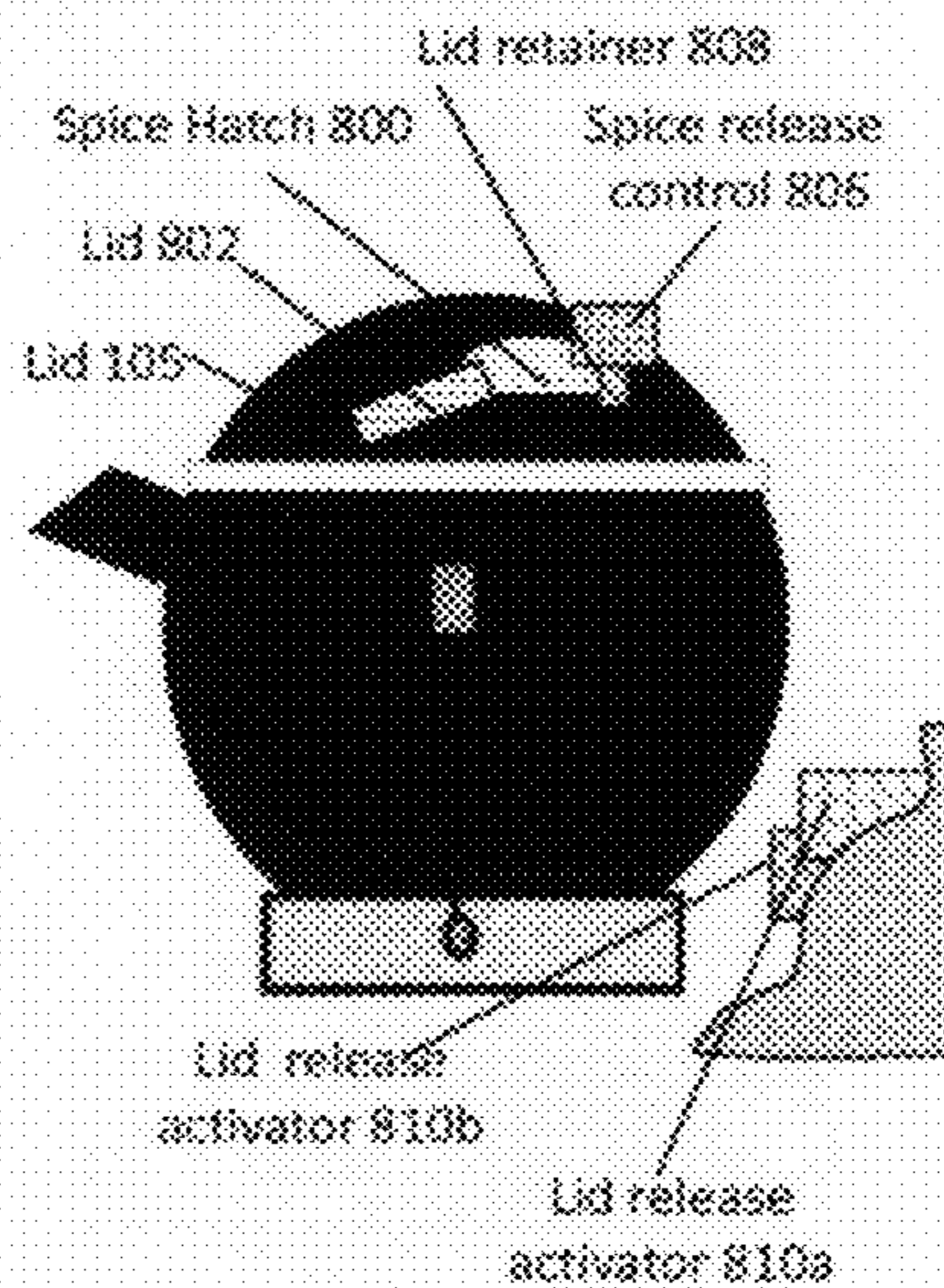
FIG. 8d: SIDE VIEW, After release
