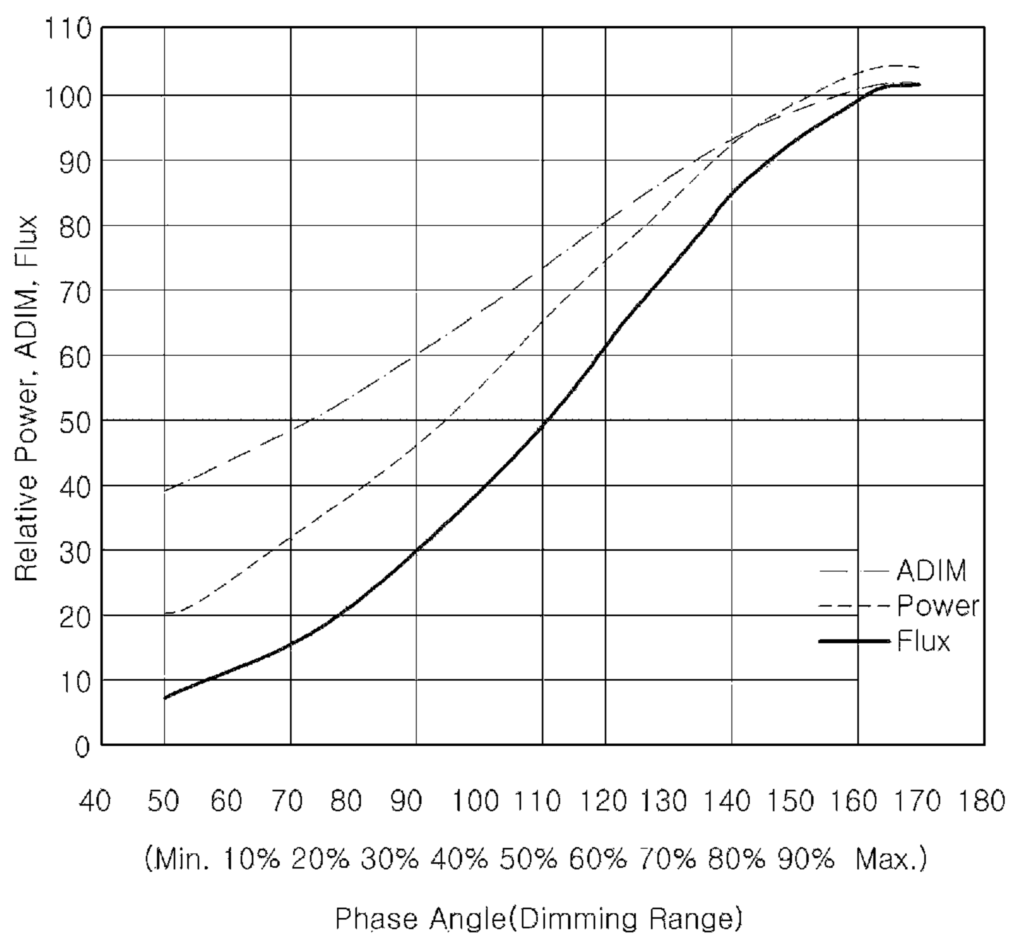
Dimming ADIM, Power, Flux Curve
