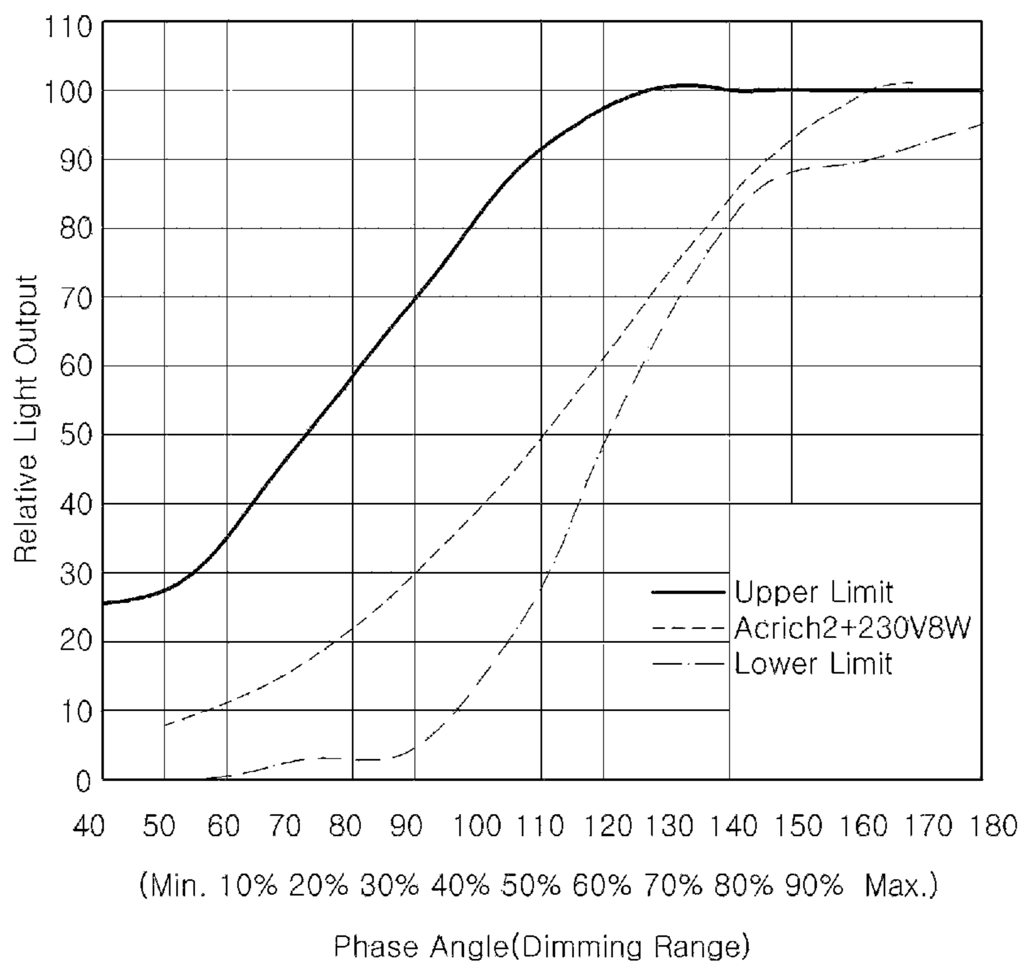
Dimming Light Output Curve
